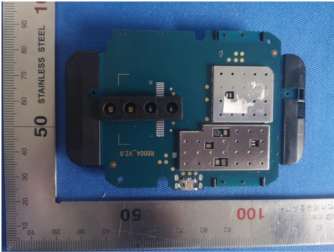
Internal 7 Main board back
