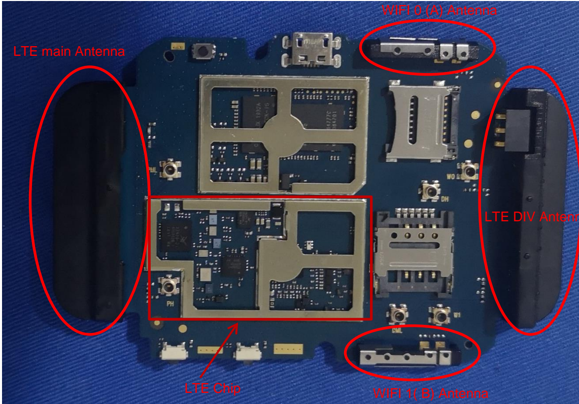
Internal 6 Main board face
