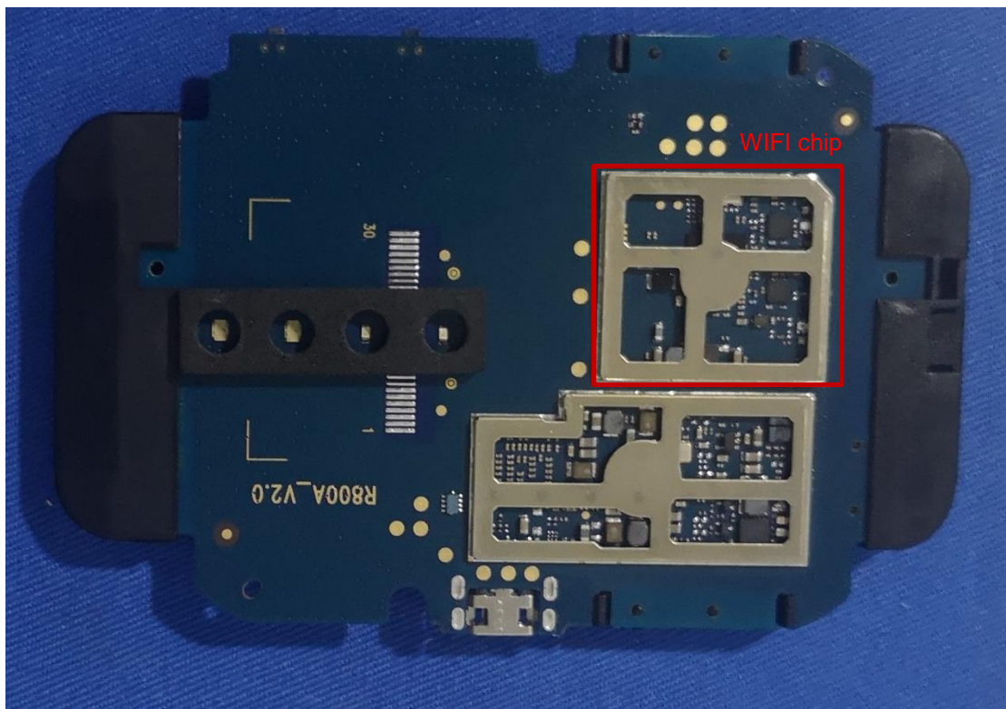
Internal 8 Main board back
