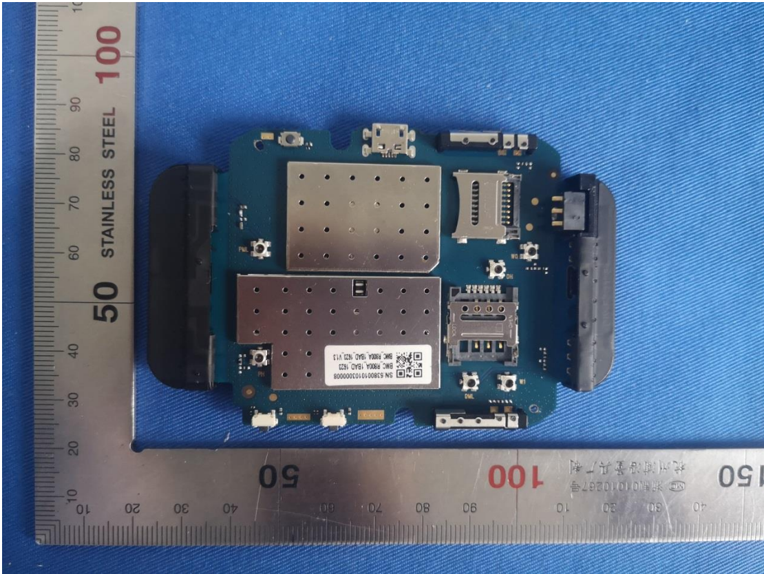
Internal 5-- Main board face
