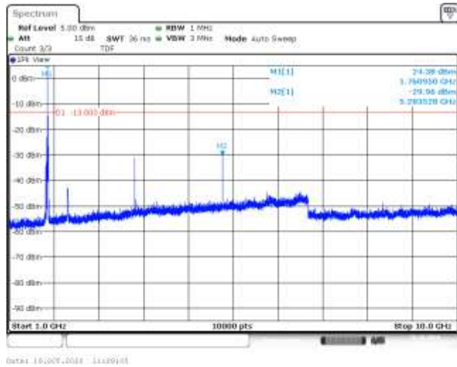
Band66-20MHz-16QAM-132572-1RB#0-Range2:1000~10000MHz--29.96-PASS
