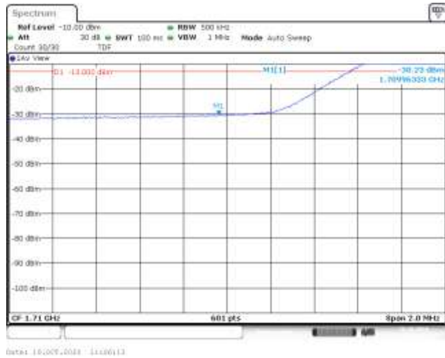
Band66-20MHz-16QAM-132072-100RB#0--30.23-PASS
