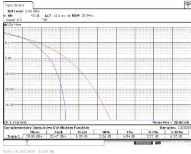
Band66-10MHz-16QAM-132022-50RB#0-5.71-13-PASS
