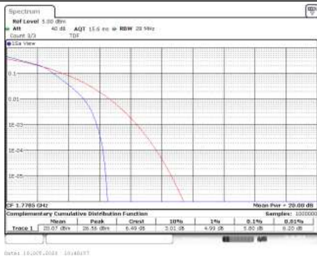
Band66-3MHz-16QAM-132657-15RB#0-5.80-13-PASS
