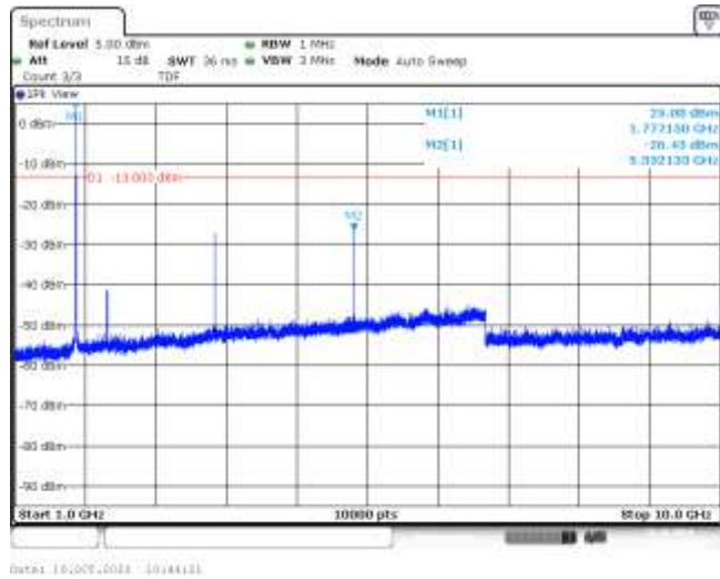
Band66-3MHz-16QAM-132657-1RB#0-Range2:1000~10000MHz--26.43-PASS
