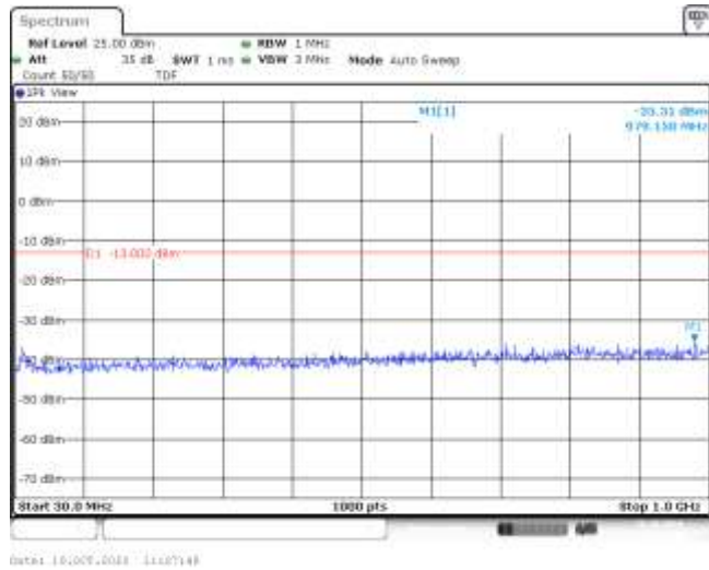
Band66-20MHz-QPSK-132322-1RB#0-Range1:30~1000MHz--35.31-PASS
