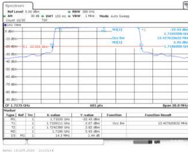
Band66-15MHz-QPSK-132047-75RB#0-13.428-14.300-PASS
