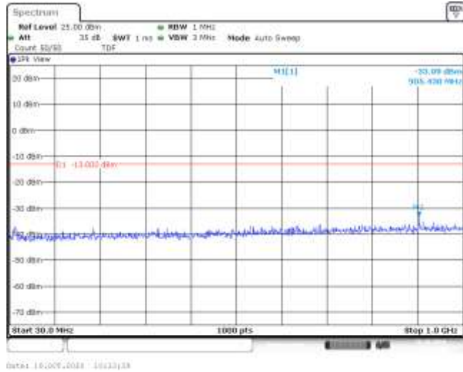
Band66-1.4MHz-16QAM-132665-1RB#0-Range1:30~1000MHz--33.09-PASS
