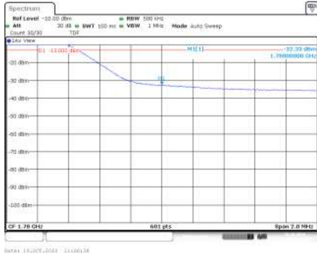
Band66-20MHz-QPSK-132572-100RB#0--32.33-PASS
