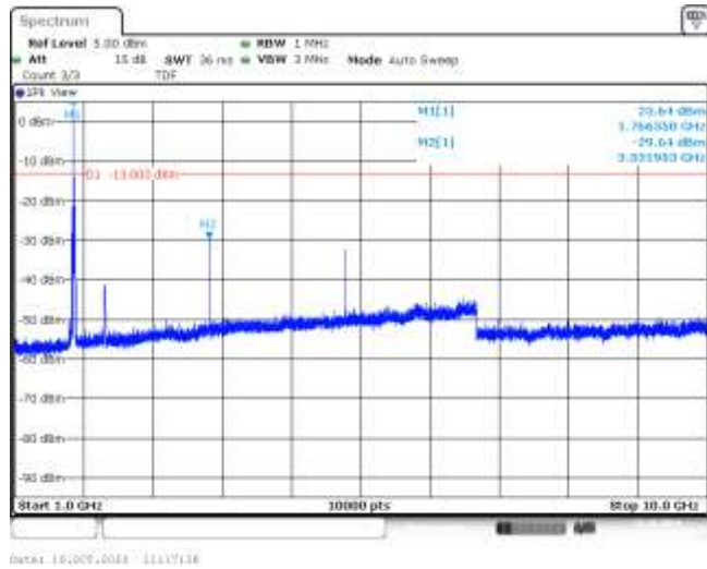
Band66-15MHz-16QAM-132597-1RB#0-Range2:1000~10000MHz--29.64-PASS
