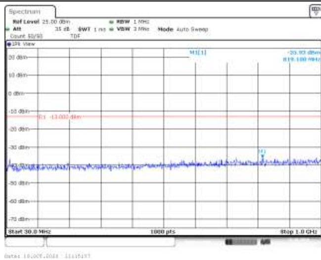
Band66-15MHz-16QAM-132047-1RB#0-Range1:30~1000MHz--35.93-PASS
