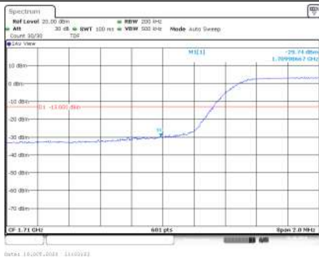
Band66-10MHz-16QAM-132022-50RB#0--29.74-PASS
