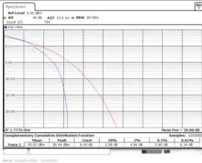
Band66-5MHz-16QAM-132647-25RB#0-5.80-13-PASS
