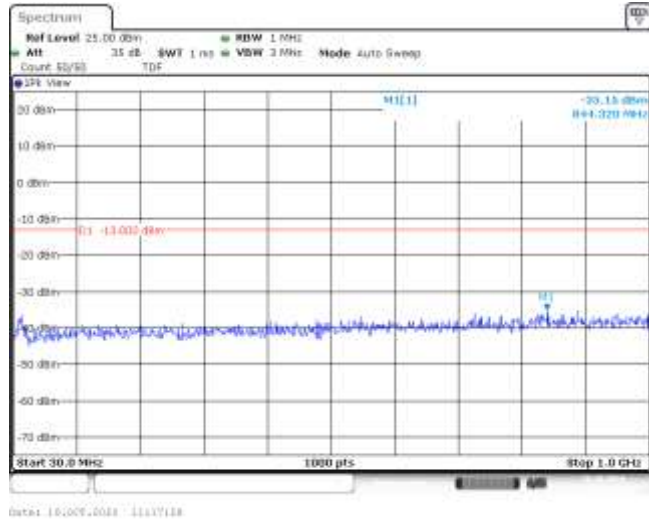
Band66-15MHz-16QAM-132597-1RB#0-Range1:30~1000MHz--35.15-PASS
