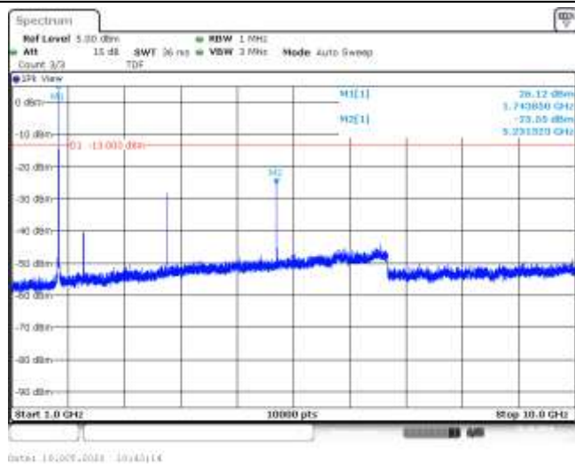
Band66-3MHz-QPSK-132322-1RB#0-Range2:1000~10000MHz--25.55-PASS
