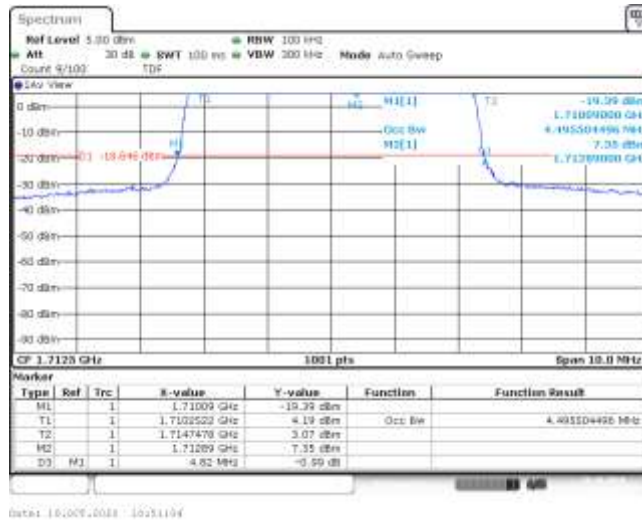
Band66-5MHz-QPSK-131997-25RB#0-4.496-4.820-PASS
