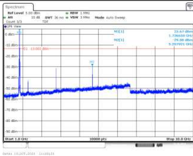
Band66-20MHz-16QAM-132322-1RB#0-Range2:1000~10000MHz--29.08-PASS
