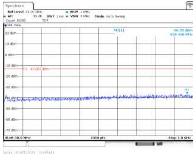
Band66-10MHz-16QAM-132322-1RB#0-Range1:30~1000MHz--36.2-PASS
