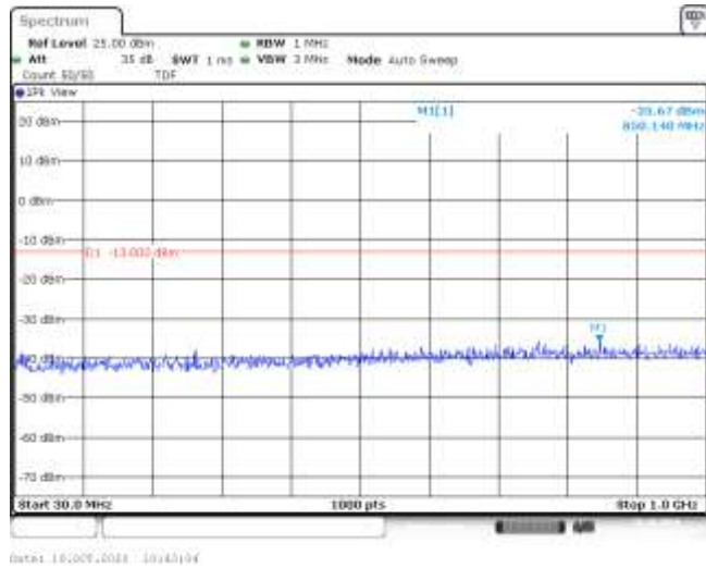
Band66-3MHz-QPSK-132322-1RB#0-Range1:30~1000MHz--35.67-PASS
