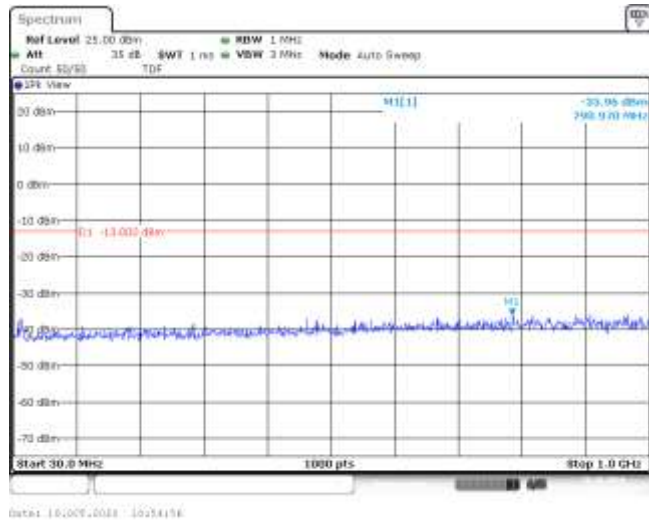
Band66-5MHz-QPSK-132322-1RB#0-Range1:30~1000MHz--35.96-PASS
