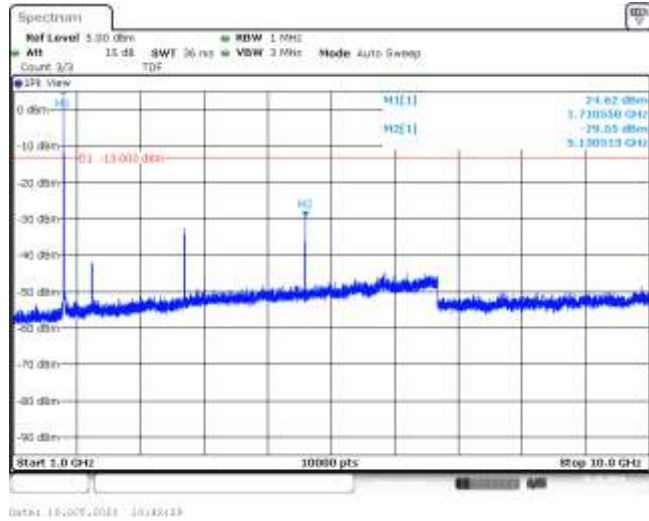
Band66-3MHz-QPSK-131987-1RB#0-Range2:1000~10000MHz--29.55-PASS
