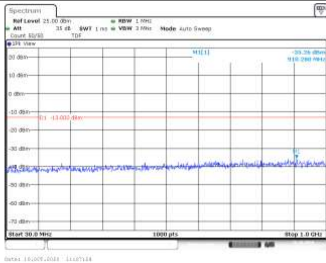
Band66-20MHz-16QAM-132072-1RB#0-Range1:30~1000MHz--35.26-PASS
