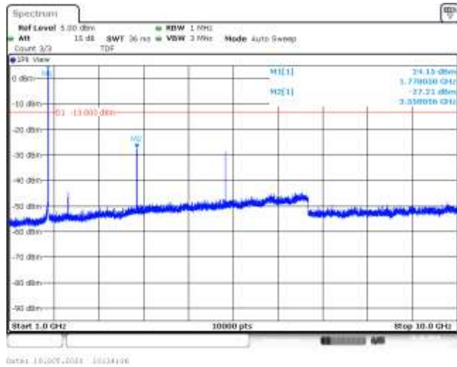
Band66-1.4MHz-16QAM-132665-1RB#0-Range2:1000~10000MHz--27.21-PASS
