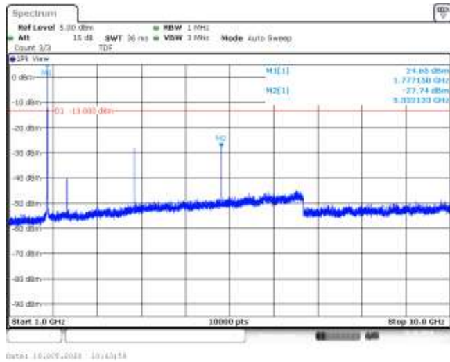
Band66-3MHz-QPSK-132657-1RB#0-Range2:1000~10000MHz--27.74-PASS
