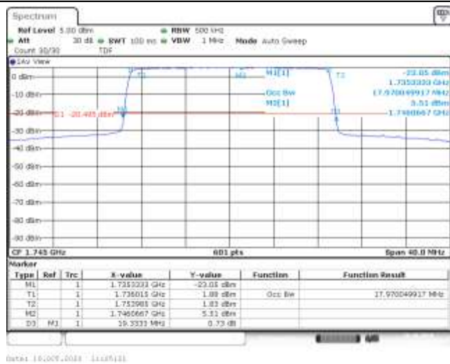
Band66-20MHz-16QAM-132322-100RB#0-17.97-19.333-PASS
