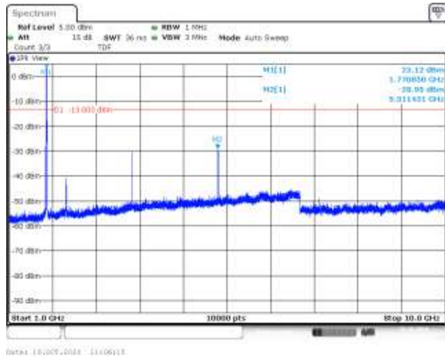
Band66-10MHz-16QAM-132622-1RB#0-Range2:1000~10000MHz--28.95-PASS
