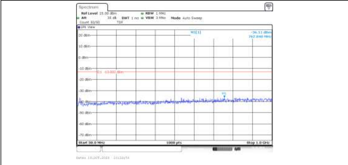
Band66-1.4MHz-16QAM-132322-1RB#0-Range1:30~1000MHz--36.11-PASS
