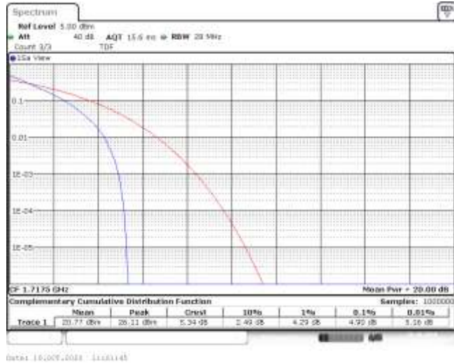
Band66-15MHz-QPSK-132047-75RB#0-4.90-13-PASS
