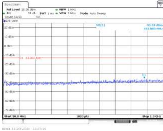
Band66-15MHz-QPSK-132597-1RB#0-Range1:30~1000MHz--35.59-PASS
