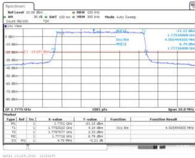
Band66-5MHz-16QAM-132647-25RB#0-4.505-4.790-PASS
