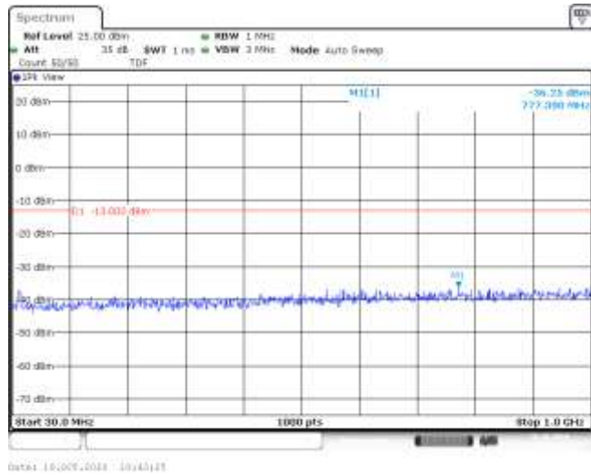
Band66-3MHz-16QAM-132322-1RB#0-Range1:30~1000MHz--36.25-PASS
