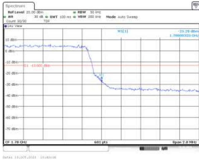
Band66-3MHz-16QAM-132657-15RB#0--25.28-PASS
