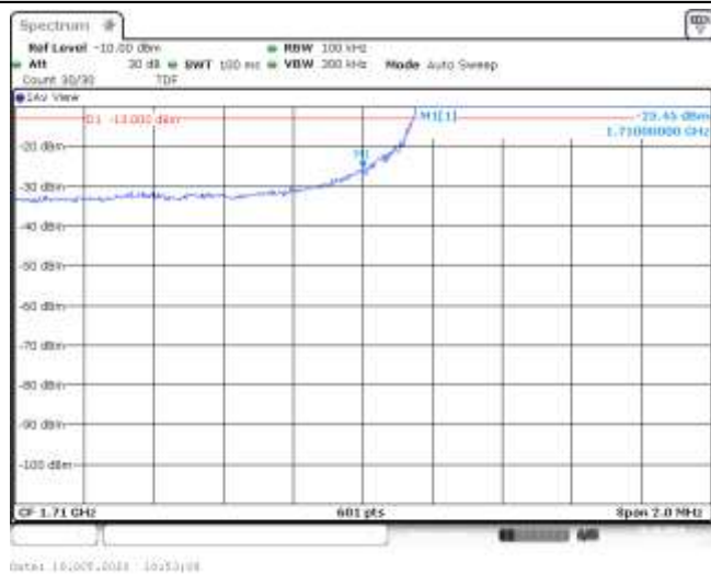
Band66-5MHz-QPSK-131997-25RB#0--25.45-PASS
