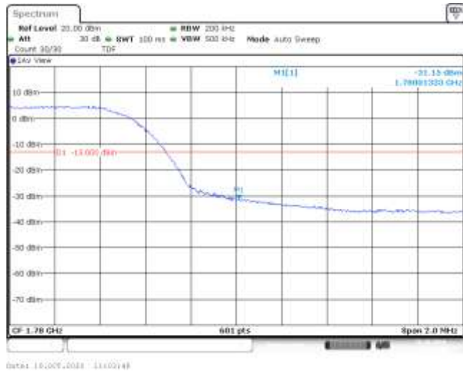
Band66-10MHz-QPSK-132622-50RB#0--31.15-PASS
