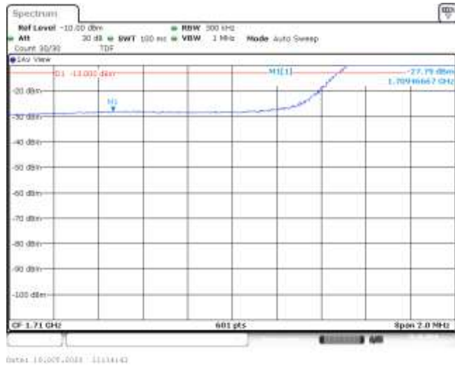
Band66-15MHz-QPSK-132047-75RB#0--27.79-PASS
