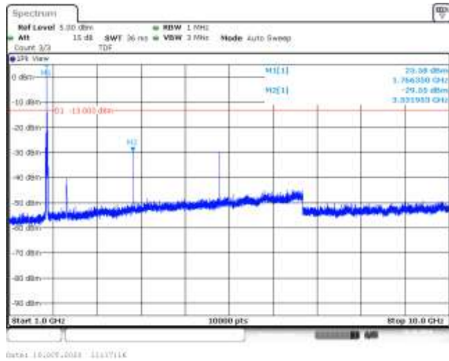
Band66-15MHz-QPSK-132597-1RB#0-Range2:1000~10000MHz--29.55-PASS
