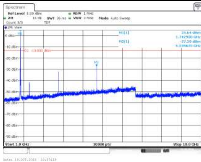
Band66-5MHz-16QAM-132322-1RB#0-Range2:1000~10000MHz--27.2-PASS
