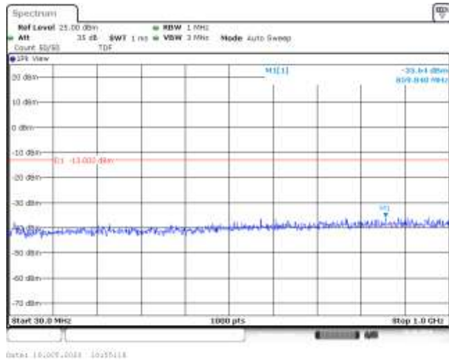
Band66-5MHz-16QAM-132322-1RB#0-Range1:30~1000MHz--35.64-PASS
