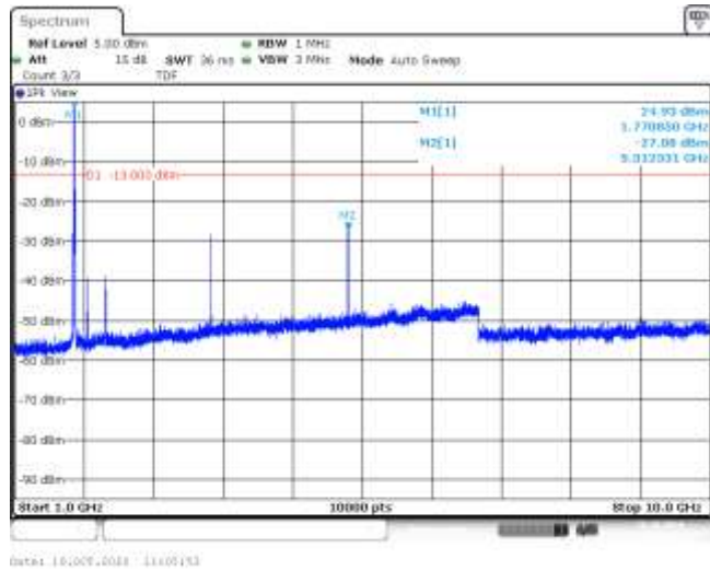
Band66-10MHz-QPSK-132622-1RB#0-Range2:1000~10000MHz--27.08-PASS
