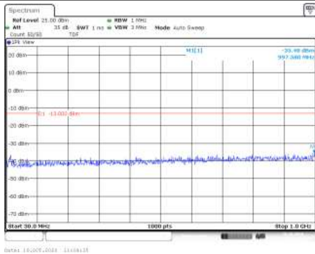
Band66-10MHz-16QAM-132022-1RB#0-Range1:30~1000MHz--35.48-PASS
