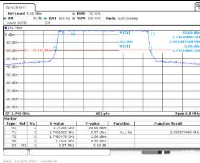
Band66-3MHz-16QAM-132322-15RB#0-2.696-2.870-PASS
