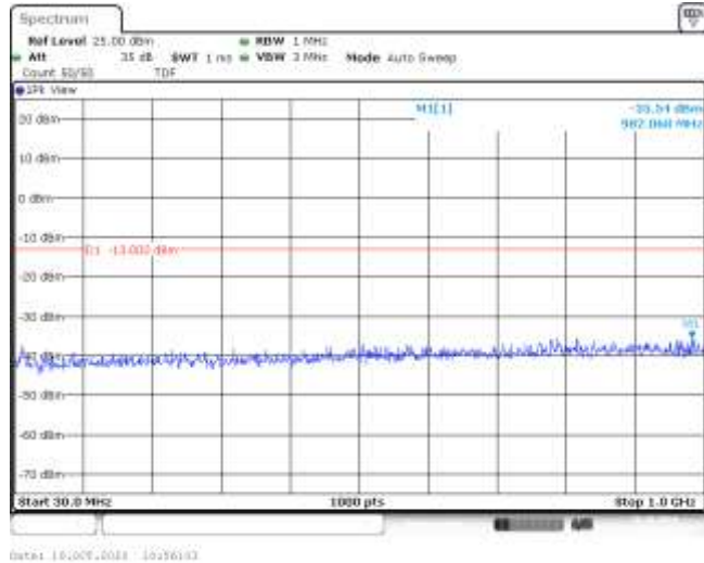
Band66-5MHz-16QAM-132647-1RB#0-Range1:30~1000MHz--35.54-PASS
