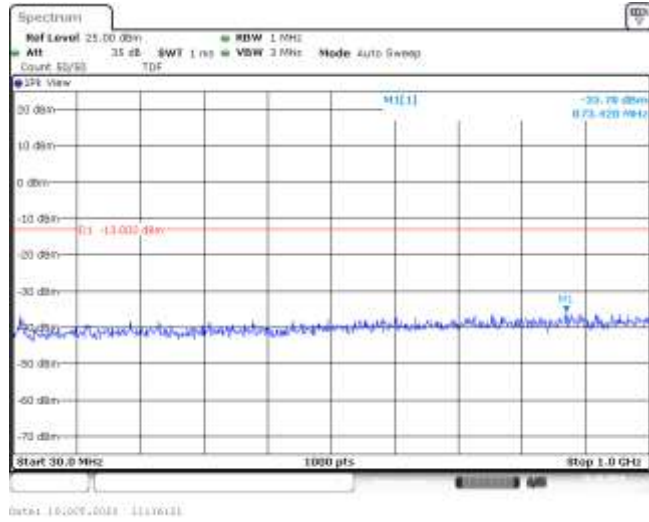
Band66-15MHz-QPSK-132322-1RB#0-Range1:30~1000MHz--35.78-PASS
