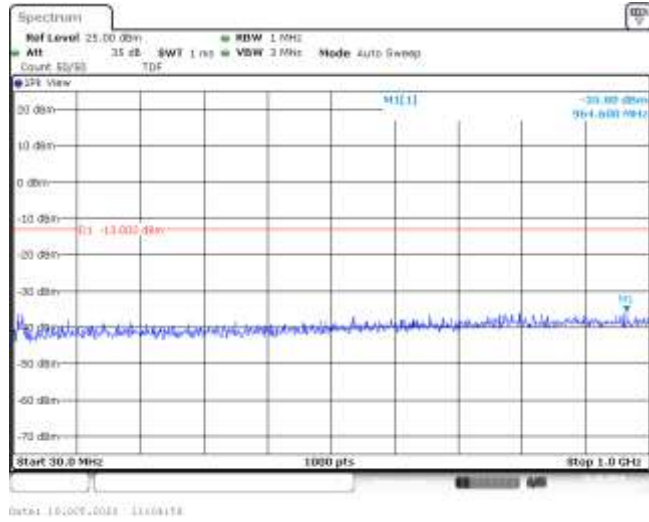
Band66-10MHz-QPSK-132322-1RB#0-Range1:30~1000MHz--35.8-PASS
