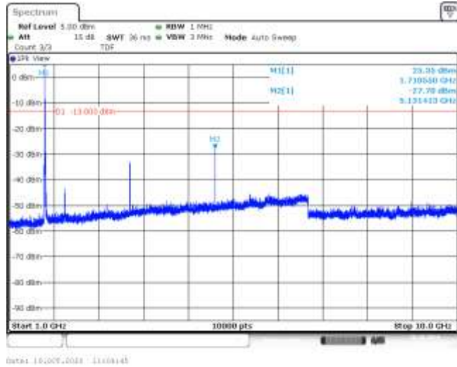
Band66-10MHz-16QAM-132022-1RB#0-Range2:1000~10000MHz--27.7-PASS
