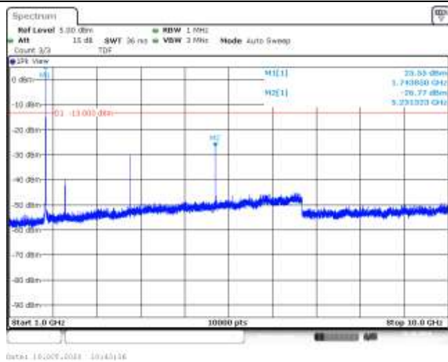
Band66-3MHz-16QAM-132322-1RB#0-Range2:1000~10000MHz--26.77-PASS
