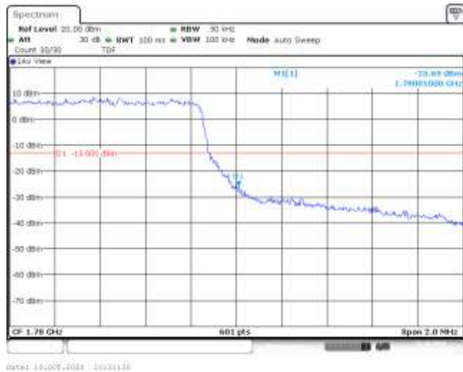
Band66-1.4MHz-16QAM-132665-6RB#0--25.69-PASS
