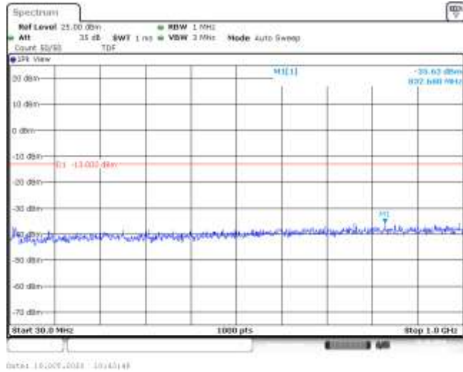
Band66-3MHz-QPSK-132657-1RB#0-Range1:30~1000MHz--35.63-PASS
