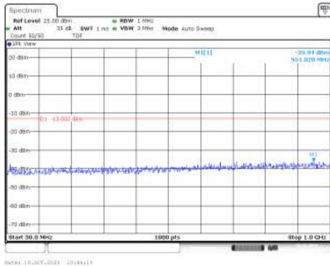
Band66-3MHz-16QAM-132657-1RB#0-Range1:30~1000MHz--35.94-PASS
