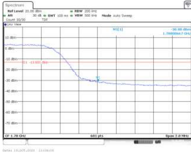
Band66-10MHz-16QAM-132622-50RB#0--30.88-PASS
