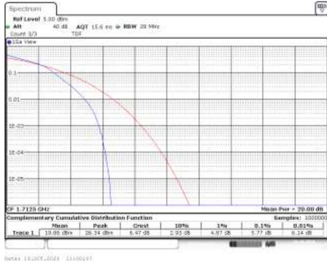
Band66-5MHz-16QAM-131997-25RB#0-5.77-13-PASS
