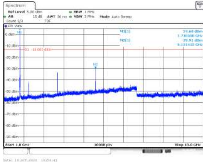
Band66-5MHz-16QAM-131997-1RB#0-Range2:1000~10000MHz--29.91-PASS
