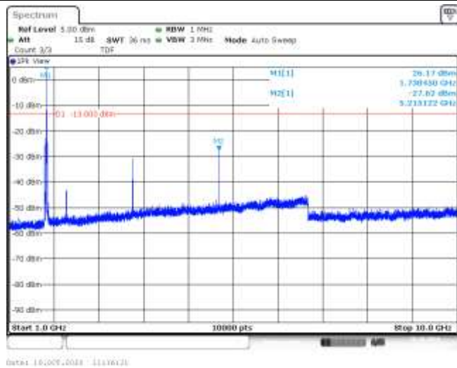
Band66-15MHz-QPSK-132322-1RB#0-Range2:1000~10000MHz--27.62-PASS
