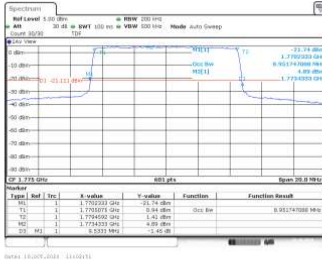
Band66-10MHz-16QAM-132622-50RB#0-8.952-9.533-PASS
