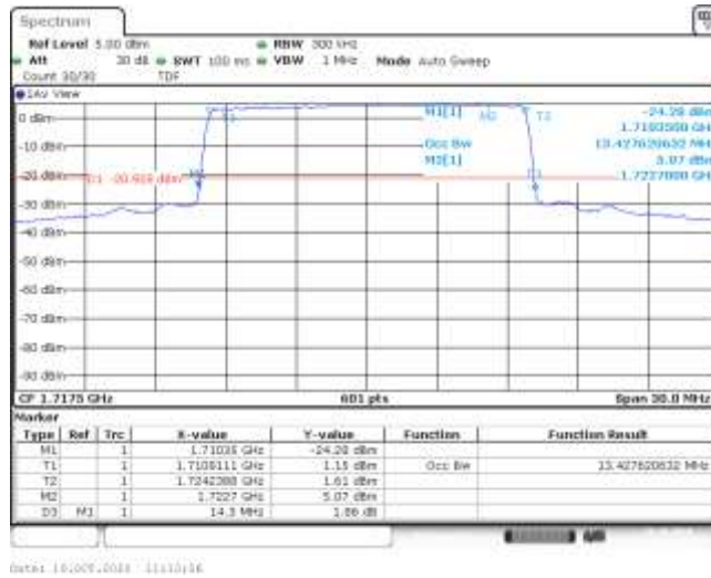
Band66-15MHz-16QAM-132047-75RB#0-13.428-14.300-PASS
