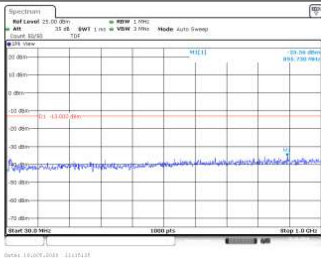
Band66-15MHz-QPSK-132047-1RB#0-Range1:30~1000MHz--35.56-PASS
