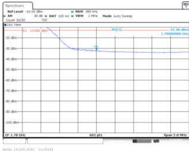
Band66-15MHz-16QAM-132597-75RB#0--31.96-PASS
