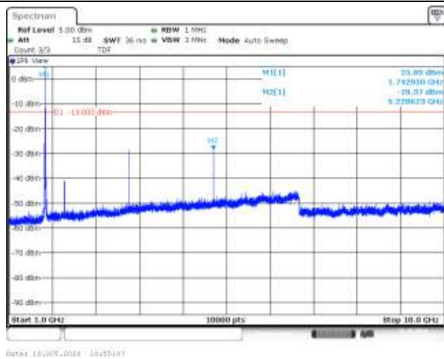
Band66-5MHz-QPSK-132322-1RB#0-Range2:1000~10000MHz--28.37-PASS
