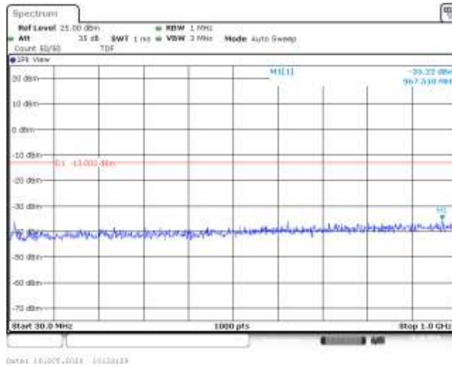
Band66-1.4MHz-QPSK-132322-1RB#0-Range1:30~1000MHz--35.22-PASS
