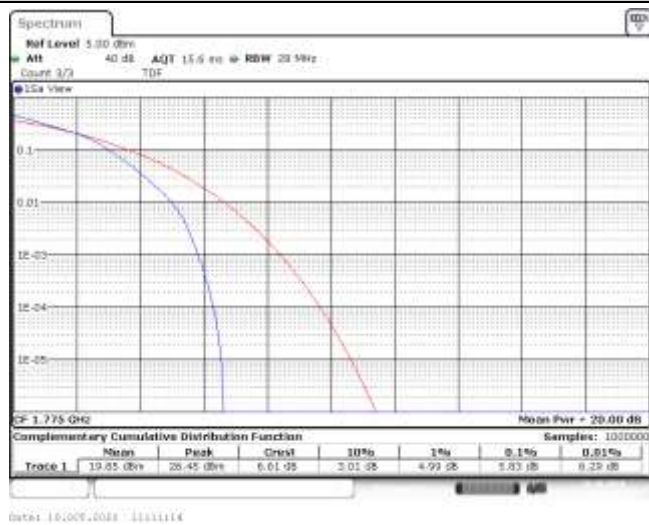
Band66-10MHz-16QAM-132622-50RB#0-5.83-13-PASS
