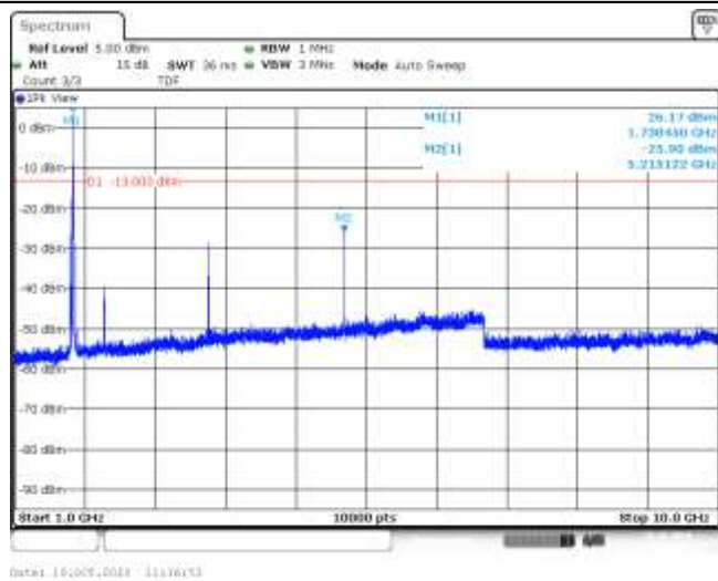
Band66-15MHz-16QAM-132322-1RB#0-Range2:1000~10000MHz--25.9-PASS
