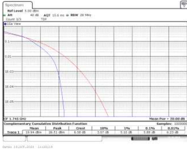
Band66-15MHz-16QAM-132322-75RB#0-5.88-13-PASS
