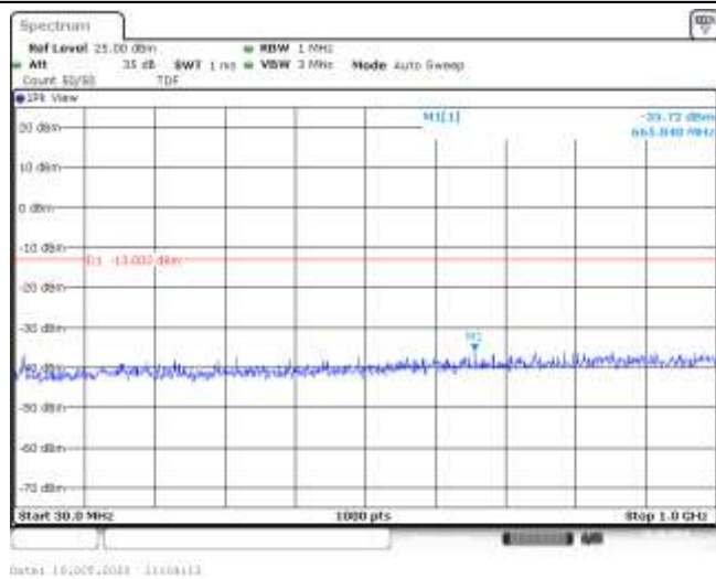
Band66-10MHz-QPSK-132022-1RB#0-Range1:30~1000MHz--35.72-PASS
