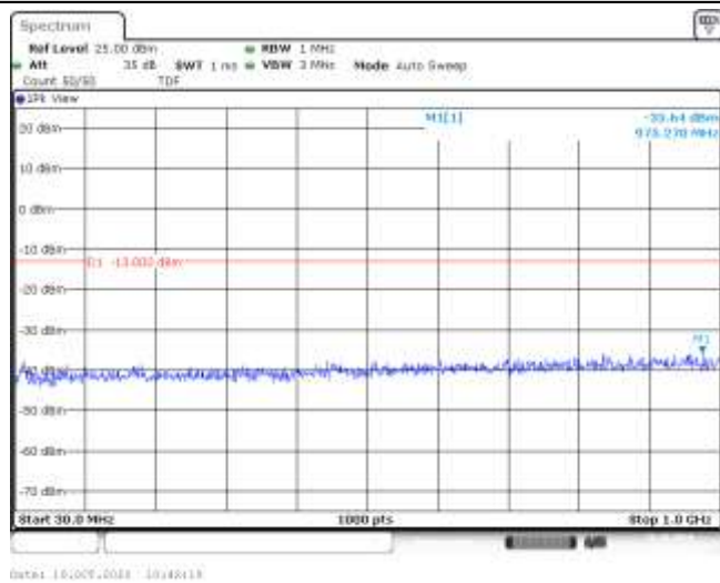
Band66-3MHz-QPSK-131987-1RB#0-Range1:30~1000MHz--35.64-PASS
