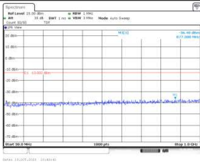
Band66-3MHz-16QAM-131987-1RB#0-Range1:30~1000MHz--36.4-PASS
