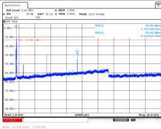
Band66-10MHz-QPSK-132322-1RB#0-Range2:1000~10000MHz--29.04-PASS
