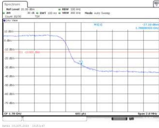
Band66-5MHz-QPSK-132647-25RB#0--27.10-PASS
