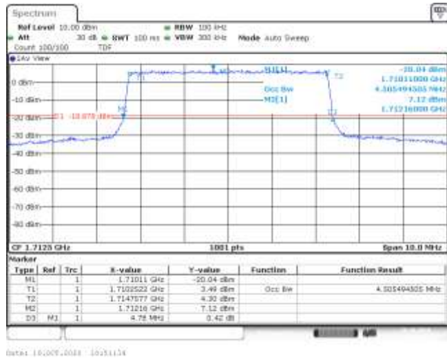
Band66-5MHz-16QAM-131997-25RB#0-4.505-4.780-PASS
