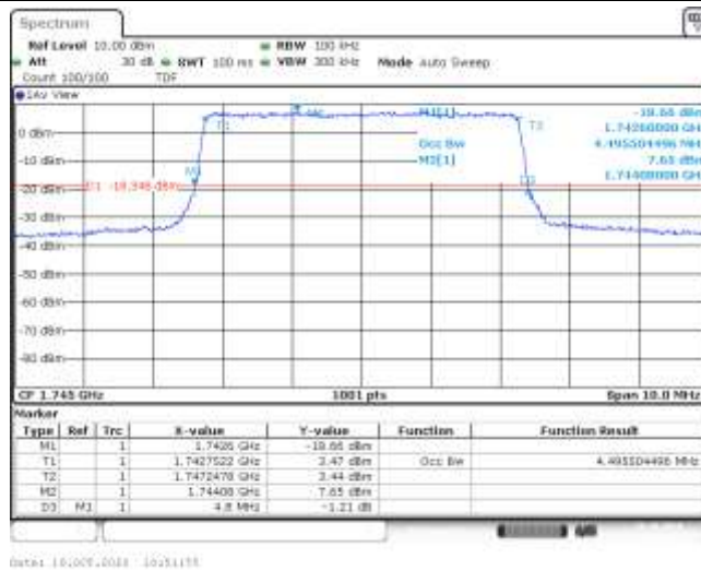
Band66-5MHz-QPSK-132322-25RB#0-4.496-4.800-PASS
