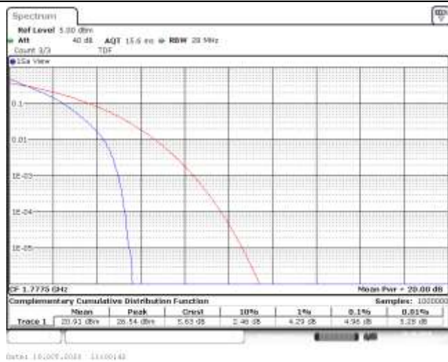
Band66-5MHz-QPSK-132647-25RB#0-4.96-13-PASS
