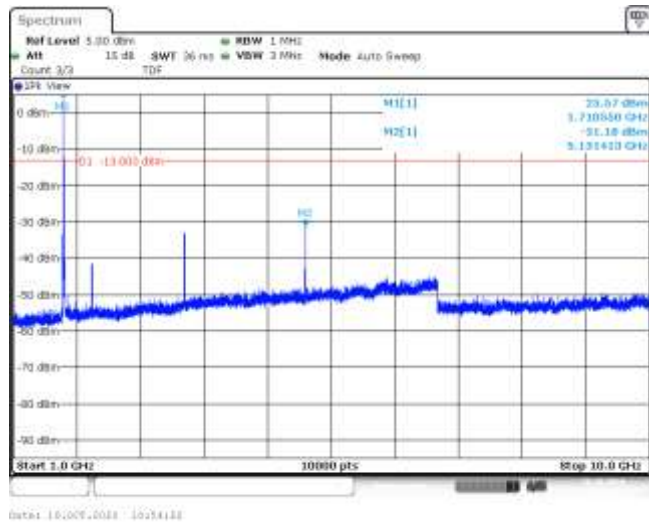
Band66-5MHz-QPSK-131997-1RB#0-Range2:1000~10000MHz--31.18-PASS
