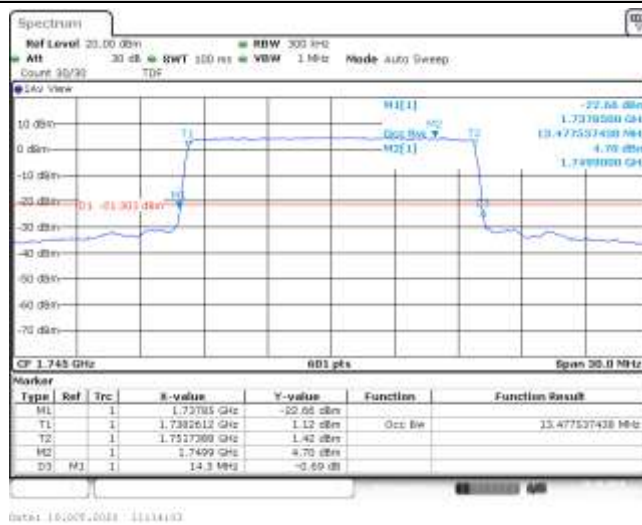
Band66-15MHz-16QAM-132322-75RB#0-13.478-14.300-PASS
