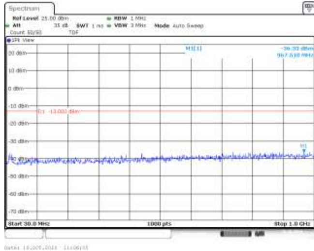
Band66-10MHz-16QAM-132622-1RB#0-Range1:30~1000MHz--36.33-PASS
