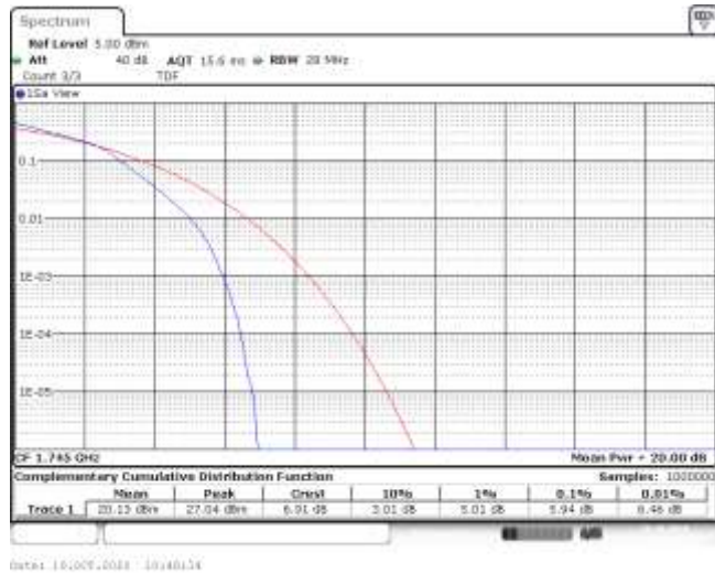
Band66-3MHz-16QAM-132322-15RB#0-5.94-13-PASS
