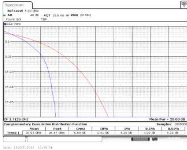
Band66-5MHz-QPSK-131997-25RB#0-4.90-13-PASS
