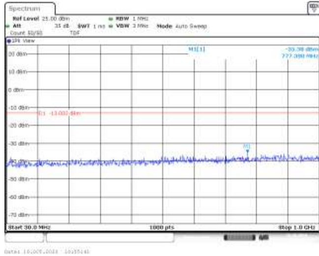
Band66-5MHz-QPSK-132647-1RB#0-Range1:30~1000MHz--35.38-PASS
