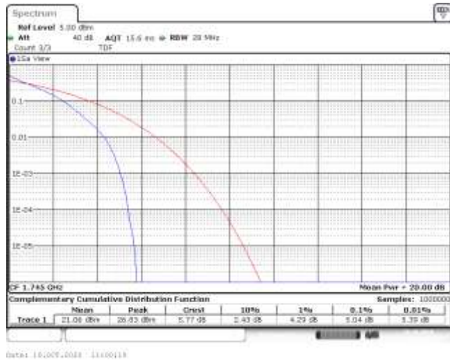
Band66-5MHz-QPSK-132322-25RB#0-5.04-13-PASS
