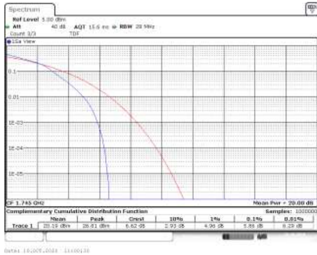
Band66-5MHz-16QAM-132322-25RB#0-5.86-13-PASS
