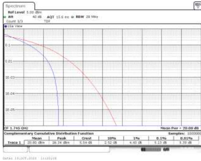
Band66-15MHz-QPSK-132322-75RB#0-5.13-13-PASS
