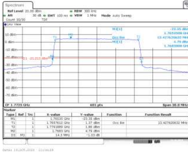
Band66-15MHz-16QAM-132597-75RB#0-13.428-14.300-PASS
