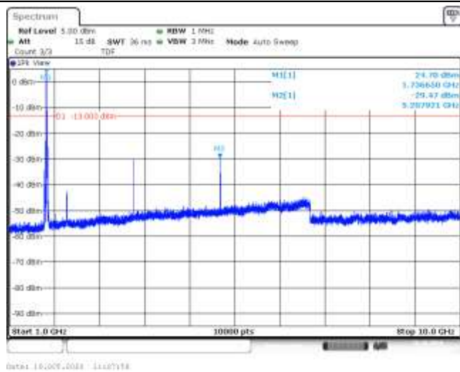
Band66-20MHz-QPSK-132322-1RB#0-Range2:1000~10000MHz--29.47-PASS
