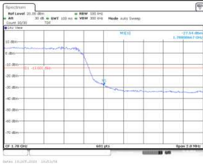
Band66-5MHz-16QAM-132647-25RB#0--27.54-PASS
