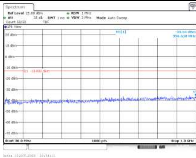
Band66-5MHz-QPSK-131997-1RB#0-Range1:30~1000MHz--35.64-PASS
