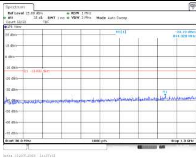
Band66-20MHz-QPSK-132072-1RB#0-Range1:30~1000MHz--35.73-PASS
