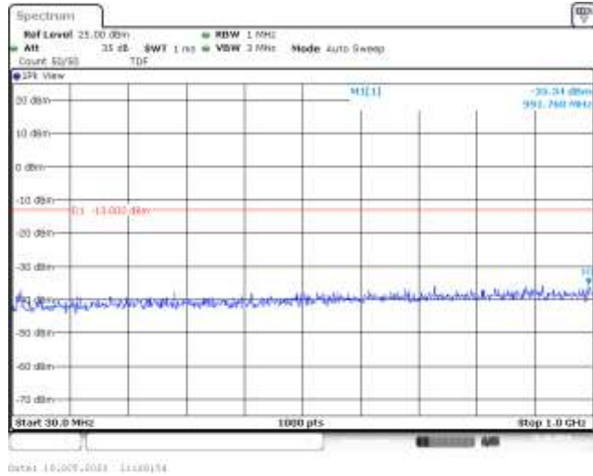
Band66-20MHz-16QAM-132572-1RB#0-Range1:30~1000MHz--35.34-PASS
