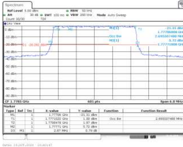
Band66-3MHz-16QAM-132657-15RB#0-2.696-2.870-PASS
