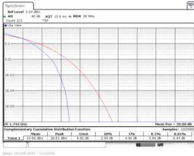
Band66-10MHz-16QAM-132322-50RB#0-5.86-13-PASS
