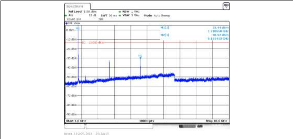
Band66-1.4MHz-16QAM-131979-1RB#0-Range2:1000~10000MHz--30.92-PASS
