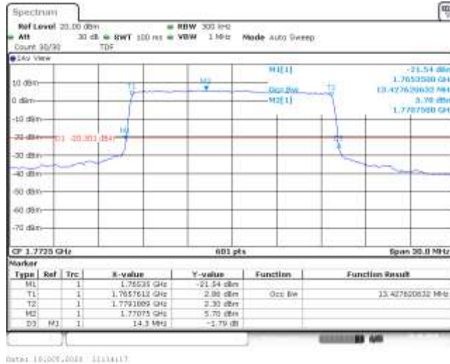
Band66-15MHz-QPSK-132597-75RB#0-13.428-14.300-PASS
