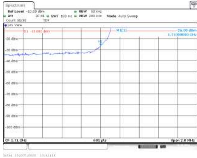
Band66-3MHz-16QAM-131987-15RB#0--26.00-PASS
