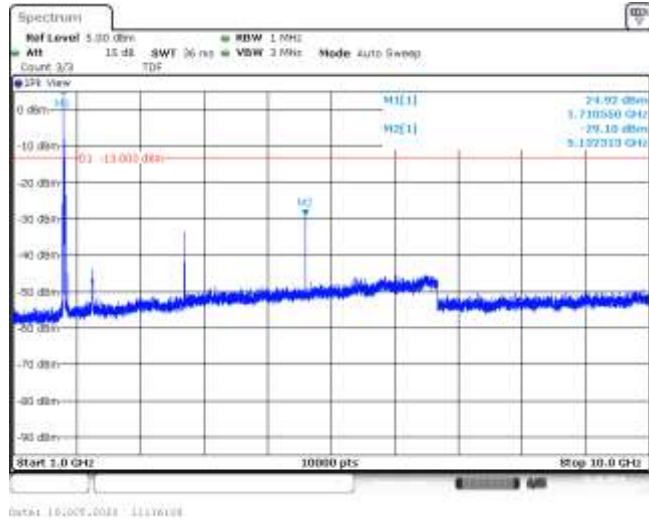
Band66-15MHz-16QAM-132047-1RB#0-Range2:1000~10000MHz--29.1-PASS
