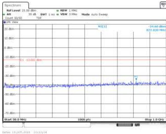
Band66-1.4MHz-QPSK-132665-1RB#0-Range1:30~1000MHz--34.6-PASS
