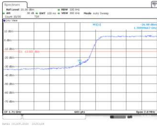
Band66-5MHz-16QAM-131997-25RB#0--26.98-PASS
