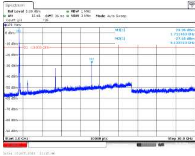
Band66-15MHz-QPSK-132047-1RB#0-Range2:1000~10000MHz--27.65-PASS
