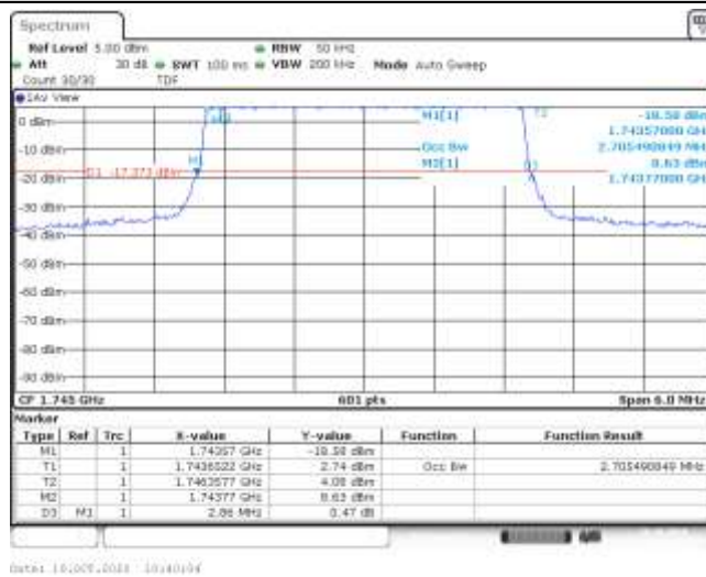
Band66-3MHz-QPSK-132322-15RB#0-2.705-2.860-PASS
