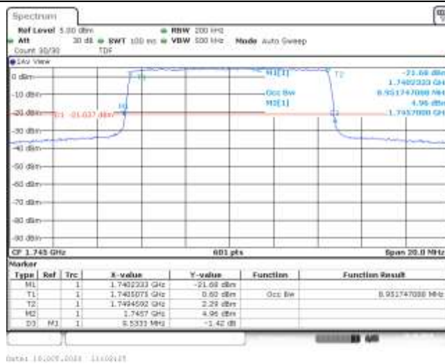
Band66-10MHz-16QAM-132322-50RB#0-8.952-9.533-PASS
