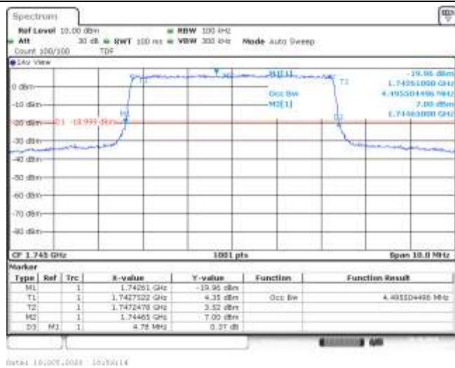
Band66-5MHz-16QAM-132322-25RB#0-4.496-4.780-PASS
