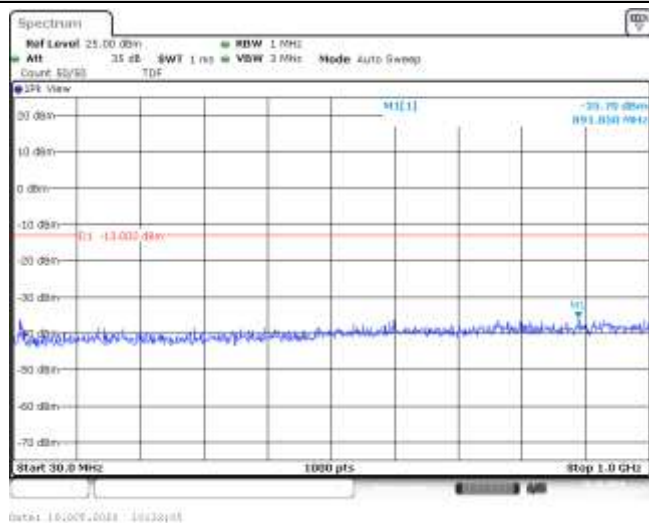
Band66-1.4MHz-16QAM-131979-1RB#0-Range1:30~1000MHz--35.7-PASS
