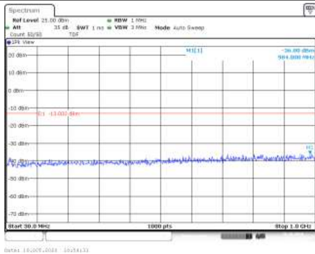
Band66-5MHz-16QAM-131997-1RB#0-Range1:30~1000MHz--36-PASS
