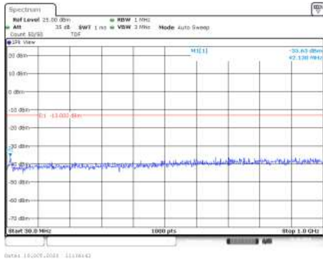
Band66-15MHz-16QAM-132322-1RB#0-Range1:30~1000MHz--35.63-PASS
