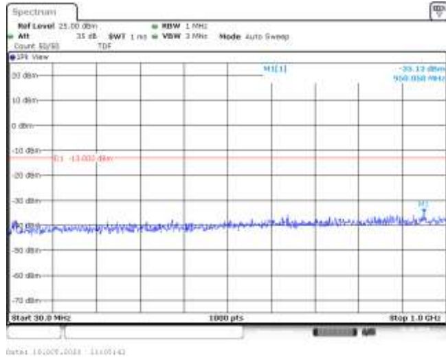
Band66-10MHz-QPSK-132622-1RB#0-Range1:30~1000MHz--35.13-PASS
