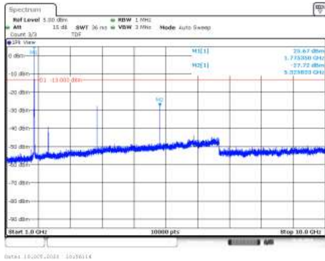
Band66-5MHz-16QAM-132647-1RB#0-Range2:1000~10000MHz--27.72-PASS
