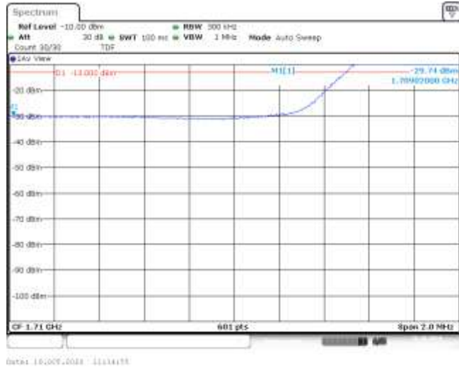
Band66-15MHz-16QAM-132047-75RB#0--29.74-PASS
