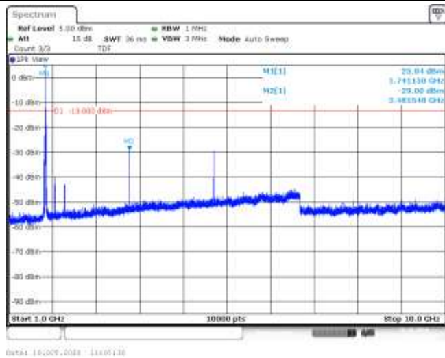
Band66-10MHz-16QAM-132322-1RB#0-Range2:1000~10000MHz--29-PASS
