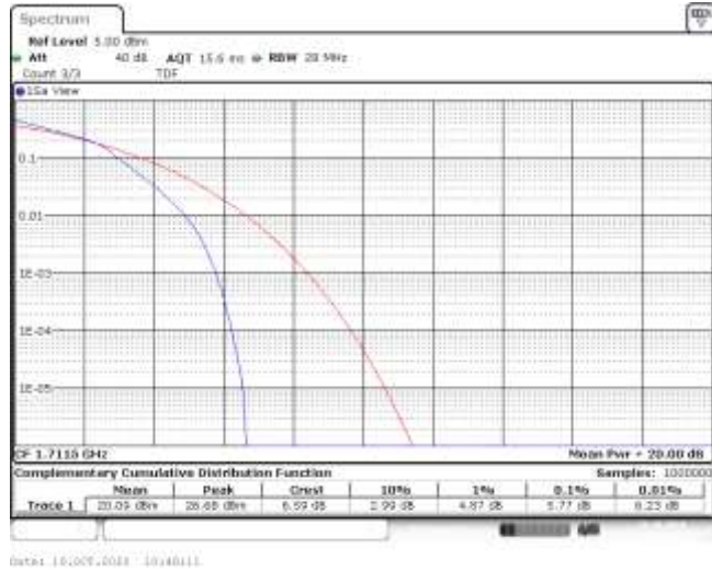
Band66-3MHz-16QAM-131987-15RB#0-5.77-13-PASS
