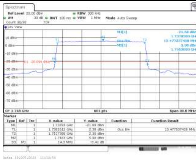
Band66-15MHz-QPSK-132322-75RB#0-13.478-14.300-PASS
