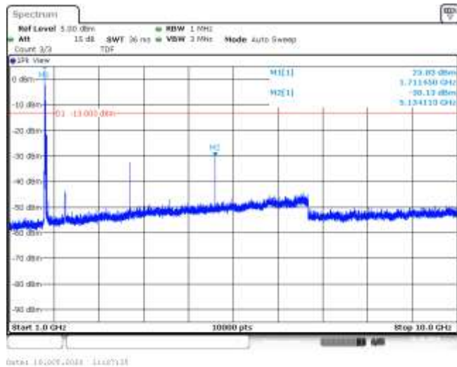
Band66-20MHz-16QAM-132072-1RB#0-Range2:1000~10000MHz--30.13-PASS
