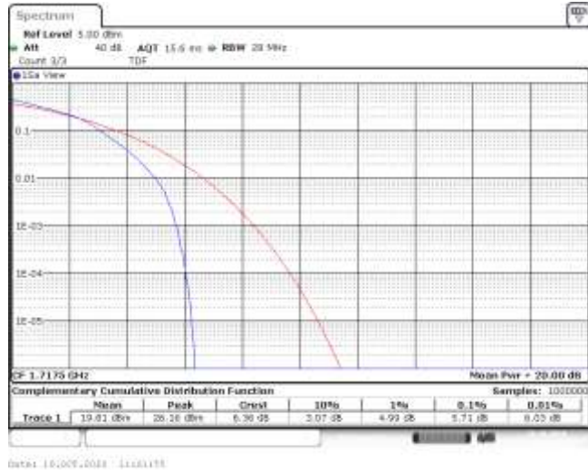
Band66-15MHz-16QAM-132047-75RB#0-5.71-13-PASS
