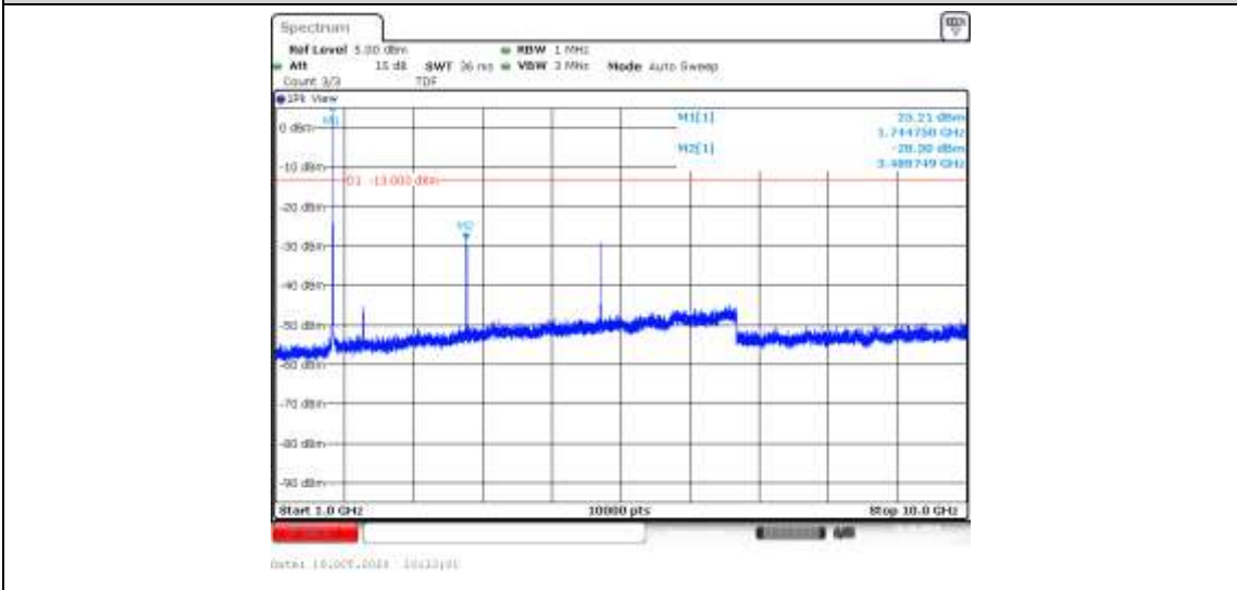
Band66-1.4MHz-16QAM-132322-1RB#0-Range2:1000~10000MHz--28.3-PASS
