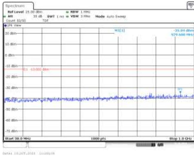
Band66-20MHz-16QAM-132322-1RB#0-Range1:30~1000MHz--35.04-PASS
