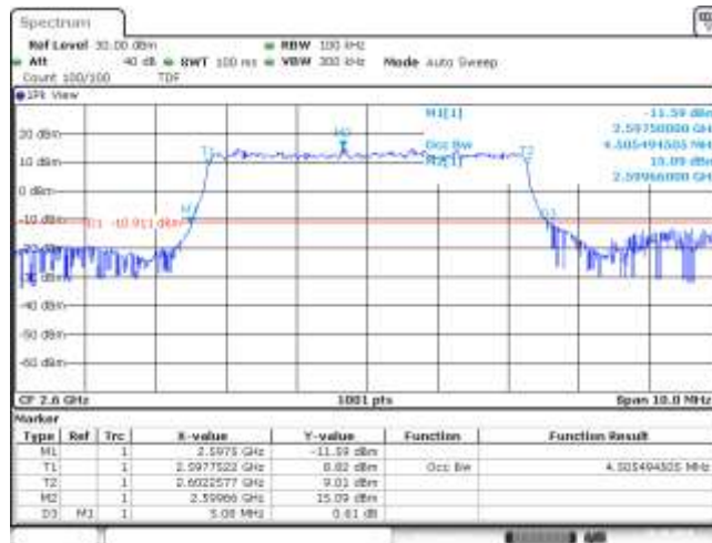
Band41-5MHz-QPSK-40690-25RB#0-4.505
