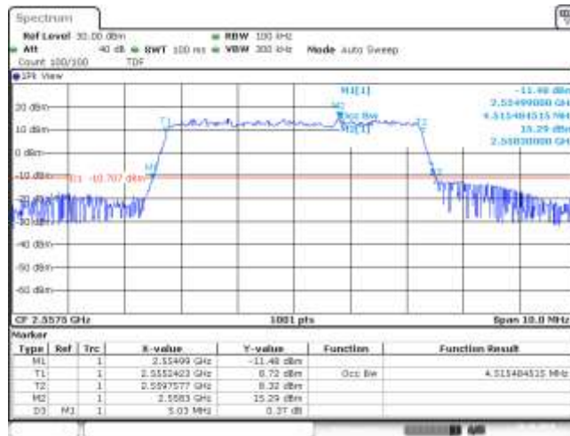
Band41-5MHz-QPSK-40265-25RB#0-4.515
