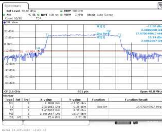
Band41-20MHz-16QAM-41140-100RB#0-17.97
