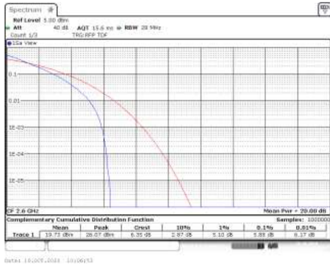
Band41-15MHz-QPSK-41165-75RB#0
