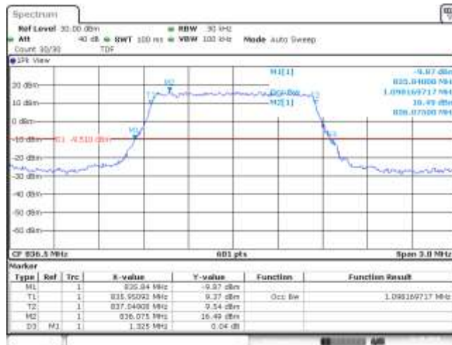
Band26-1.4MHz-QPSK-26915-6RB#0-1.098
