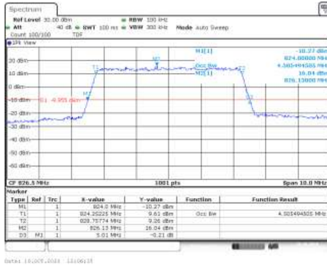
Band26-5MHz-16QAM-26915-25RB#0-4.505
