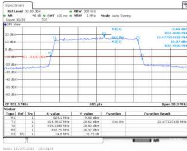
Band26-15MHz-16QAM-26915-75RB#0-13.478
