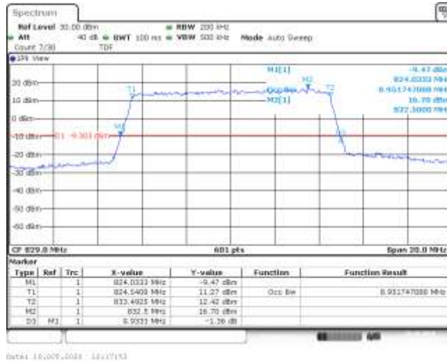
Band26-10MHz-QPSK-26915-50RB#0-8.952
