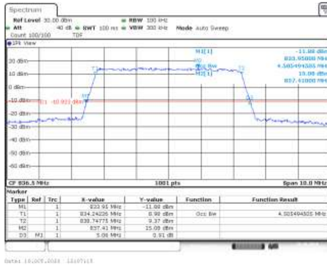
Band26-5MHz-16QAM-27015-25RB#0-4.505
