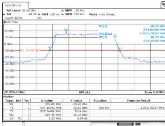
Band26-1.4MHz-QPSK-26797-6RB#0-1.093
