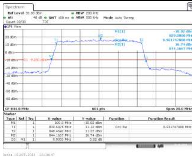
Band26-10MHz-16QAM-26840-50RB#0-8.952
