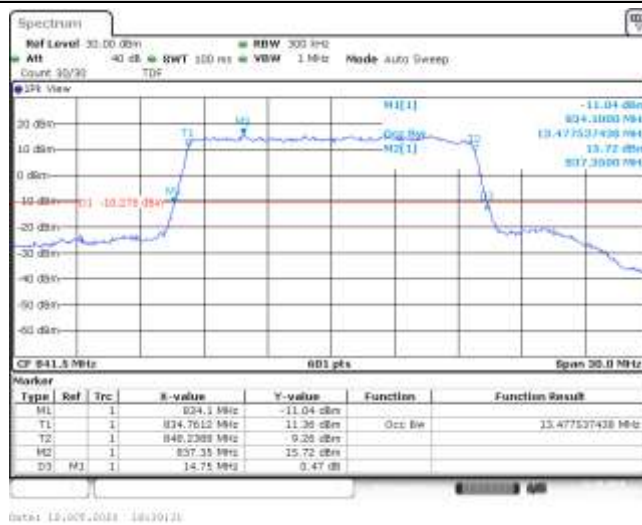
Band26-15MHz-16QAM-26965-75RB#0-13.478
