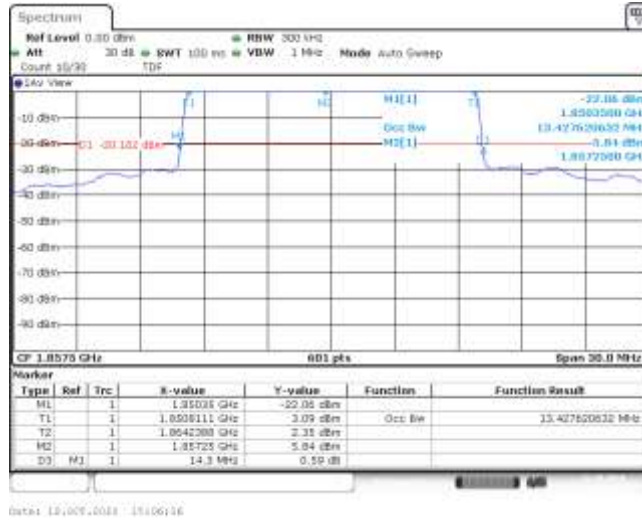
Band25-15MHz-QPSK-26365-75RB#0-13.428
