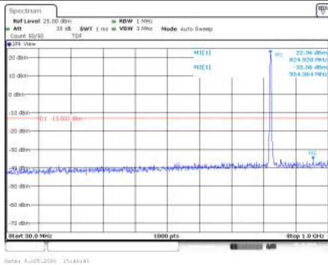
Band5-3MHz-16QAM-20415-15RB#0-Range1:30~1000MHz--35.56-PASS
