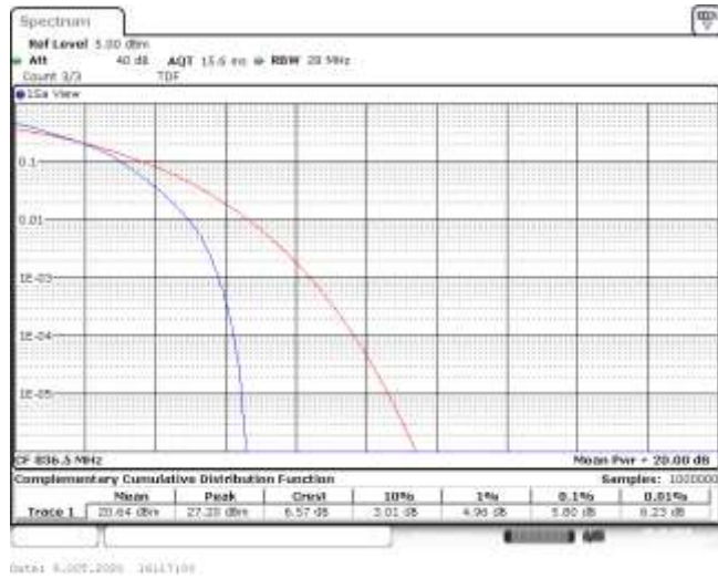
Band5-10MHz-16QAM-20525-50RB#0-5.80-13-PASS
