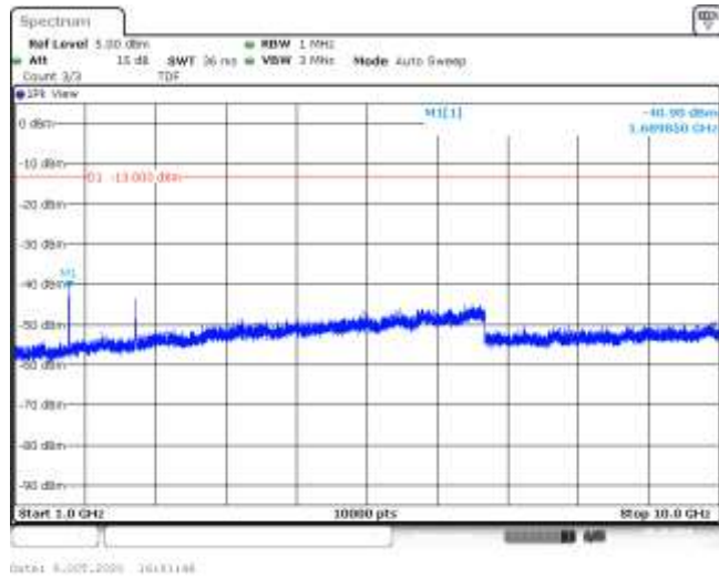
Band5-5MHz-QPSK-20625-25RB#0-Range2:1000~10000MHz--40.9-PASS
