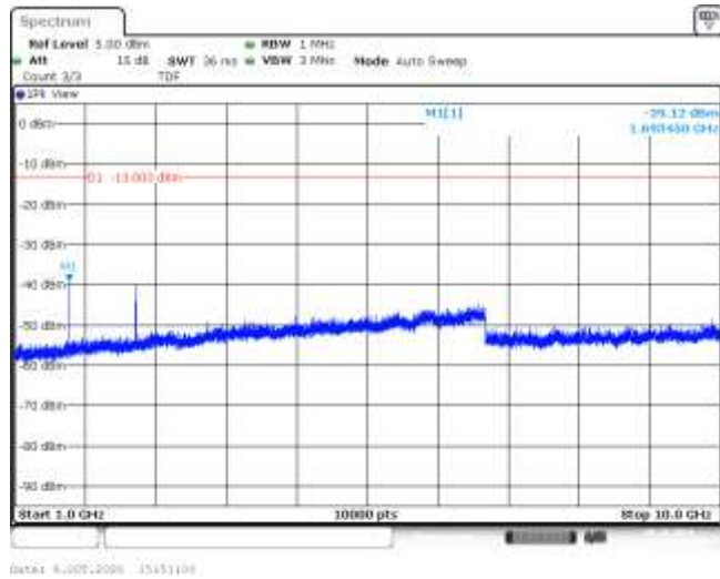
Band5-3MHz-QPSK-20635-15RB#0-Range2:1000~10000MHz--39.12-PASS
