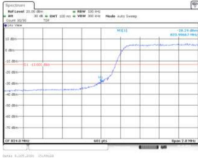
Band5-5MHz-16QAM-20425-25RB#0--28.24-PASS
