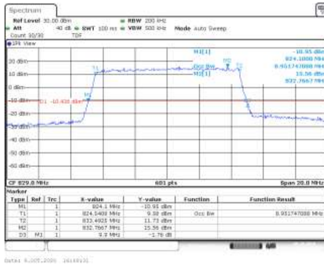
Band5-10MHz-16QAM-20450-50RB#0-8.952-9.900-PASS
