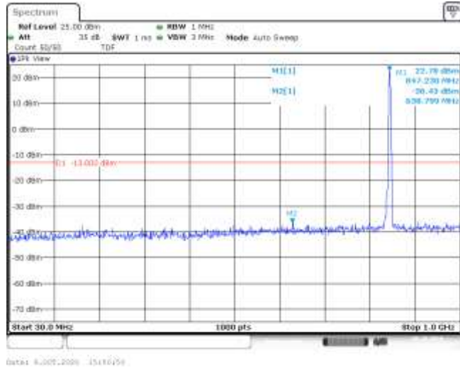
Band5-3MHz-QPSK-20635-15RB#0-Range1:30~1000MHz--36.43-PASS
