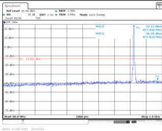
Band5-5MHz-16QAM-20425-25RB#0-Range1:30~1000MHz--36.28-PASS
