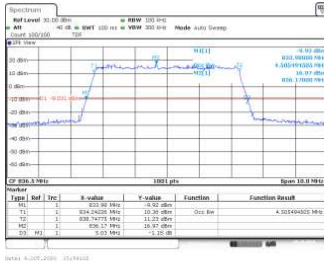
Band5-5MHz-QPSK-20525-25RB#0-4.505-5.030-PASS
