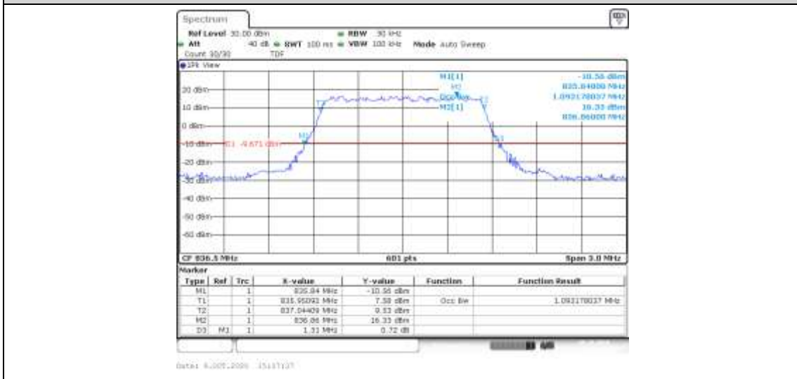
Band5-1.4MHz-QPSK-20525-6RB#0-1.093-1.310-PASS
