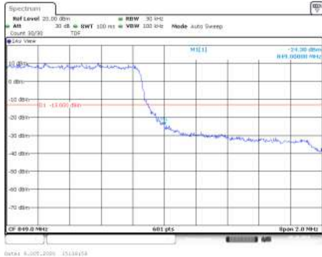
Band5-1.4MHz-QPSK-20643-6RB#0--24.30-PASS
