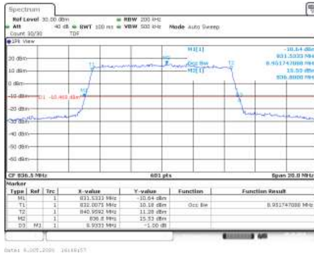
Band5-10MHz-16QAM-20525-50RB#0-8.952-9.933-PASS
