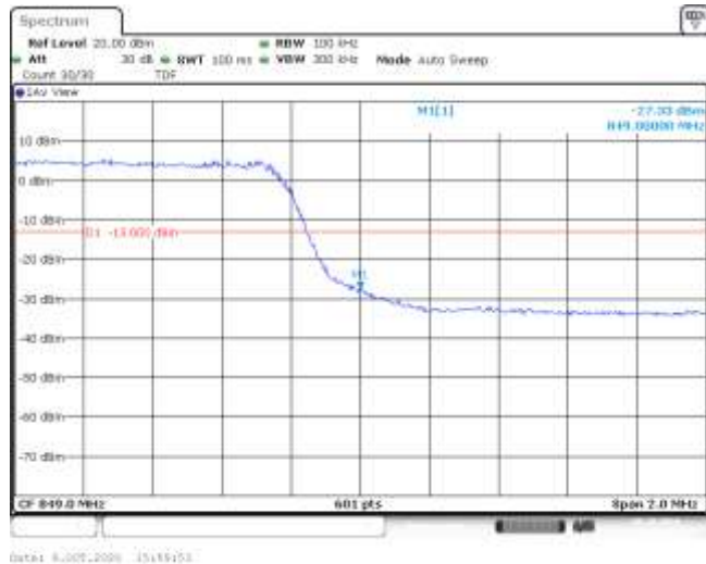
Band5-5MHz-16QAM-20625-25RB#0--27.33-PASS
