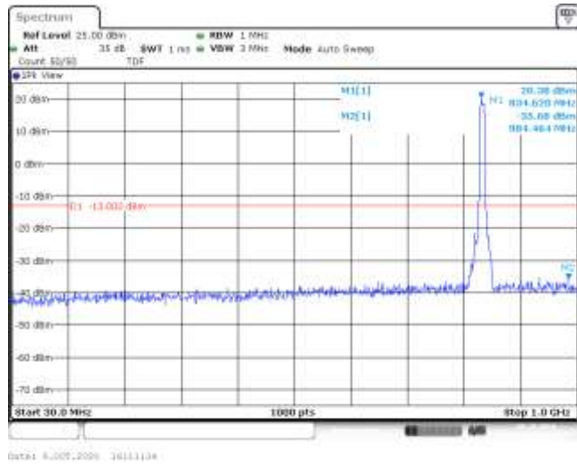
Band5-10MHz-16QAM-20525-50RB#0-Range1:30~1000MHz--35.68-PASS
