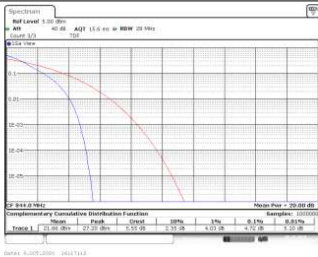
Band5-10MHz-QPSK-20600-50RB#0-4.72-13-PASS
