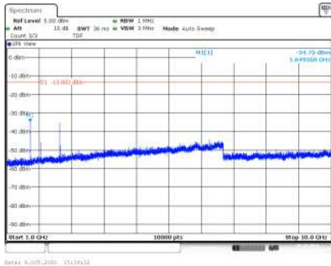
Band5-1.4MHz-QPSK-20407-6RB#0-Range2:1000~10000MHz--34.75-PASS
