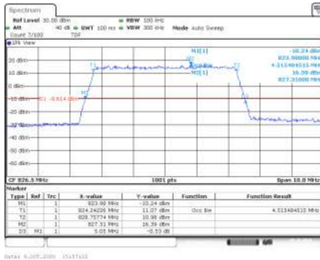
Band5-5MHz-QPSK-20425-25RB#0-4.515-5.050-PASS
