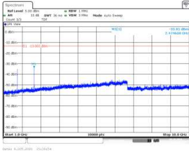
Band5-1.4MHz-16QAM-20407-6RB#0-Range2:1000~10000MHz--33.81-PASS
