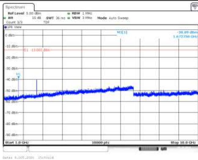
Band5-3MHz-QPSK-20525-15RB#0-Range2:1000~10000MHz--38.89-PASS
