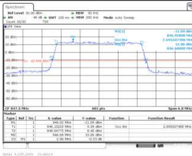
Band5-3MHz-16QAM-20635-15RB#0-2.696-2.960-PASS
