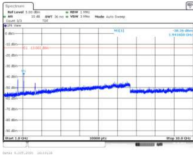
Band5-10MHz-QPSK-20450-50RB#0-Range2:1000~10000MHz--38.26-PASS
