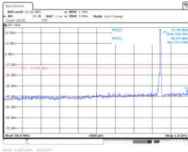
Band5-5MHz-16QAM-20625-25RB#0-Range1:30~1000MHz--36.04-PASS
