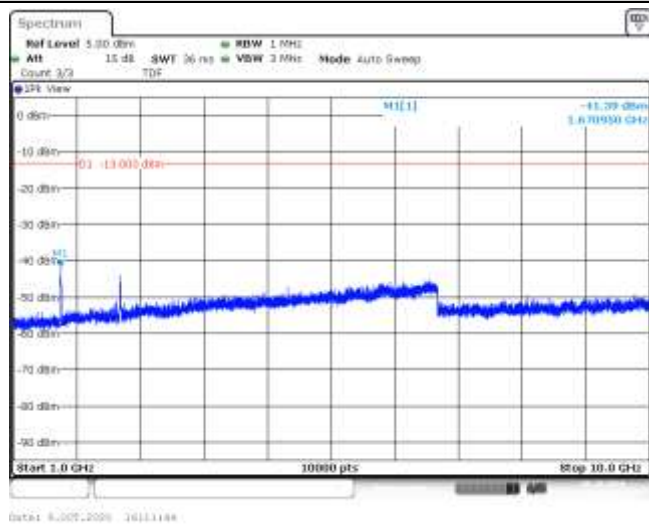
Band5-10MHz-16QAM-20525-50RB#0-Range2:1000~10000MHz--41.39-PASS
