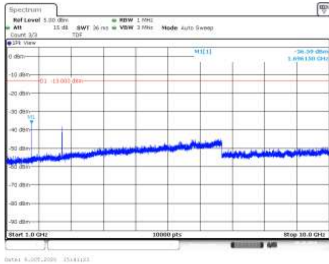
Band5-1.4MHz-16QAM-20643-6RB#0-Range2:1000~10000MHz--36.59-PASS
