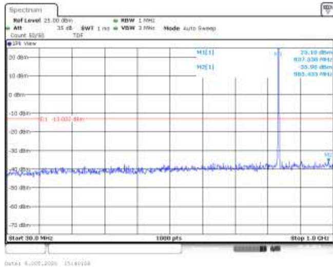
Band5-1.4MHz-16QAM-20525-6RB#0-Range1:30~1000MHz--35.9-PASS
