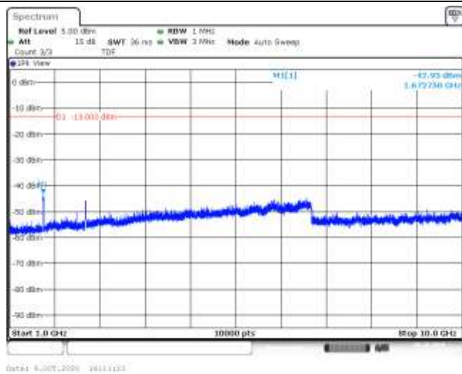
Band5-10MHz-QPSK-20525-50RB#0-Range2:1000~10000MHz--42.93-PASS
