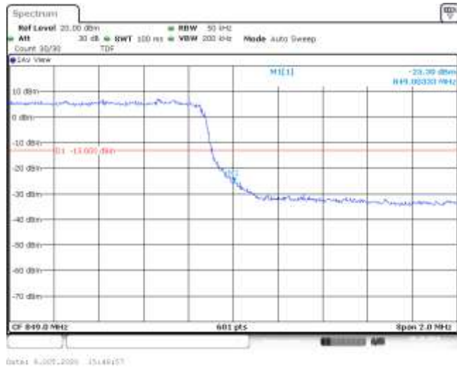
Band5-3MHz-QPSK-20635-15RB#0--25.30-PASS
