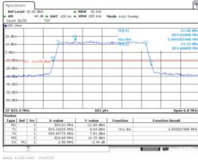
Band5-3MHz-16QAM-20415-15RB#0-2.696-2.990-PASS
