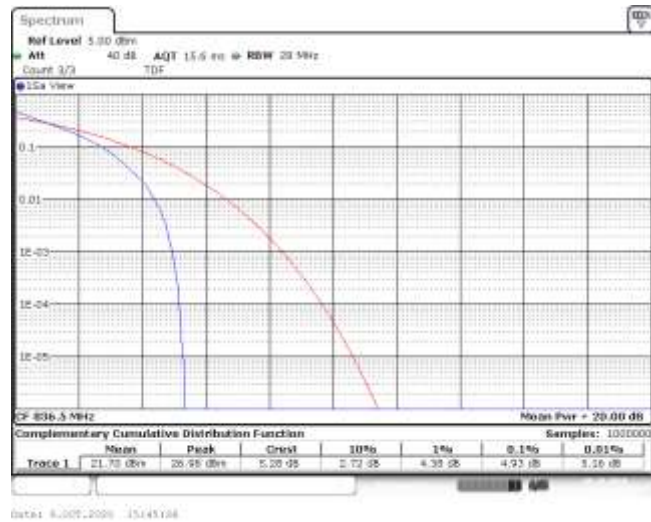
Band5-1.4MHz-QPSK-20525-6RB#0-4.93-13-PASS
