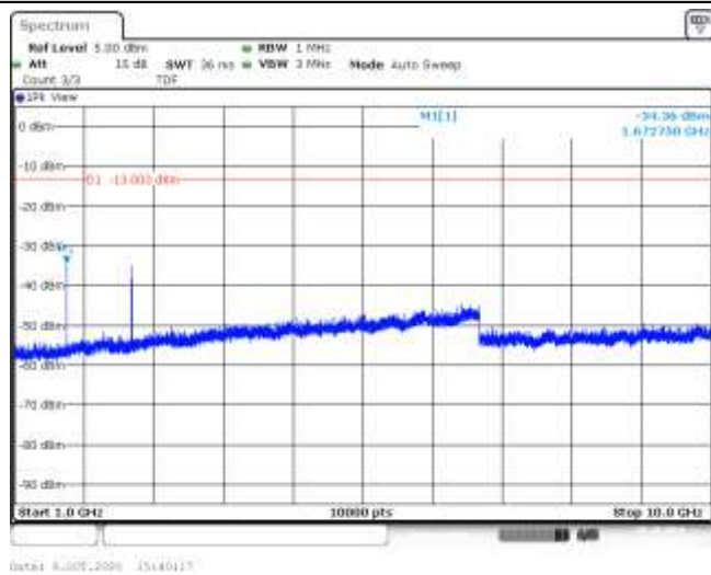
Band5-1.4MHz-QPSK-20525-6RB#0-Range2:1000~10000MHz--34.36-PASS
