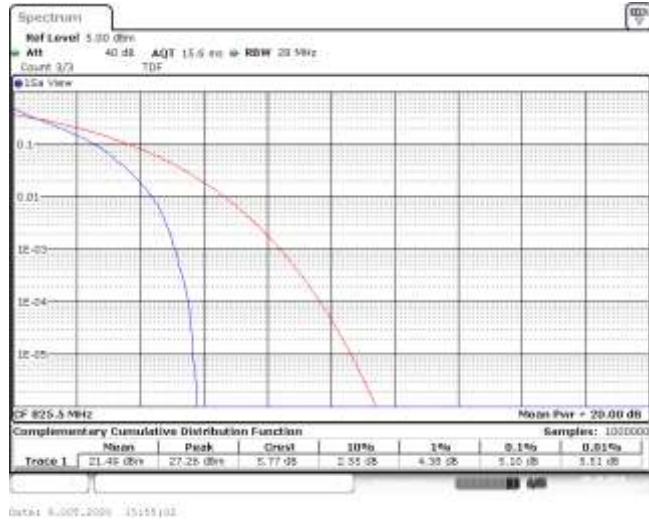
Band5-3MHz-QPSK-20415-15RB#0-5.10-13-PASS
