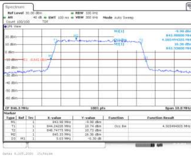
Band5-5MHz-QPSK-20625-25RB#0-4.505-5.030-PASS
