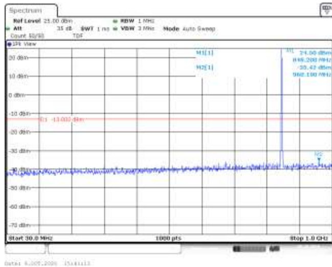
Band5-1.4MHz-16QAM-20643-6RB#0-Range1:30~1000MHz--35.42-PASS
