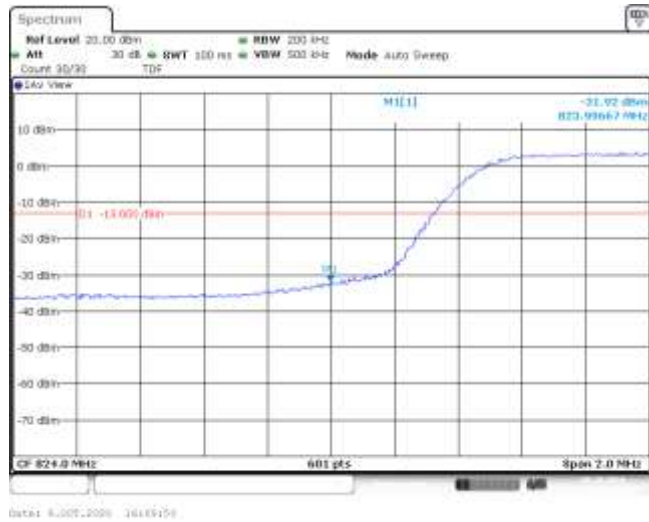
Band5-10MHz-16QAM-20450-50RB#0--31.92-PASS
