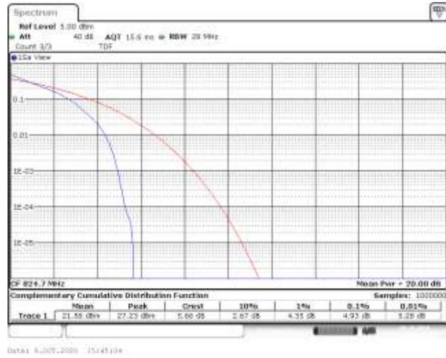
Band5-1.4MHz-QPSK-20407-6RB#0-4.93-13-PASS
