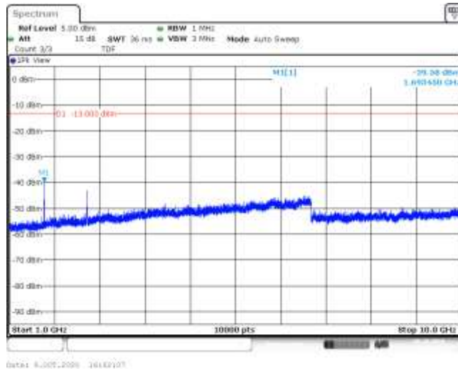
Band5-5MHz-16QAM-20625-25RB#0-Range2:1000~10000MHz--39.58-PASS
