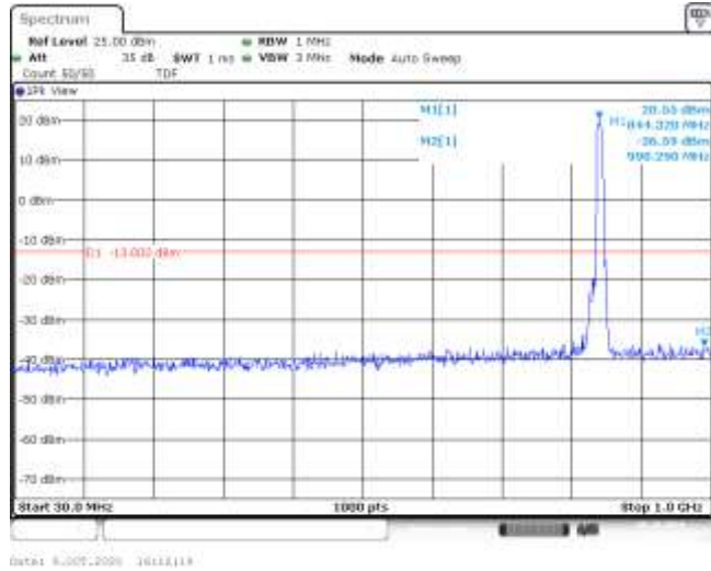
Band5-10MHz-16QAM-20600-50RB#0-Range1:30~1000MHz--36.59-PASS
