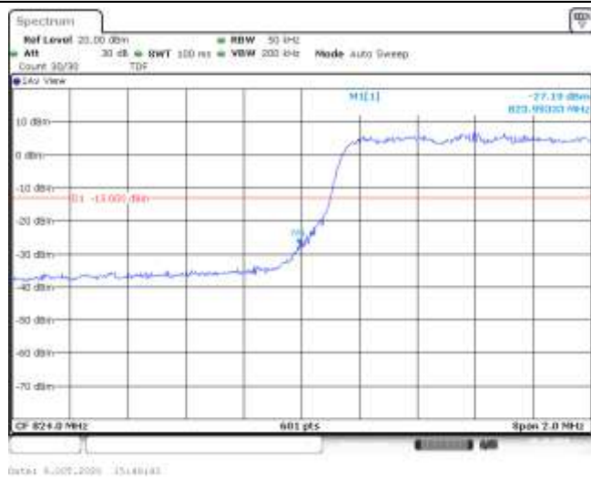
Band5-3MHz-16QAM-20415-15RB#0--27.19-PASS
