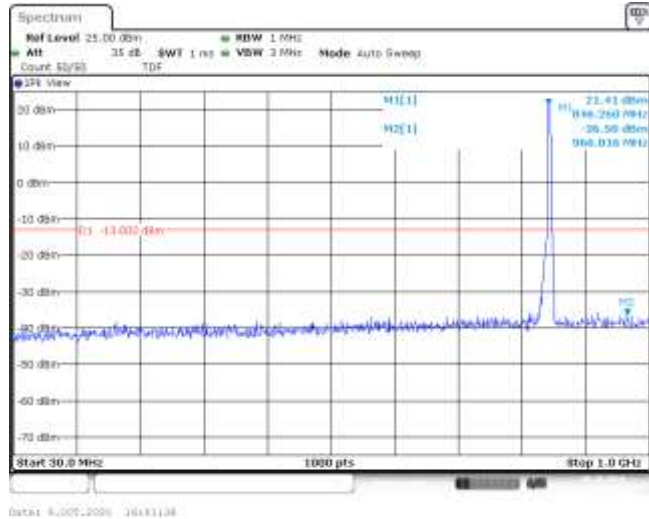
Band5-5MHz-QPSK-20625-25RB#0-Range1:30~1000MHz--36.5-PASS
