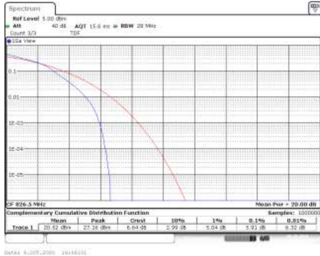
Band5-5MHz-16QAM-20425-25RB#0-5.91-13-PASS
