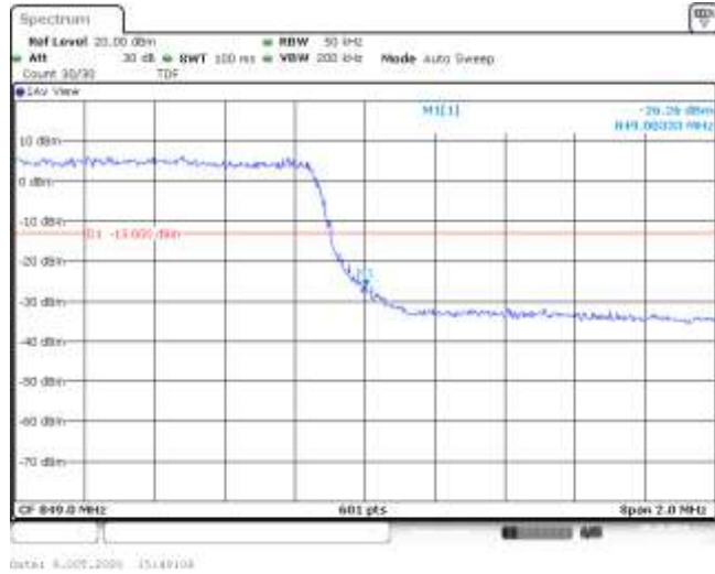
Band5-3MHz-16QAM-20635-15RB#0--26.26-PASS
