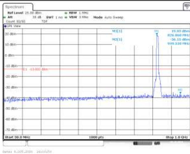
Band5-10MHz-16QAM-20450-50RB#0-Range1:30~1000MHz--36.15-PASS
