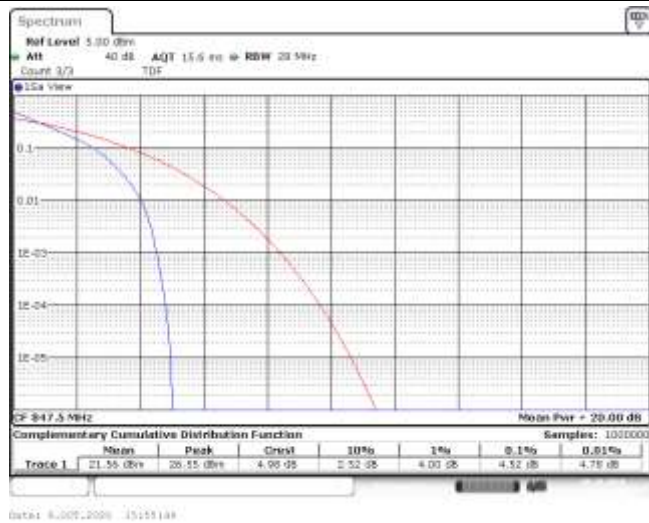
Band5-3MHz-QPSK-20635-15RB#0-4.52-13-PASS
