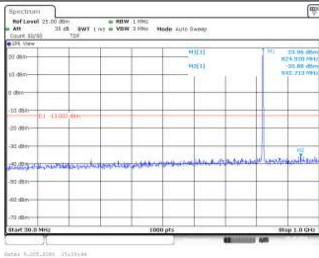
Band5-1.4MHz-16QAM-20407-6RB#0-Range1:30~1000MHz--35.88-PASS
