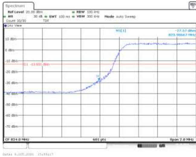
Band5-5MHz-QPSK-20425-25RB#0--27.57-PASS
