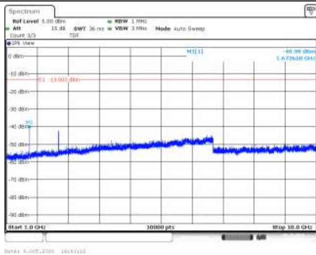
Band5-5MHz-16QAM-20525-25RB#0-Range2:1000~10000MHz--40.98-PASS
