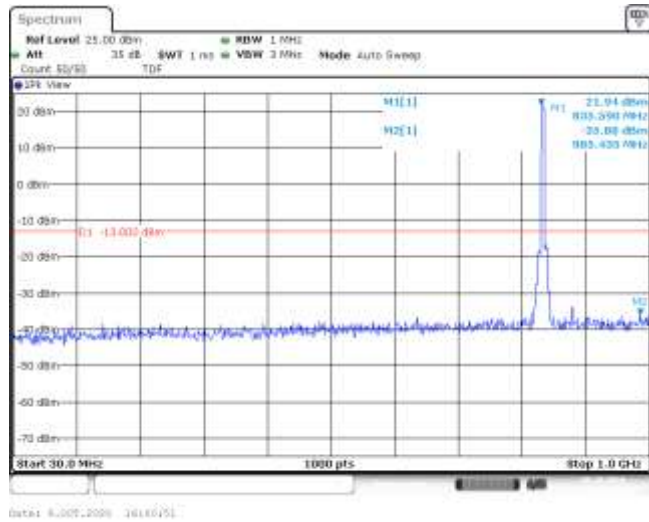
Band5-5MHz-QPSK-20525-25RB#0-Range1:30~1000MHz--35.88-PASS
