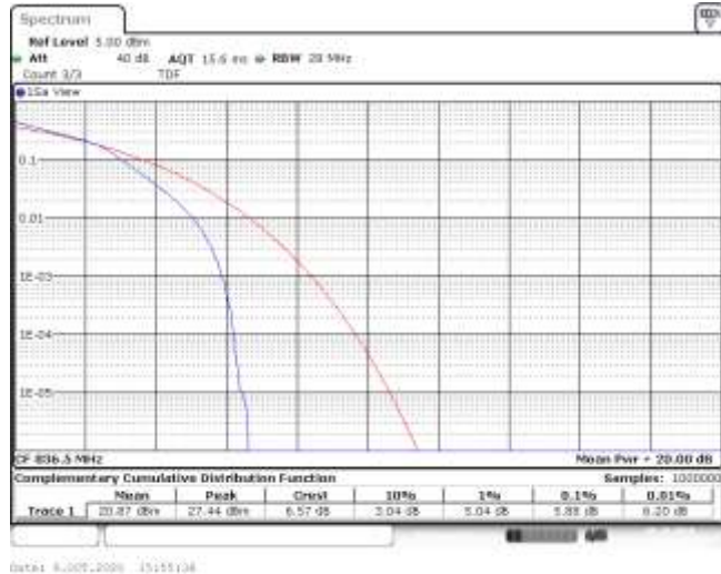
Band5-3MHz-16QAM-20525-15RB#0-5.88-13-PASS
