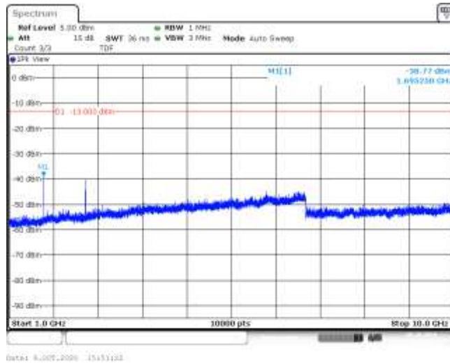
Band5-3MHz-16QAM-20635-15RB#0-Range2:1000~10000MHz--38.77-PASS
