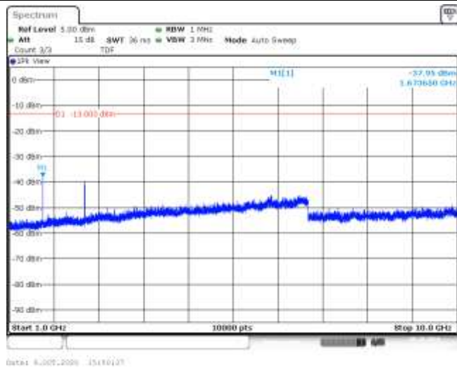
Band5-3MHz-16QAM-20525-15RB#0-Range2:1000~10000MHz--37.95-PASS
