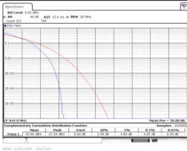
Band5-10MHz-16QAM-20600-50RB#0-5.65-13-PASS
