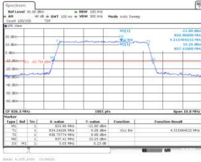
Band5-5MHz-16QAM-20525-25RB#0-4.515-5.050-PASS
