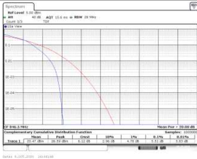
Band5-5MHz-16QAM-20625-25RB#0-5.51-13-PASS
