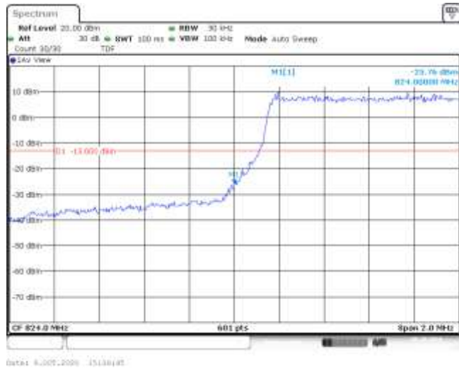
Band5-1.4MHz-16QAM-20407-6RB#0--25.76-PASS
