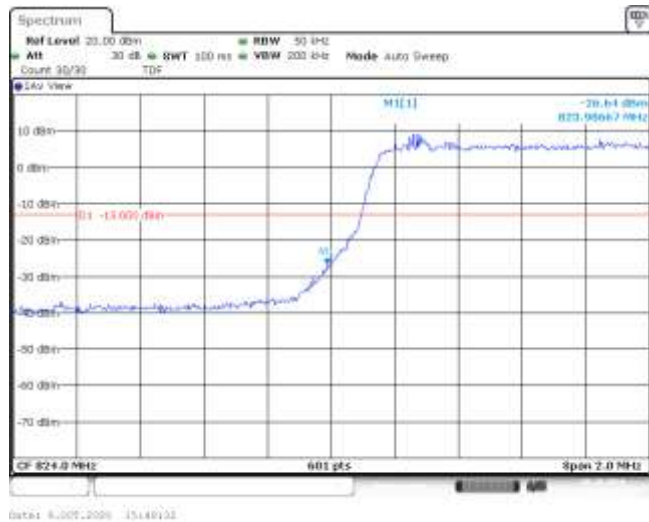
Band5-3MHz-QPSK-20415-15RB#0--26.64-PASS
