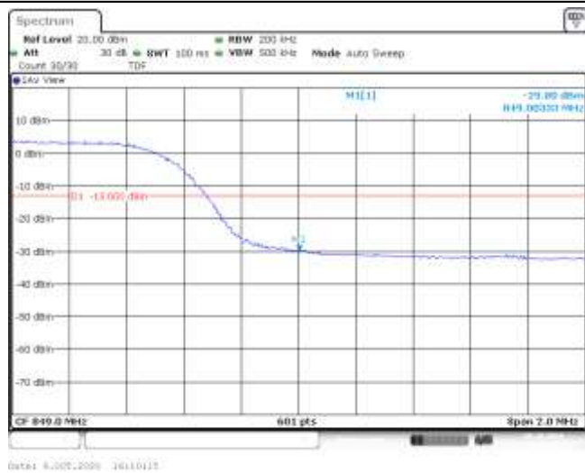
Band5-10MHz-16QAM-20600-50RB#0--29.80-PASS
