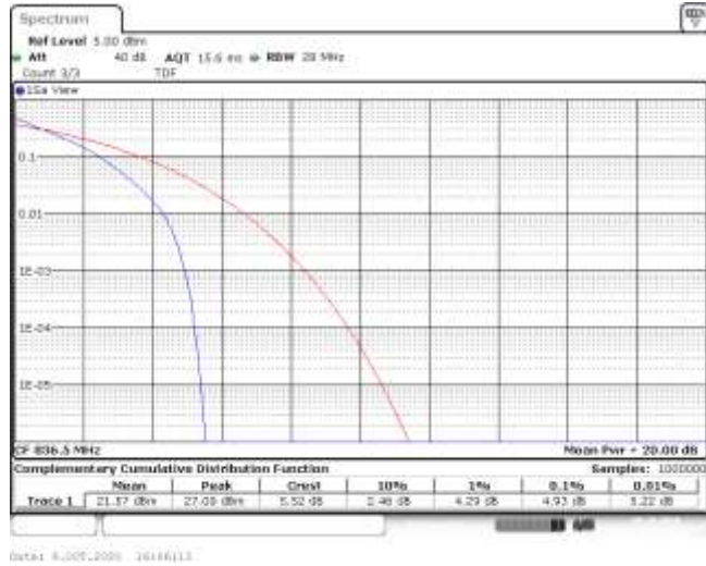
Band5-5MHz-QPSK-20525-25RB#0-4.93-13-PASS
