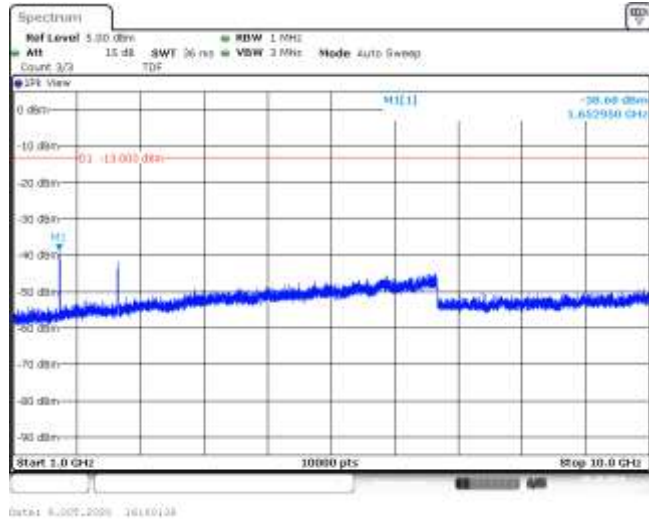
Band5-5MHz-16QAM-20425-25RB#0-Range2:1000~10000MHz--38.68-PASS
