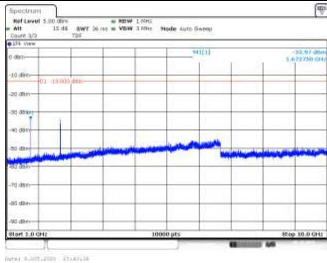
Band5-1.4MHz-16QAM-20525-6RB#0-Range2:1000~10000MHz--33.97-PASS
