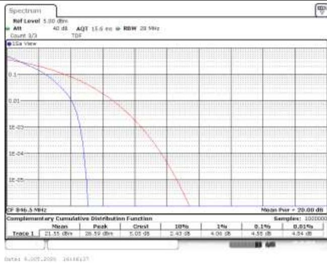
Band5-5MHz-QPSK-20625-25RB#0-4.58-13-PASS
