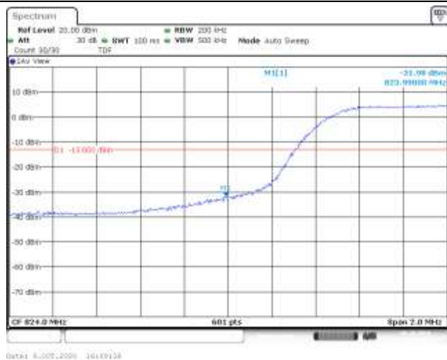
Band5-10MHz-QPSK-20450-50RB#0--31.98-PASS
