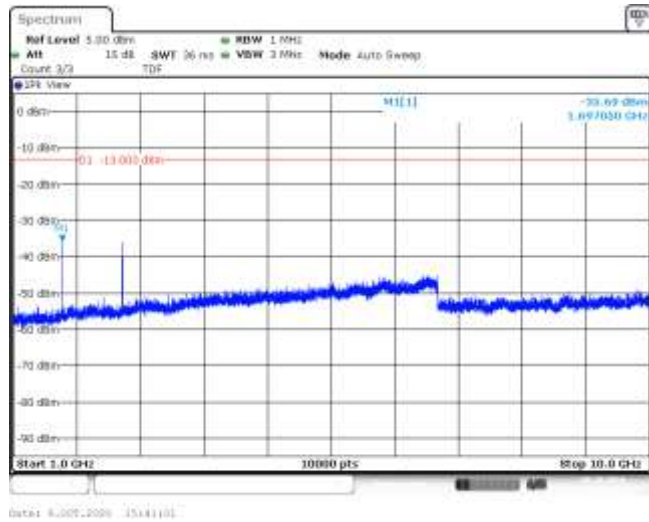
Band5-1.4MHz-QPSK-20643-6RB#0-Range2:1000~10000MHz--35.69-PASS
