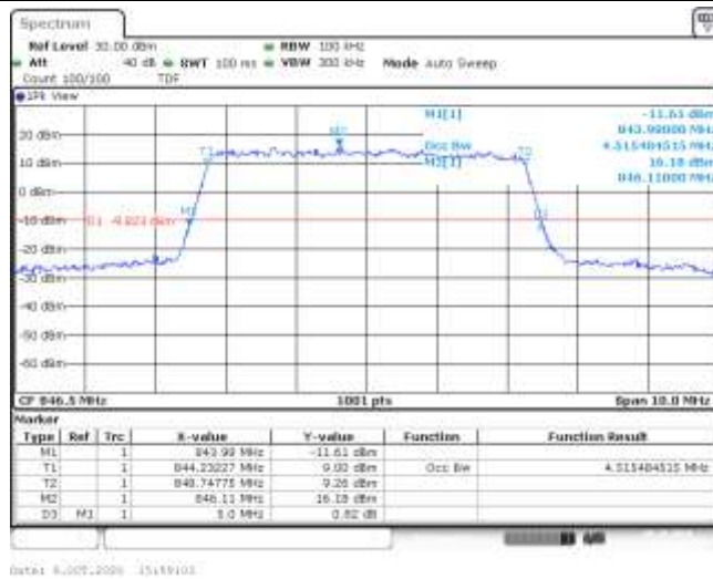
Band5-5MHz-16QAM-20625-25RB#0-4.515-5.000-PASS
