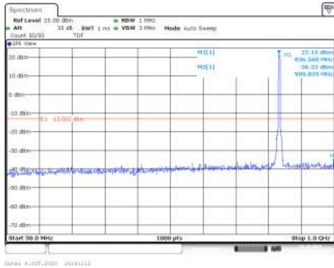
Band5-5MHz-16QAM-20525-25RB#0-Range1:30~1000MHz--36.32-PASS
