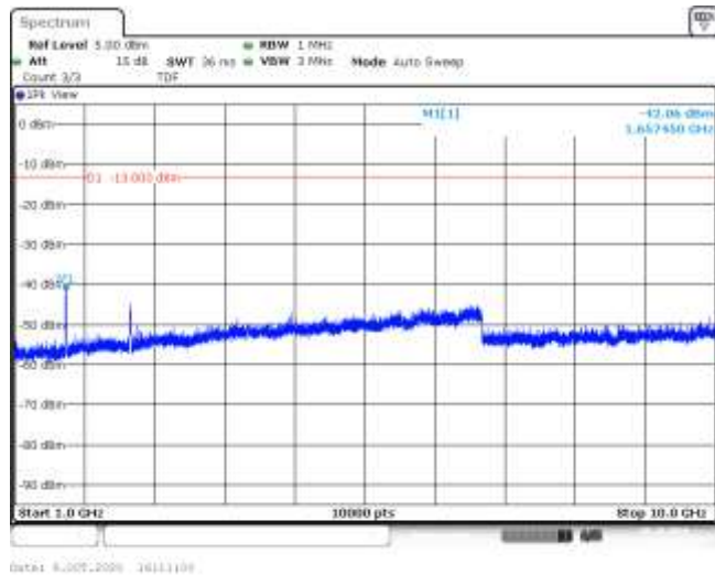
Band5-10MHz-16QAM-20450-50RB#0-Range2:1000~10000MHz--42.06-PASS
