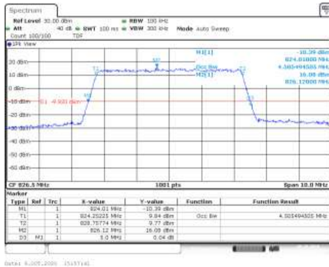
Band5-5MHz-16QAM-20425-25RB#0-4.505-5.000-PASS
