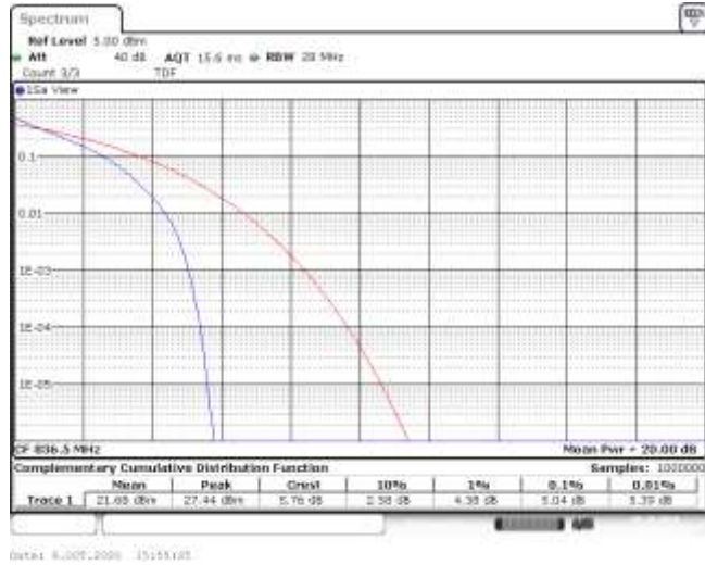
Band5-3MHz-QPSK-20525-15RB#0-5.04-13-PASS
