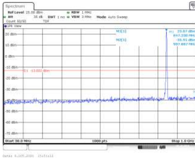
Band5-3MHz-16QAM-20635-15RB#0-Range1:30~1000MHz--35.91-PASS
