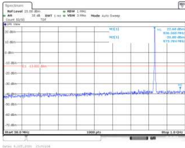
Band5-3MHz-QPSK-20525-15RB#0-Range1:30~1000MHz--35-PASS
