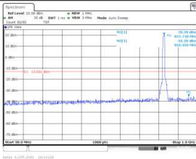
Band5-10MHz-QPSK-20450-50RB#0-Range1:30~1000MHz--35.28-PASS
