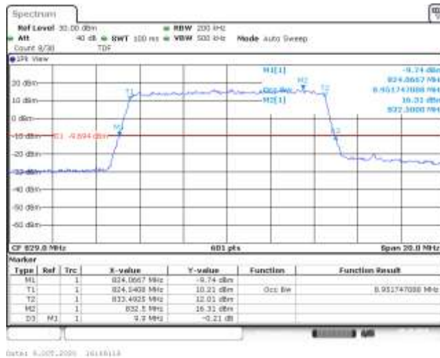
Band5-10MHz-QPSK-20450-50RB#0-8.952-9.900-PASS
