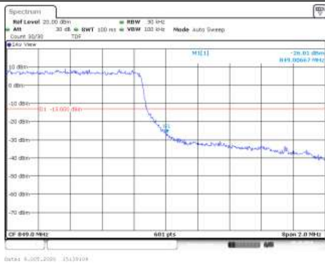
Band5-1.4MHz-16QAM-20643-6RB#0--26.01-PASS
