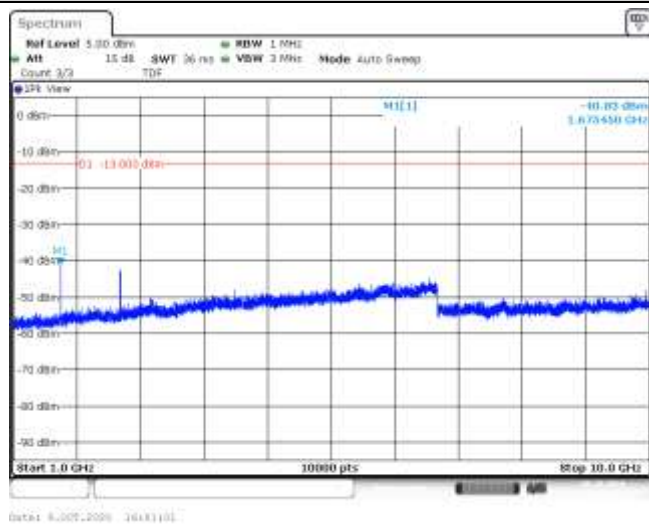
Band5-5MHz-QPSK-20525-25RB#0-Range2:1000~10000MHz--40.83-PASS
