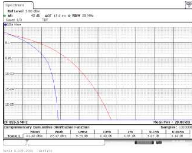
Band5-5MHz-QPSK-20425-25RB#0-5.07-13-PASS
