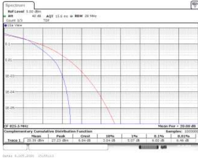
Band5-3MHz-16QAM-20415-15RB#0-6.00-13-PASS
