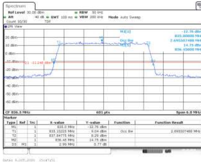
Band5-3MHz-16QAM-20525-15RB#0-2.696-2.990-PASS
