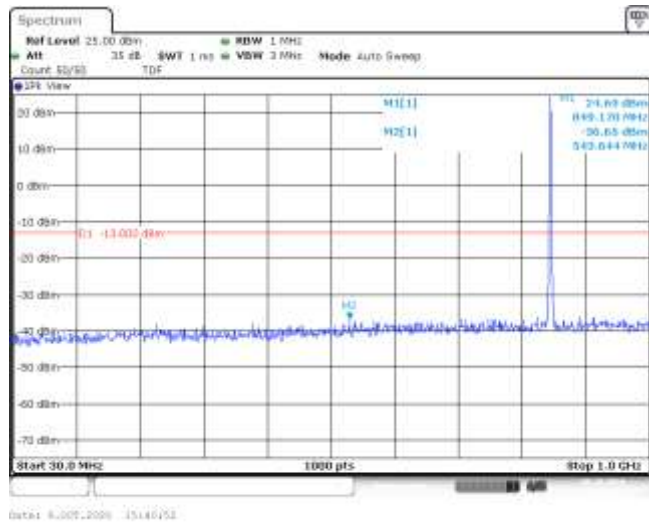
Band5-1.4MHz-QPSK-20643-6RB#0-Range1:30~1000MHz--36.65-PASS
