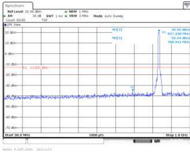
Band5-10MHz-QPSK-20525-50RB#0-Range1:30~1000MHz--35.34-PASS
