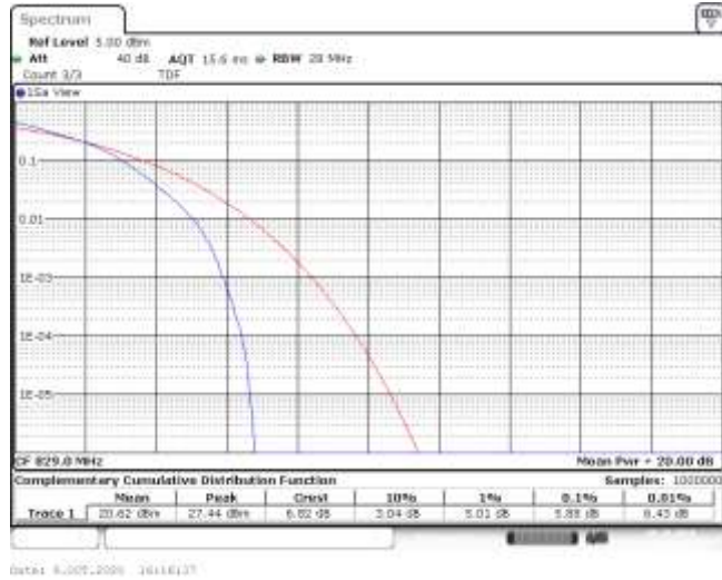
Band5-10MHz-16QAM-20450-50RB#0-5.88-13-PASS
