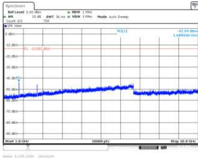
Band5-10MHz-16QAM-20600-50RB#0-Range2:1000~10000MHz--42.94-PASS
