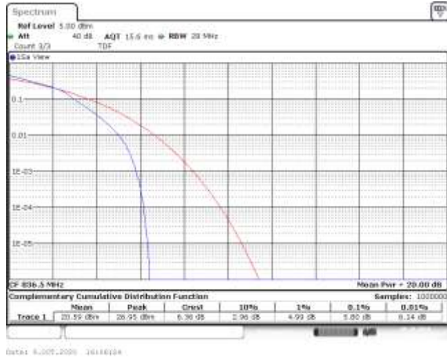
Band5-5MHz-16QAM-20525-25RB#0-5.80-13-PASS
