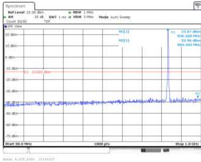
Band5-3MHz-16QAM-20525-15RB#0-Range1:30~1000MHz--35.96-PASS
