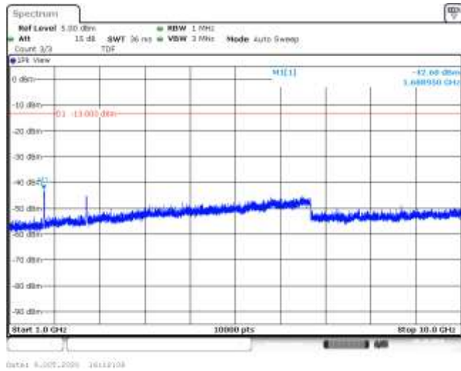
Band5-10MHz-QPSK-20600-50RB#0-Range2:1000~10000MHz--42.68-PASS
