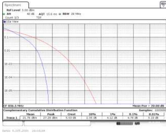
Band5-10MHz-QPSK-20525-50RB#0-4.78-13-PASS
