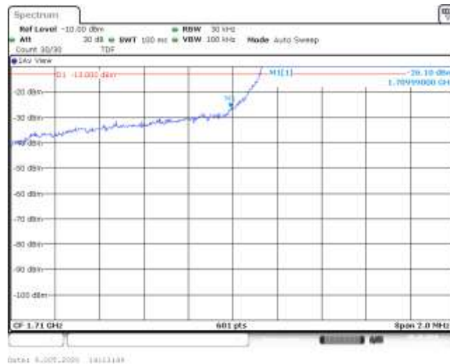
Band4-1.4MHz-16QAM-19957-6RB#0--26.10-PASS
