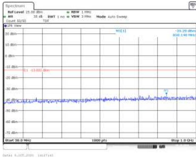
Band4-3MHz-16QAM-19965-15RB#0-Range1:30~1000MHz--35.2-PASS
