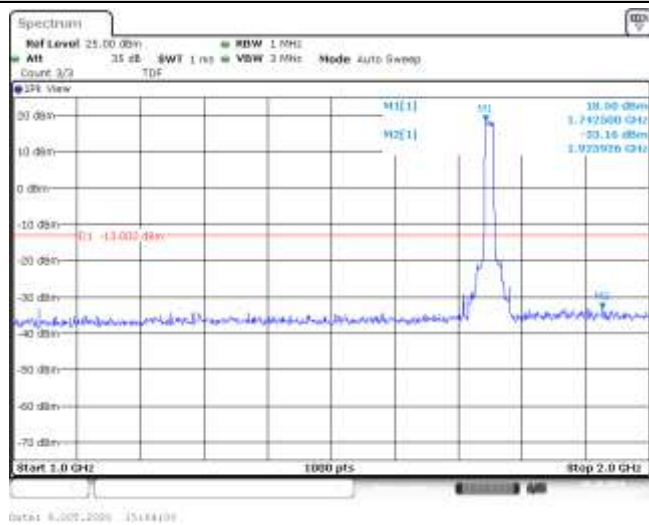
Band4-15MHz-QPSK-20325-75RB#0-Range2:1000~2000MHz--33.16-PASS
