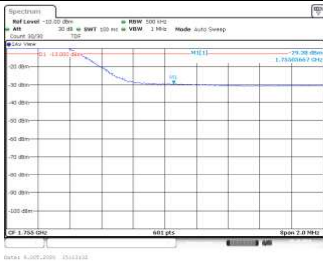
Band4-20MHz-16QAM-20300-100RB#0--29.38-PASS
