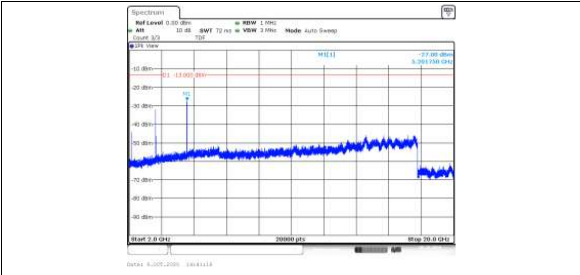
Band4-5MHz-16QAM-20175-25RB#0-Range3:2000~20000MHz--27-PASS
