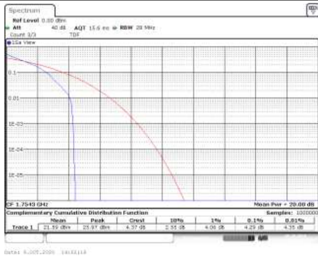
Band4-1.4MHz-QPSK-20393-1RB#0-4.29-13-PASS
