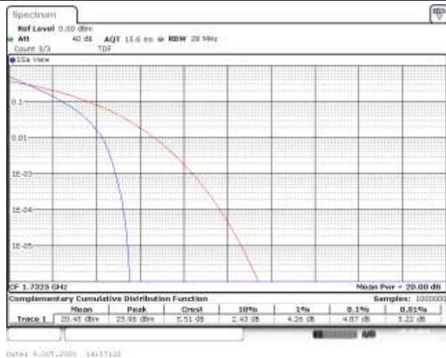
Band4-10MHz-QPSK-20175-50RB#0-4.87-13-PASS
