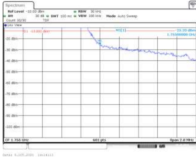
Band4-1.4MHz-16QAM-20393-6RB#0--25.33-PASS
