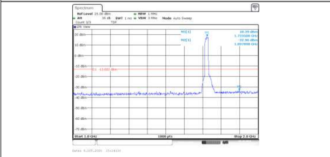
Band4-20MHz-16QAM-20050-100RB#0-Range2:1000~2000MHz--32.96-PASS
