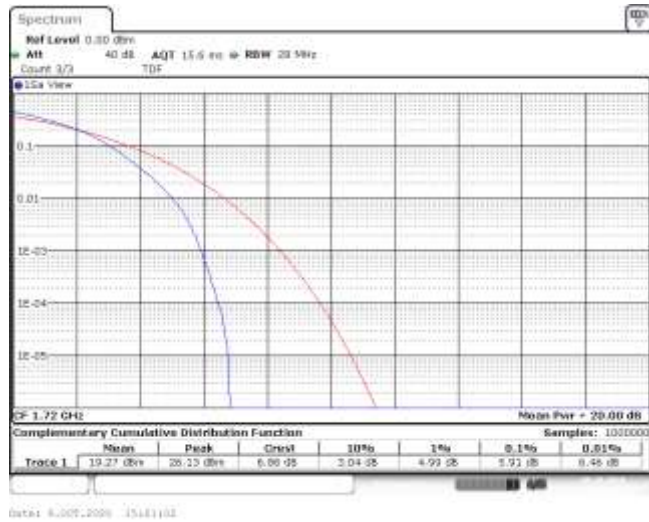
Band4-20MHz-16QAM-20050-100RB#0-5.91-13-PASS
