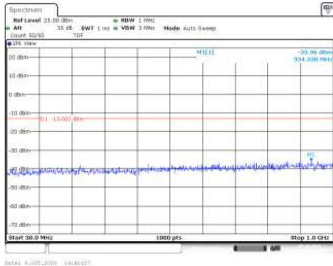
Band4-5MHz-QPSK-20175-25RB#0-Range1:30~1000MHz--35.96-PASS
