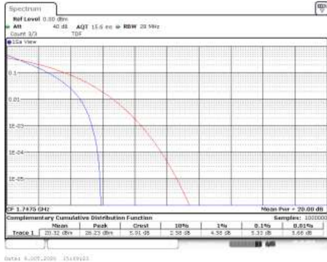
Band4-15MHz-QPSK-20325-75RB#0-5.33-13-PASS
