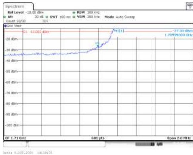
Band4-5MHz-QPSK-19975-25RB#0--27.33-PASS
