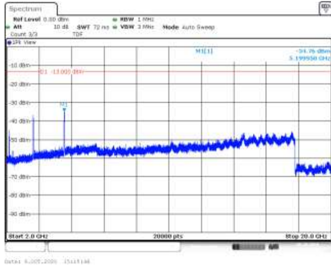
Band4-20MHz-16QAM-20175-100RB#0-Range3:2000~20000MHz--34.76-PASS
