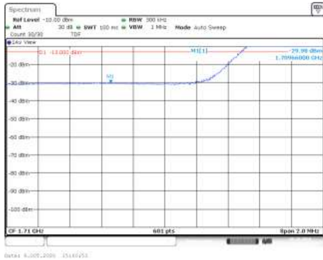
Band4-15MHz-QPSK-20025-75RB#0--29.98-PASS
