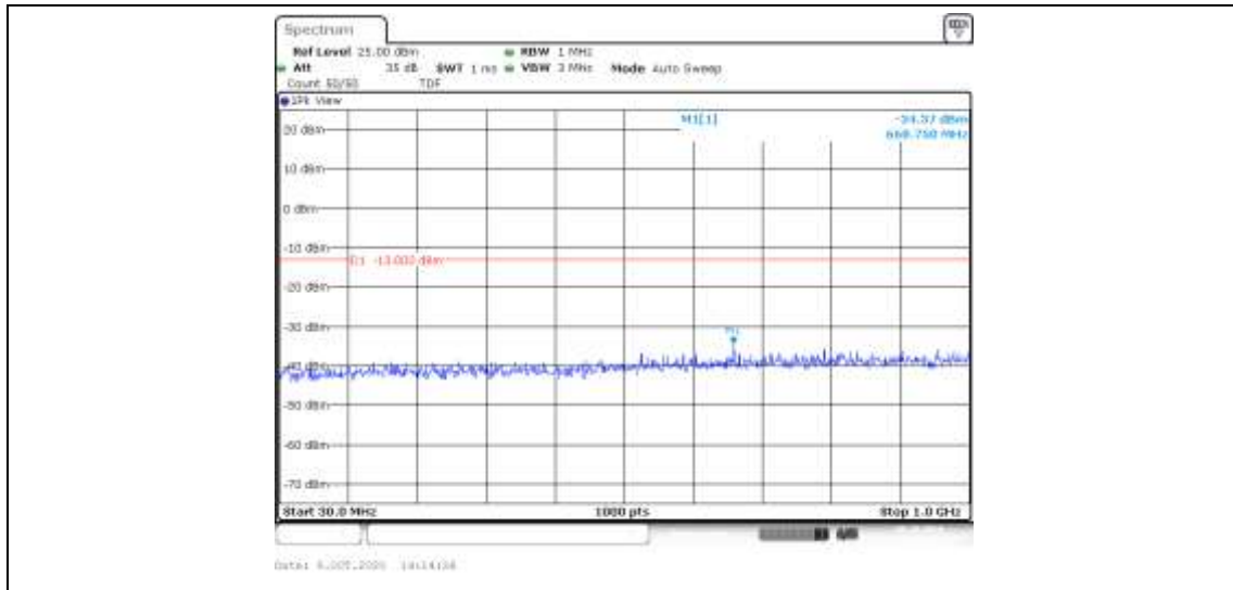
Band4-1.4MHz-QPSK-19957-6RB#0-Range1:30~1000MHz--34.37-PASS
