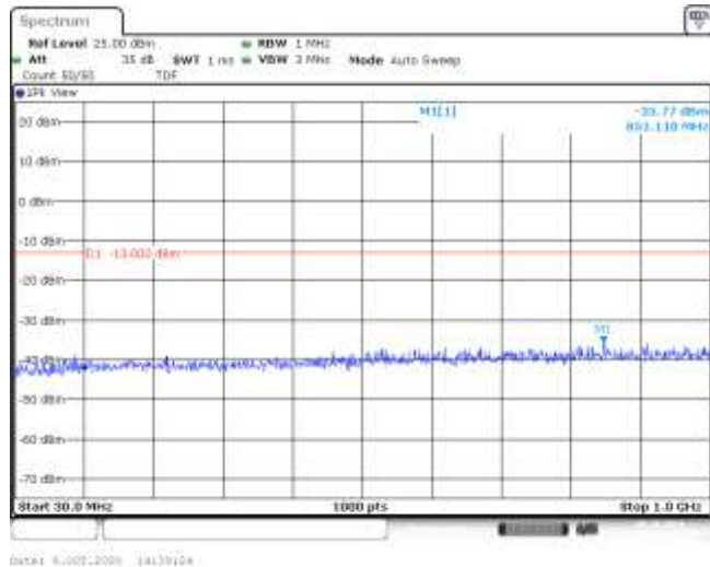
Band4-5MHz-QPSK-19975-25RB#0-Range1:30~1000MHz--35.77-PASS
