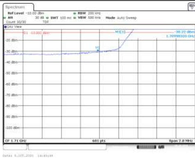
Band4-10MHz-16QAM-20000-50RB#0--30.22-PASS
