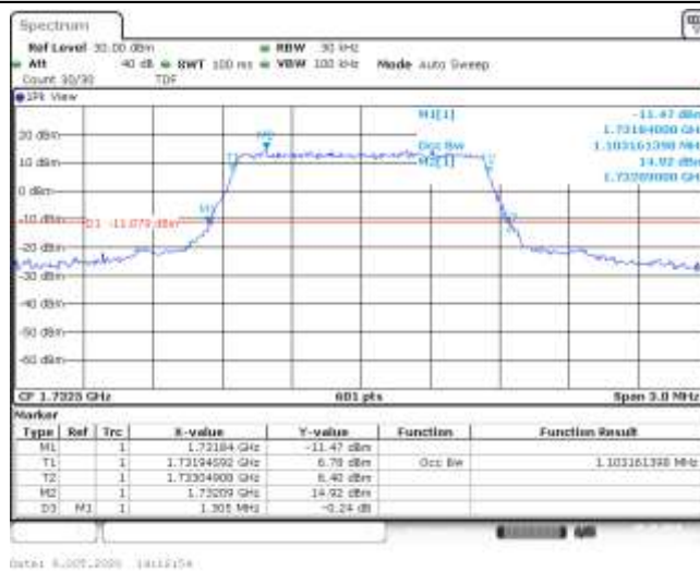
Band4-1.4MHz-16QAM-20175-6RB#0-1.103-1.305-PASS
