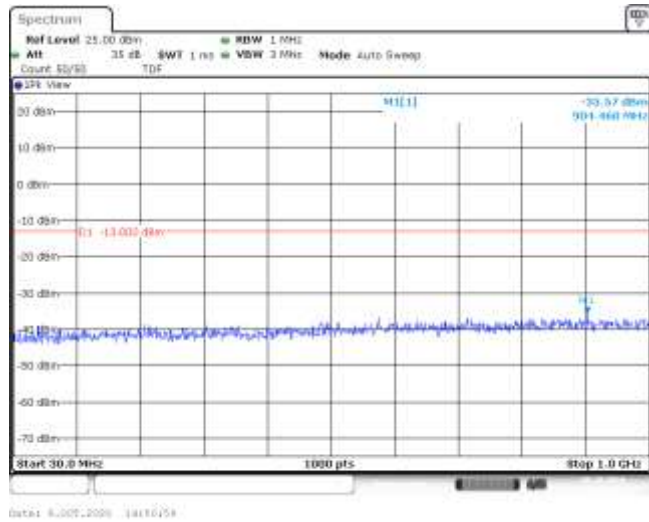
Band4-10MHz-16QAM-20000-50RB#0-Range1:30~1000MHz--35.57-PASS
