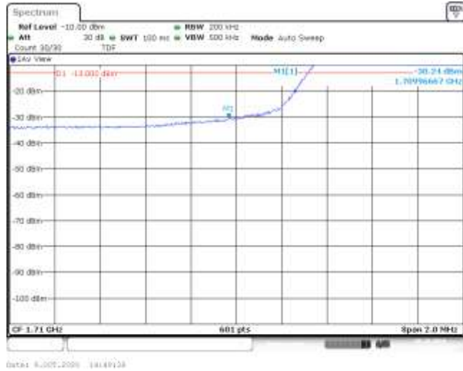
Band4-10MHz-QPSK-20000-50RB#0--30.24-PASS
