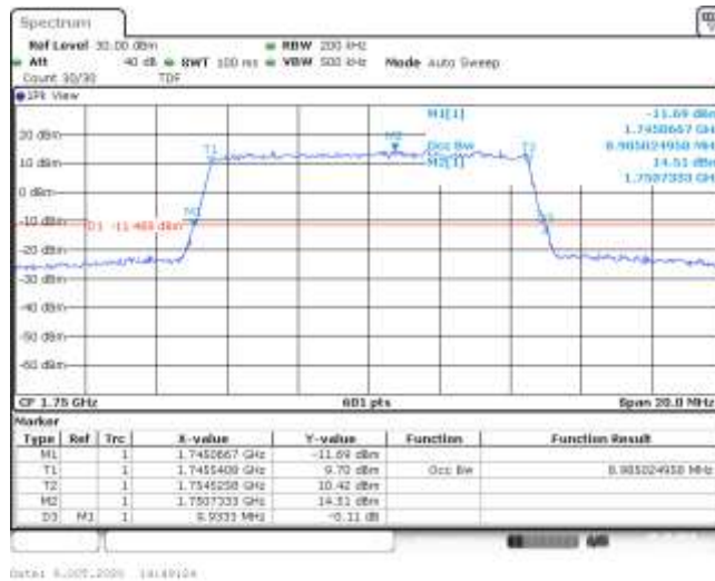
Band4-10MHz-16QAM-20350-50RB#0-8.985-9.933-PASS
