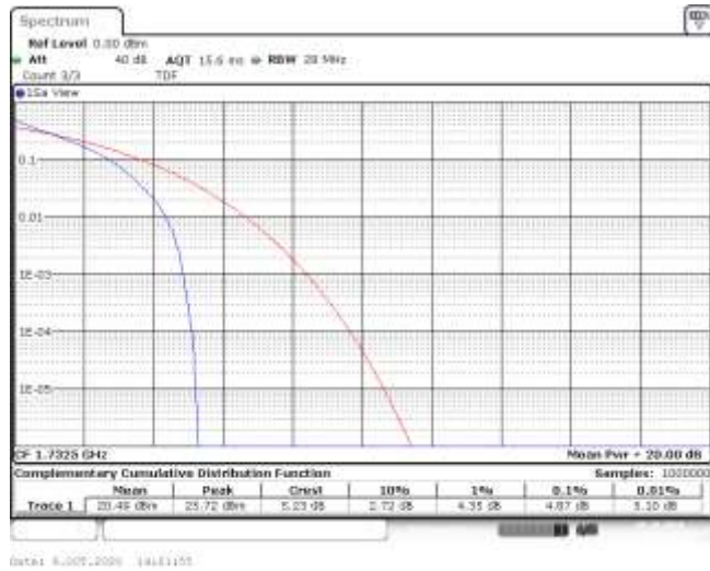
Band4-1.4MHz-QPSK-20175-6RB#0-4.87-13-PASS
