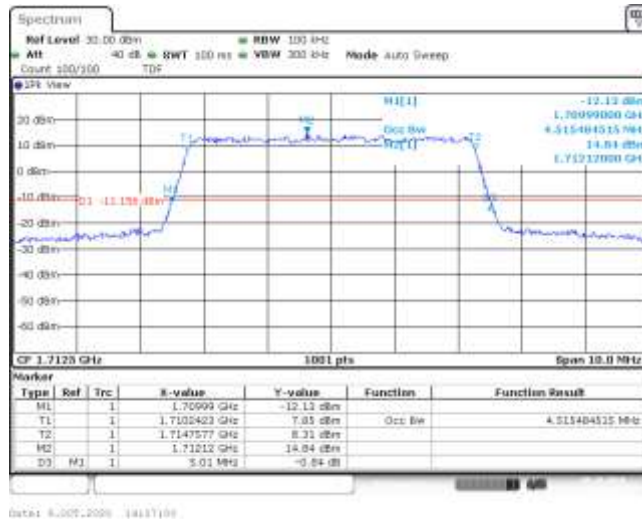
Band4-5MHz-16QAM-19975-25RB#0-4.515-5.010-PASS
