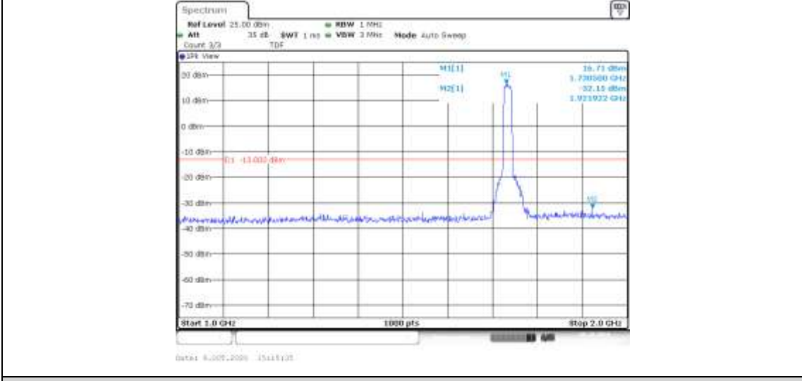
Band4-20MHz-16QAM-20175-100RB#0-Range2:1000~2000MHz--32.15-PASS
