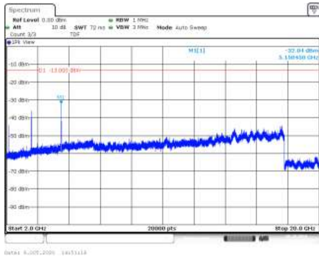
Band4-10MHz-16QAM-20000-50RB#0-Range3:2000~20000MHz--32.04-PASS
