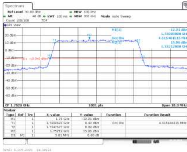
Band4-5MHz-16QAM-20375-25RB#0-4.515-5.010-PASS
