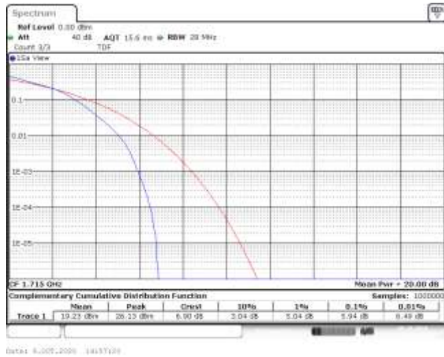
Band4-10MHz-16QAM-20000-50RB#0-5.94-13-PASS
