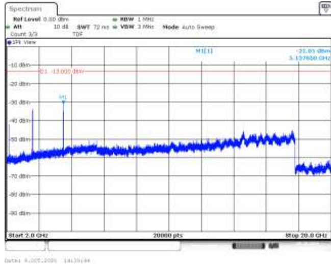
Band4-5MHz-QPSK-19975-25RB#0-Range3:2000~20000MHz--31.01-PASS
