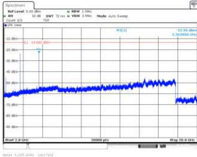
Band4-1.4MHz-16QAM-20393-6RB#0-Range3:2000~20000MHz--22.95-PASS
