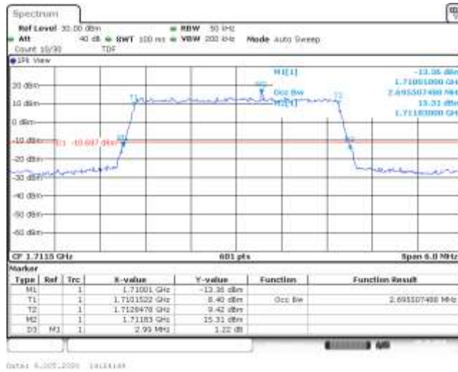
Band4-3MHz-QPSK-19965-15RB#0-2.696-2.990-PASS
