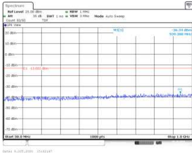
Band4-15MHz-QPSK-20175-75RB#0-Range1:30~1000MHz--36.34-PASS
