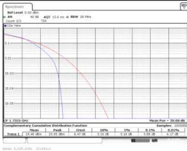
Band4-15MHz-16QAM-20175-75RB#0-5.88-13-PASS
