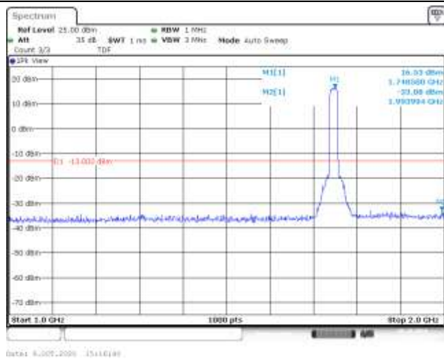
Band4-20MHz-16QAM-20300-100RB#0-Range2:1000~2000MHz--33.08-PASS
