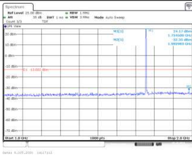
Band4-1.4MHz-16QAM-20393-6RB#0-Range2:1000~2000MHz--32.35-PASS
