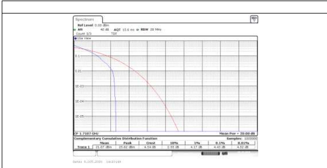
Band4-1.4MHz-QPSK-19957-1RB#0-4.43-13-PASS
