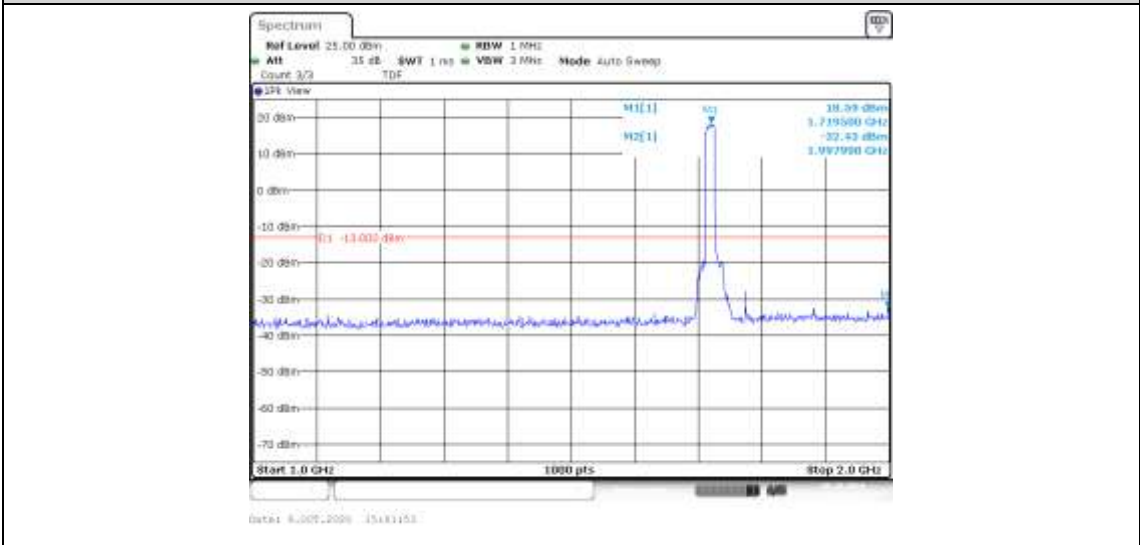
Band4-15MHz-QPSK-20025-75RB#0-Range2:1000~2000MHz--32.43-PASS
