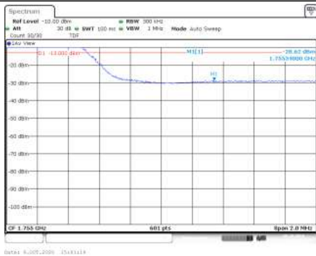
Band4-15MHz-QPSK-20325-75RB#0--28.62-PASS
