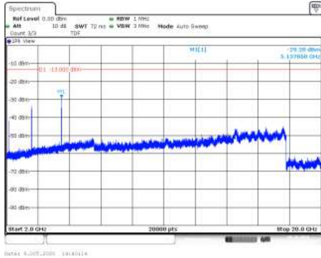
Band4-5MHz-16QAM-19975-25RB#0-Range3:2000~20000MHz--29.2-PASS
