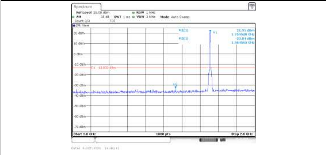
Band4-5MHz-16QAM-20375-25RB#0-Range2:1000~2000MHz--33.04-PASS
