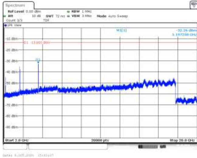
Band4-15MHz-QPSK-20175-75RB#0-Range3:2000~20000MHz--32.26-PASS
