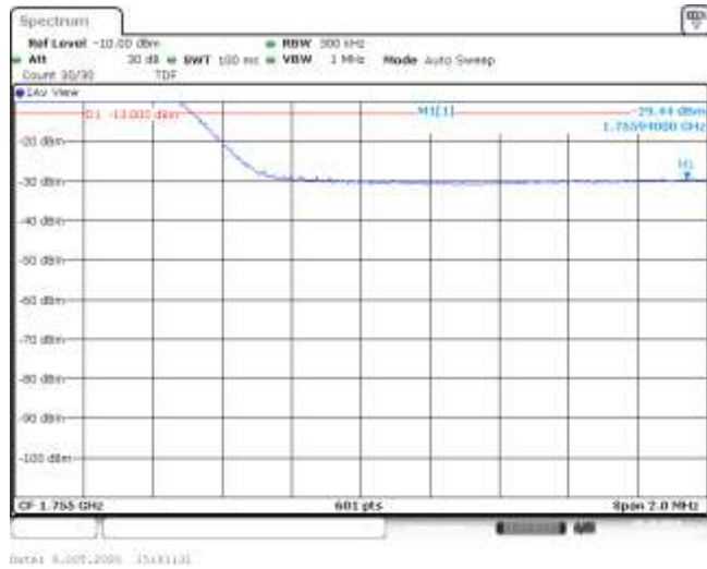
Band4-15MHz-16QAM-20325-75RB#0--29.44-PASS
