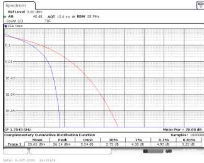
Band4-1.4MHz-QPSK-20393-6RB#0-4.93-13-PASS
