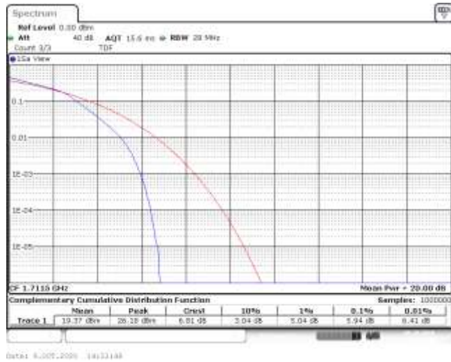
Band4-3MHz-16QAM-19965-15RB#0-5.94-13-PASS
