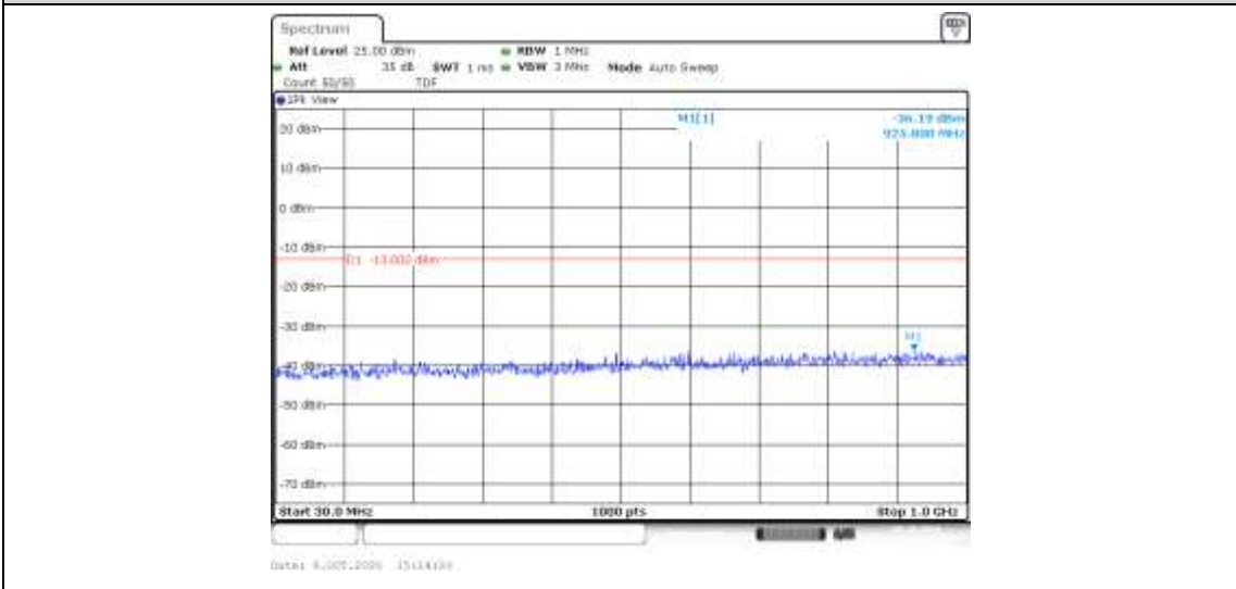
Band4-20MHz-16QAM-20050-100RB#0-Range1:30~1000MHz--36.19-PASS
