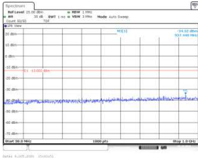
Band4-15MHz-QPSK-20325-75RB#0-Range1:30~1000MHz--34.52-PASS
