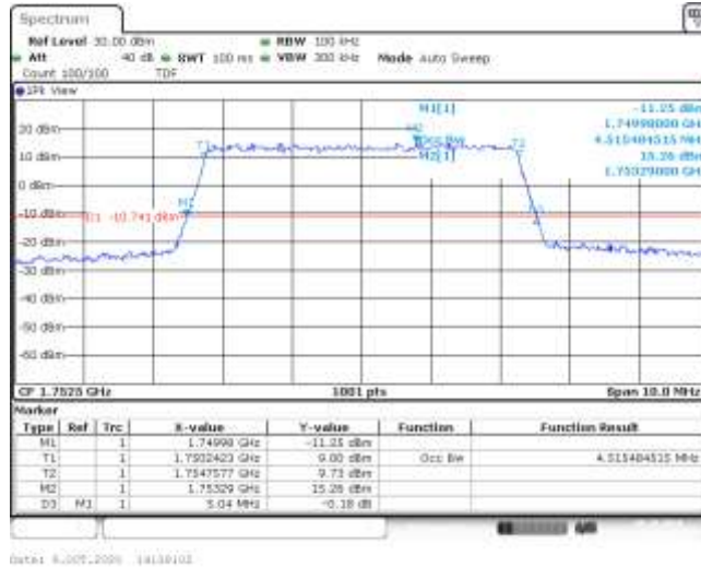
Band4-5MHz-QPSK-20375-25RB#0-4.515-5.040-PASS
