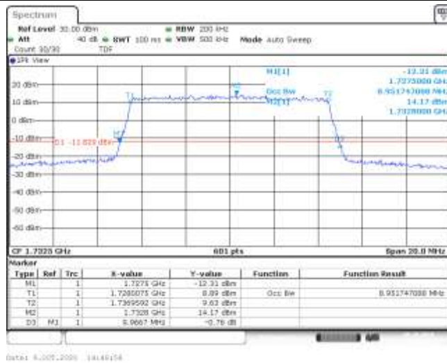
Band4-10MHz-16QAM-20175-50RB#0-8.952-9.967-PASS
