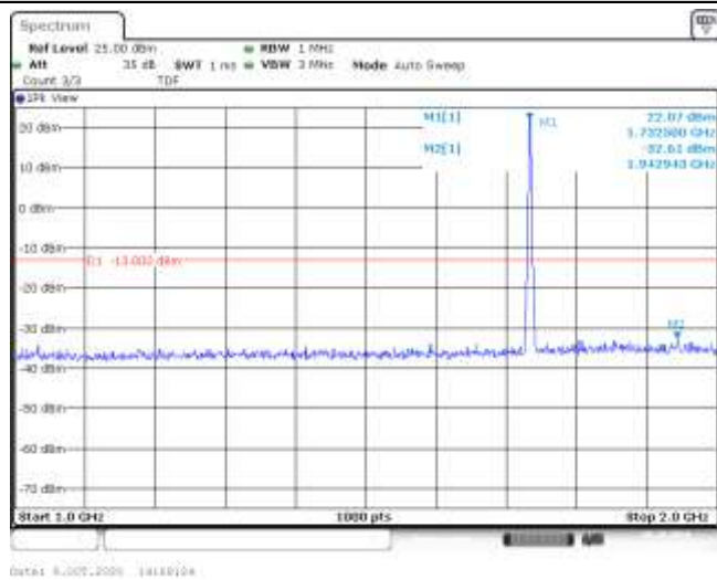
Band4-3MHz-QPSK-20175-15RB#0-Range2:1000~2000MHz--32.61-PASS
