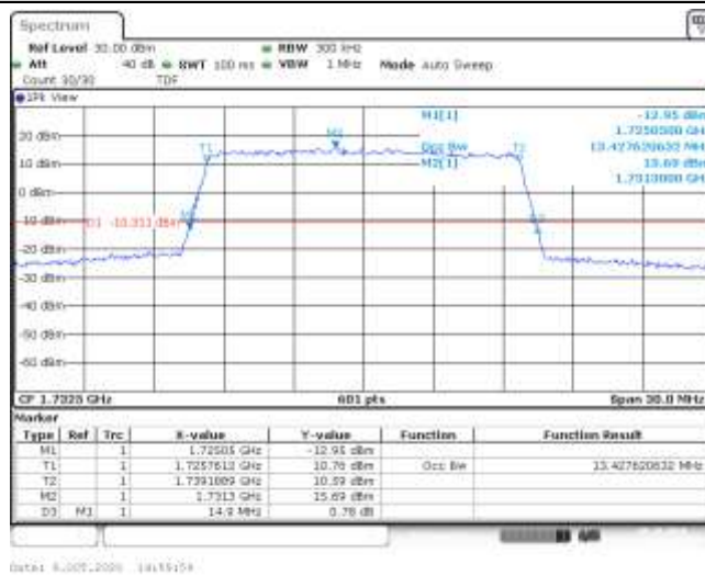
Band4-15MHz-QPSK-20175-75RB#0-13.428-14.900-PASS
