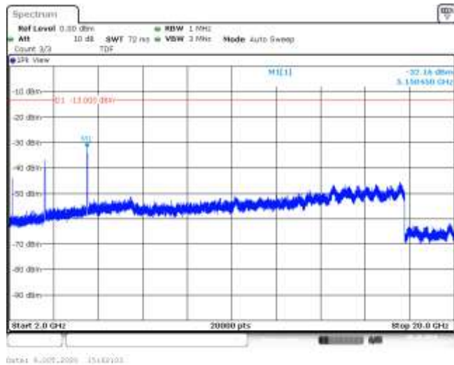
Band4-15MHz-QPSK-20025-75RB#0-Range3:2000~20000MHz--32.16-PASS
