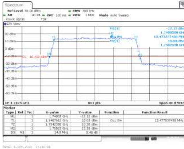
Band4-15MHz-QPSK-20325-75RB#0-13.478-14.900-PASS
