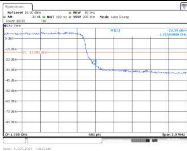
Band4-3MHz-QPSK-20385-15RB#0--25.39-PASS
