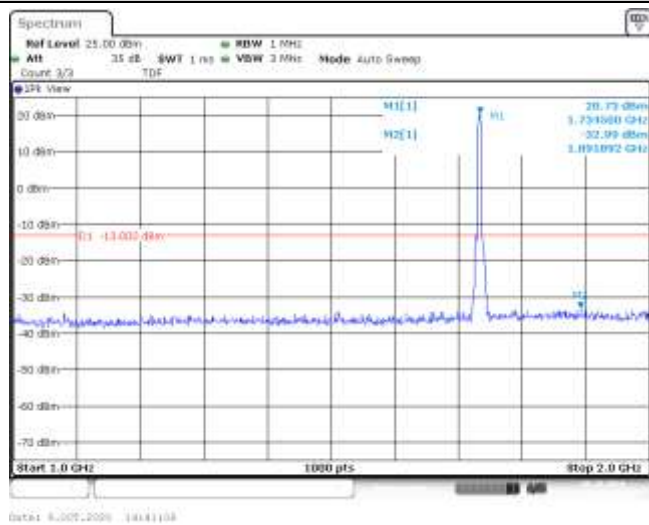
Band4-5MHz-16QAM-20175-25RB#0-Range2:1000~2000MHz--32.99-PASS
