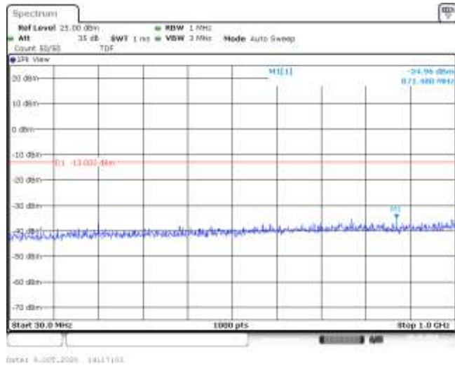
Band4-1.4MHz-16QAM-20393-6RB#0-Range1:30~1000MHz--34.96-PASS
