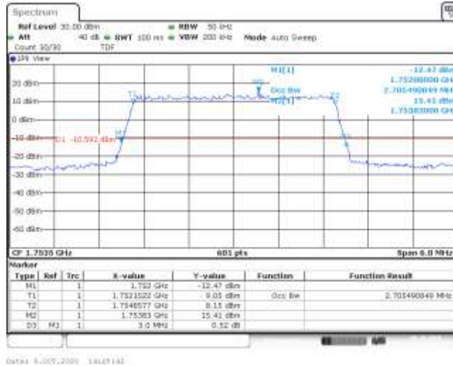
Band4-3MHz-QPSK-20385-15RB#0-2.705-3.000-PASS
