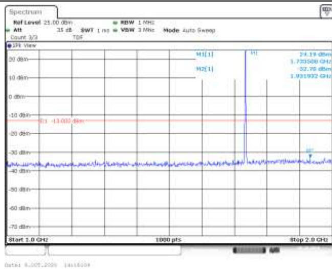
Band4-1.4MHz-16QAM-20175-6RB#0-Range2:1000~2000MHz--32.7-PASS
