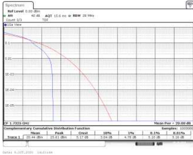
Band4-1.4MHz-16QAM-20175-1RB#0-5.10-13-PASS
