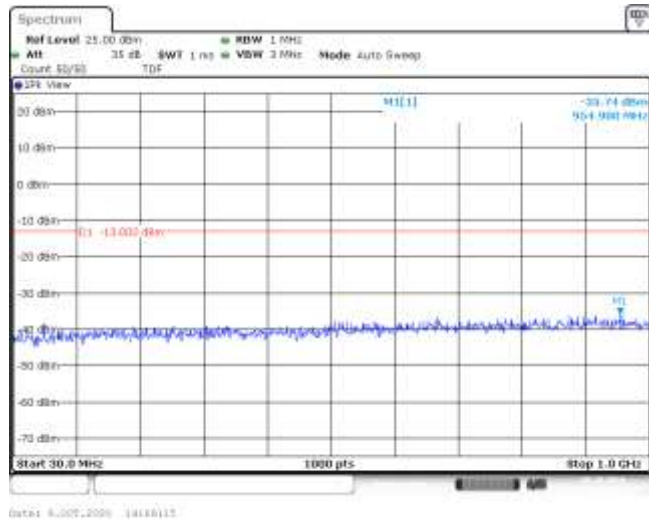
Band4-3MHz-QPSK-20175-15RB#0-Range1:30~1000MHz--35.74-PASS
