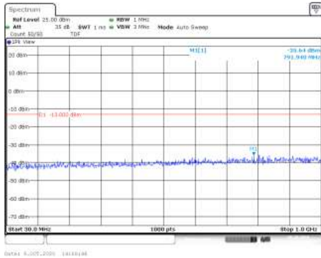
Band4-3MHz-16QAM-20175-15RB#0-Range1:30~1000MHz--35.64-PASS
