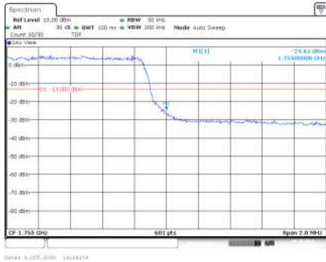
Band4-3MHz-16QAM-20385-15RB#0--24.61-PASS
