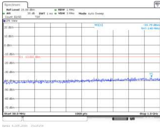
Band4-20MHz-QPSK-20300-100RB#0-Range1:30~1000MHz--35.79-PASS
