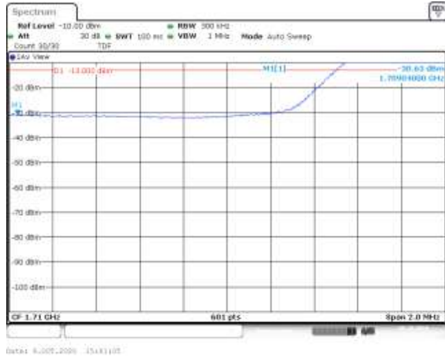
Band4-15MHz-16QAM-20025-75RB#0--30.63-PASS
