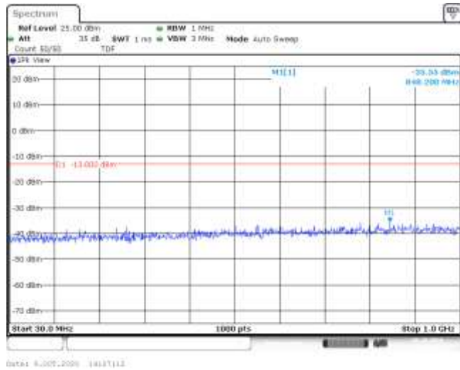
Band4-3MHz-QPSK-19965-15RB#0-Range1:30~1000MHz--35.55-PASS
