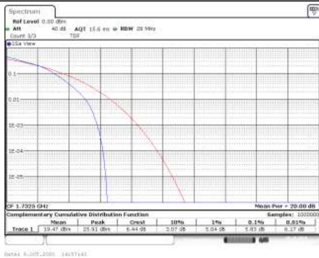
Band4-10MHz-16QAM-20175-50RB#0-5.83-13-PASS
