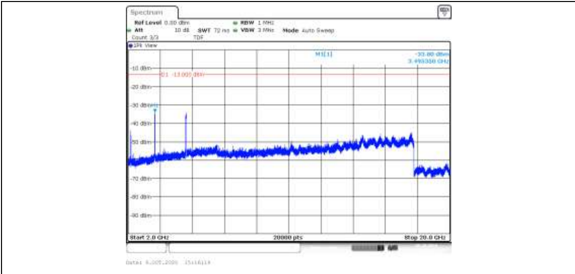
Band4-20MHz-QPSK-20300-100RB#0-Range3:2000~20000MHz--33.8-PASS
