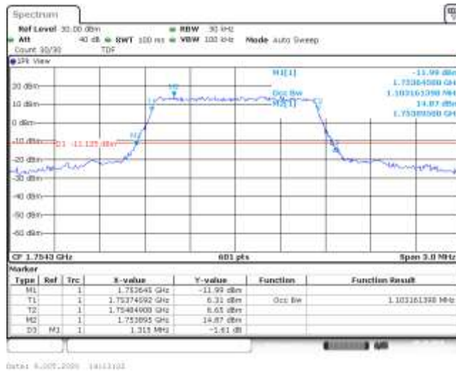
Band4-1.4MHz-16QAM-20393-6RB#0-1.103-1.315-PASS
