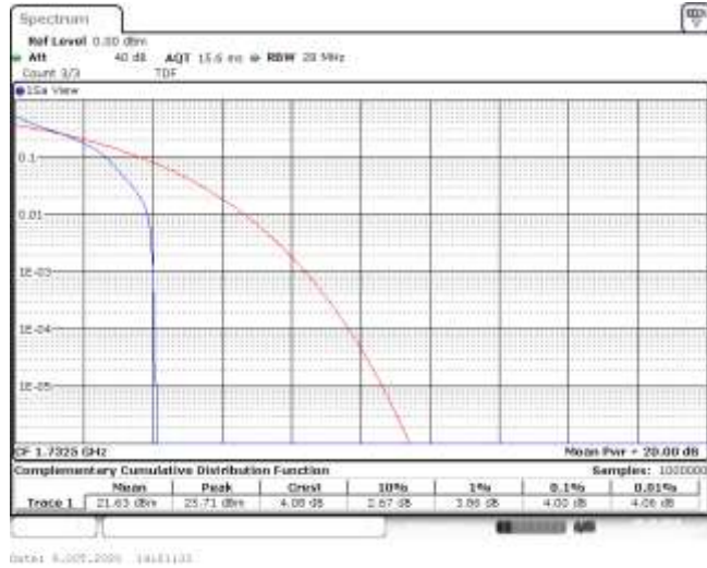
Band4-1.4MHz-QPSK-20175-1RB#0-4.00-13-PASS
