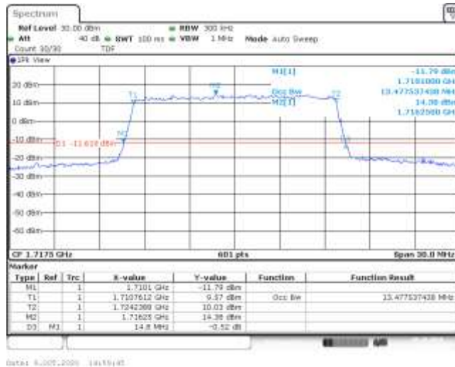
Band4-15MHz-16QAM-20025-75RB#0-13.478-14.800-PASS
