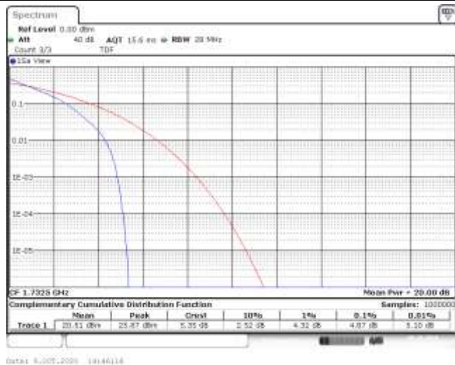
Band4-5MHz-QPSK-20175-25RB#0-4.87-13-PASS
