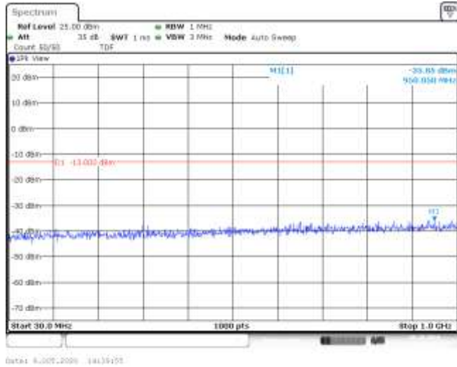
Band4-5MHz-16QAM-19975-25RB#0-Range1:30~1000MHz--35.85-PASS
