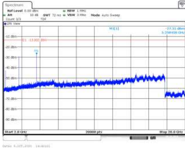
Band4-5MHz-16QAM-20375-25RB#0-Range3:2000~20000MHz--27.31-PASS
