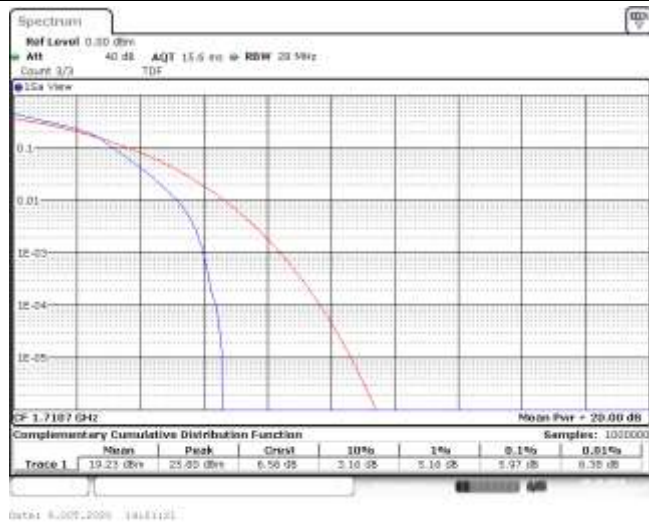
Band4-1.4MHz-16QAM-19957-6RB#0-5.97-13-PASS
