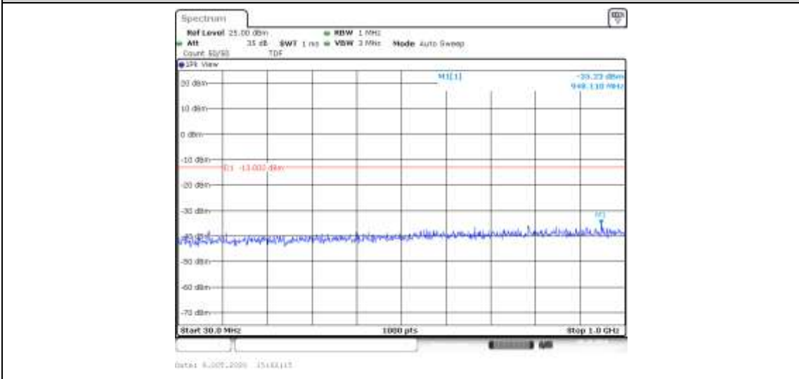
Band4-15MHz-16QAM-20025-75RB#0-Range1:30~1000MHz--35.23-PASS
