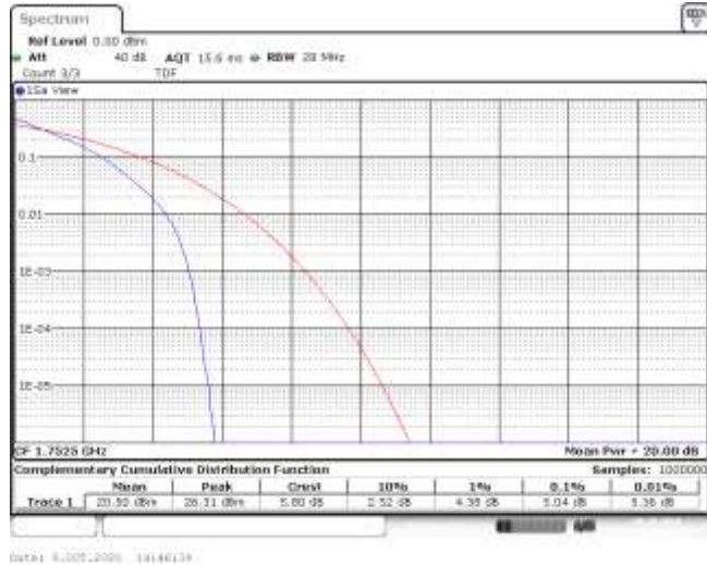
Band4-5MHz-QPSK-20375-25RB#0-5.04-13-PASS
