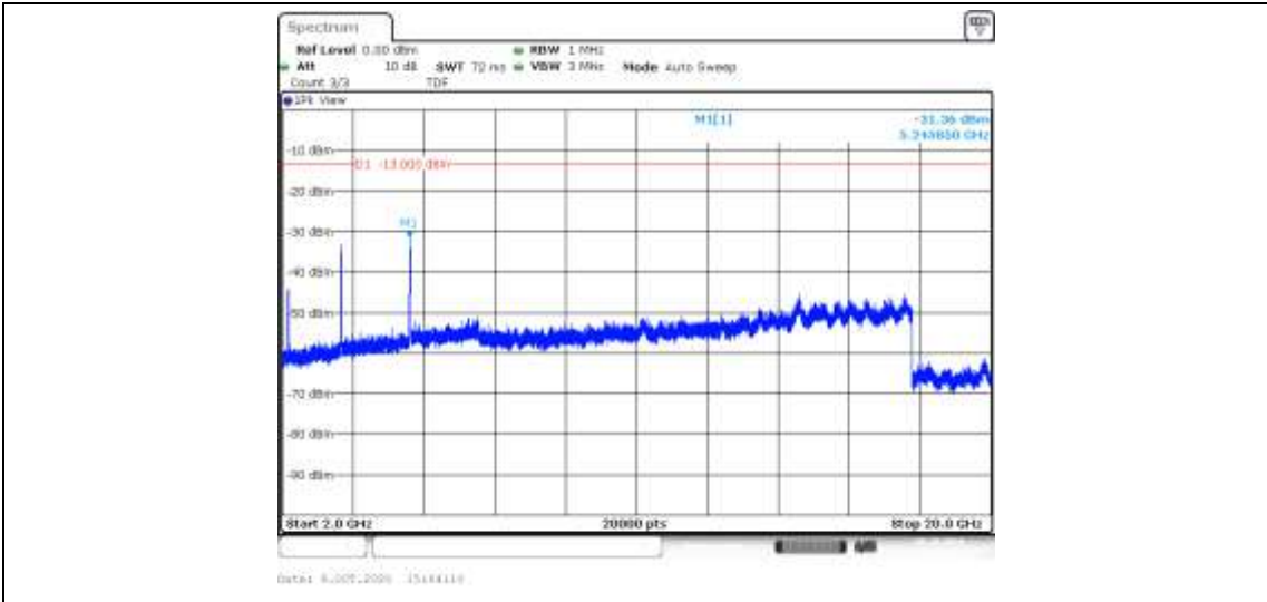
Band4-15MHz-QPSK-20325-75RB#0-Range3:2000~20000MHz--31.36-PASS
