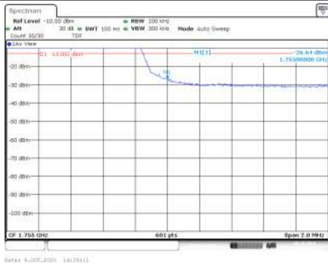
Band4-5MHz-16QAM-20375-25RB#0--26.64-PASS
