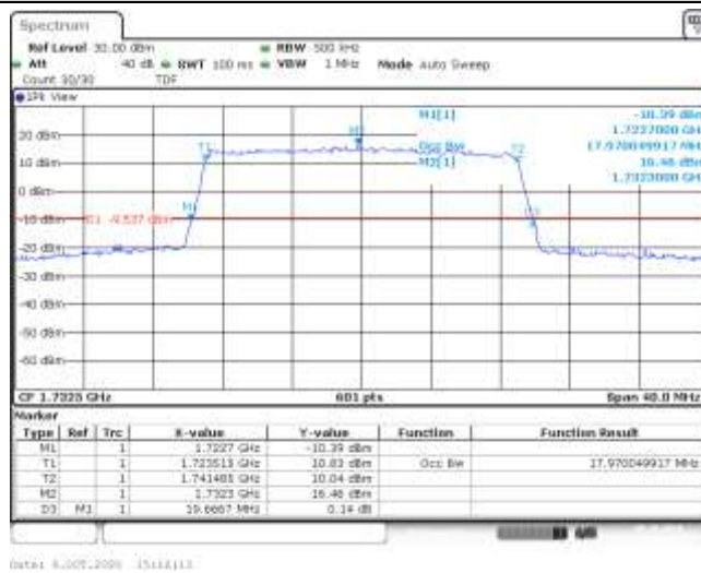
Band4-20MHz-16QAM-20175-100RB#0-17.97-19.667-PASS
