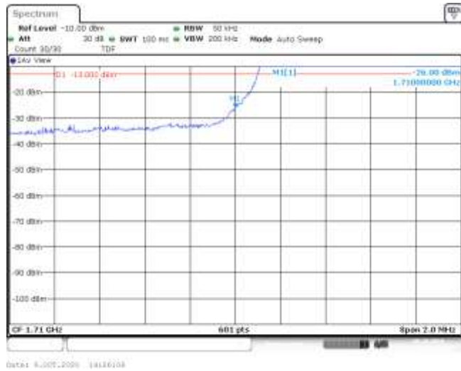
Band4-3MHz-QPSK-19965-15RB#0--26.00-PASS
