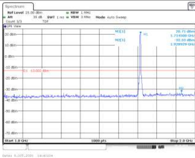
Band4-5MHz-16QAM-19975-25RB#0-Range2:1000~2000MHz--32.53-PASS
