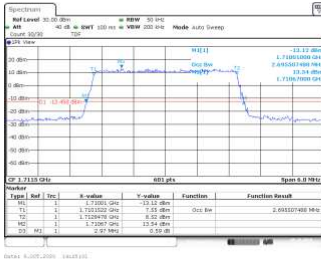
Band4-3MHz-16QAM-19965-15RB#0-2.696-2.970-PASS
