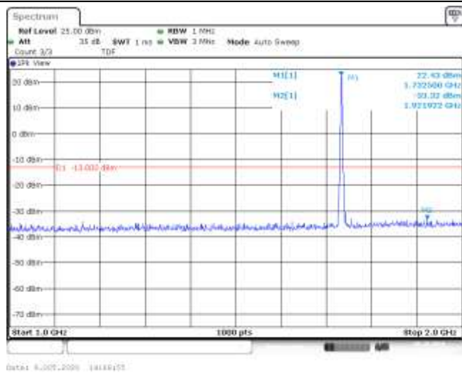
Band4-3MHz-16QAM-20175-15RB#0-Range2:1000~2000MHz--33.32-PASS
