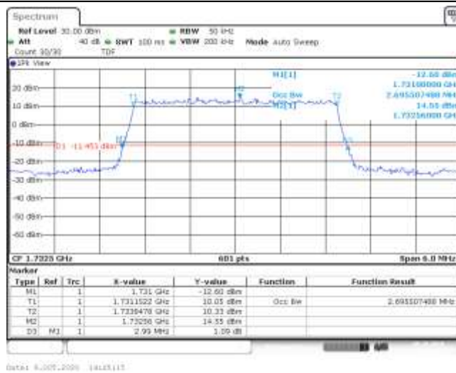
Band4-3MHz-QPSK-20175-15RB#0-2.696-2.990-PASS
