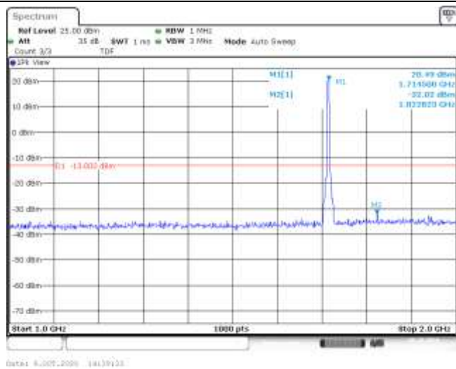
Band4-5MHz-QPSK-19975-25RB#0-Range2:1000~2000MHz--32.02-PASS
