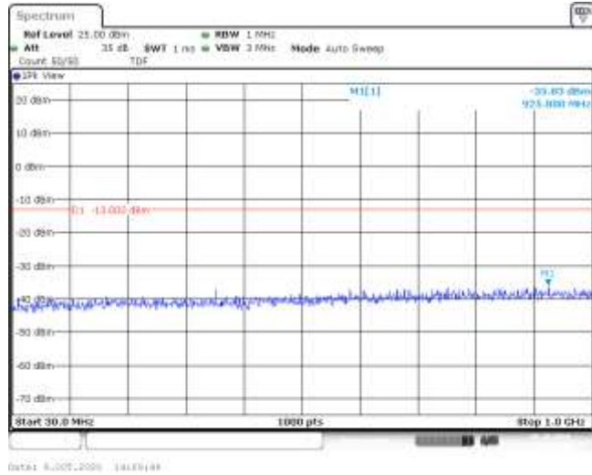
Band4-3MHz-16QAM-20385-15RB#0-Range1:30~1000MHz--35.83-PASS
