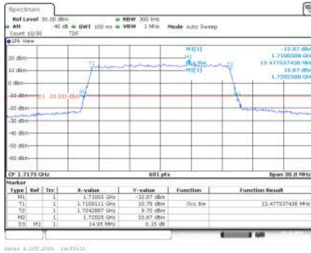
Band4-15MHz-QPSK-20025-75RB#0-13.478-14.950-PASS
