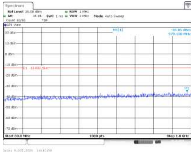
Band4-5MHz-16QAM-20175-25RB#0-Range1:30~1000MHz--35.81-PASS
