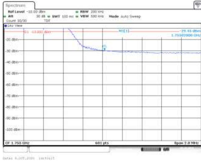
Band4-10MHz-16QAM-20350-50RB#0--29.45-PASS
