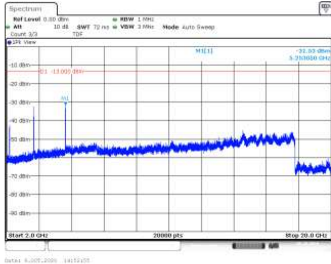
Band4-10MHz-QPSK-20350-50RB#0-Range3:2000~20000MHz--31.53-PASS
