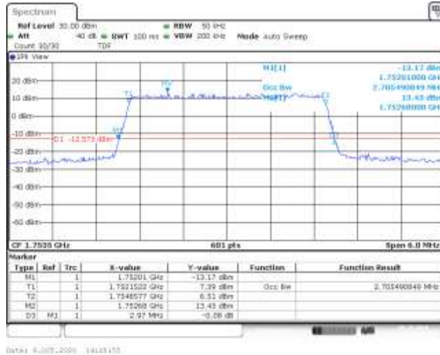
Band4-3MHz-16QAM-20385-15RB#0-2.705-2.970-PASS
