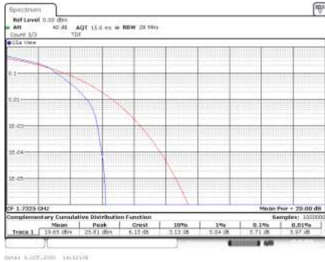
Band4-1.4MHz-16QAM-20175-6RB#0-5.71-13-PASS
