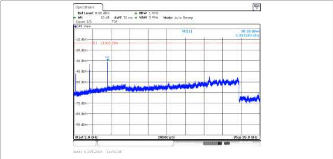
Band4-10MHz-16QAM-20350-50RB#0-Range3:2000~20000MHz--30.2-PASS
