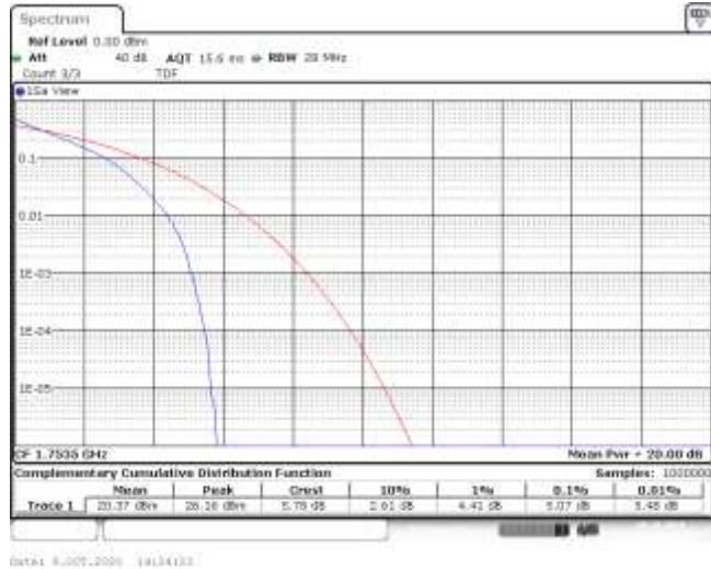
Band4-3MHz-QPSK-20385-15RB#0-5.07-13-PASS
