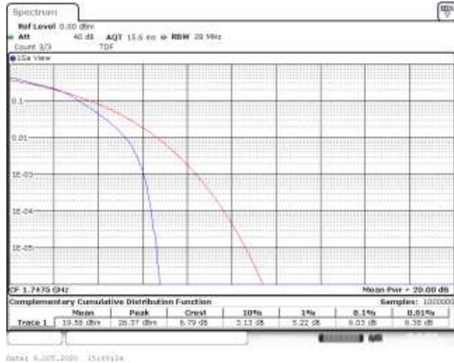
Band4-15MHz-16QAM-20325-75RB#0-6.03-13-PASS
