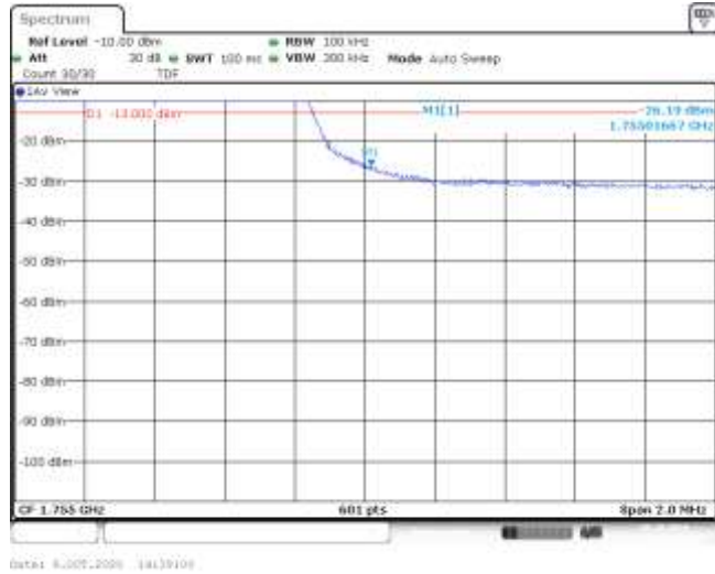
Band4-5MHz-QPSK-20375-25RB#0--26.19-PASS
