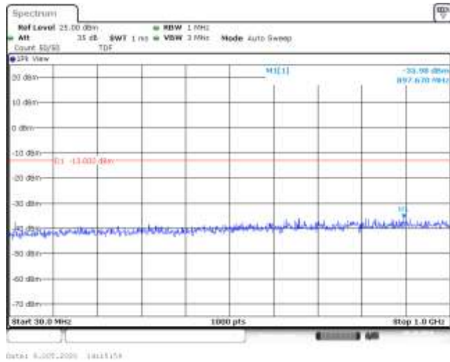
Band4-1.4MHz-16QAM-20175-6RB#0-Range1:30~1000MHz--35.98-PASS
