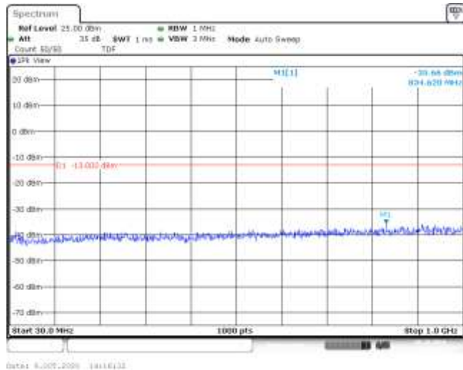
Band4-1.4MHz-QPSK-20393-6RB#0-Range1:30~1000MHz--35.66-PASS
