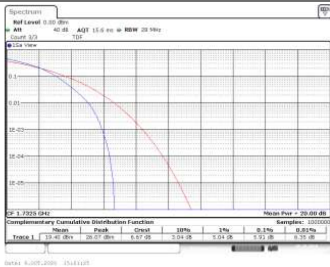
Band4-20MHz-16QAM-20175-100RB#0-5.91-13-PASS
