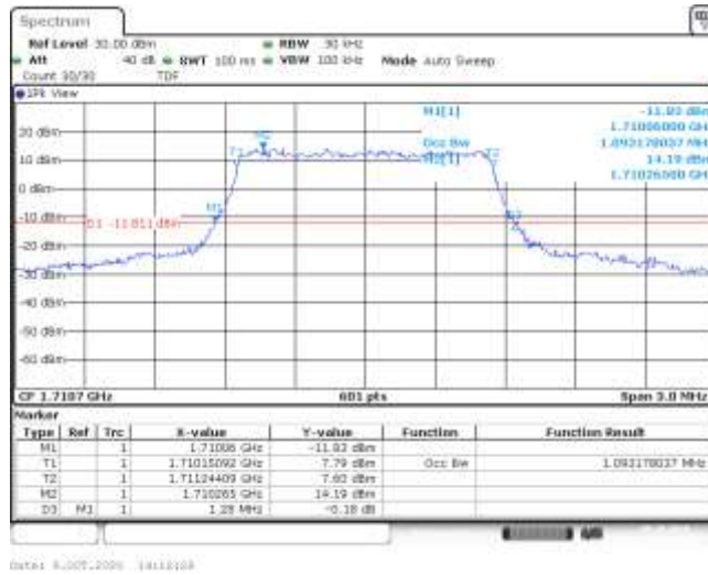
Band4-1.4MHz-16QAM-19957-6RB#0-1.093-1.280-PASS
