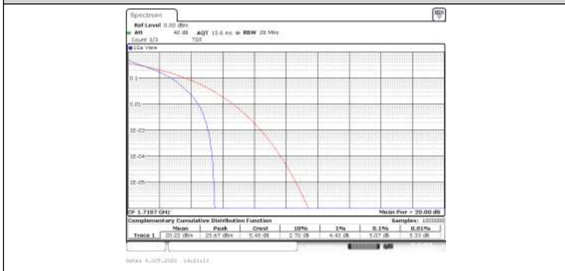
Band4-1.4MHz-QPSK-19957-6RB#0-5.07-13-PASS
