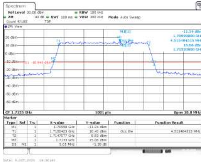
Band4-5MHz-QPSK-19975-25RB#0-4.515-5.050-PASS
