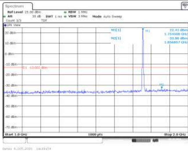
Band4-3MHz-16QAM-20385-15RB#0-Range2:1000~2000MHz--33.06-PASS
