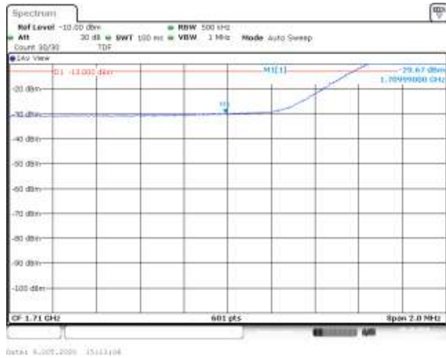
Band4-20MHz-16QAM-20050-100RB#0--29.67-PASS
