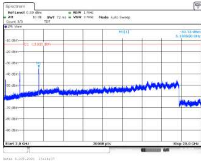
Band4-20MHz-QPSK-20050-100RB#0-Range3:2000~20000MHz--33.75-PASS
