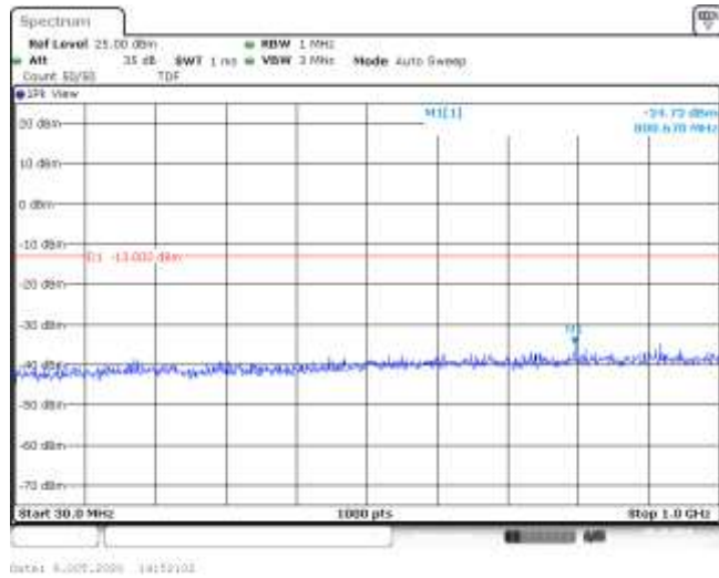
Band4-10MHz-16QAM-20175-50RB#0-Range1:30~1000MHz--34.73-PASS
