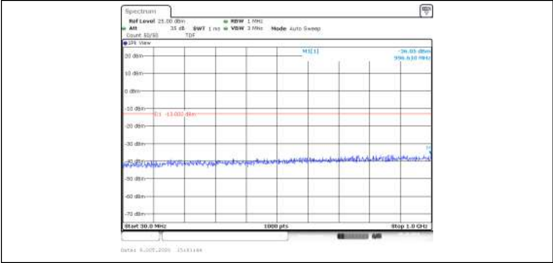
Band4-15MHz-QPSK-20025-75RB#0-Range1:30~1000MHz--36.05-PASS
