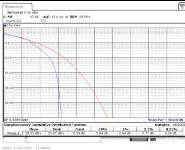
Band4-5MHz-16QAM-20175-25RB#0-5.77-13-PASS
