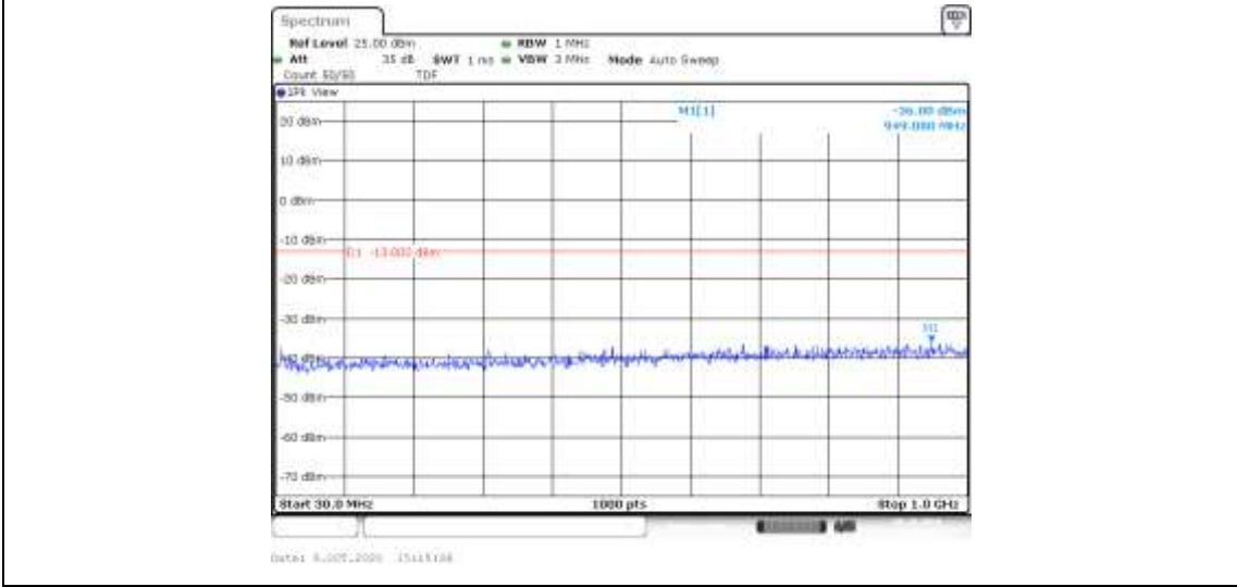
Band4-20MHz-16QAM-20175-100RB#0-Range1:30~1000MHz--36-PASS
