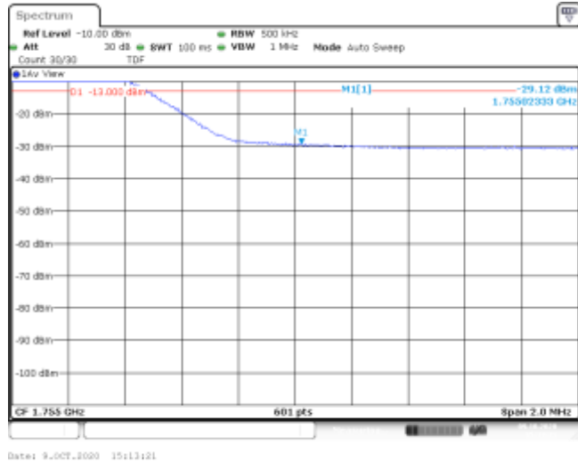
Band4-20MHz-QPSK-20300-100RB#0--29.12-PASS
