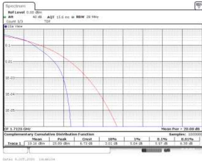
Band4-5MHz-16QAM-19975-25RB#0-5.97-13-PASS
