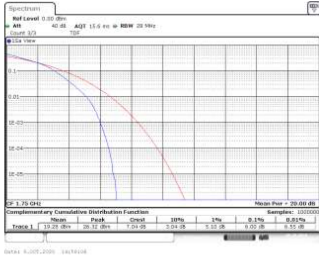
Band4-10MHz-16QAM-20350-50RB#0-6.00-13-PASS
