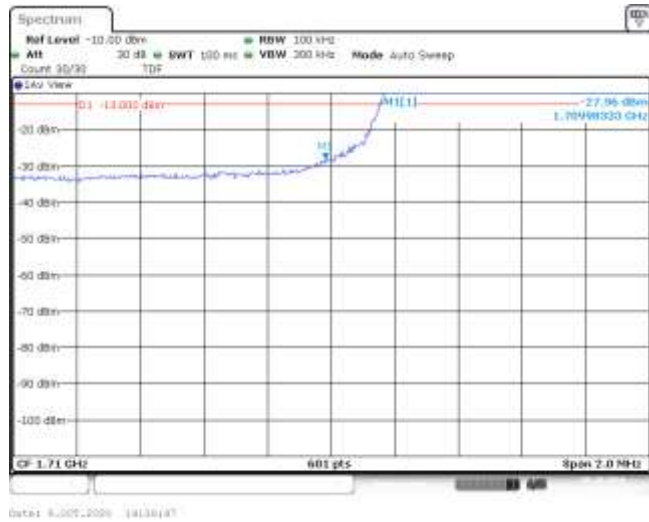
Band4-5MHz-16QAM-19975-25RB#0--27.96-PASS
