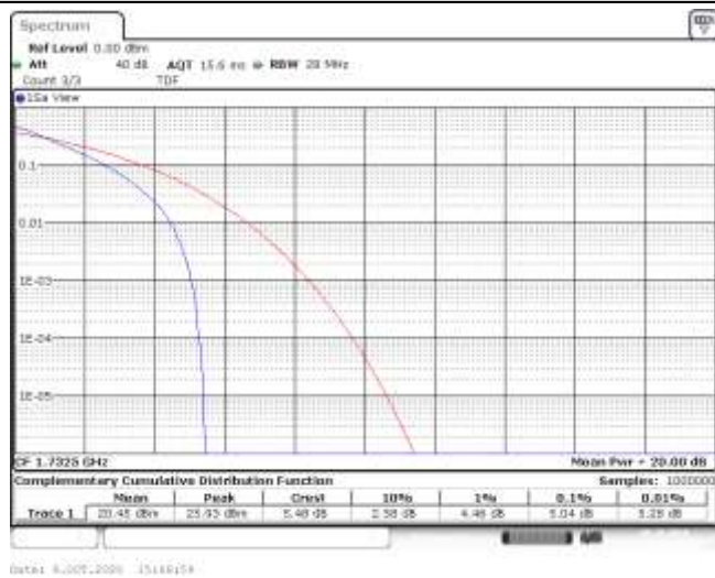
Band4-15MHz-QPSK-20175-75RB#0-5.04-13-PASS
