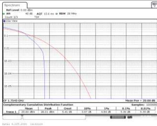
Band4-1.4MHz-16QAM-20393-1RB#0-5.30-13-PASS
