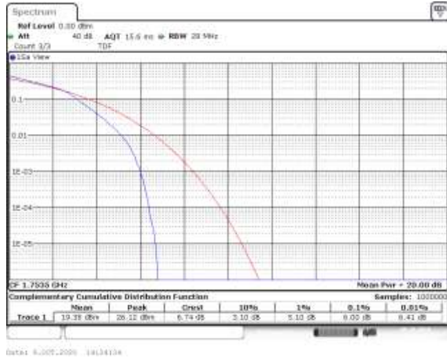
Band4-3MHz-16QAM-20385-15RB#0-6.00-13-PASS
