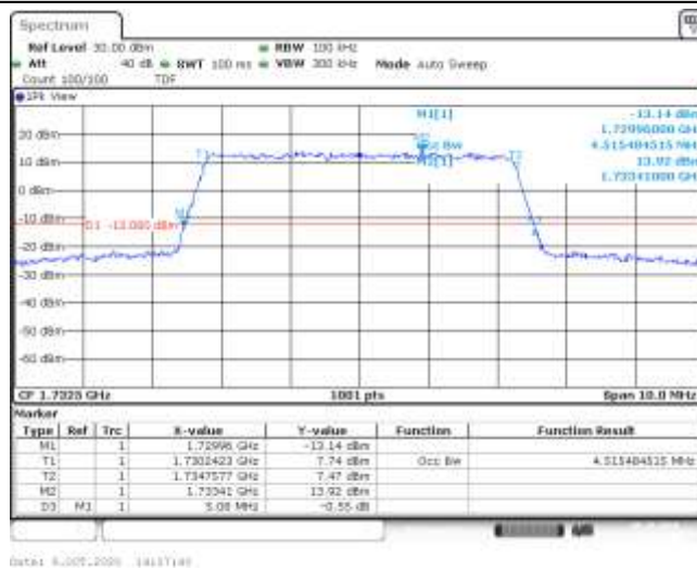
Band4-5MHz-16QAM-20175-25RB#0-4.515-5.080-PASS
