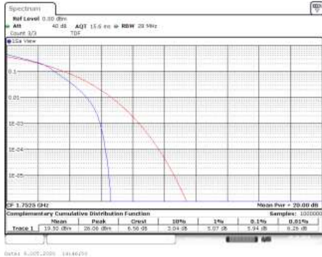
Band4-5MHz-16QAM-20375-25RB#0-5.94-13-PASS
