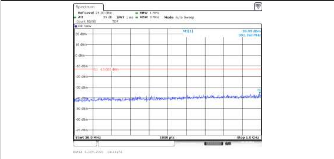
Band4-1.4MHz-16QAM-19957-6RB#0-Range1:30~1000MHz--35.93-PASS
