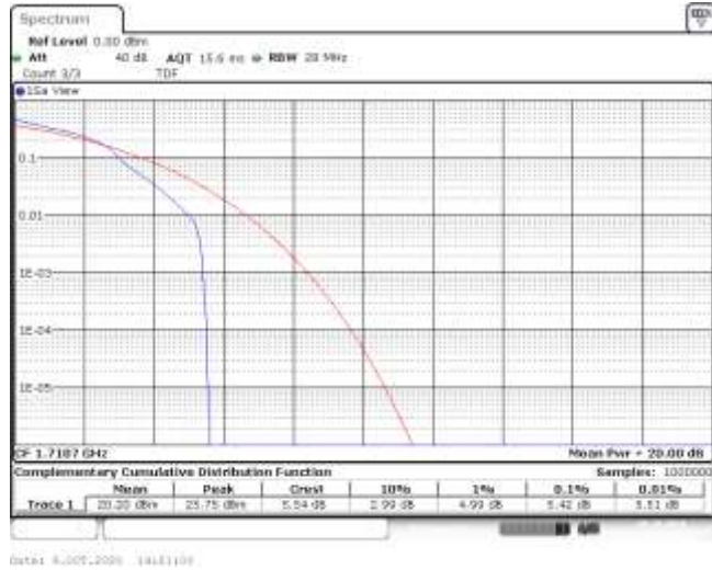
Band4-1.4MHz-16QAM-19957-1RB#0-5.42-13-PASS
