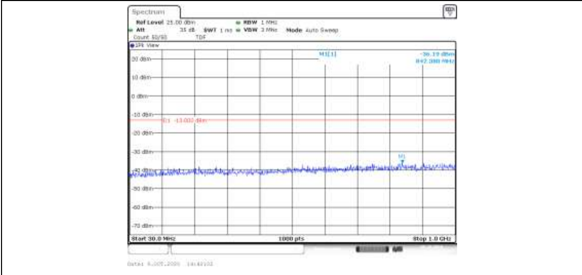
Band4-5MHz-16QAM-20375-25RB#0-Range1:30~1000MHz--36.19-PASS
