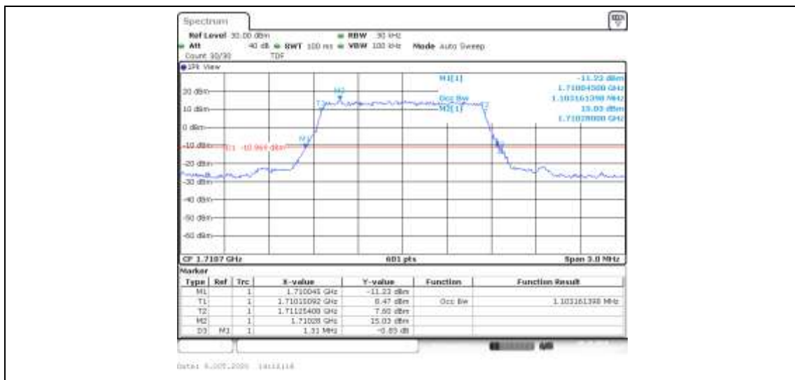
Band4-1.4MHz-QPSK-19957-6RB#0-1.103-1.310-PASS
