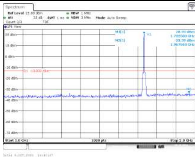
Band4-5MHz-QPSK-20175-25RB#0-Range2:1000~2000MHz--33.39-PASS
