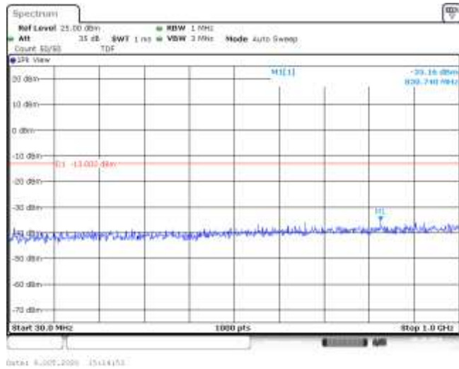
Band4-20MHz-QPSK-20175-100RB#0-Range1:30~1000MHz--35.16-PASS
