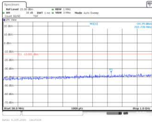
Band4-1.4MHz-QPSK-20175-6RB#0-Range1:30~1000MHz--34.79-PASS
