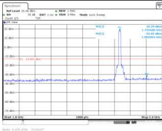
Band4-15MHz-QPSK-20175-75RB#0-Range2:1000~2000MHz--33.05-PASS
