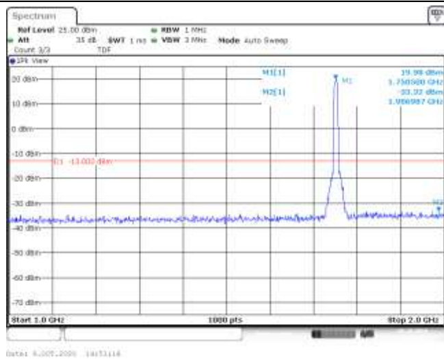
Band4-10MHz-16QAM-20350-50RB#0-Range2:1000~2000MHz--33.32-PASS
