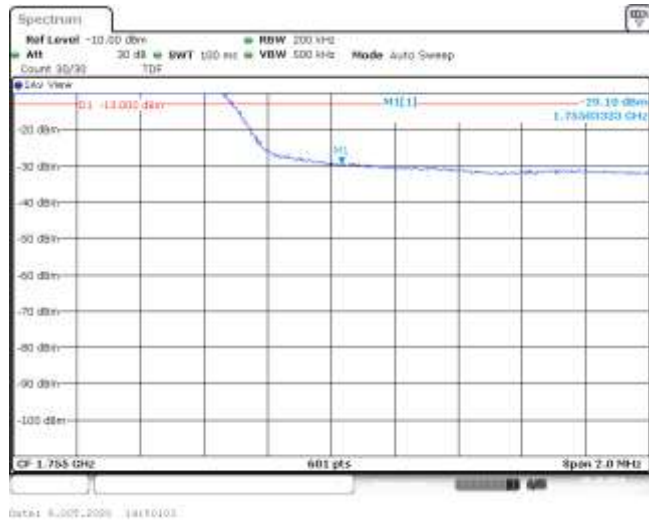
Band4-10MHz-QPSK-20350-50RB#0--29.10-PASS
