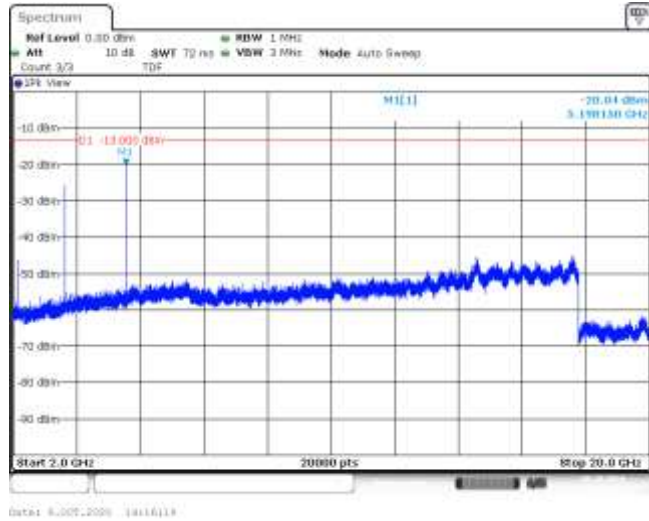
Band4-1.4MHz-16QAM-20175-6RB#0-Range3:2000~20000MHz--20.04-PASS
