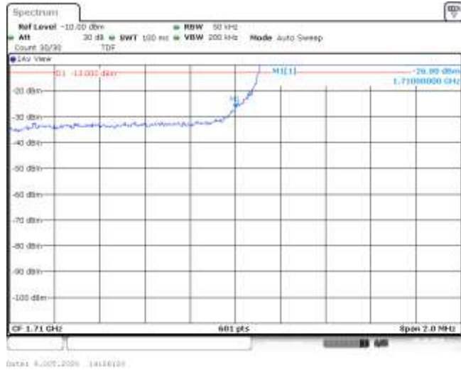
Band4-3MHz-16QAM-19965-15RB#0--26.80-PASS
