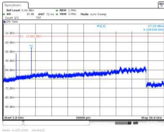
Band4-3MHz-16QAM-19965-15RB#0-Range3:2000~20000MHz--27.23-PASS
