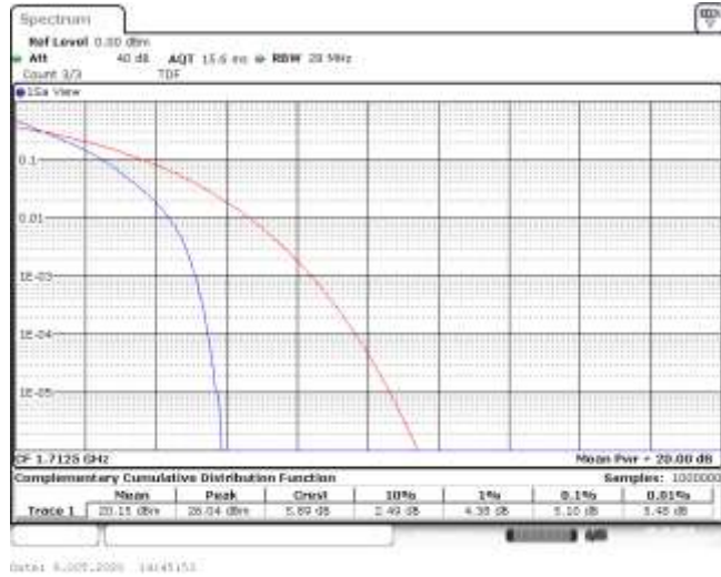
Band4-5MHz-QPSK-19975-25RB#0-5.10-13-PASS
