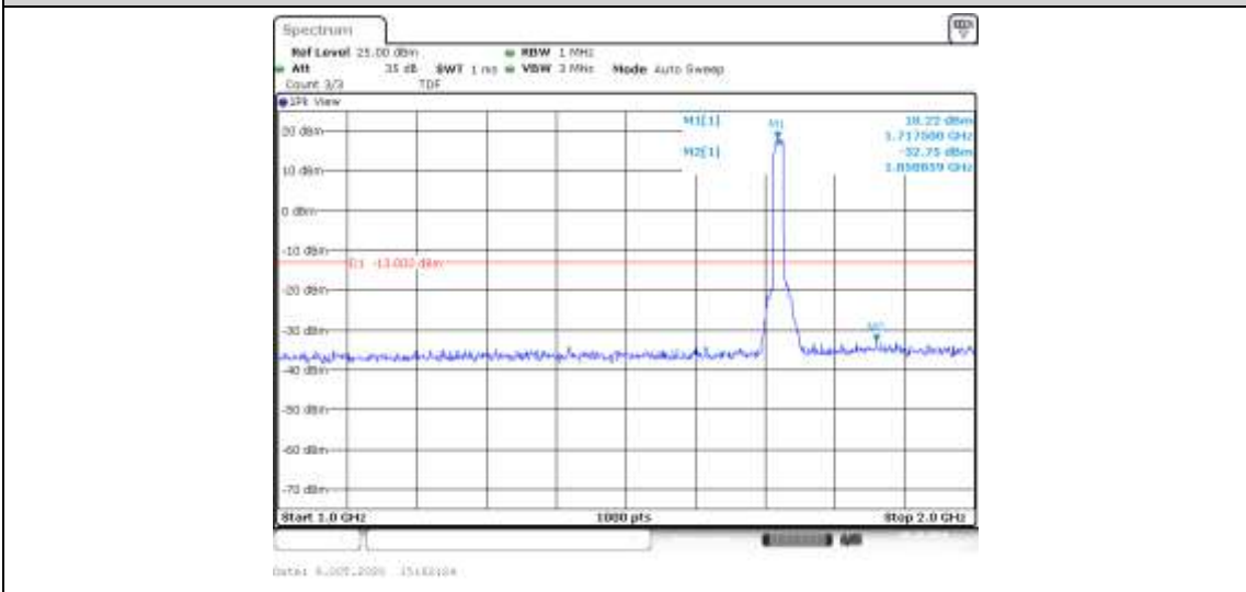
Band4-15MHz-16QAM-20025-75RB#0-Range2:1000~2000MHz--32.75-PASS
