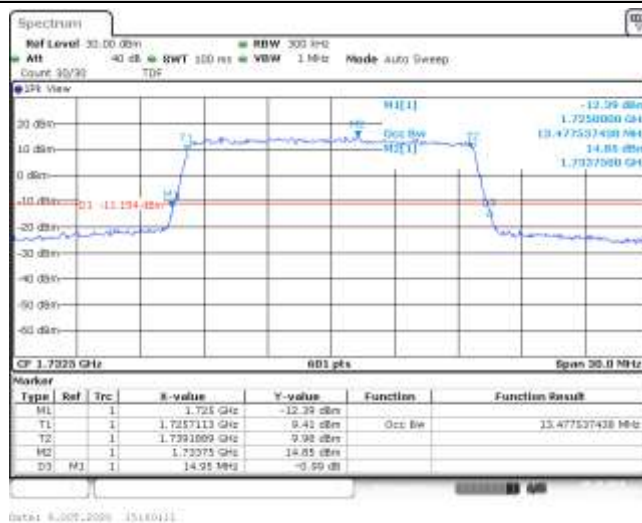
Band4-15MHz-16QAM-20175-75RB#0-13.478-14.950-PASS
