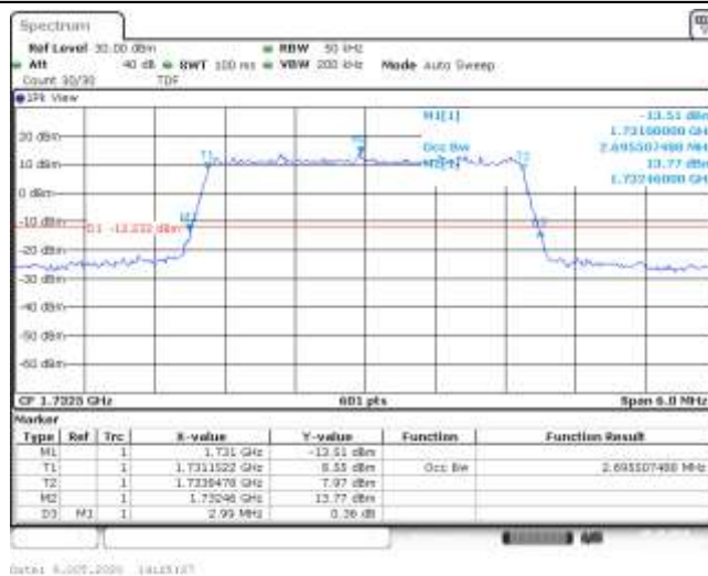
Band4-3MHz-16QAM-20175-15RB#0-2.696-2.990-PASS
