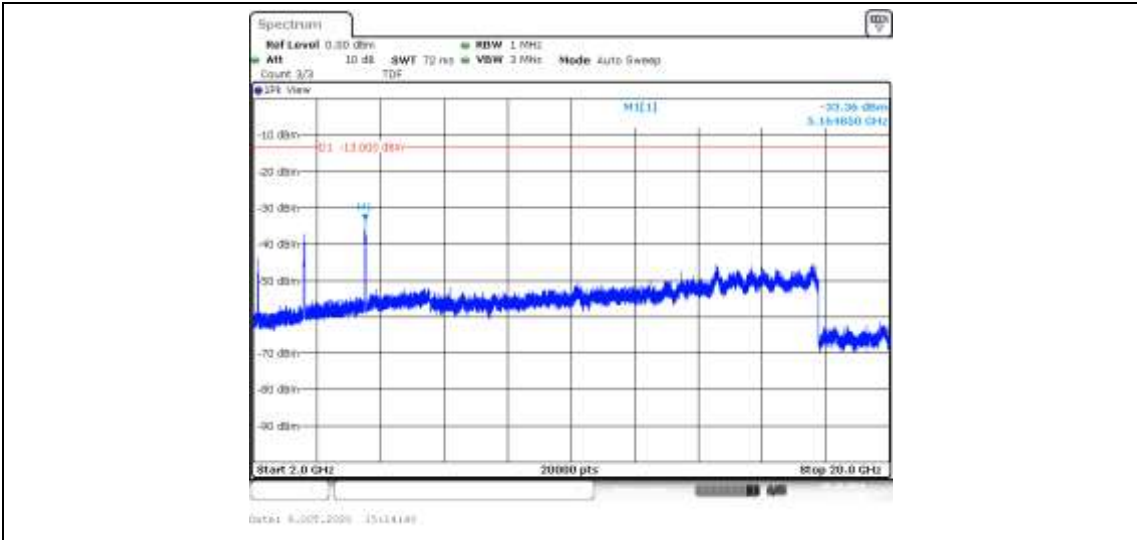
Band4-20MHz-16QAM-20050-100RB#0-Range3:2000~20000MHz--33.36-PASS
