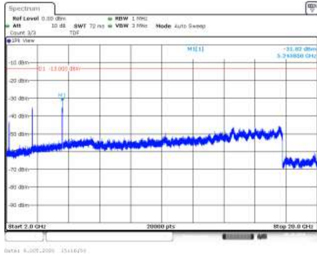
Band4-20MHz-16QAM-20300-100RB#0-Range3:2000~20000MHz--31.82-PASS
