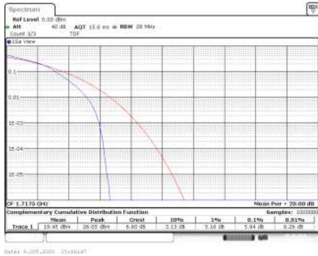
Band4-15MHz-16QAM-20025-75RB#0-5.94-13-PASS
