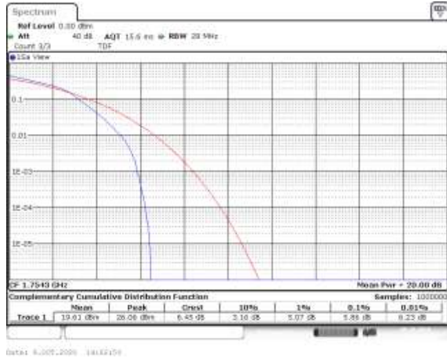
Band4-1.4MHz-16QAM-20393-6RB#0-5.86-13-PASS
