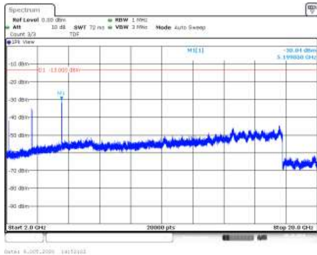
Band4-10MHz-16QAM-20175-50RB#0-Range3:2000~20000MHz--30.04-PASS
