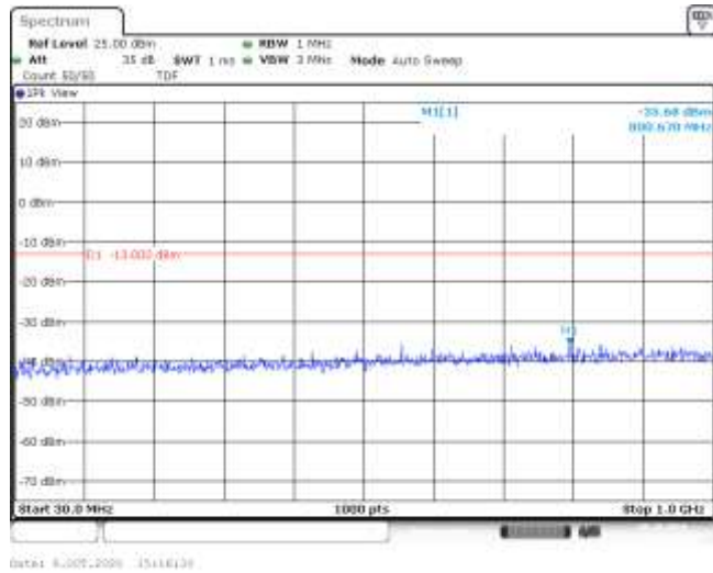
Band4-20MHz-16QAM-20300-100RB#0-Range1:30~1000MHz--35.68-PASS
