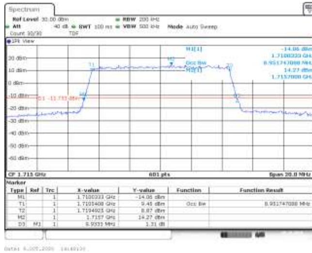
Band4-10MHz-16QAM-20000-50RB#0-8.952-9.933-PASS
