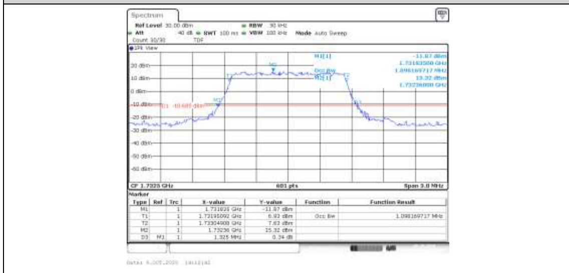
Band4-1.4MHz-QPSK-20175-6RB#0-1.098-1.325-PASS
