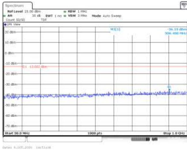
Band4-10MHz-16QAM-20350-50RB#0-Range1:30~1000MHz--36.19-PASS
