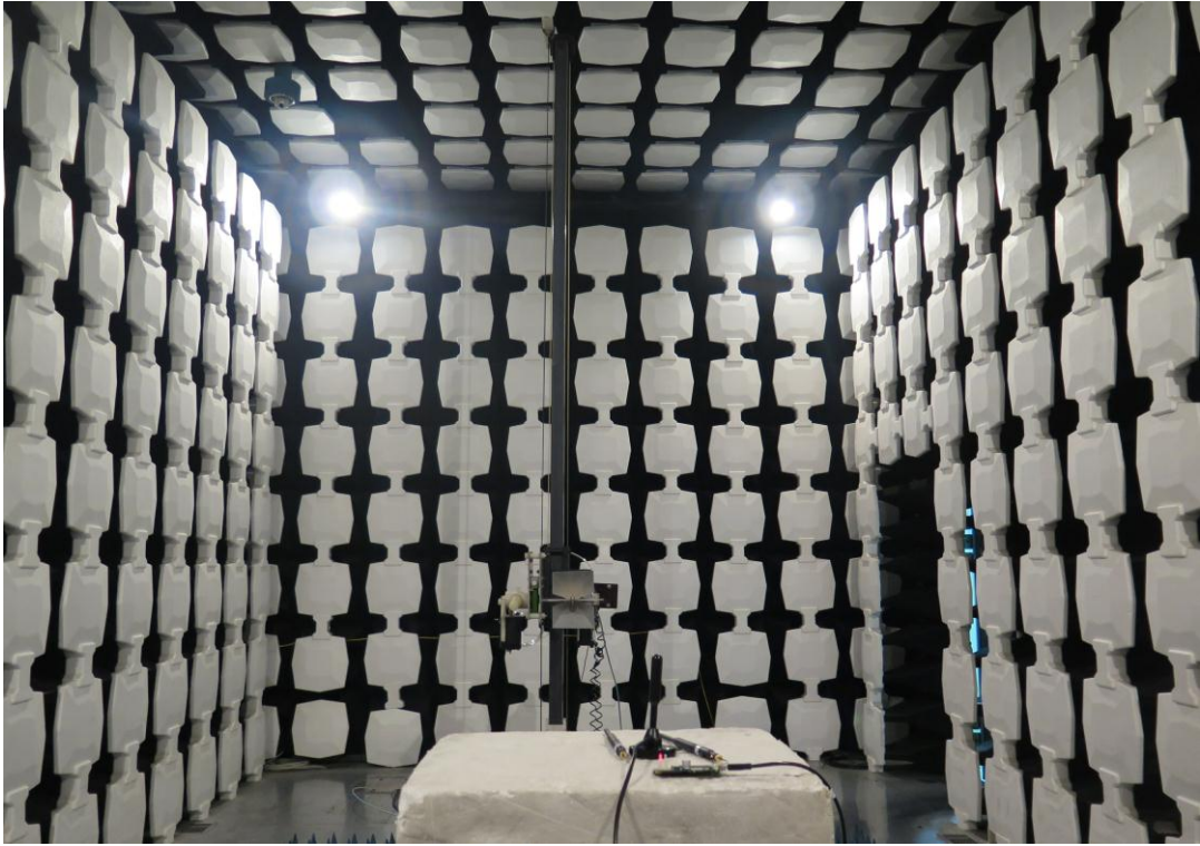
Pic3. ERP and EIRP Test Setup Photo 2
