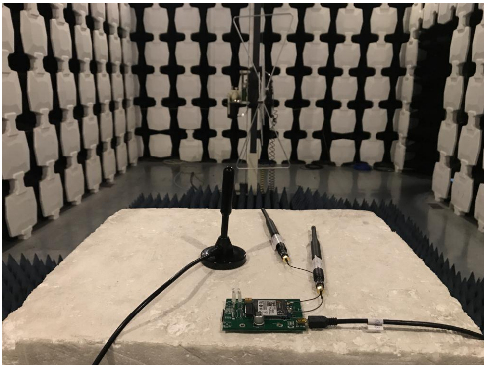
Pic2. ERP and EIRP Test Setup Photo 1
