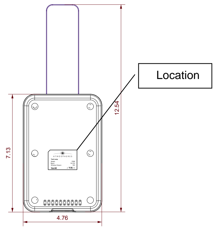
Bottom View
