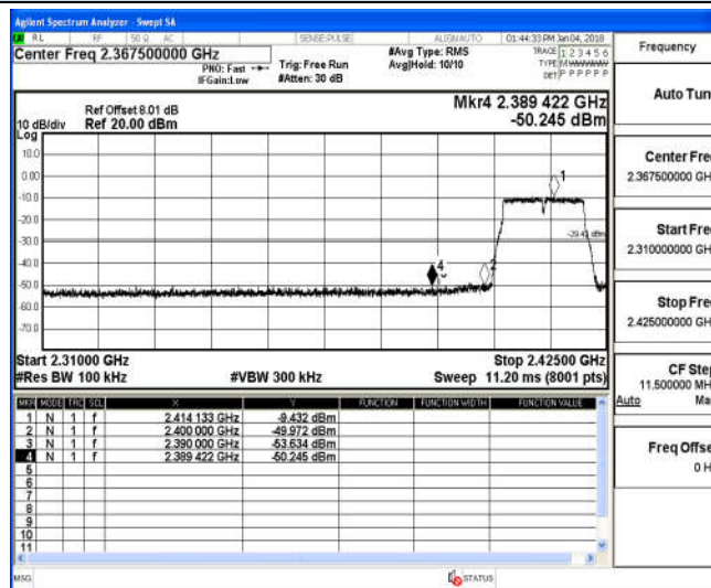
Channel 1 / 2412 MHz
