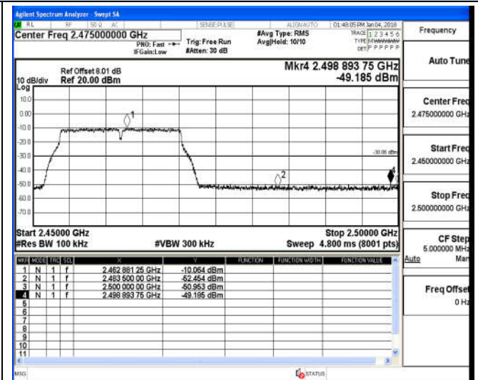
Channel 11 / 2462 MHz
