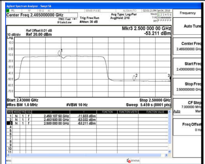
Channel 9 / 2452 MHz – Average
