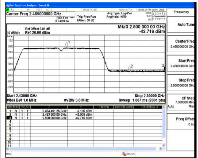
Channel 9 / 2452 MHz – Peak
