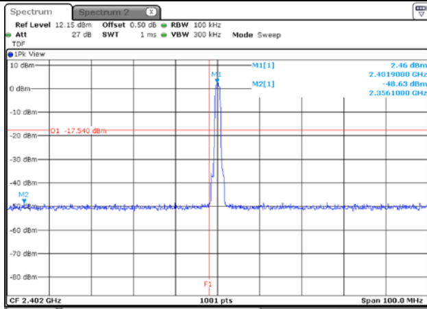
Conducted band-edge / Low ch.
