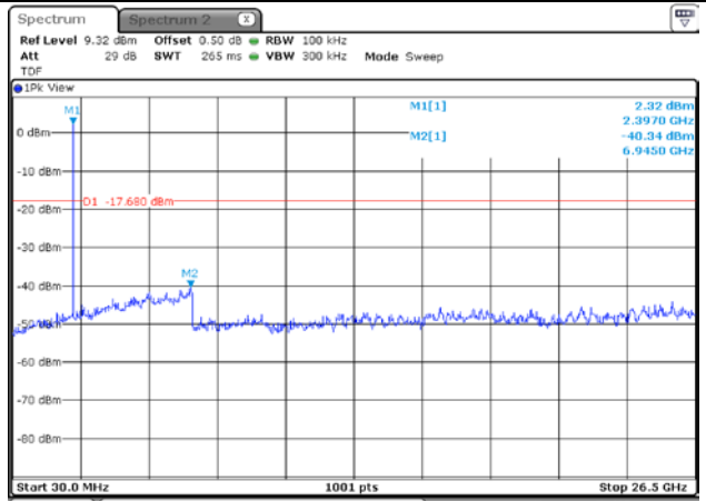
Conducted spurious / Low ch.
