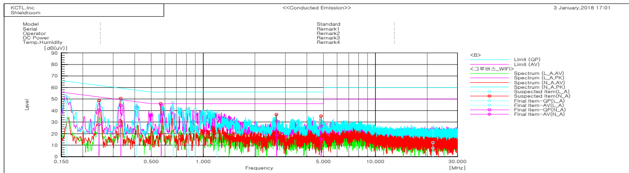
Figure 6. plot of Conducted Emission
