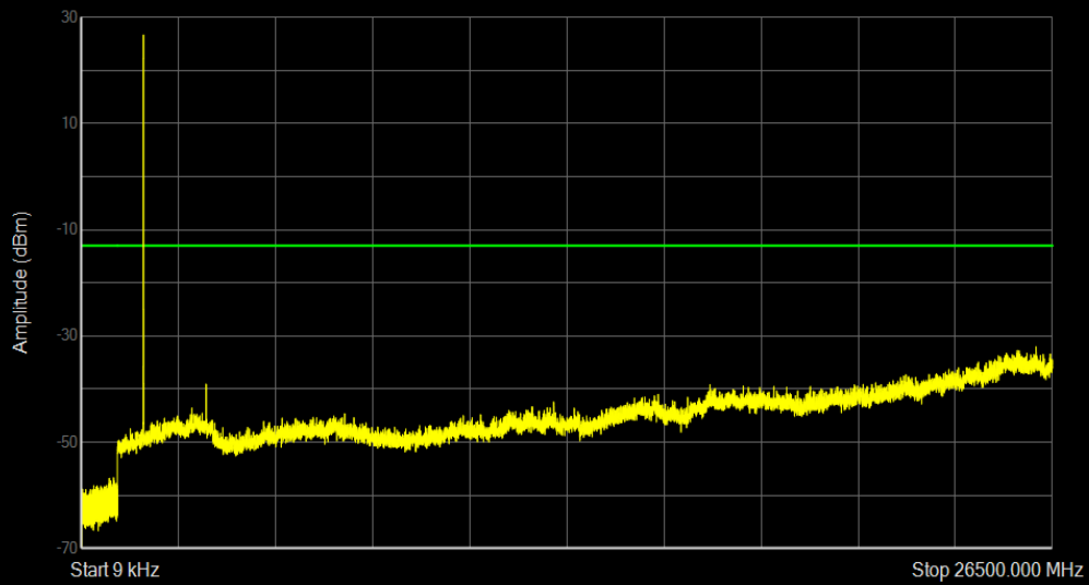
Band66 16QAM BW=1.4MHz Channel=131979 RB Size=1 Position=#0
