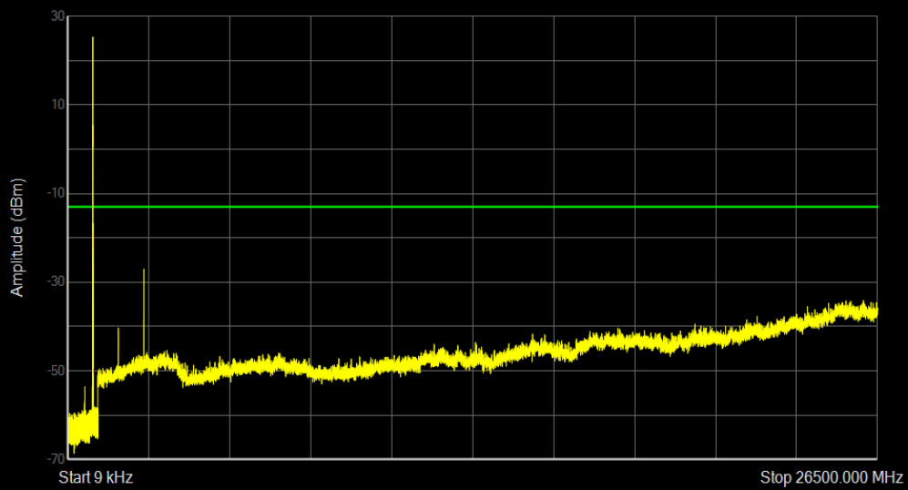
Band5 16QAM BW=5MHz Channel=20525 RB Size=1 Position=#0
