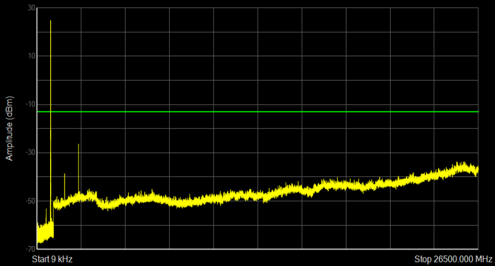
Band26(824-849) QPSK BW=1.4MHz Channel=26915 RB Size=1 Position=#0
