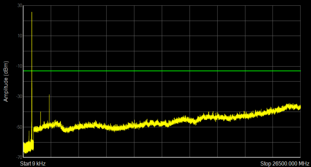
Band26(824-849) 16QAM BW=3MHz Channel=26915 RB Size=1 Position=#0
