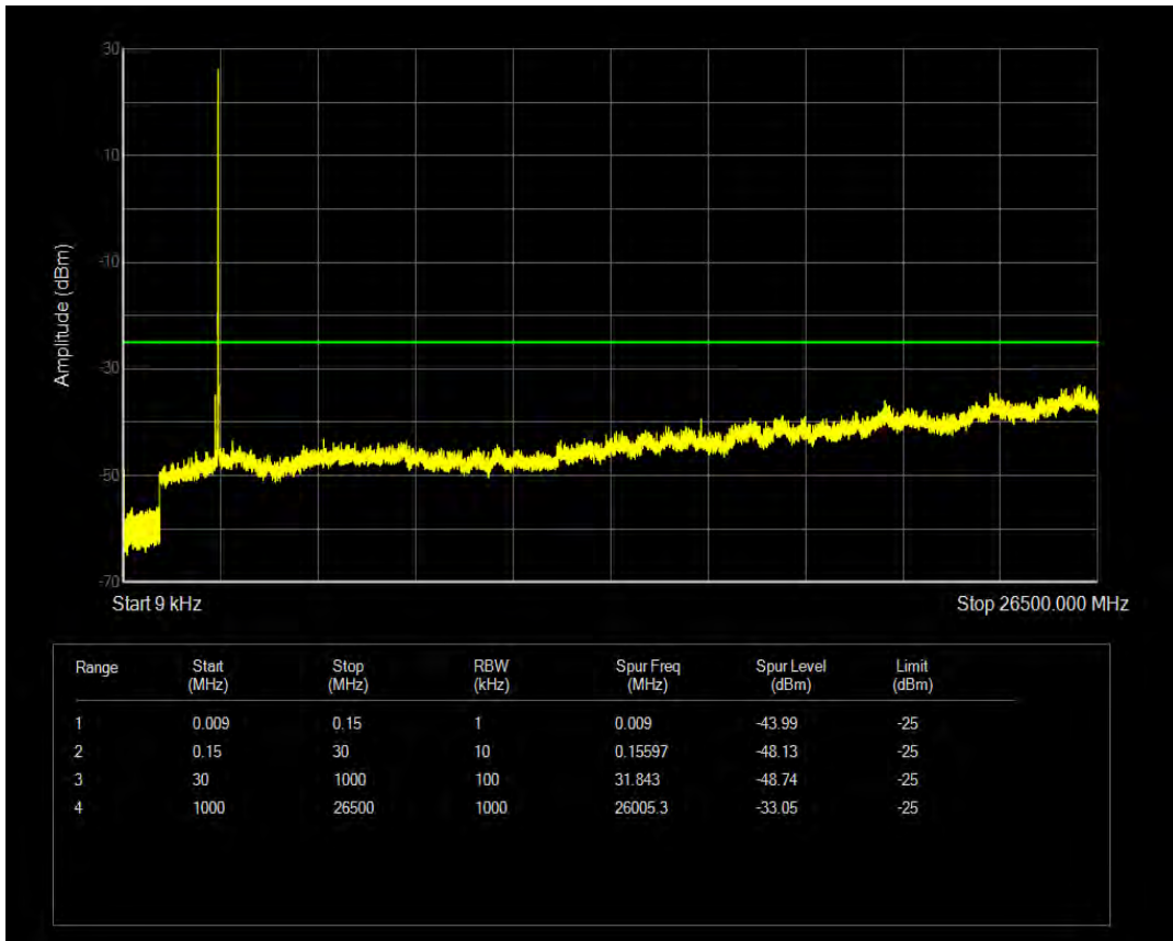
Band41 QPSK BW=10MHz Channel=40665 RB Size=50 Position=#0
