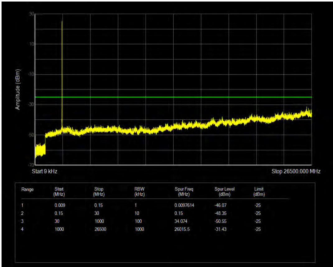
Band41 16QAM BW=5MHz Channel=40665 RB Size=25 Position=#0
