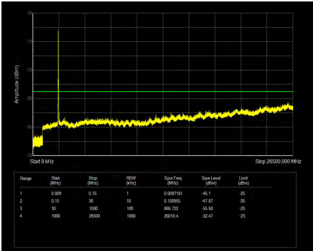
Band41 16QAM BW=15MHz Channel=40665 RB Size=75 Position=#0
