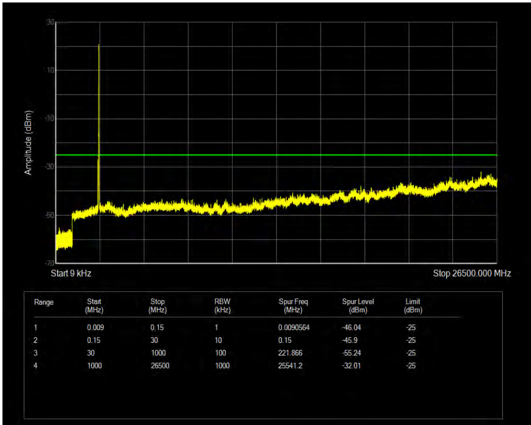
Band41 16QAM BW=10MHz Channel=40665 RB Size=50 Position=#0
