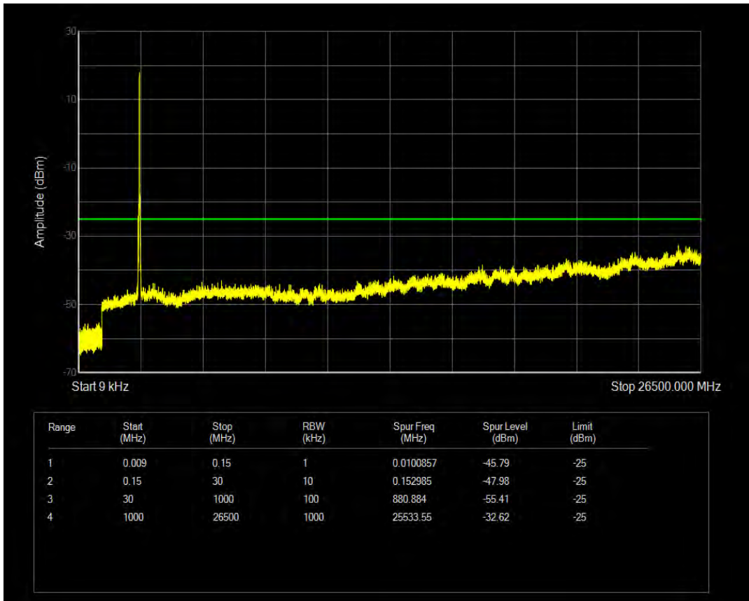
Band41 QPSK BW=20MHz Channel=40665 RB Size=100 Position=#0
