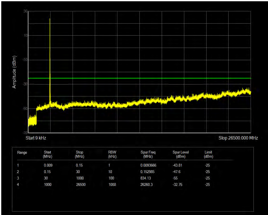
Band41 16QAM BW=20MHz Channel=40665 RB Size=100 Position=#0
