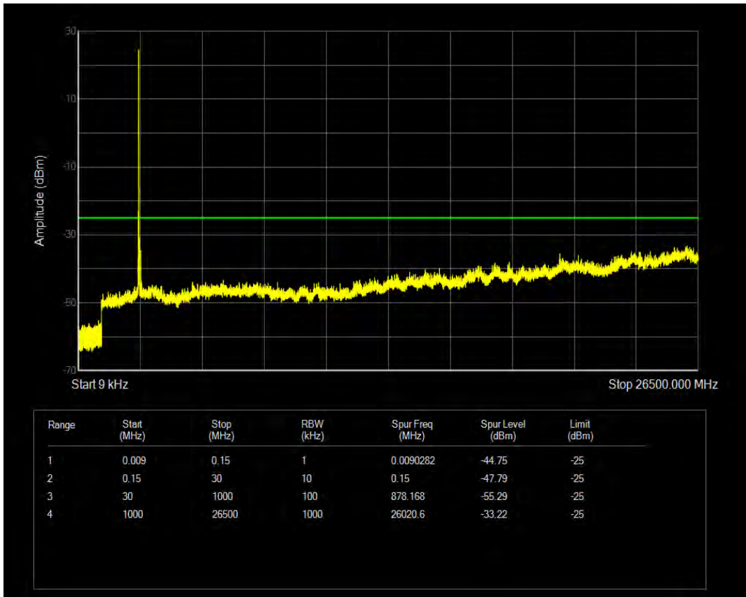
Band41 QPSK BW=15MHz Channel=40665 RB Size=75 Position=#0
