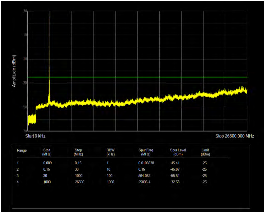
Band41 QPSK BW=20MHz Channel=40665 RB Size=100 Position=#0
