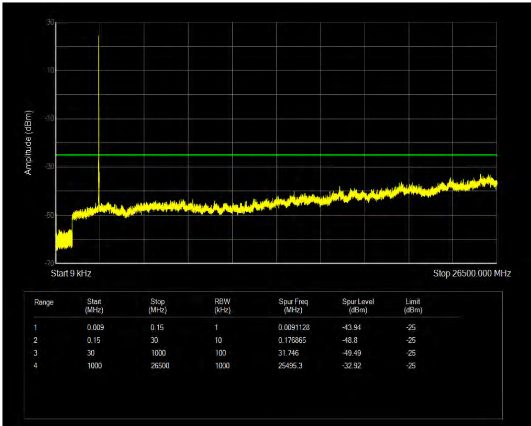
Band41 16QAM BW=10MHz Channel=40665 RB Size=50 Position=#0
