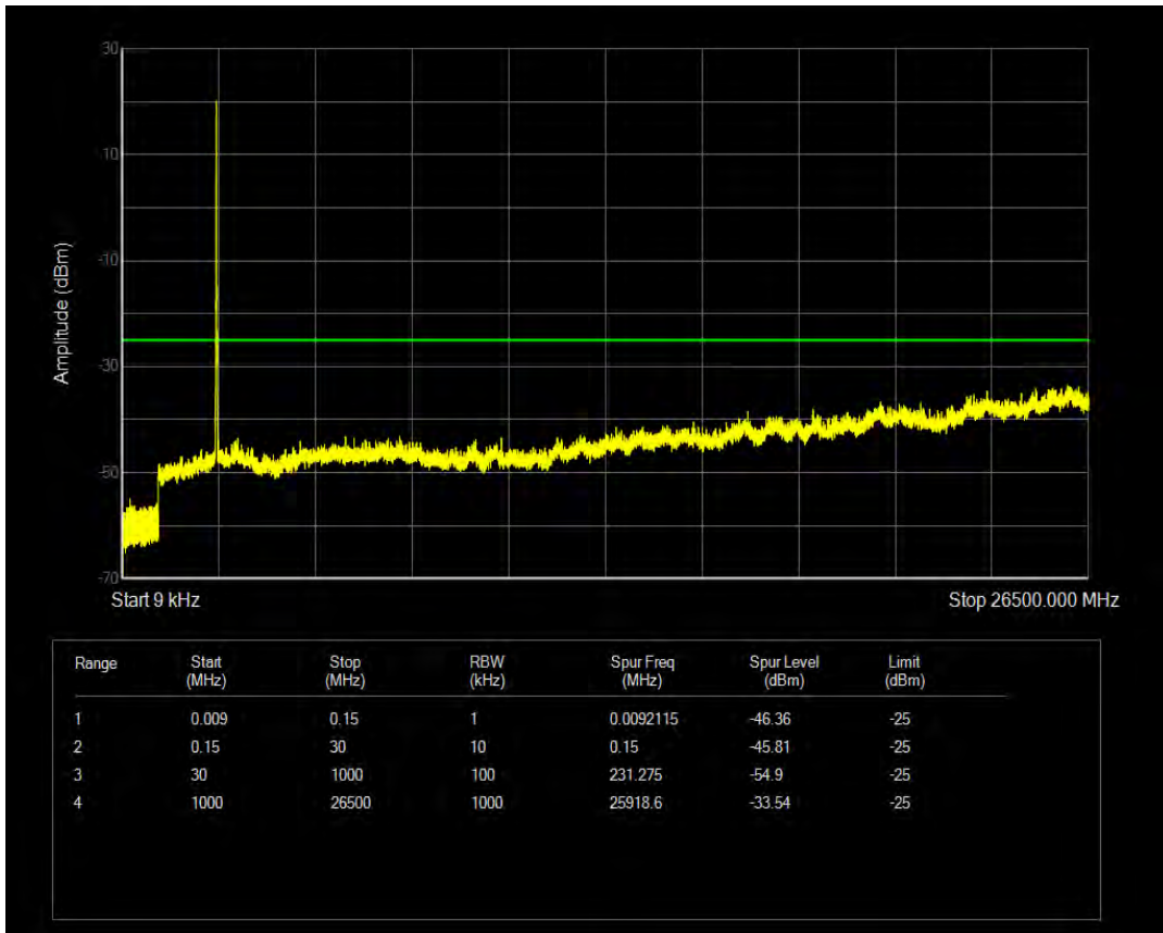
Band41 QPSK BW=10MHz Channel=40665 RB Size=50 Position=#0
