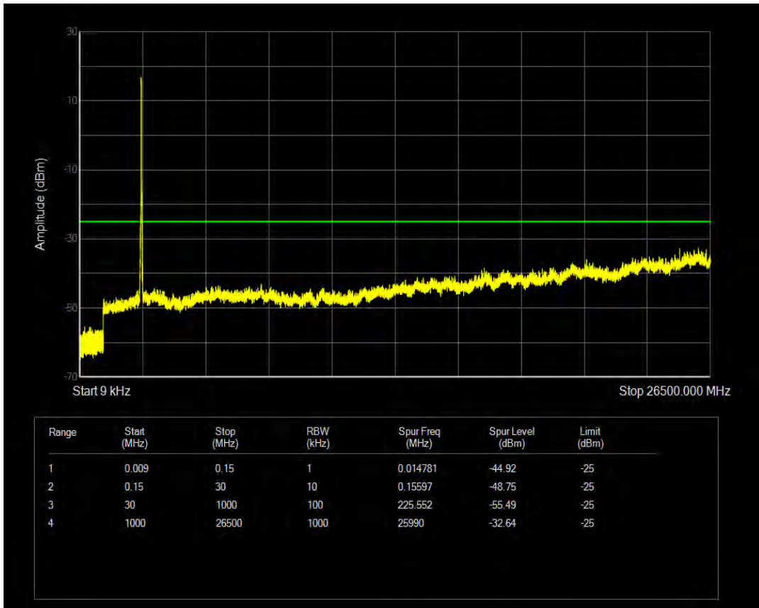
Band41 16QAM BW=20MHz Channel=40665 RB Size=100 Position=#0
