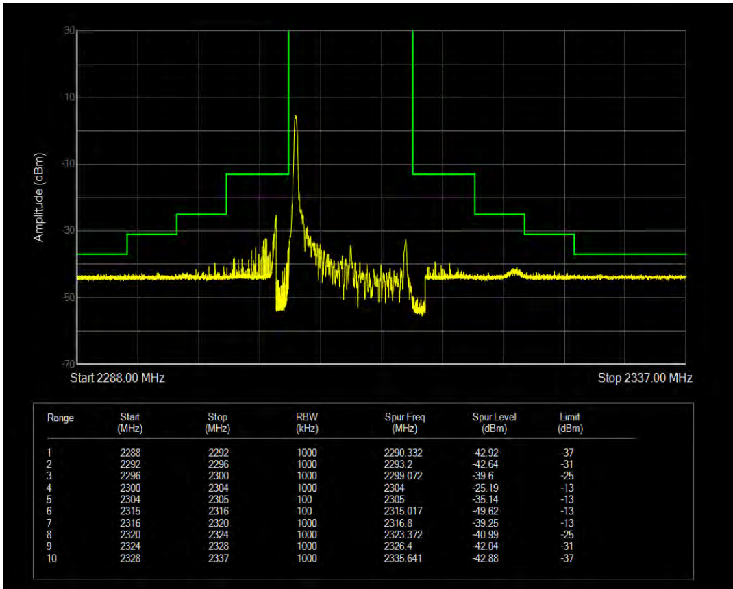
Band40a 16QAM BW=10MHz Channel=38750 RB Size=1 Position=#Max
