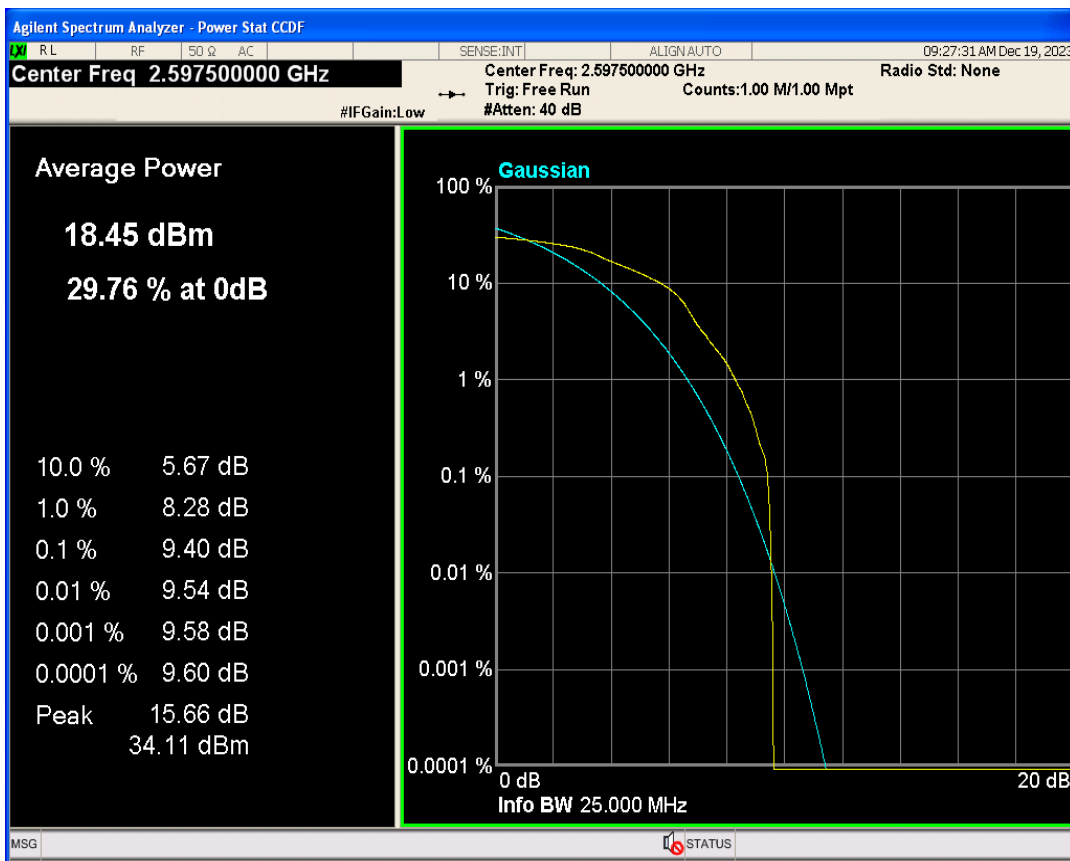
Band41 16QAM BW=10MHz Channel=40665 RB Size=1 Position=#0
