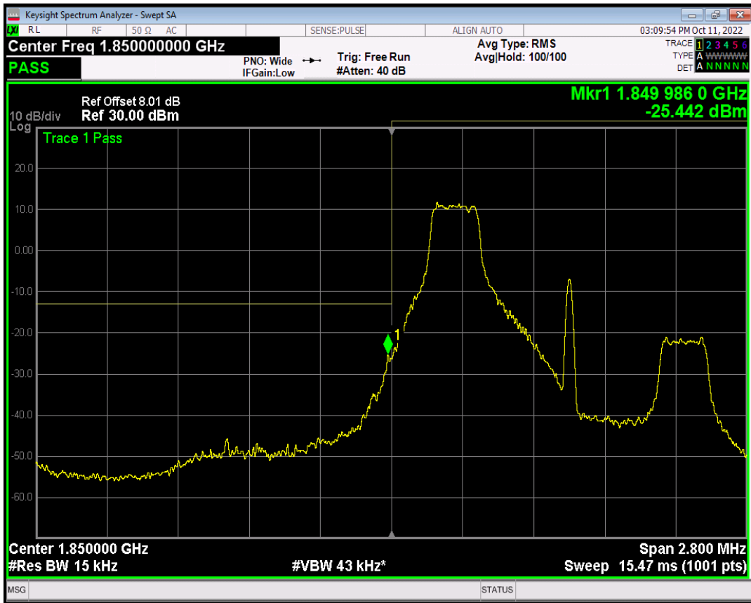
Band25 QAM16 BW=1.4MHz Channel=26047 RB Size=1 Position=#Max
