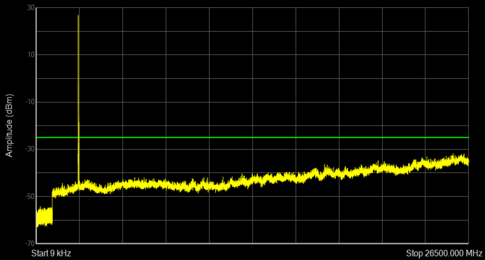
Band41 QPSK BW=10MHz Channel=40640 RB Size=1 Position=#0
