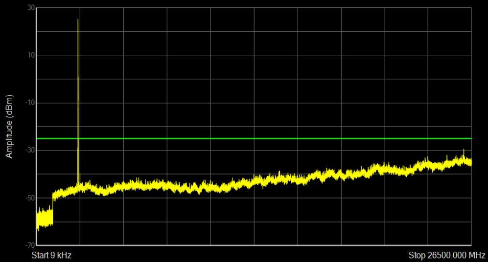
Band41 QPSK BW=15MHz Channel=40165 RB Size=1 Position=#0
