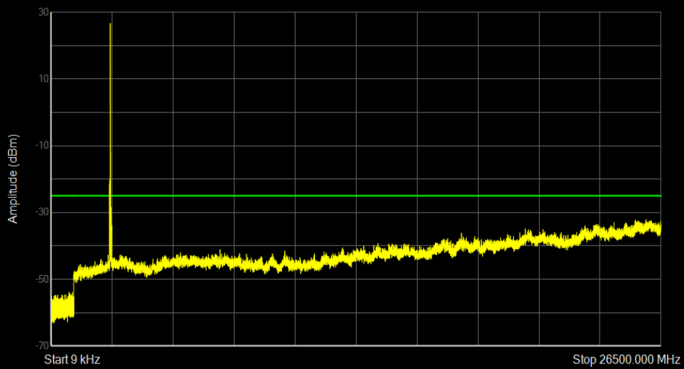
Band41 QPSK BW=15MHz Channel=40640 RB Size=1 Position=#0
