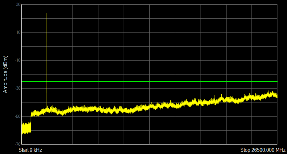
Band41 16QAM BW=5MHz Channel=41165 RB Size=1 Position=#0
