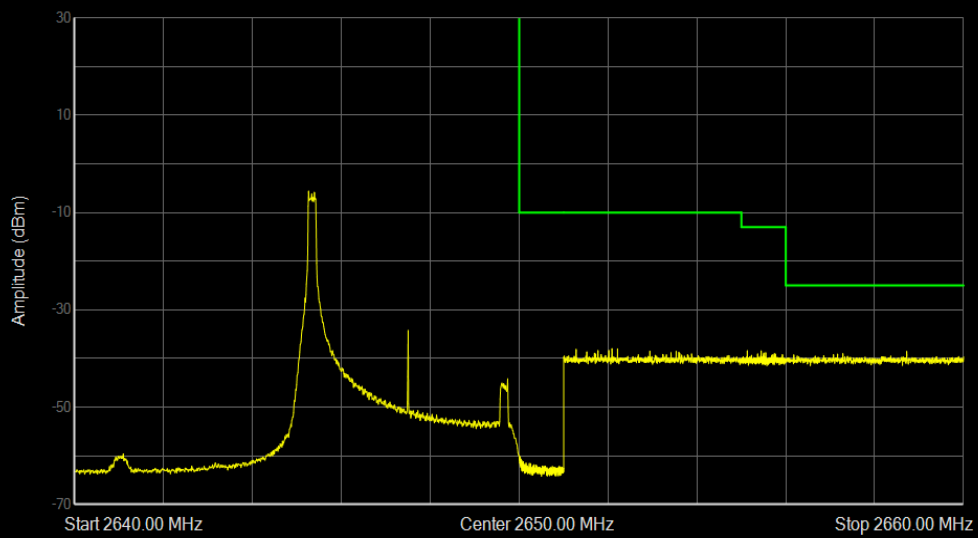
Band41 16QAM BW=5MHz Channel=41165 RB Size=1 Position=#0
