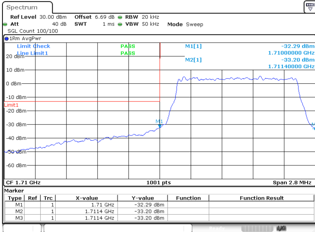
Band66 QPSK BW=1.4MHz Channel=131979 RB Size=6 Position=#0
