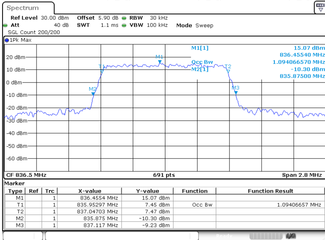
Band5 QPSK BW=1.4MHz Channel=20525 RB Size=6 Position=#0
