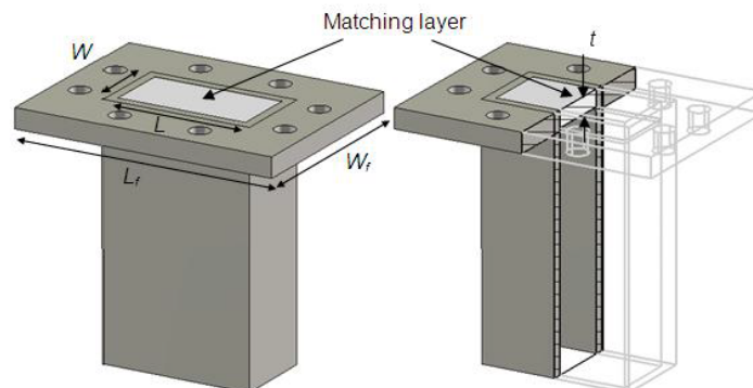
Figure 1: Validation Waveguide Dimensions
