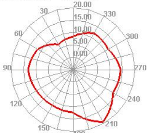
Wifi 6 TRP Phi=45
