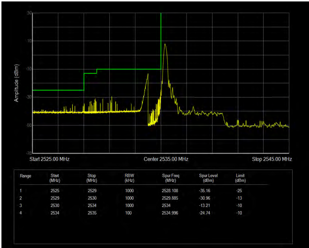
Band41(2535-2655) QAM16 BW=5MHz Channel=40065 RB Size=1 Position=#Max
