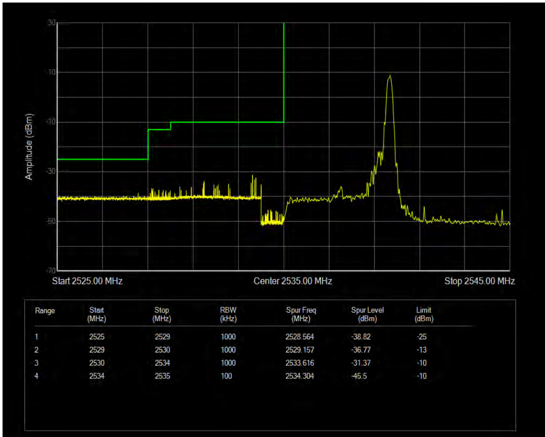
Band41(2535-2655) QAM16 BW=5MHz Channel=40065 RB Size=1 Position=#Max
