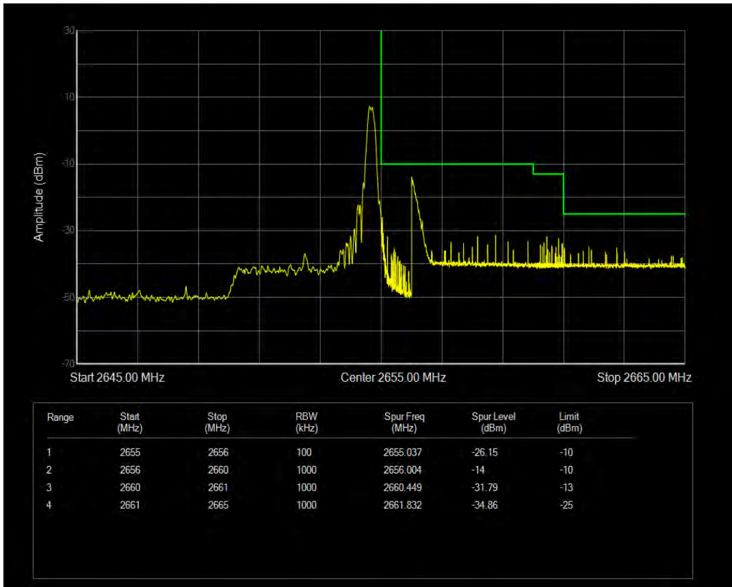
Band41(2535-2655) QAM16 BW=5MHz Channel=41215 RB Size=1 Position=#Max
