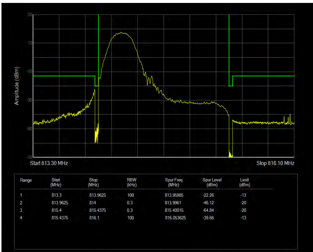
Band26(814-824) QAM16 BW=1.4MHz Channel=26697 RB Size=1 Position=#Max
