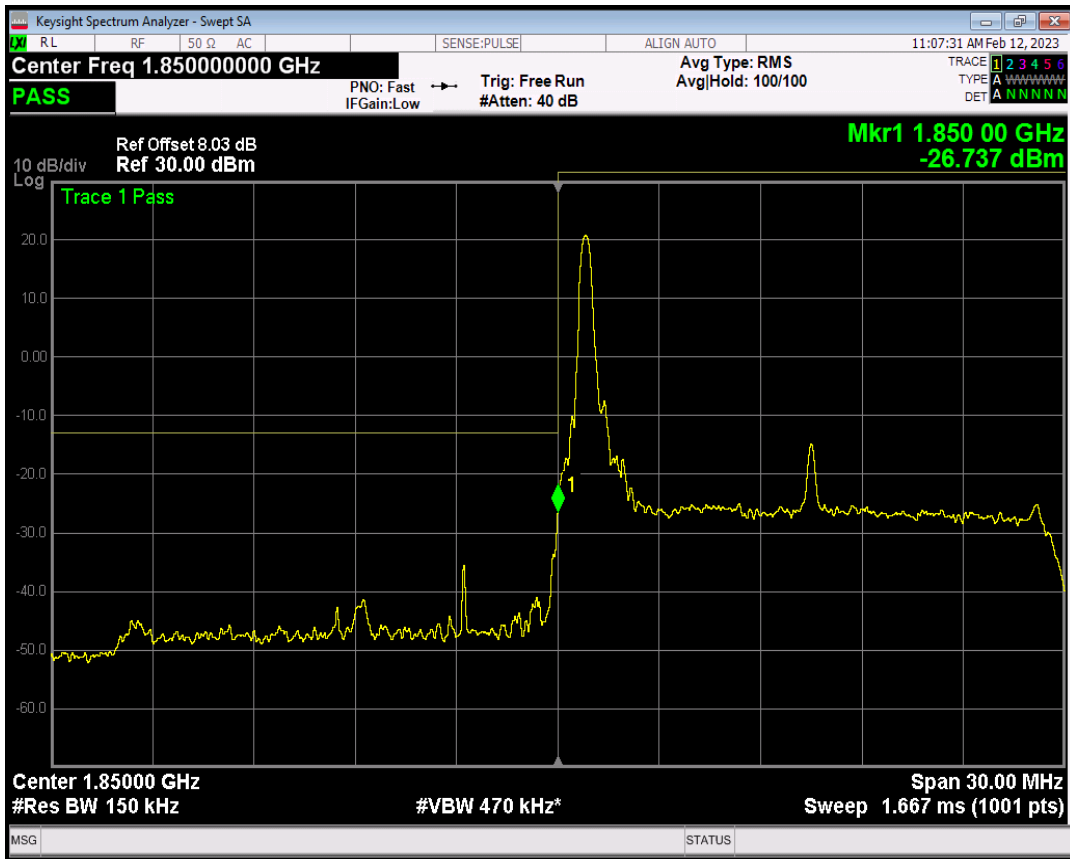
Band25 QAM16 BW=15MHz Channel=26115 RB Size=1 Position=#Max
