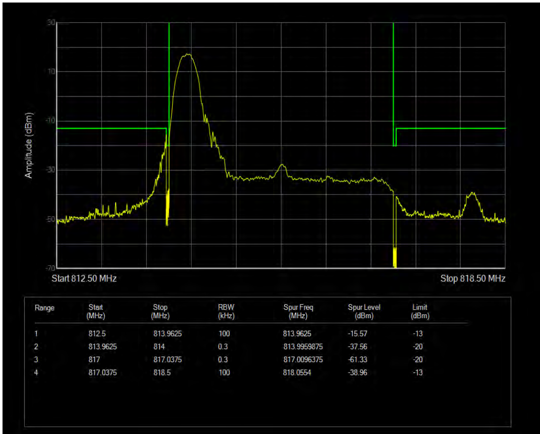
Band26(814-824) QAM16 BW=3MHz Channel=26705 RB Size=1 Position=#Max
