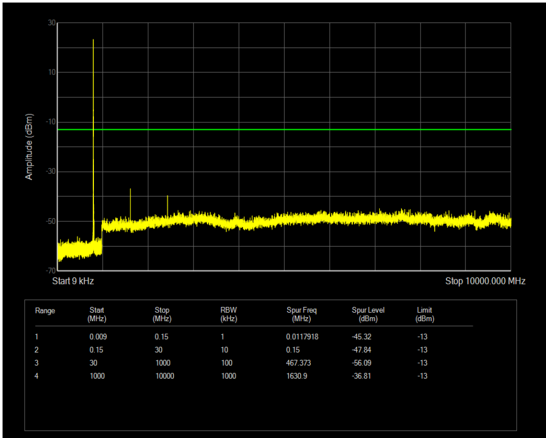
Band18 QAM16 BW=5MHz Channel=23875 RB Size=25 Position=#0
