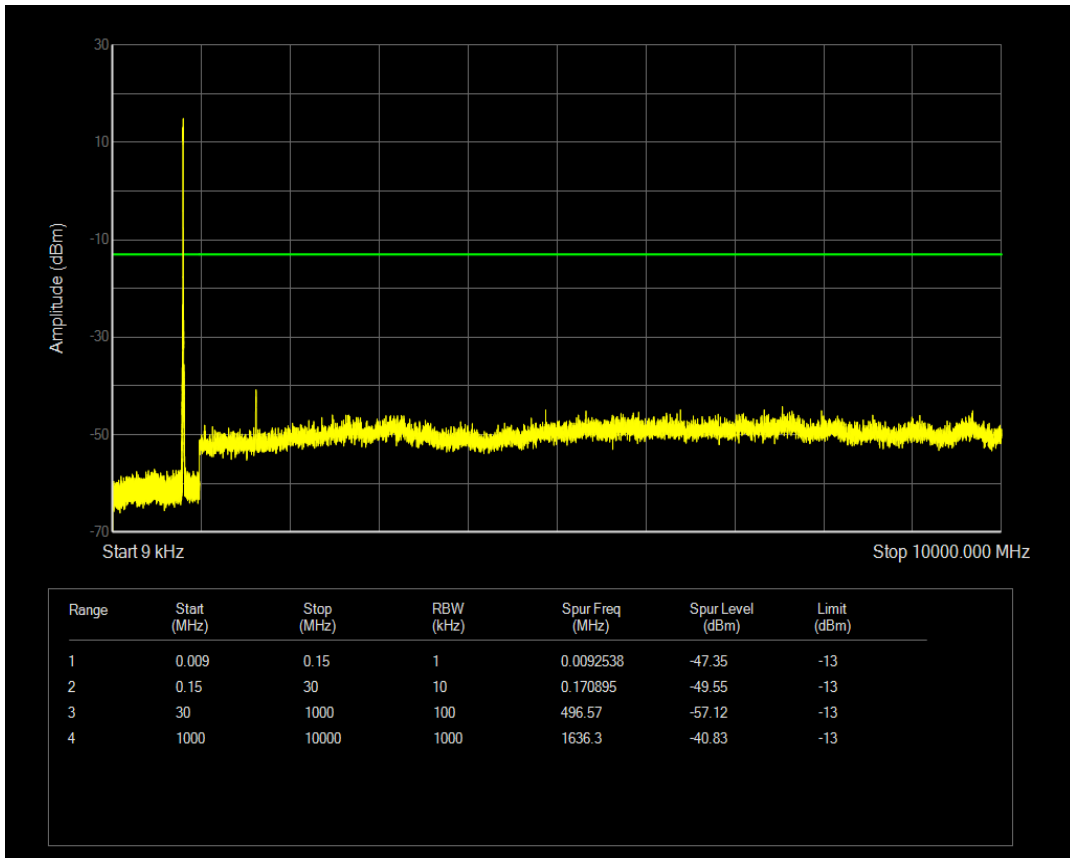
Band18 QAM16 BW=5MHz Channel=23875 RB Size=25 Position=#0
