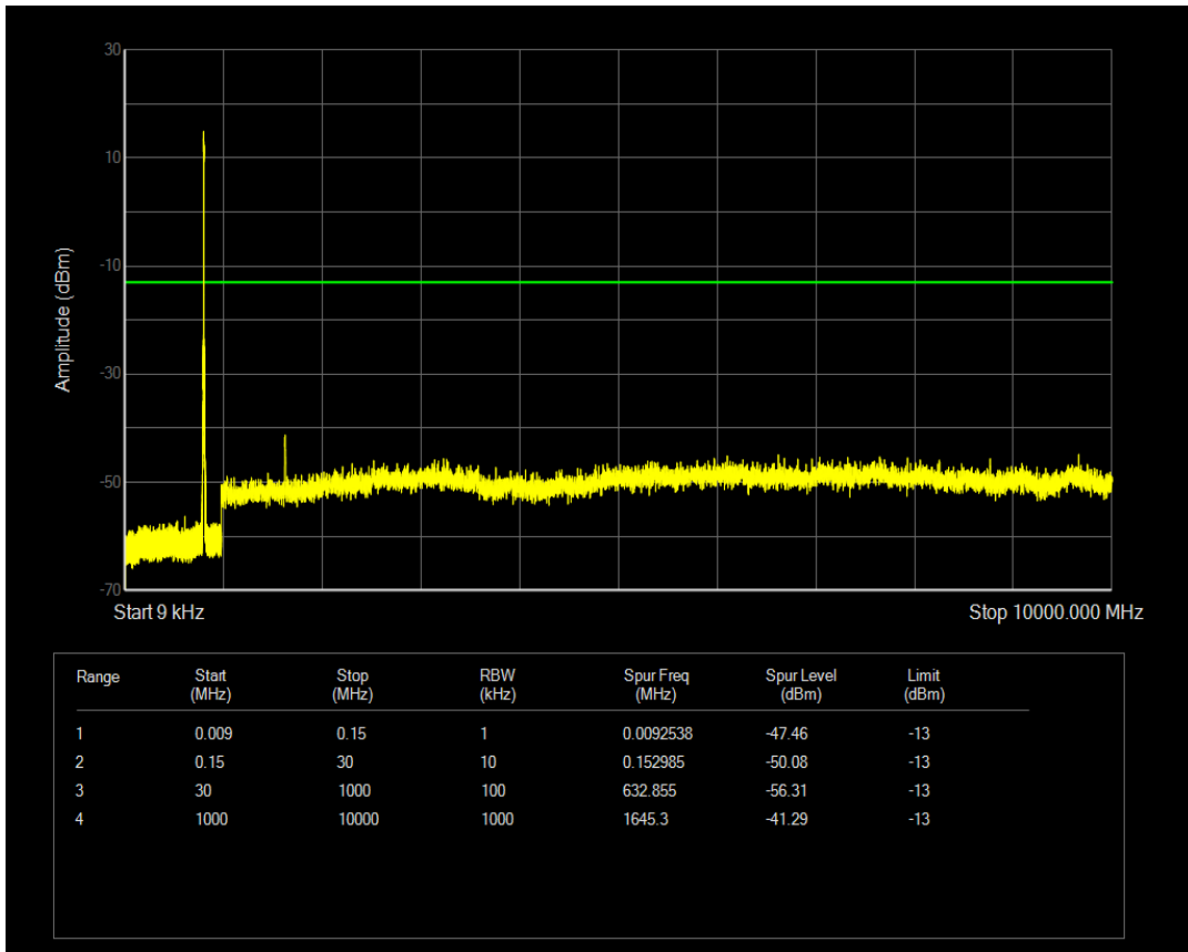
Band18 QAM16 BW=5MHz Channel=23925 RB Size=25 Position=#0
