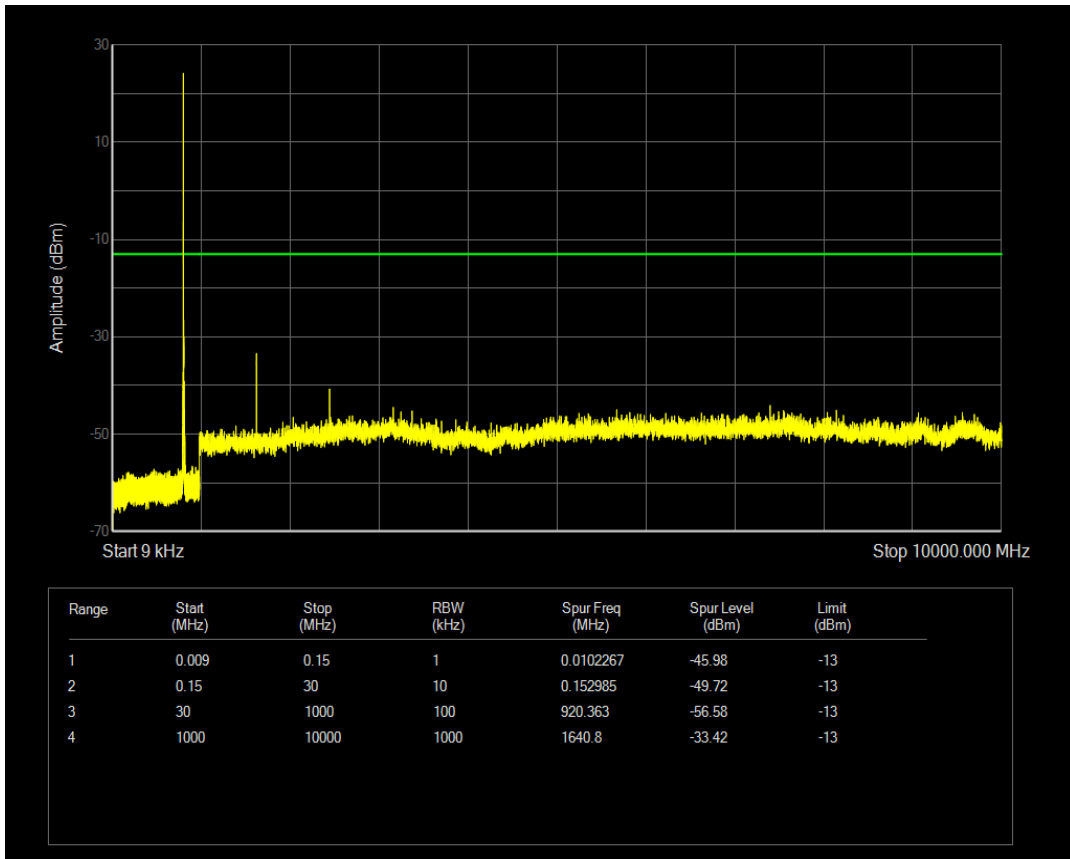
Band18 QAM16 BW=5MHz Channel=23925 RB Size=25 Position=#0
