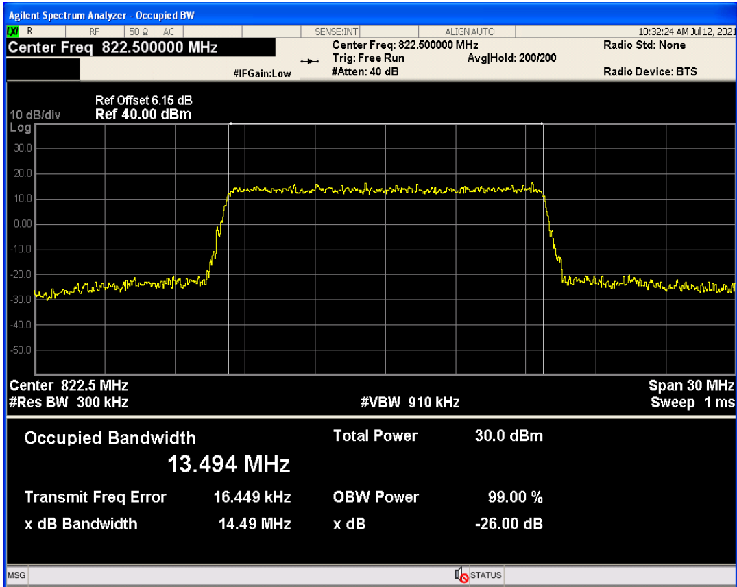
Band18 QPSK BW=15MHz Channel=23925 RB Size=75 Position=#0
