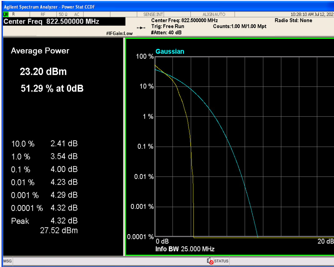
Band18 QAM16 BW=15MHz Channel=23925 RB Size=1 Position=#0
