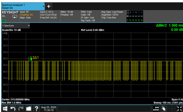
T on time slot-2:
