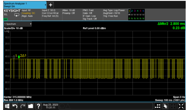
T 100ms & T on time slot-1:
