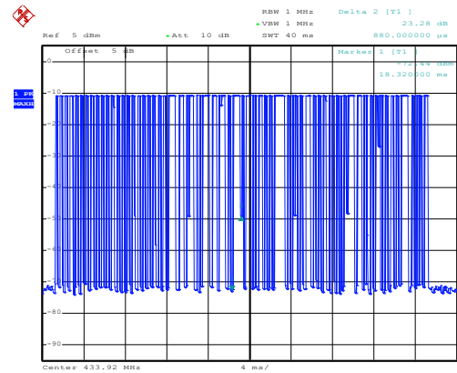
T 8=40ms:
