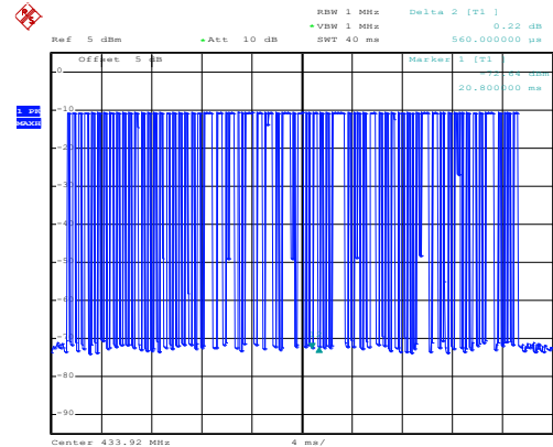
T 10=40ms:
