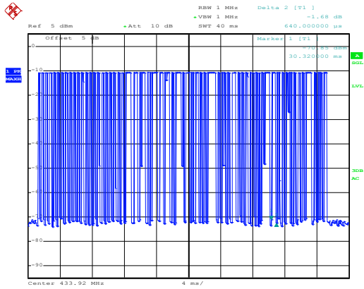
T 13=40ms:
