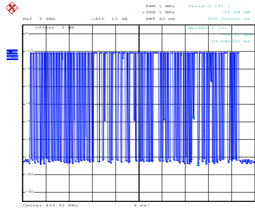
T 12=40ms:
