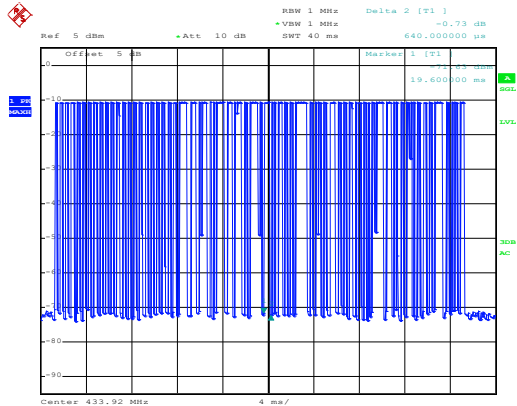
T 9=40ms:
