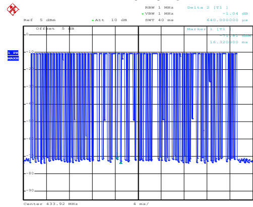
T 6=40ms:
