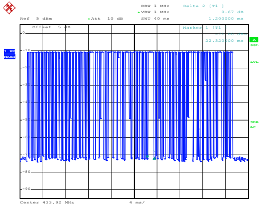
T 11=40ms:
