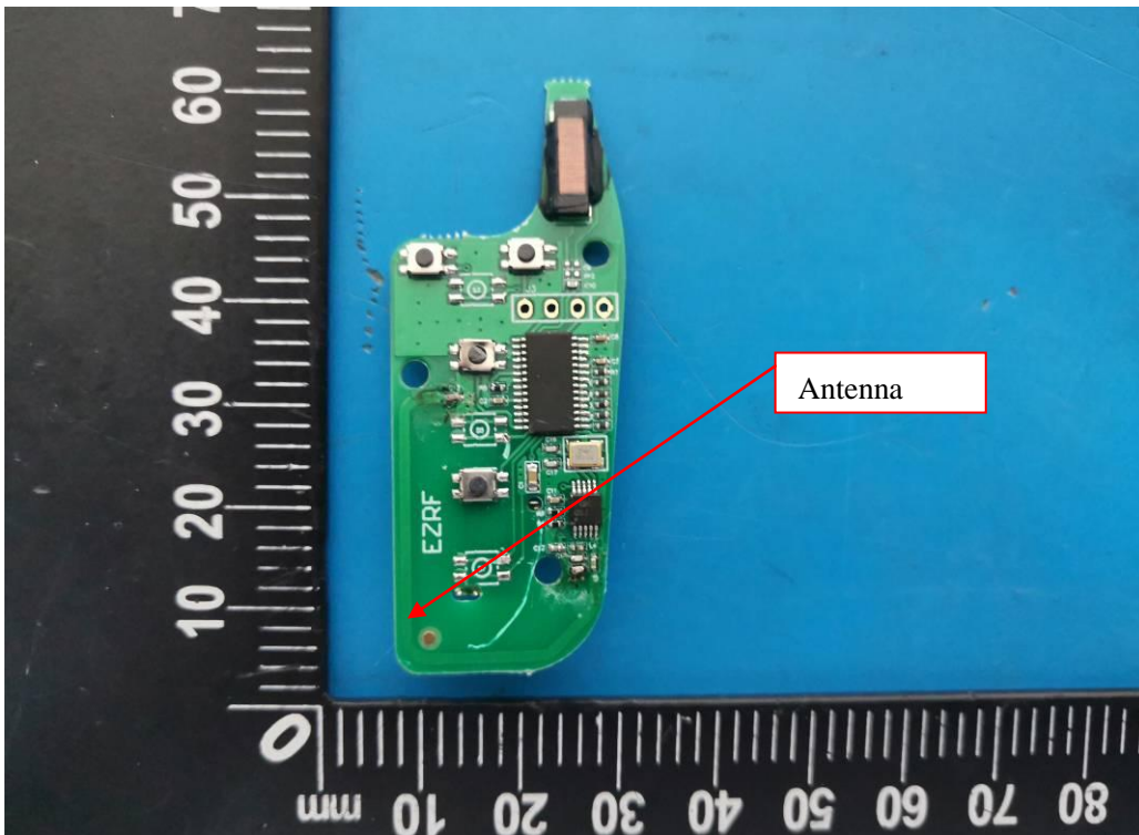
Model: RT-FD7986
