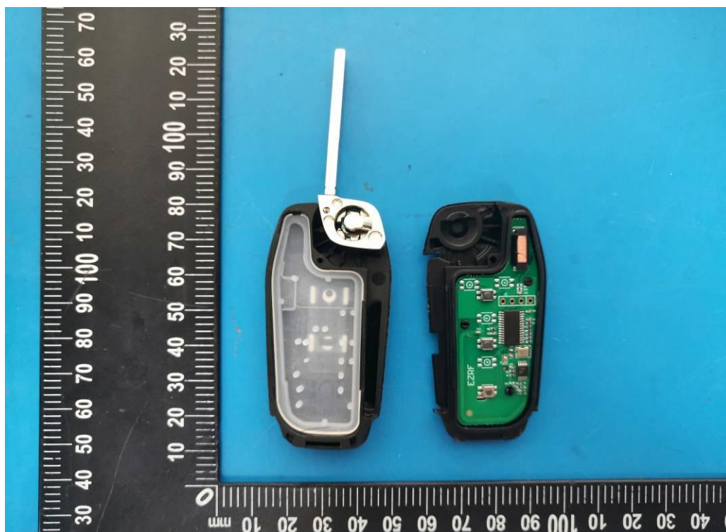
Model: RT-FD8130
