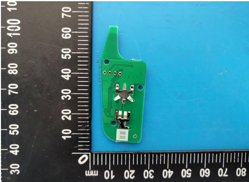
Model: RT-FD7986
