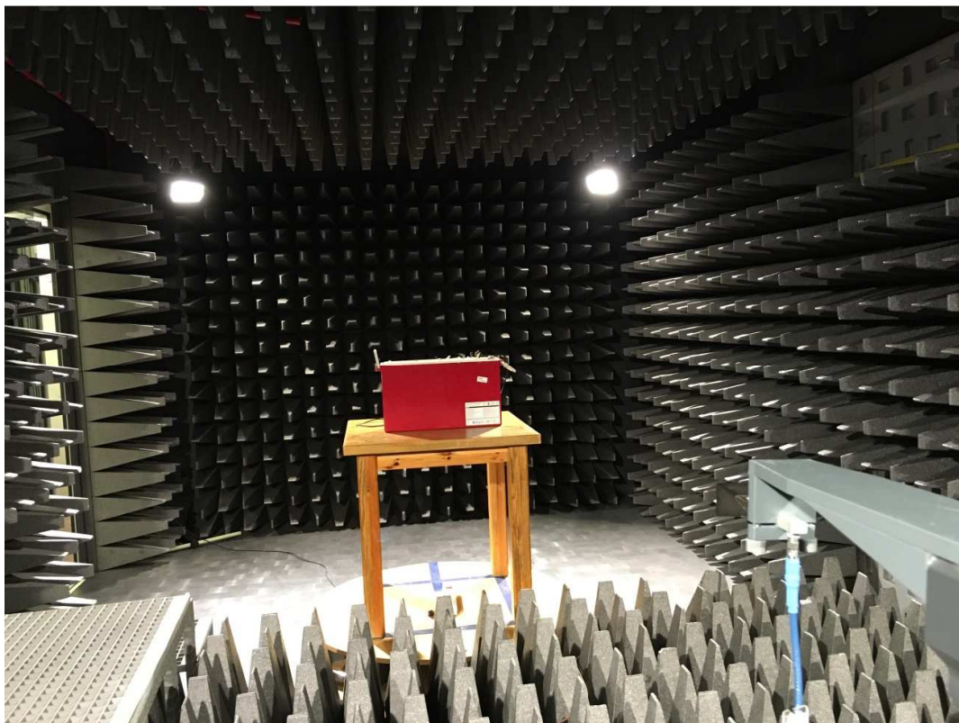
Test set up radiated emission 18 GHz – 26.5 GHz
