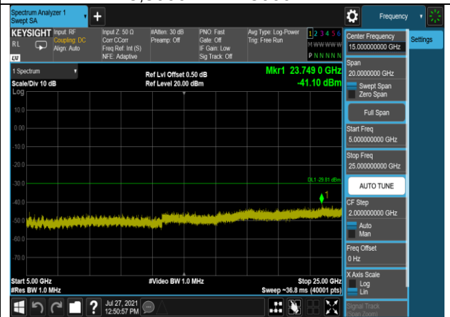
802.11n(HT40),2452MHz,Ant1,Plot 5,5000MHz~25000MHz
