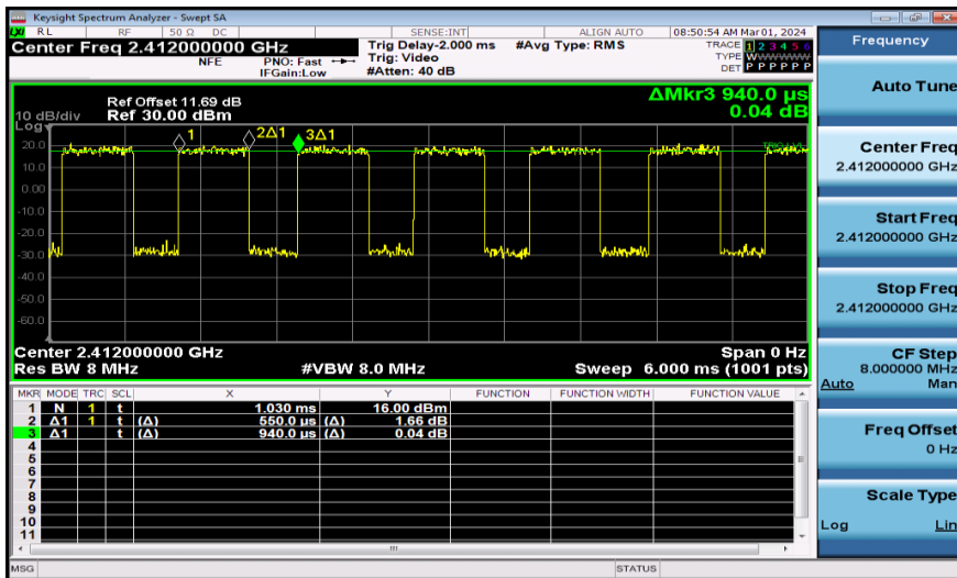
NTNV-11AX20MIMO-Ant2-2412
