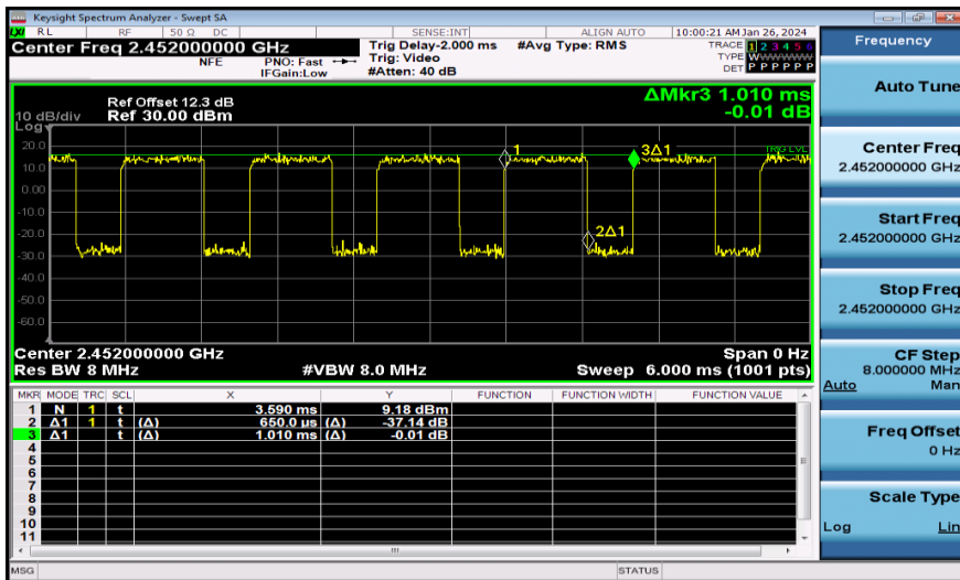
NTNV-11N40MIMO-Ant1-2452
