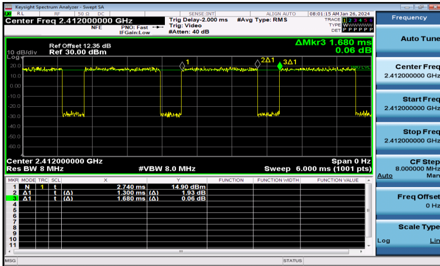
NTVN-11N20MIMO-Ant1-2412
