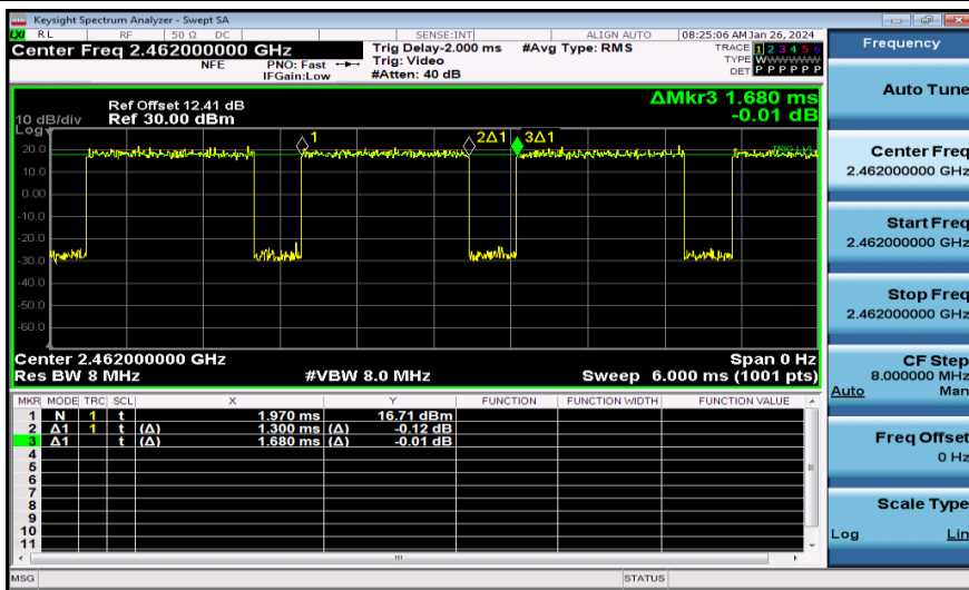
NTNV-11N20MIMO-Ant2-2462
