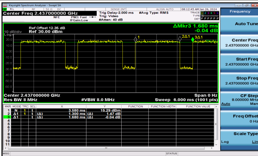
NTVN-11N20MIMO-Ant1-2437
