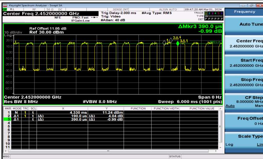
NTNV-11AX40MIMO-Ant2-2452
