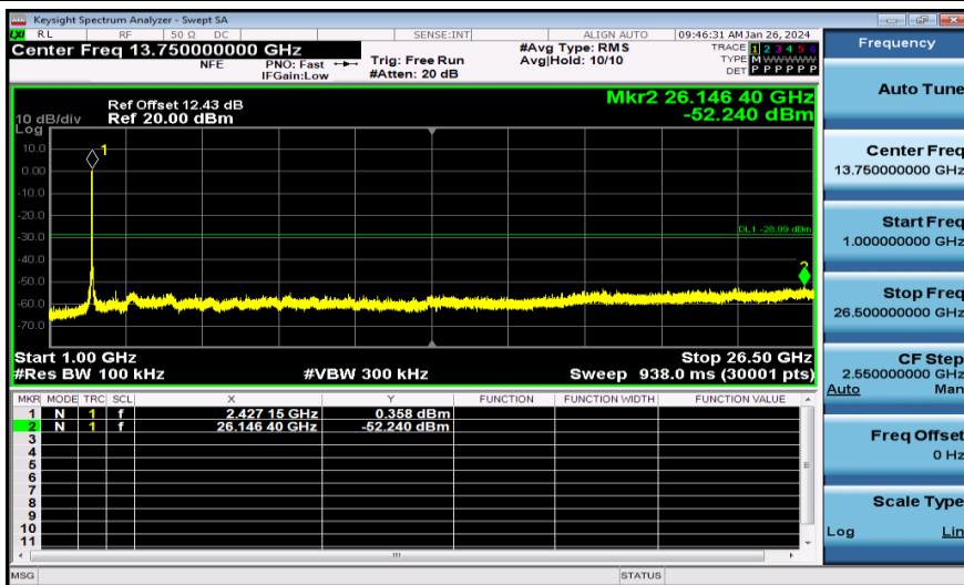
11N40MIMO-Ant2-2422-1000~26500-PASS
