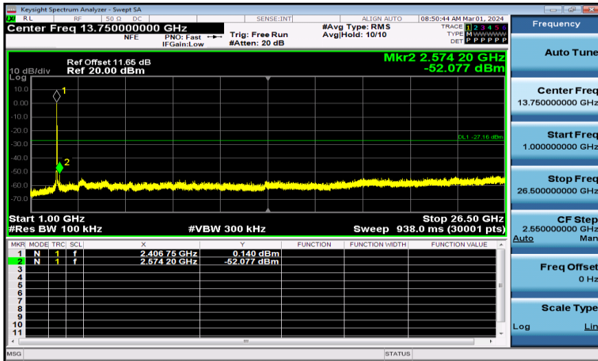
11AX20MIMO-Ant1-2412-1000~26500-PASS
