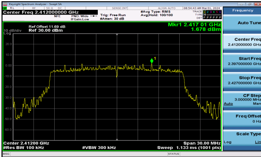
11AX20MIMO-Ant2-2412-0~Reference-PASS
