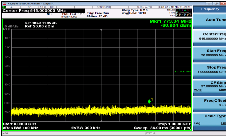
11AX20MIMO-Ant2-2462-30~1000-PASS
