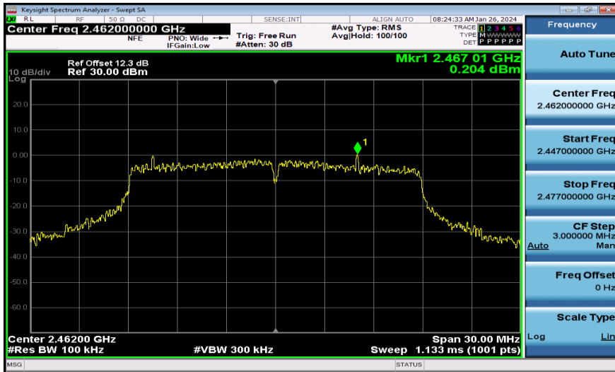
11N20MIMO-Ant1-2462-0-Reference-PASS
