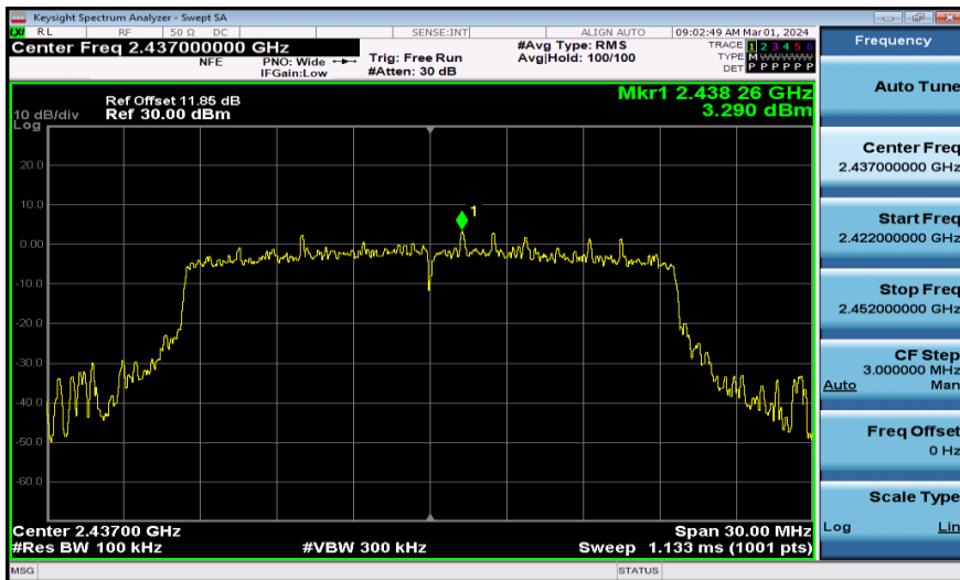
11AX20MIMO-Ant2-2437-0~Reference-PASS
