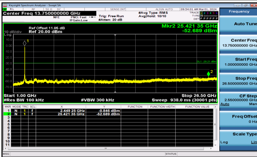
11AX40MIMO-Ant2-2452-1000~26500-PASS
