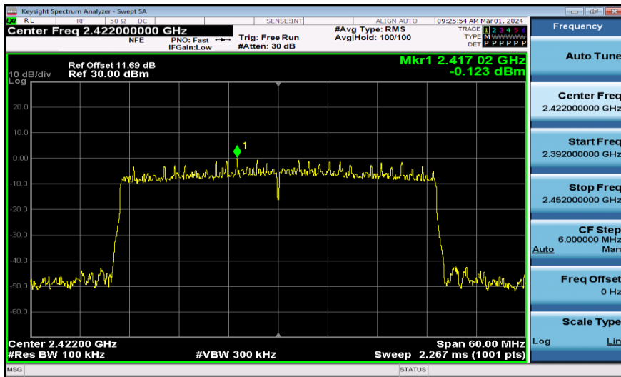
11AX40MIMO-Ant2-2422-0~Reference-PASS
