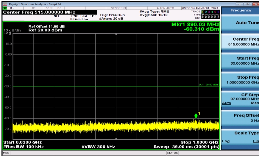
11AX40MIMO-Ant2-2437-30~1000-PASS
