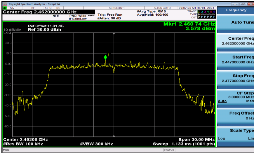
11AX20MIMO-Ant1-2462-0~Reference-PASS
