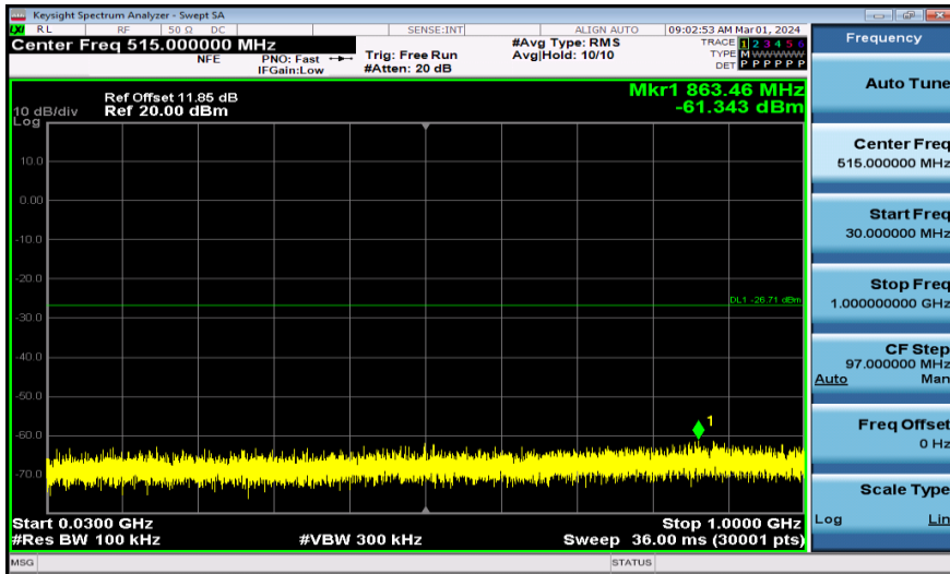
11AX20MIMO-Ant2-2437-30~1000-PASS
