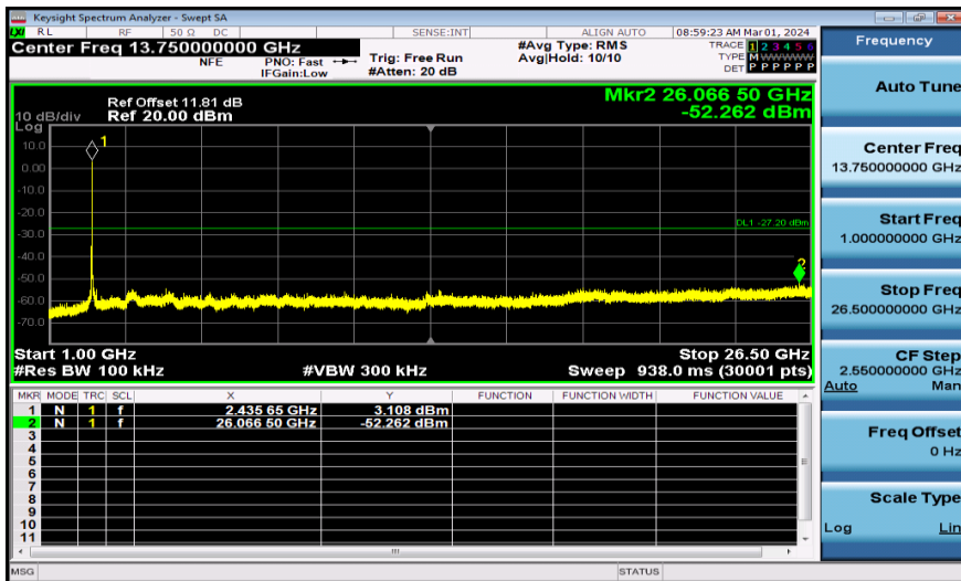
11AX20MIMO-Ant1-2437-1000~26500-PASS
