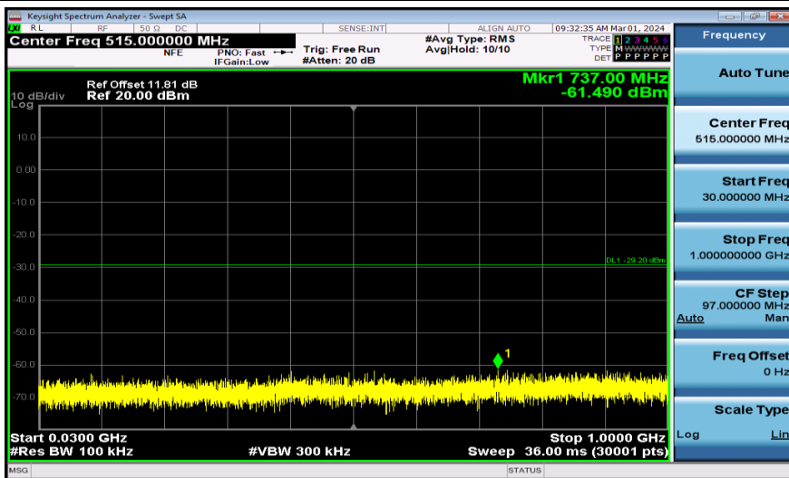
11AX40MIMO-Ant1-2437-30~1000-PASS
