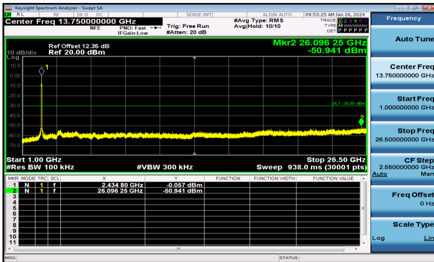
11N40MIMO-Ant1-2437-1000~26500-PASS
