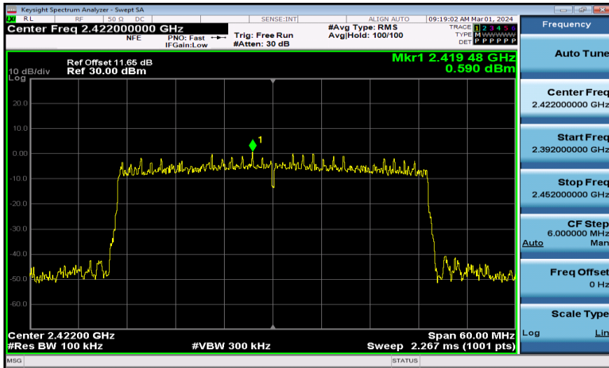
11AX40MIMO-Ant1-2422-0~Reference-PASS
