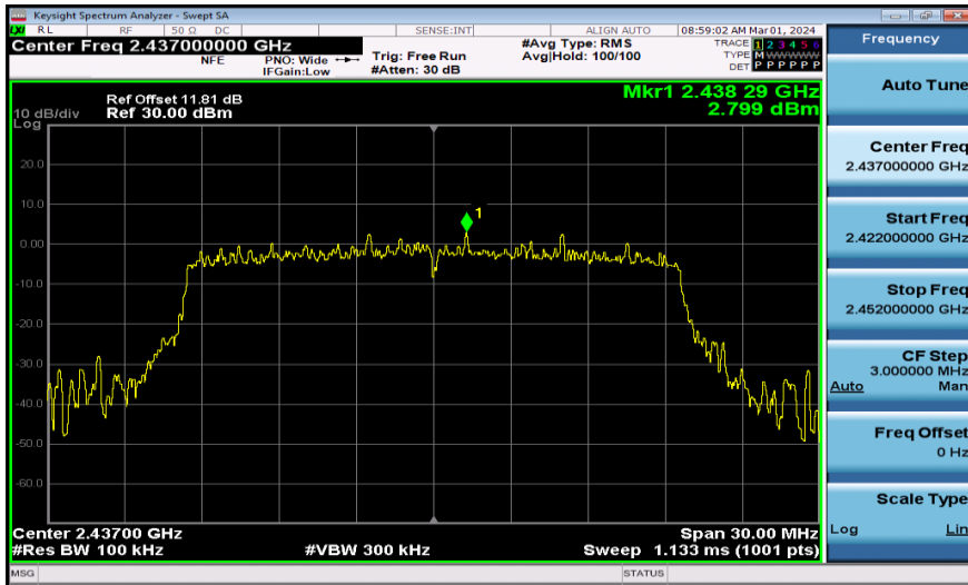
11AX20MIMO-Ant1-2437-0~Reference-PASS
