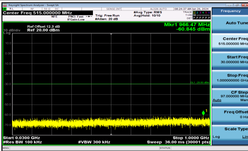
11N20MIMO-Ant1-2462-30~1000-PASS
