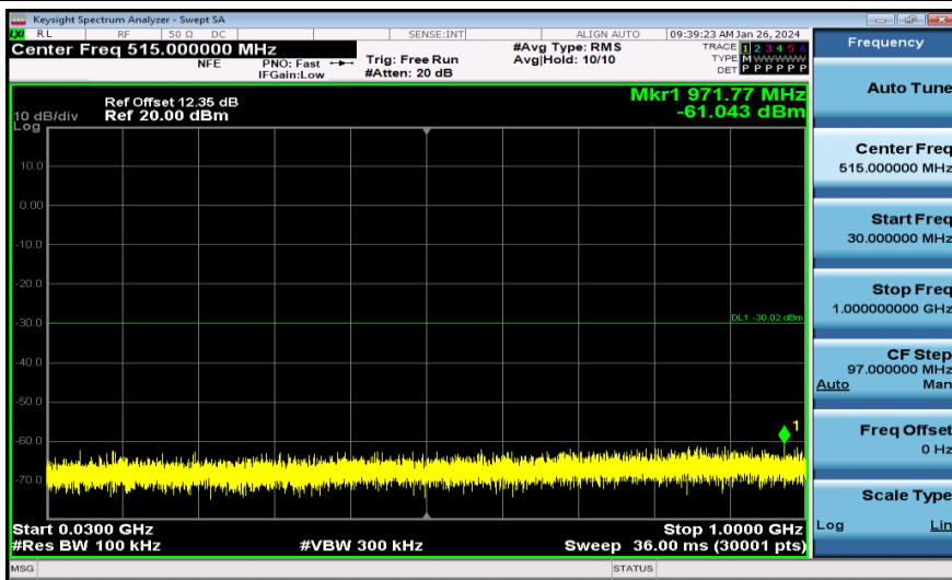
11N40MIMO-Ant1-2422-30~1000-PASS
