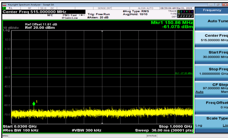
11AX20MIMO-Ant1-2437-30~1000-PASS
