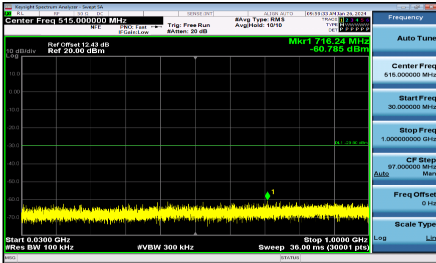
11N40MIMO-Ant2-2437-30~1000-PASS
