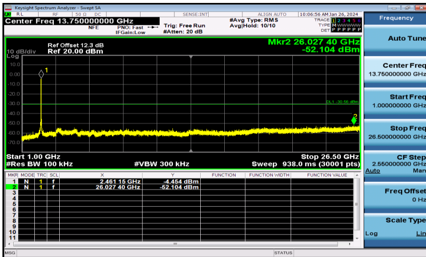
11N40MIMO-Ant1-2452-1000~26500-PASS
