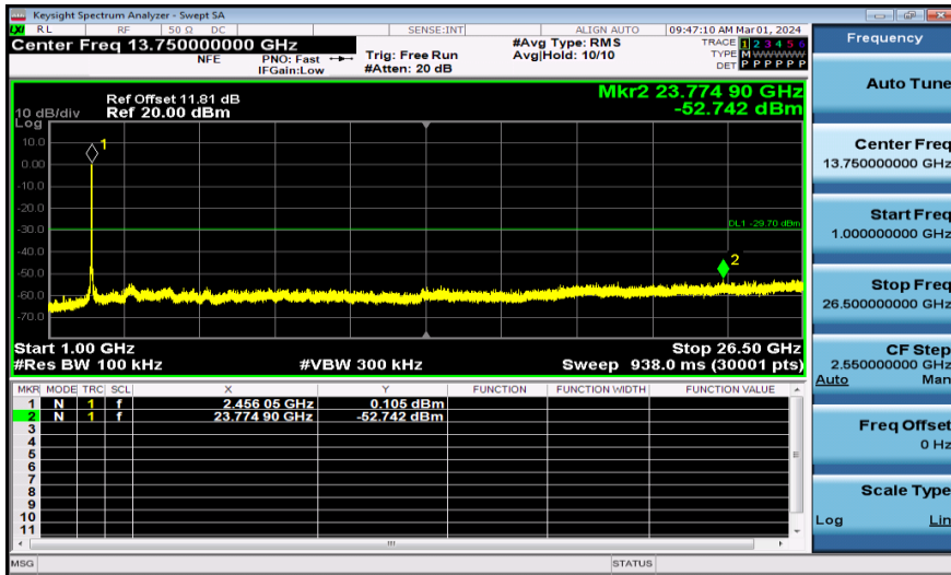
11AX40MIMO-Ant1-2452-1000~26500-PASS
