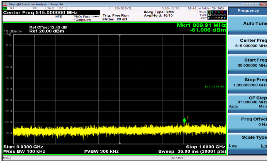
11N40MIMO-Ant2-2422-30~1000-PASS
