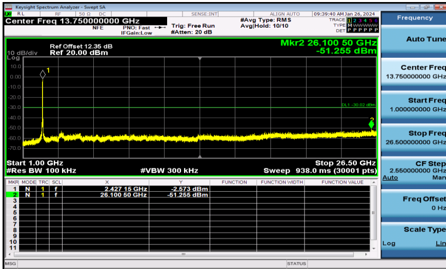
11N40MIMO-Ant1-2422-1000~26500-PASS
