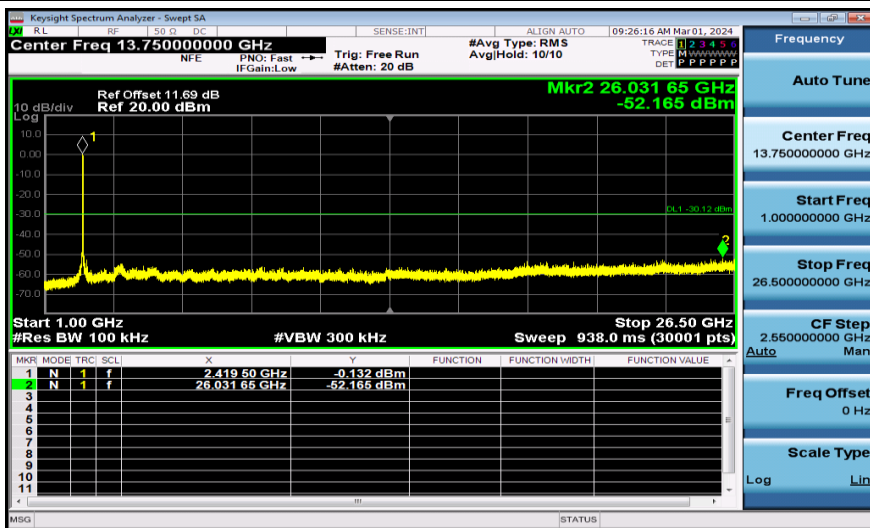
11AX40MIMO-Ant2-2422-1000~26500-PASS
