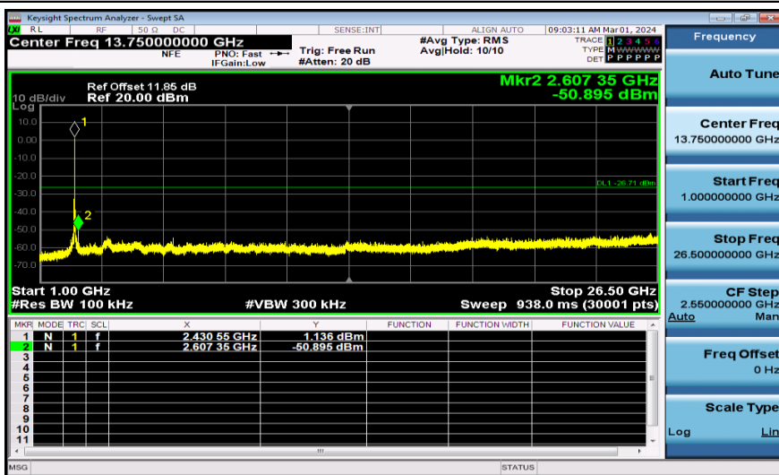
11AX20MIMO-Ant2-2437-1000~26500-PASS
