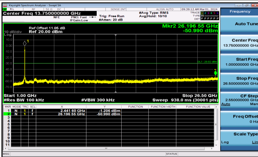
11AX40MIMO-Ant2-2437-1000~26500-PASS
