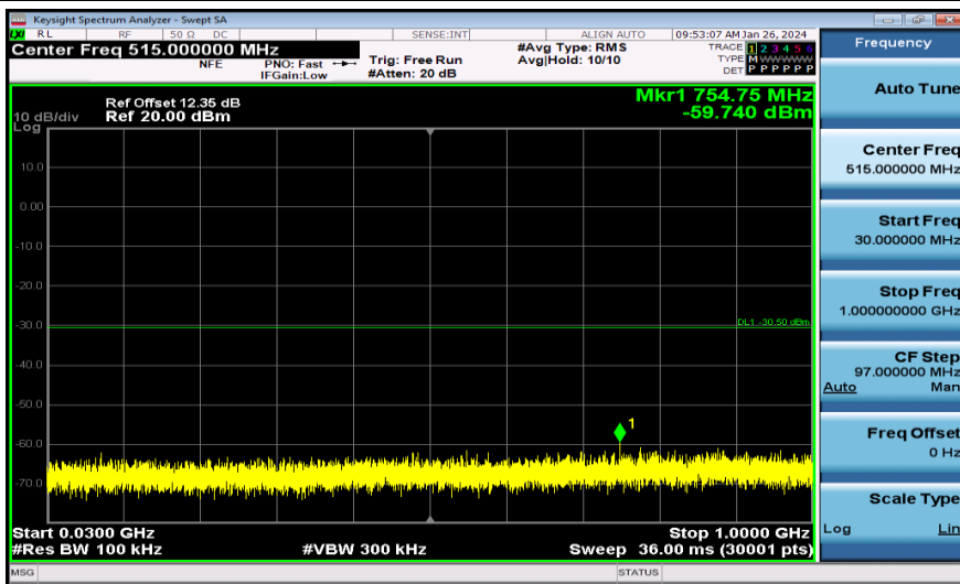
11N40MIMO-Ant1-2437-30~1000-PASS
