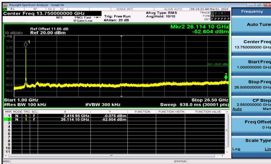
11AX40MIMO-Ant1-2422-1000~26500-PASS
