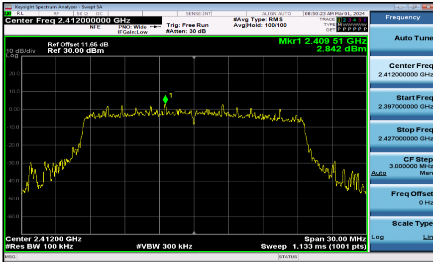
11AX20MIMO-Ant1-2412-0~Reference-PASS
