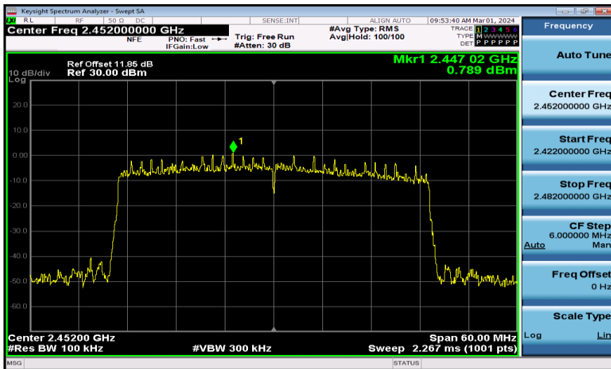
11AX40MIMO-Ant2-2452-0~Reference-PASS
