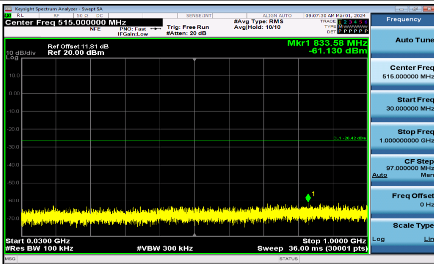
11AX20MIMO-Ant1-2462-30~1000-PASS
