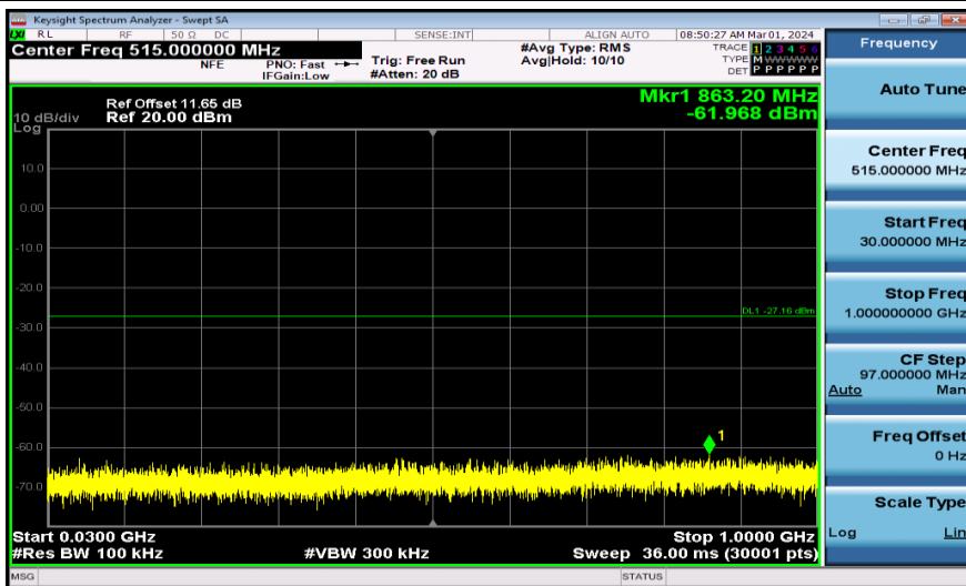
11AX20MIMO-Ant1-2412-30~1000-PASS
