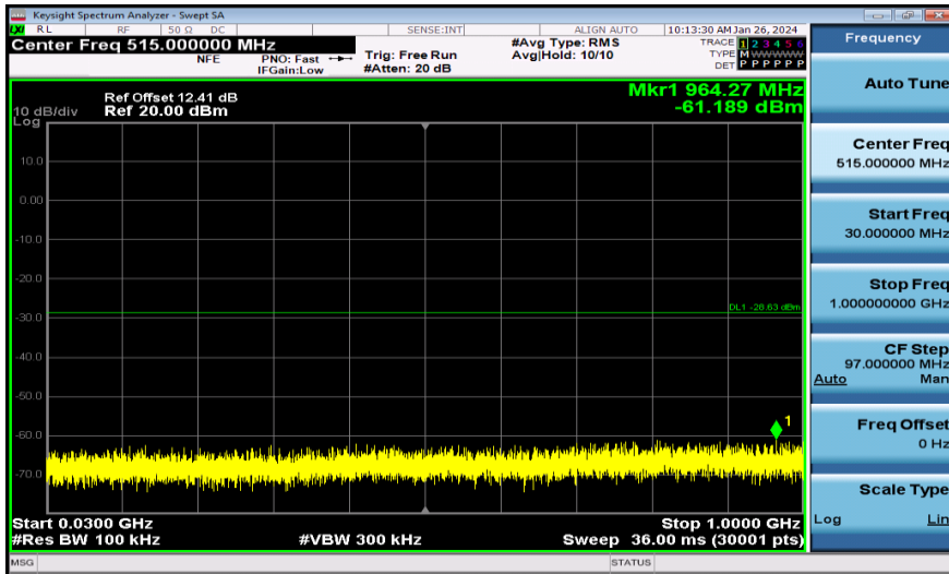
11N40MIMO-Ant2-2452-30~1000-PASS
