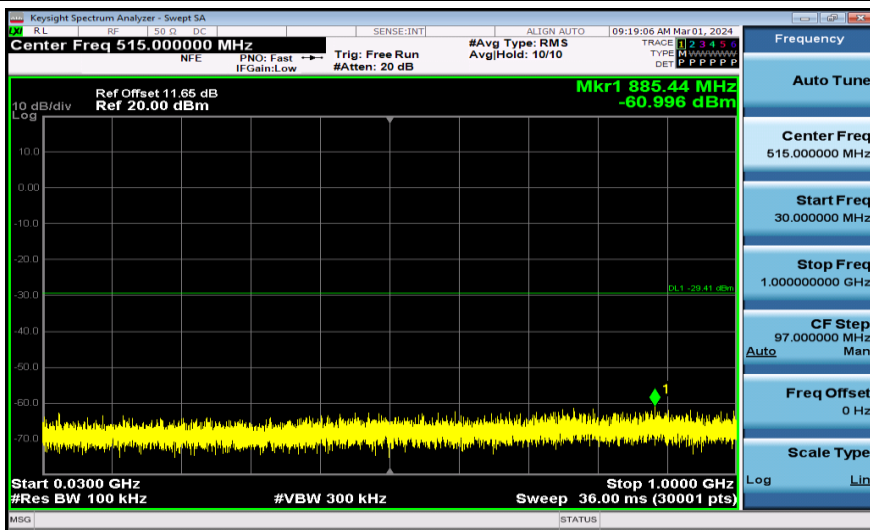
11AX40MIMO-Ant1-2422-30~1000-PASS
