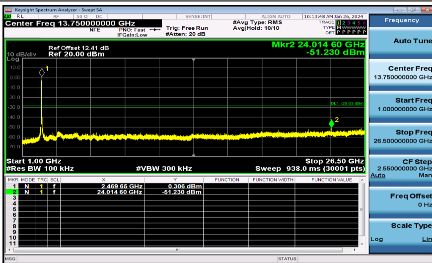
11N40MIMO-Ant2-2452-1000~26500-PASS
