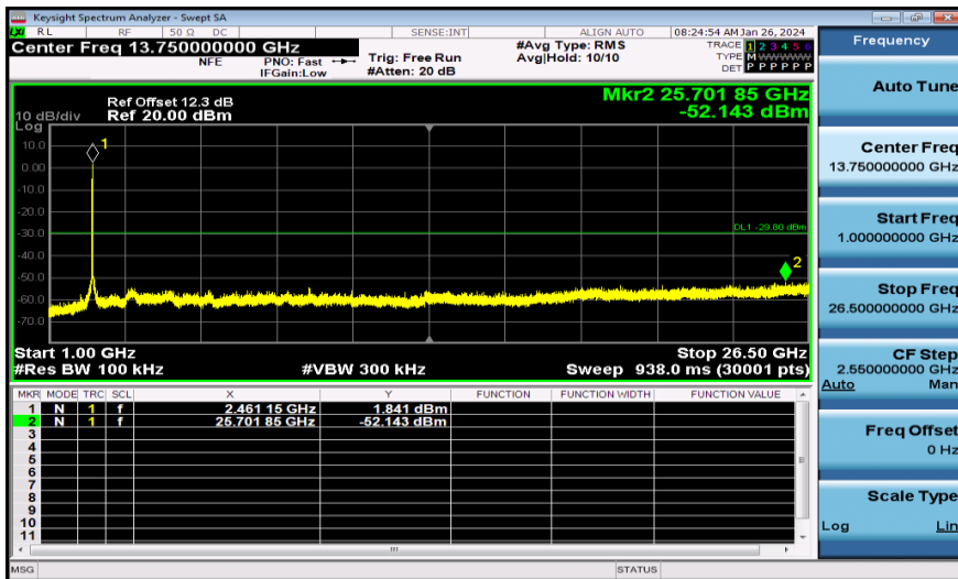
11N20MIMO-Ant1-2462-1000~26500-PASS
