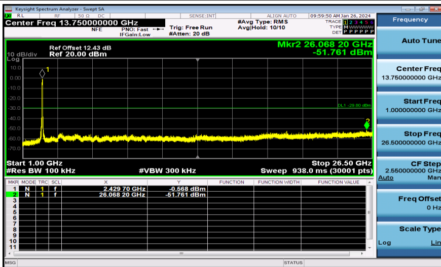
11N40MIMO-Ant2-2437-1000~26500-PASS
