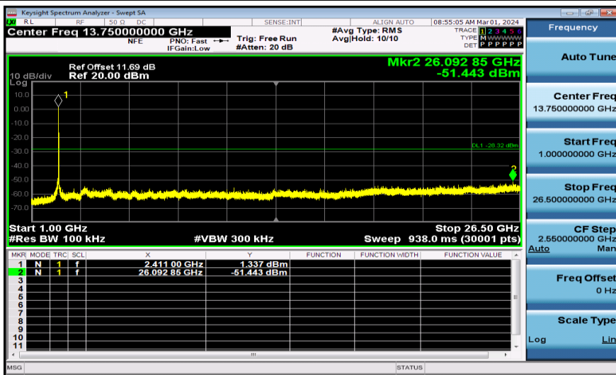
11AX20MIMO-Ant2-2412-1000~26500-PASS
