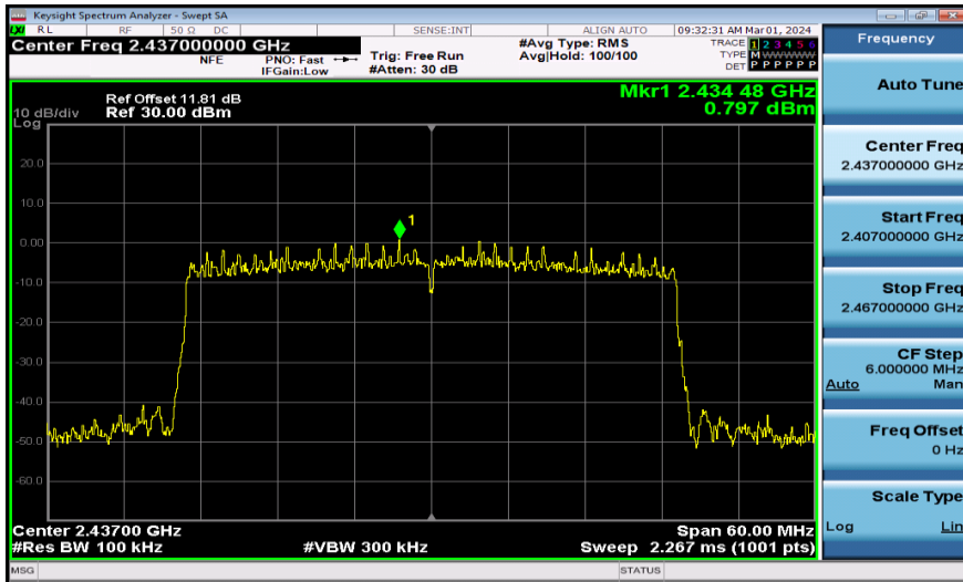
11AX40MIMO-Ant1-2437-0~Reference-PASS
