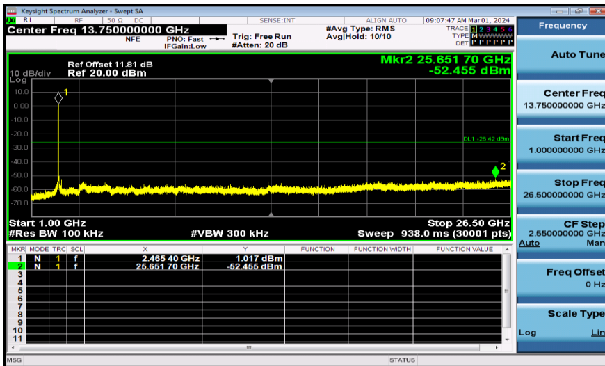
11AX20MIMO-Ant1-2462-1000~26500-PASS
