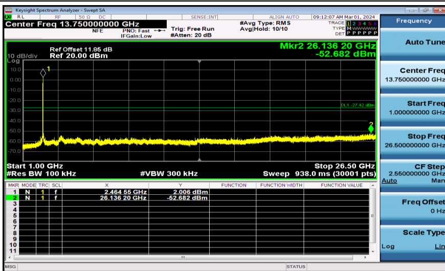
11AX20MIMO-Ant2-2462-1000~26500-PASS
