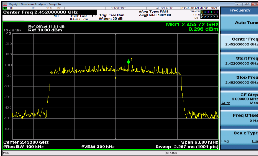
11AX40MIMO-Ant1-2452-0~Reference-PASS
