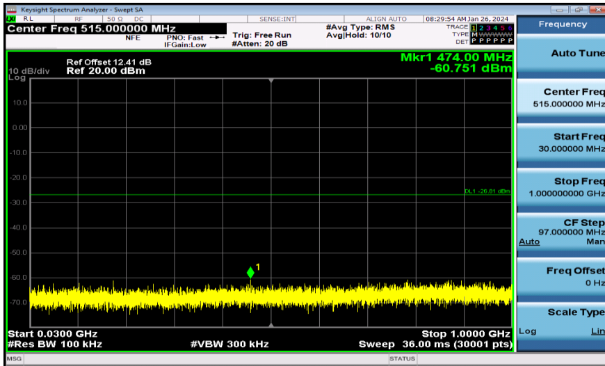
11N20MIMO-Ant2-2462-30~1000-PASS
