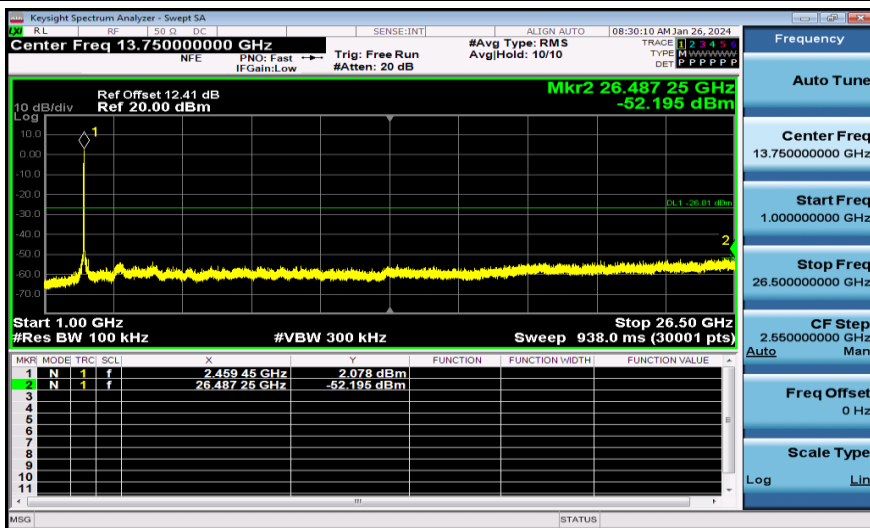
11N20MIMO-Ant2-2462-1000~26500-PASS
