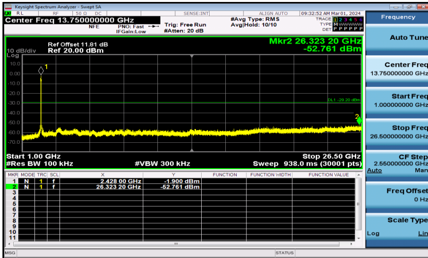
11AX40MIMO-Ant1-2437-1000~26500-PASS
