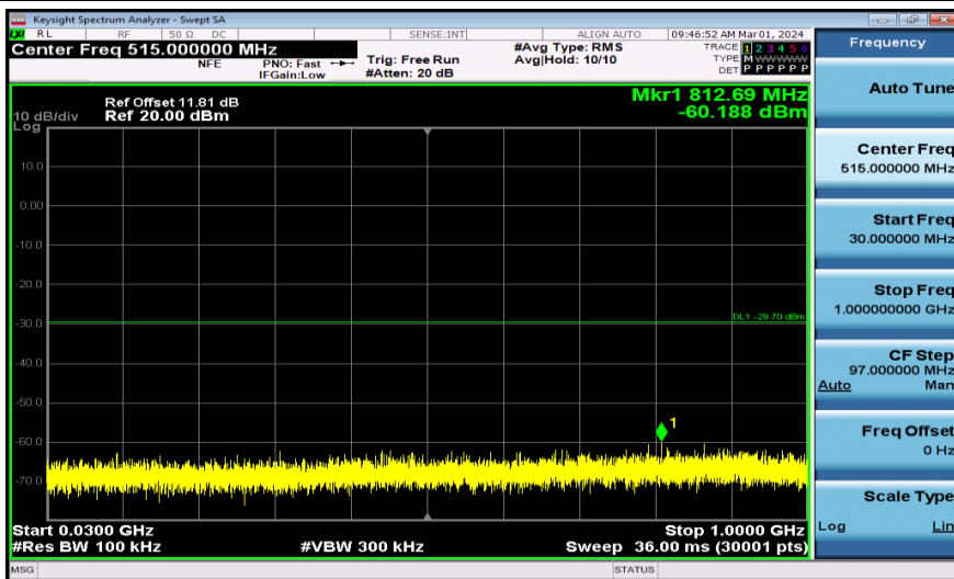
11AX40MIMO-Ant1-2452-30~1000-PASS
