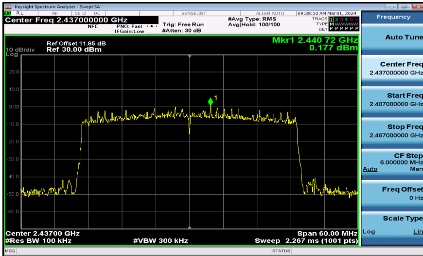
11AX40MIMO-Ant2-2437-0~Reference-PASS
