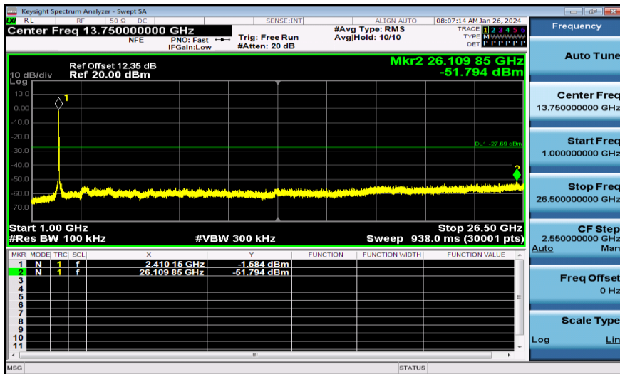
11N20MIMO-Ant1-2412-1000~26500-PASS
