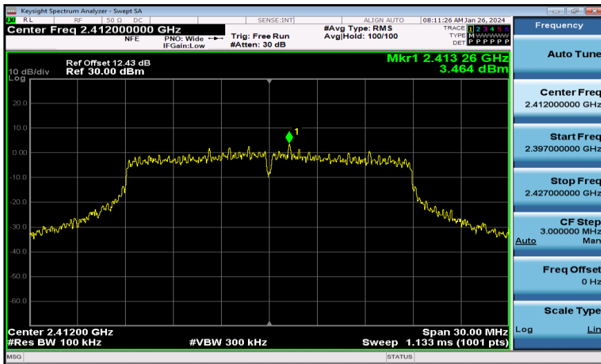
11N20MIMO-Ant2-2412-0-Reference-PASS
