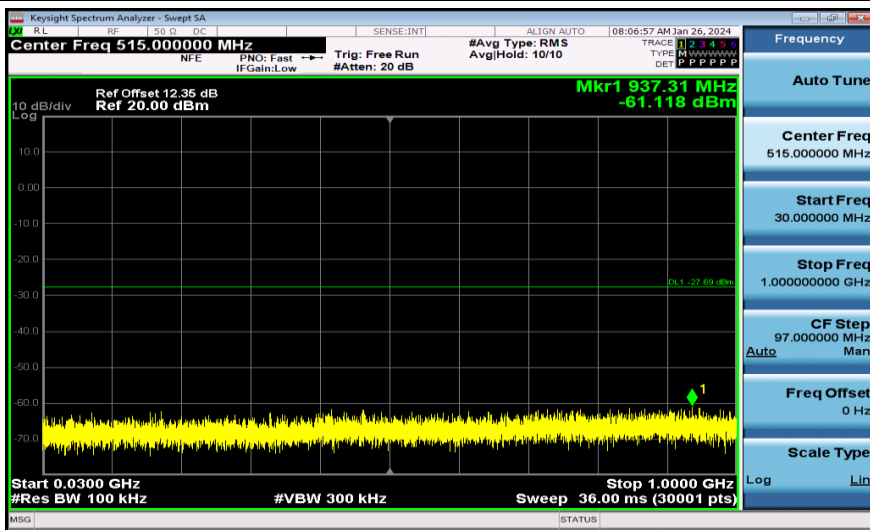
11N20MIMO-Ant1-2412-30~1000-PASS
