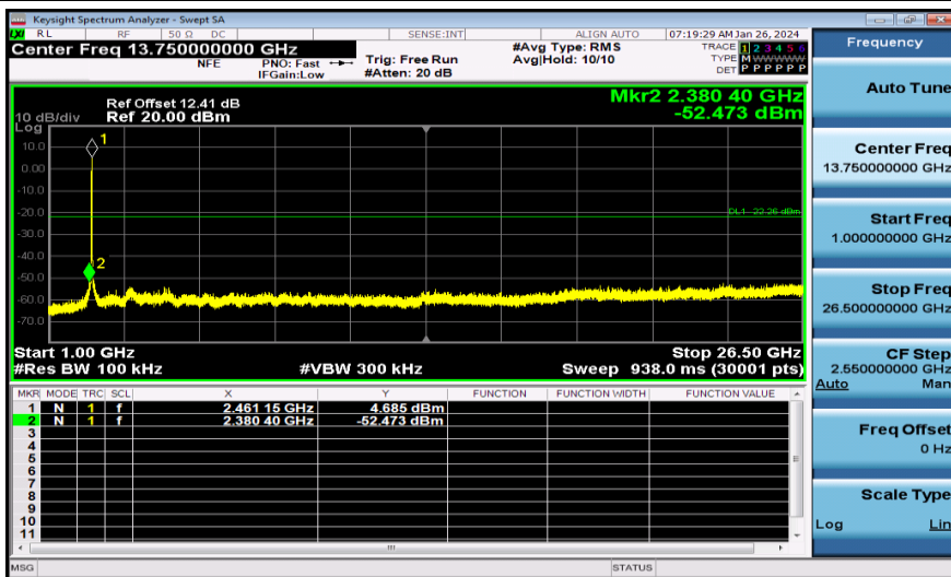
11G-Ant2-2462-1000~26500-PASS
