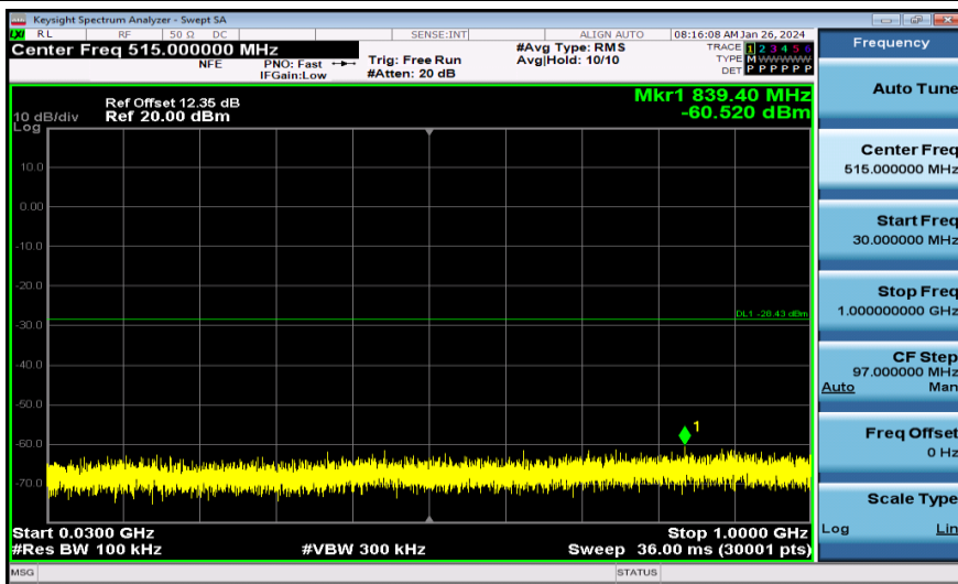
11N20MIMO-Ant1-2437-30~1000-PASS
