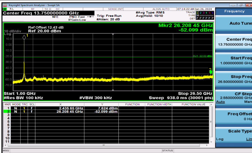
11G-Ant2-2437-1000~26500-PASS
