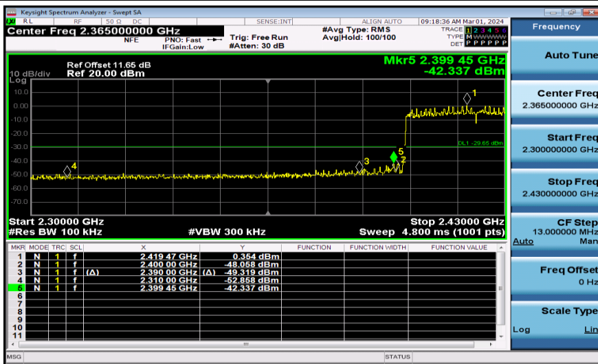
11AX40MIMO-Ant1-2422-PASS
