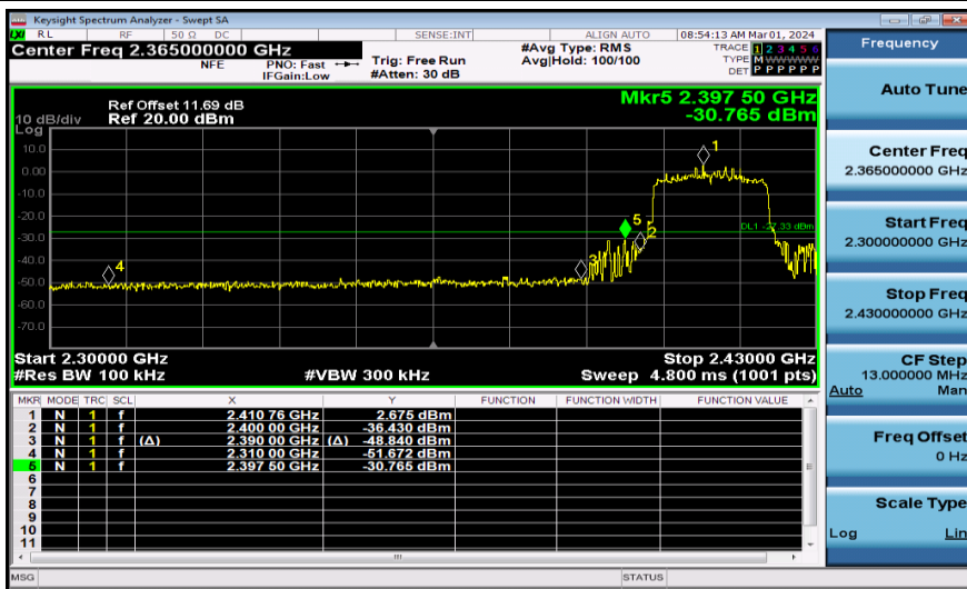
11AX20MIMO-Ant2-2412-PASS
