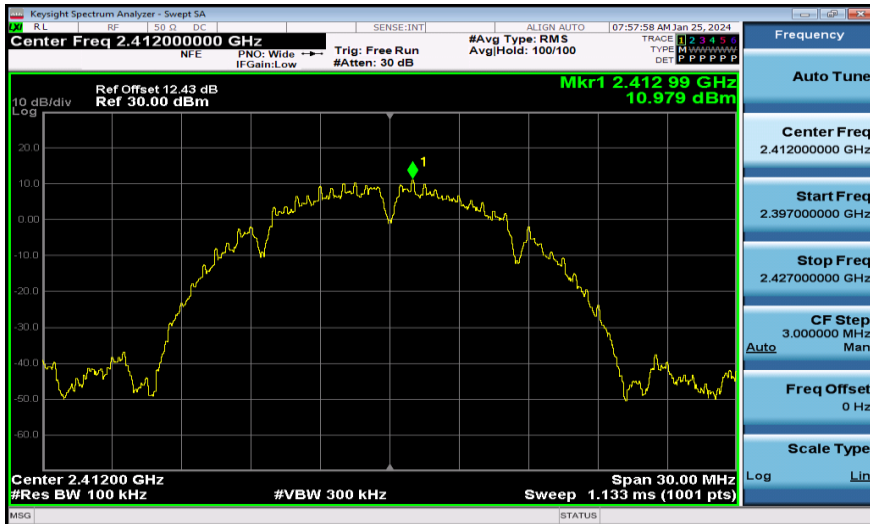
11B-Ant2-2412-0~Reference-PASS
