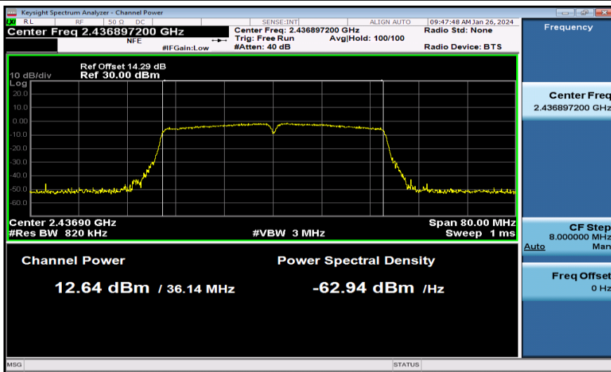
11N40MIMO-Ant1-2437-PASS
