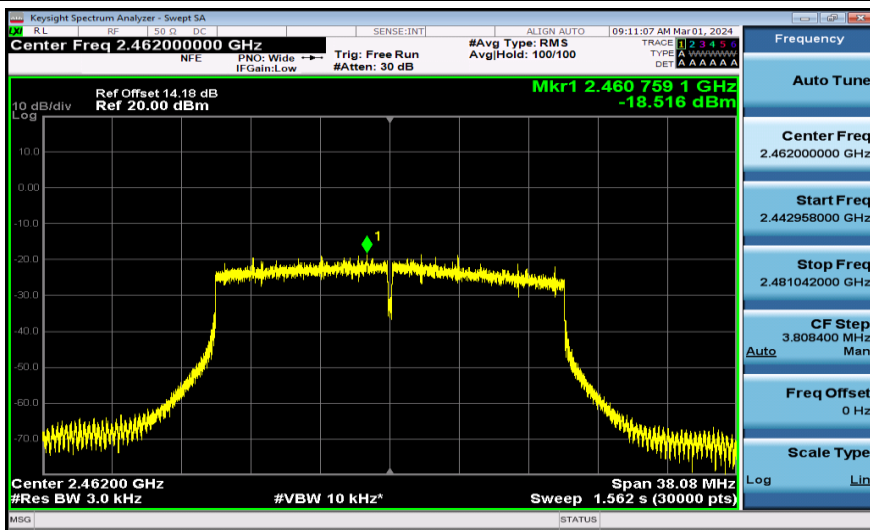
11AX20MIMO-Ant2-2462-PASS
