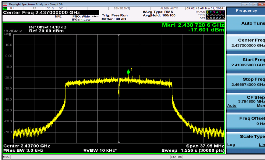
11AX20MIMO-Ant2-2437-PASS
