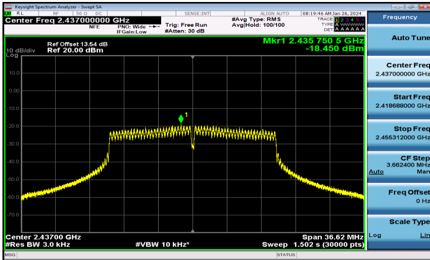
11N20MIMO-Ant2-2437-PASS
