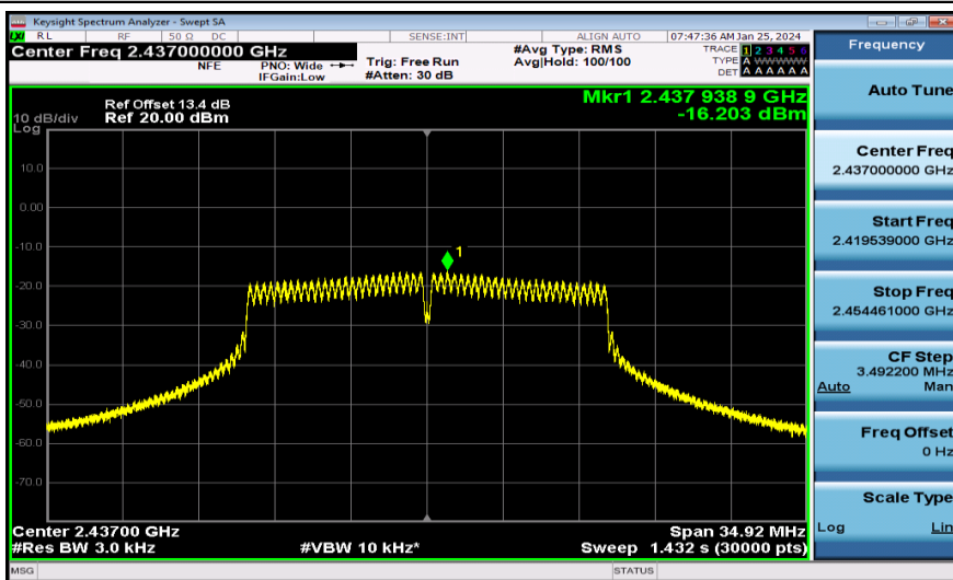
11G-Ant1-2437-PASS
