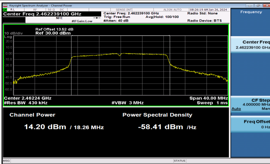
11N20MIMO-Ant2-2462-PASS
