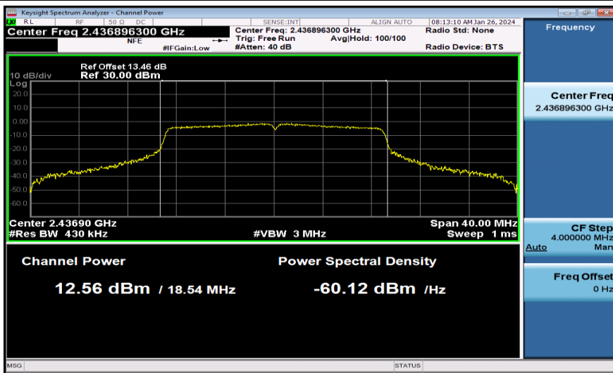
11N20MIMO-Ant1-2437-PASS
