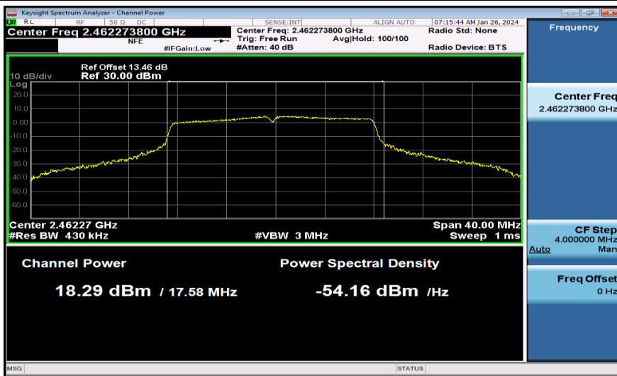
11G-Ant2-2462-PASS
