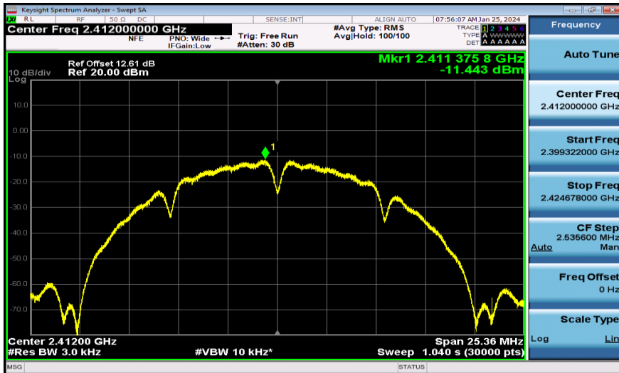
11B-Ant2-2412-PASS
