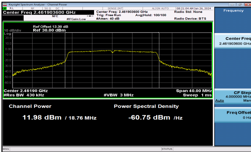
11N20MIMO-Ant1-2462-PASS
