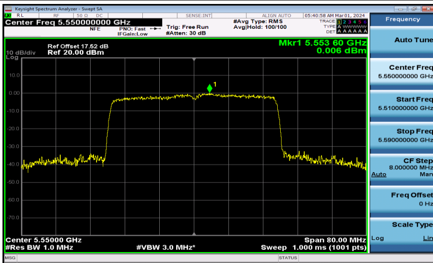
11AX40MIMO-Ant1-5550-PASS
