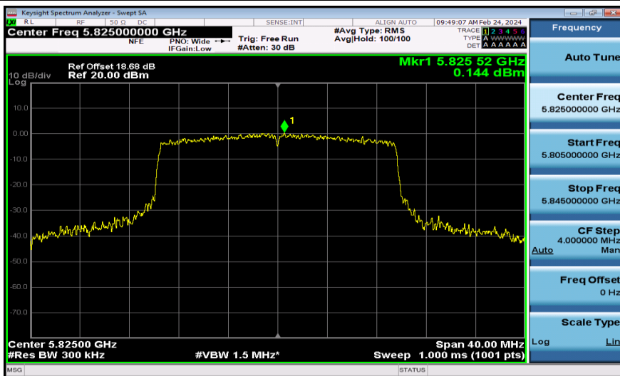
11AX20MIMO-Ant1-5825-PASS
