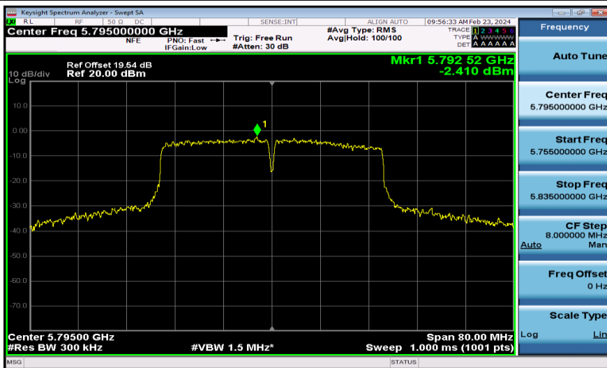
11AC40MIMO-Ant2-5795-PASS
