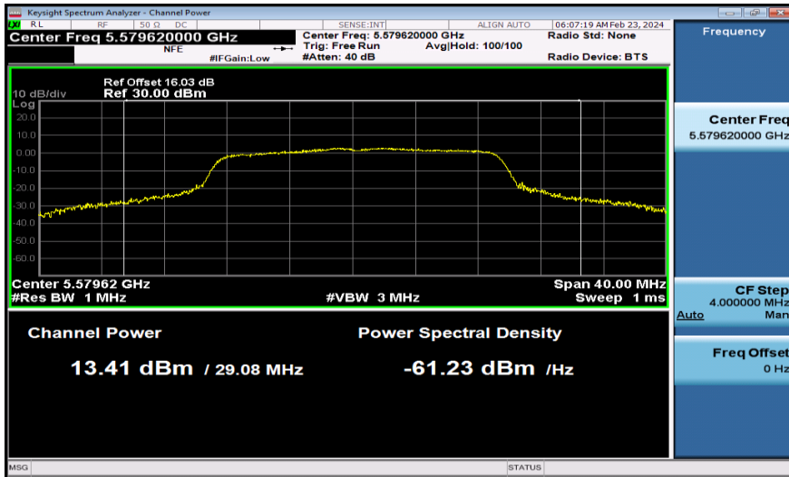
11AC20MIMO-Ant2-5580-PASS
