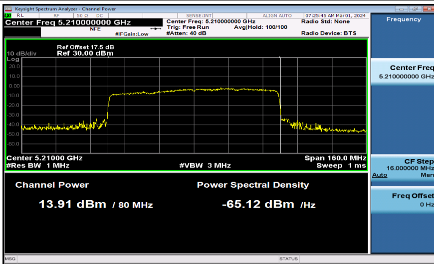
11AX80MIMO-Ant2-5210-PASS
