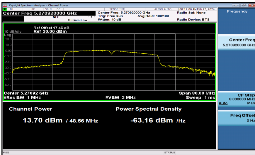
11AC40MIMO-Ant2-5270-PASS
