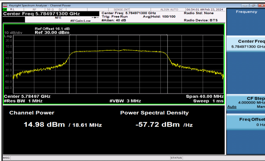
11AC20MIMO-Ant1-5785-PASS
