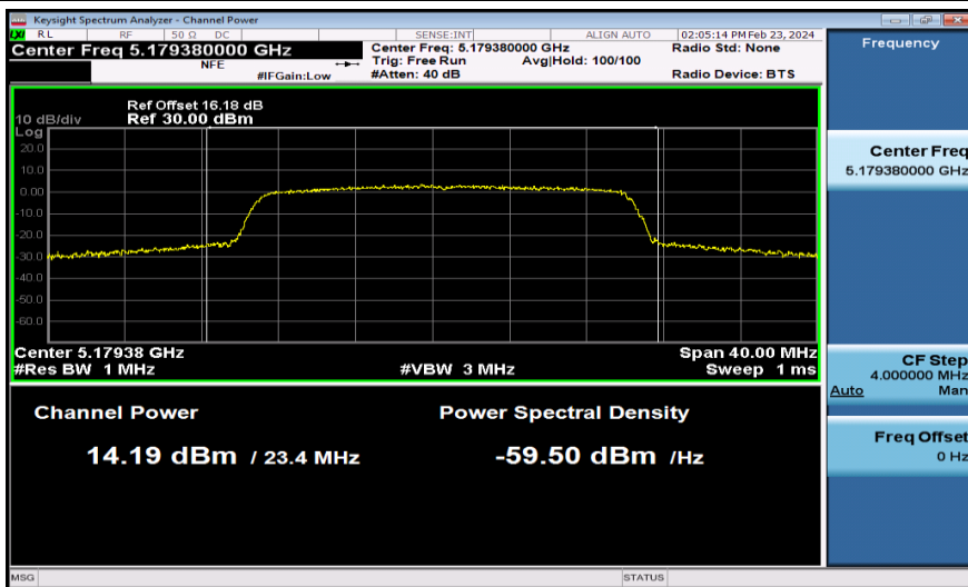
11AX20MIMO-Ant2-5180-PASS
