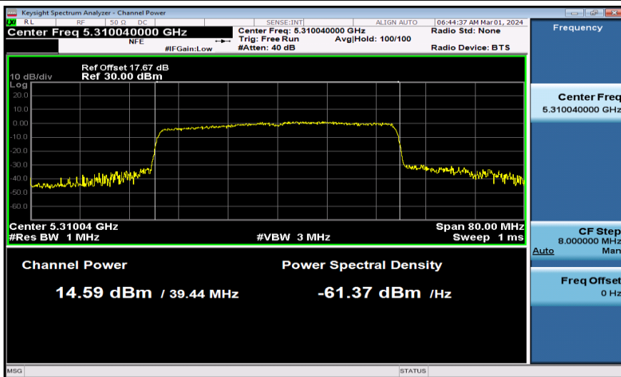
11AX40MIMO-Ant2-5310-PASS
