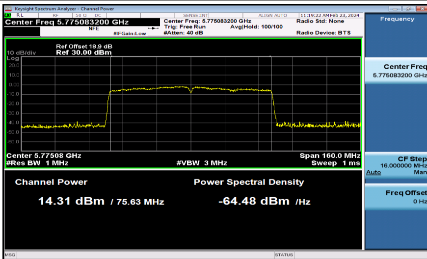
11AC80MIMO-Ant1-5775-PASS
