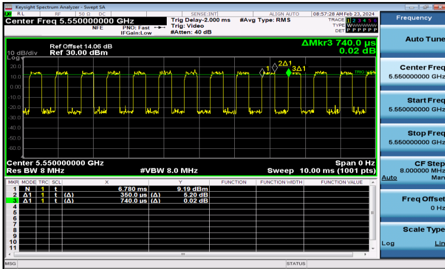
NTNV-11AC40MIMO-Ant1-5550
