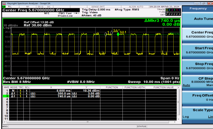
NTNV-11AC40MIMO-Ant2-5670
