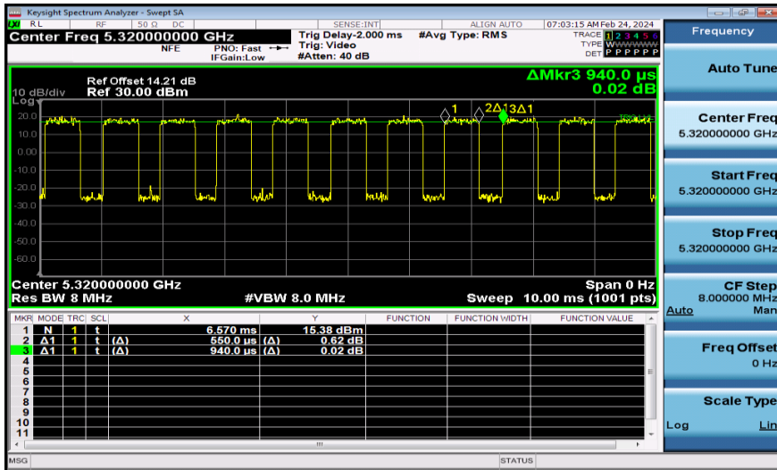
NTNV-11AX20MIMO-Ant2-5320
