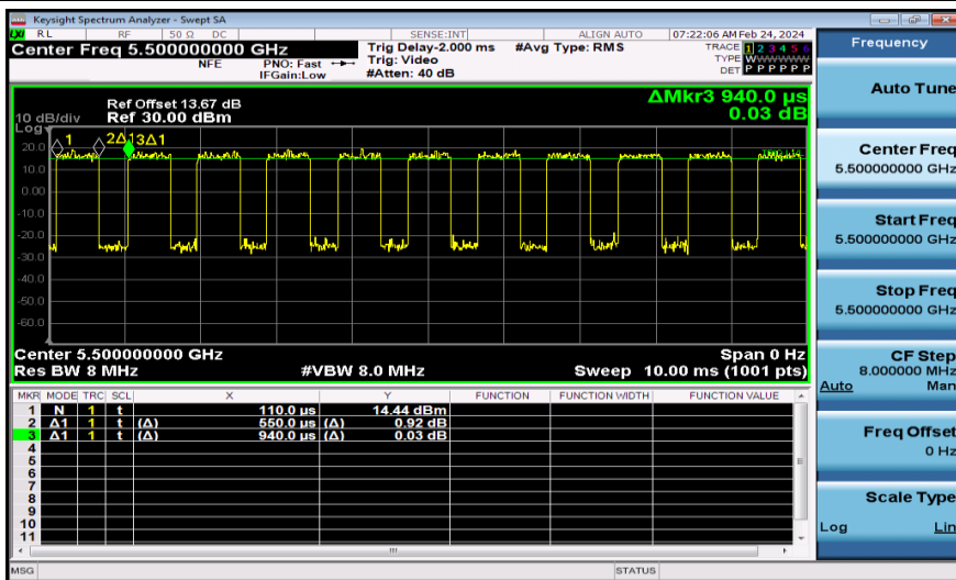
NTNV-11AX20MIMO-Ant2-5500
