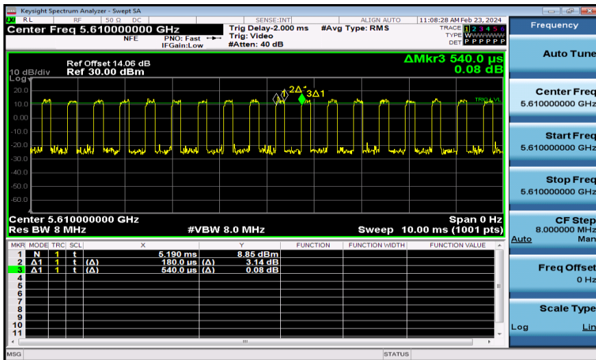
NTNV-11AC80MIMO-Ant2-5610
