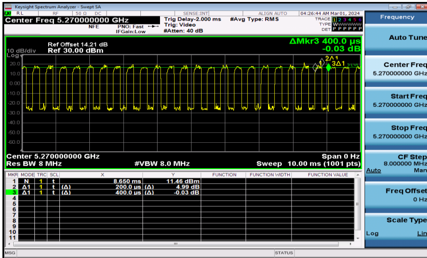
NTNV-11AX40MIMO-Ant2-5270
