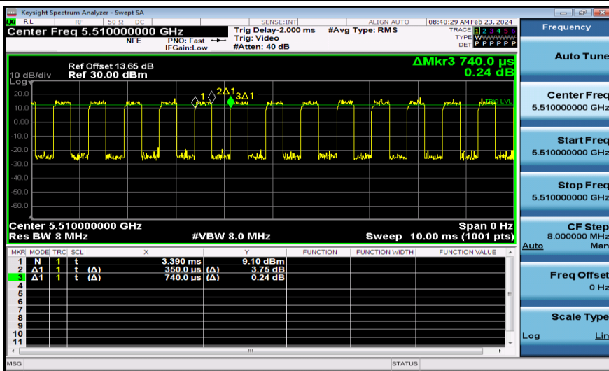
NTNV-11AC40MIMO-Ant1-5510
