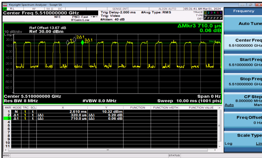
NTNV-11AX40MIMO-Ant2-5510
