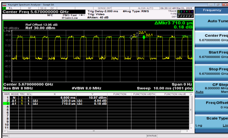
NTNV-11AX40MIMO-Ant2-5670
