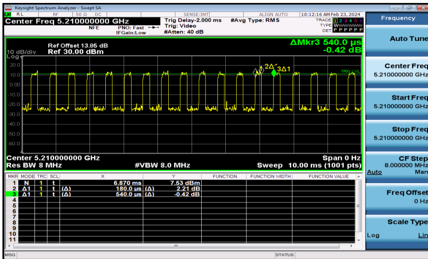
NTNV-11AC80MIMO-Ant2-5210
