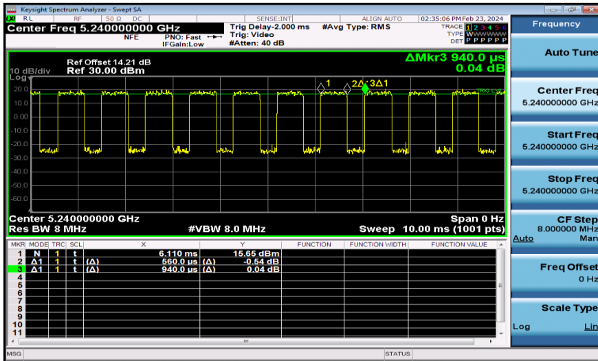
NTNV-11AX20MIMO-Ant2-5240
