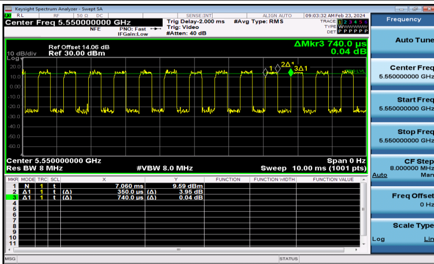
NTNV-11AC40MIMO-Ant2-5550
