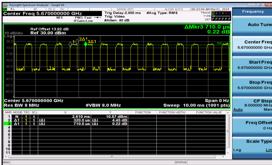
NTNV-11AX40MIMO-Ant1-5670
