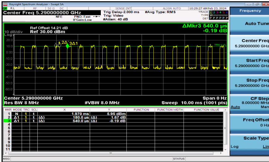
NTNV-11AC80MIMO-Ant2-5290
