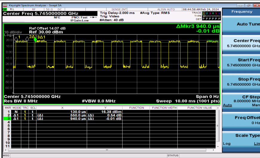
NTNV-11AX20MIMO-Ant2-5745
