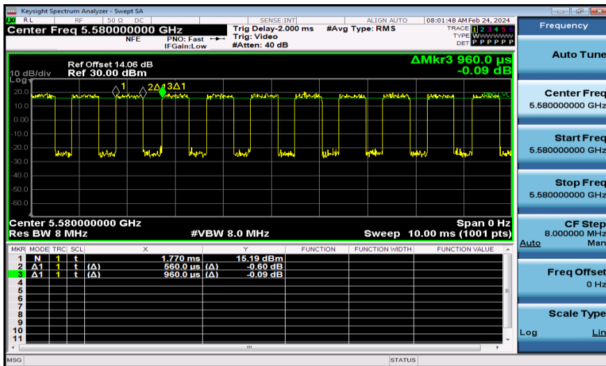
NTNV-11AX20MIMO-Ant2-5580
