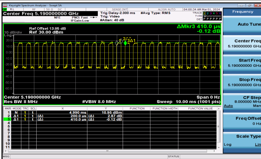
NTNV-11AX40MIMO-Ant2-5190
