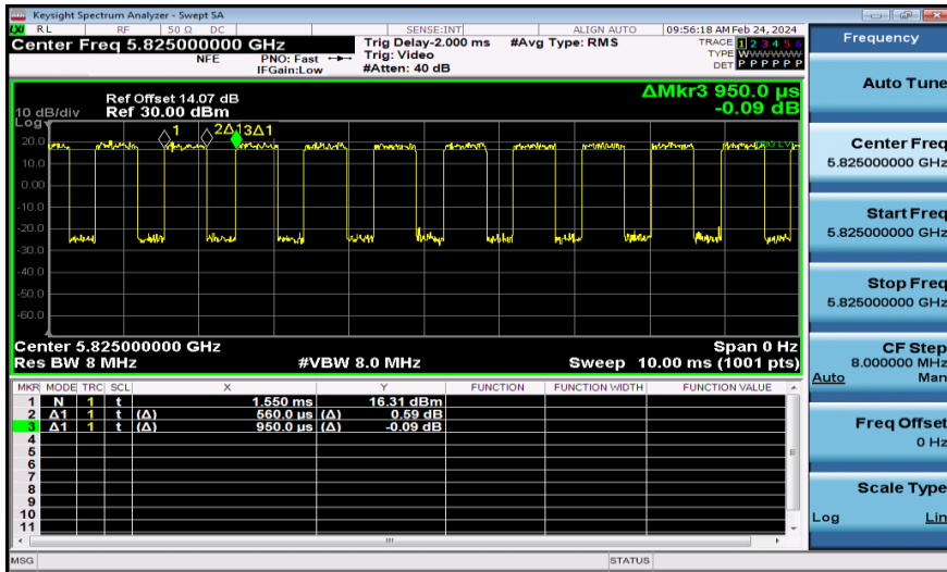
NTNV-11AX20MIMO-Ant2-5825
