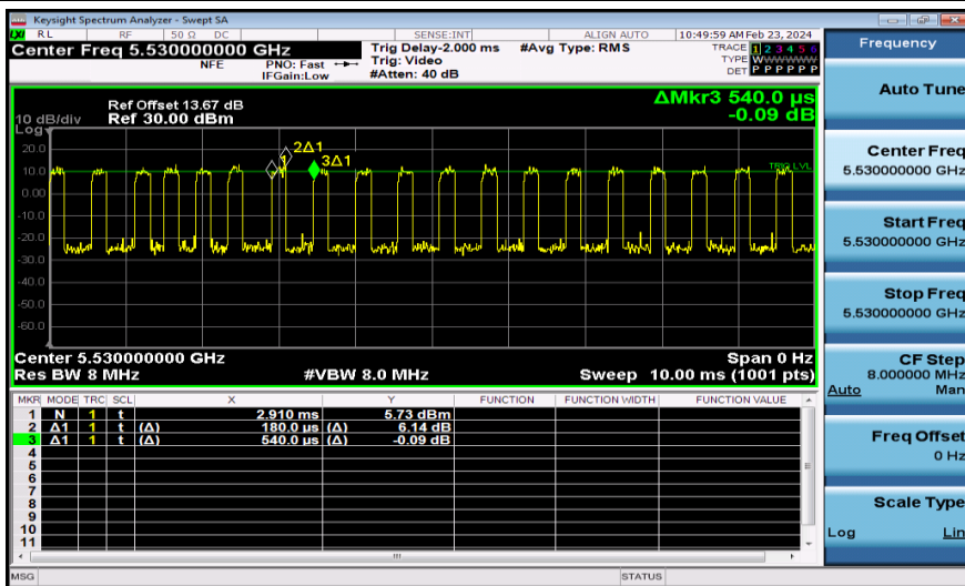
NTNV-11AC80MIMO-Ant2-5530
