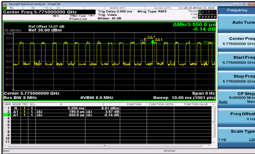
NTNV-11AC80MIMO-Ant2-5775
