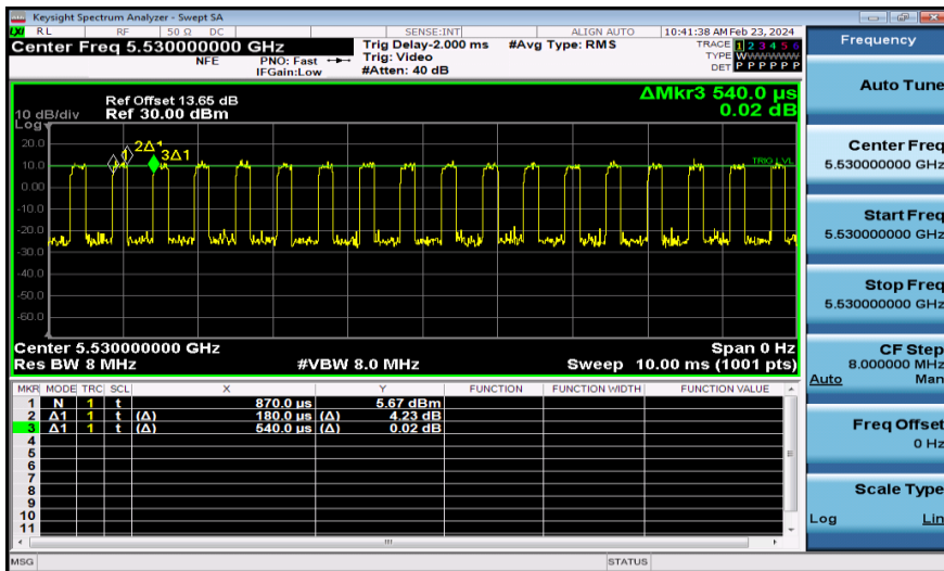
NTNV-11AC80MIMO-Ant1-5530
