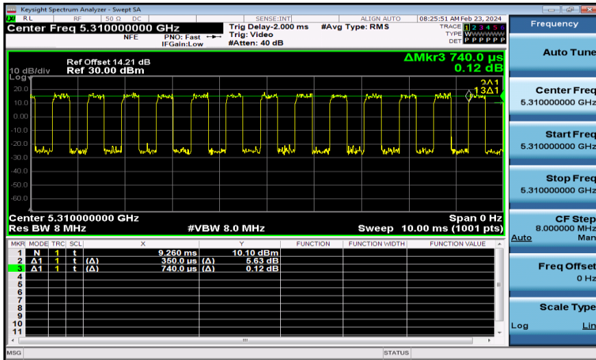
NTNV-11AC40MIMO-Ant2-5310
