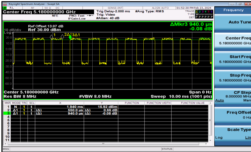
NTNV-11AX20MIMO-Ant1-5180
