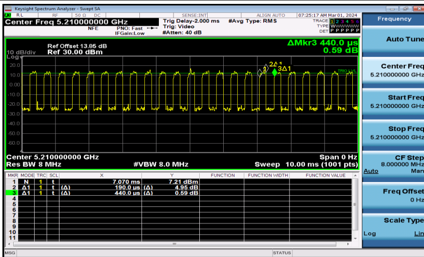
NTNV-11AX80MIMO-Ant2-5210
