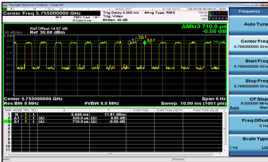
NTNV-11AX40MIMO-Ant2-5755
