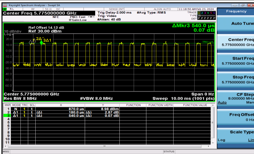
NTNV-11AC80MIMO-Ant1-5775
