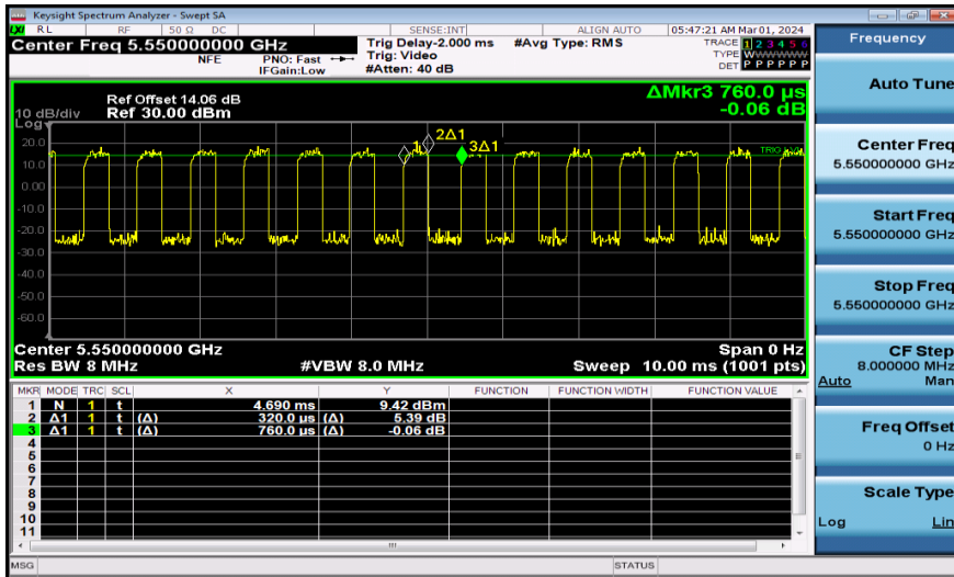
NTNV-11AX40MIMO-Ant2-5550
