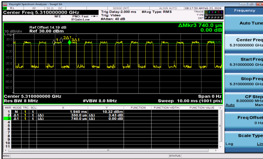
NTNV-11AC40MIMO-Ant1-5310
