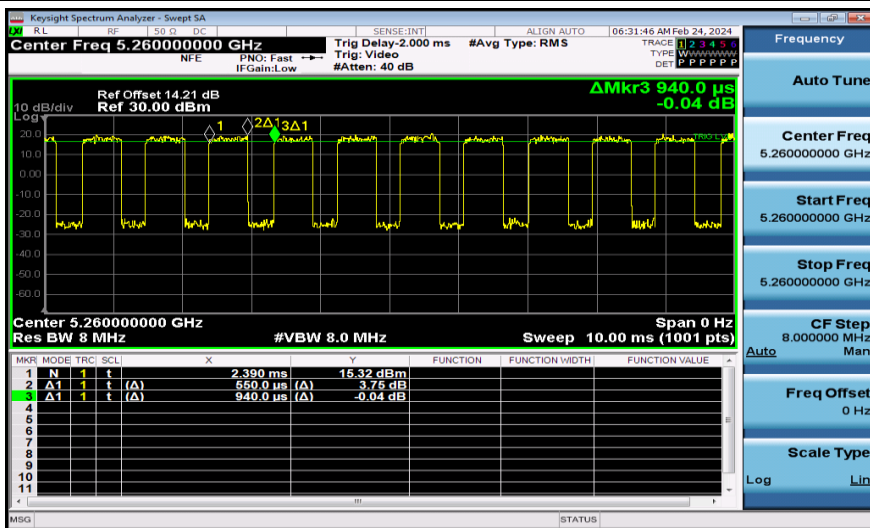
NTNV-11AX20MIMO-Ant2-5260
