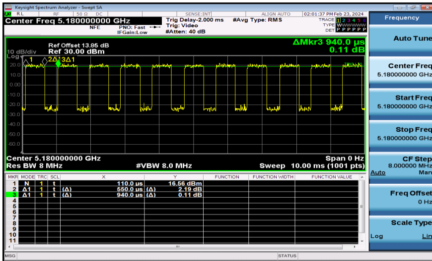
NTNV-11AX20MIMO-Ant2-5180
