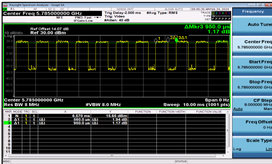
NTNV-11AX20MIMO-Ant2-5785
