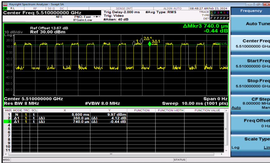
NTNV-11AC40MIMO-Ant2-5510
