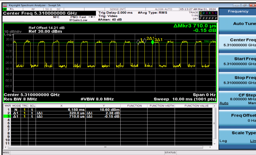
NTNV-11AX40MIMO-Ant2-5310
