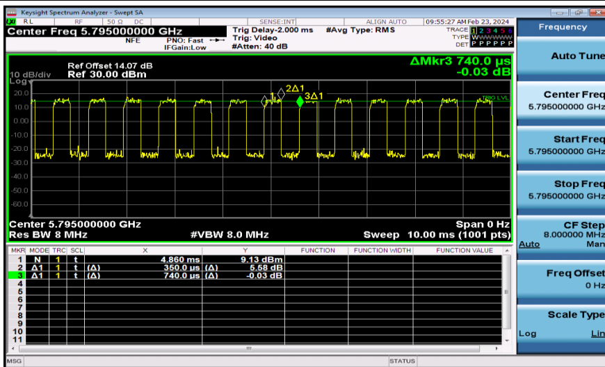
NTNV-11AC40MIMO-Ant2-5795
