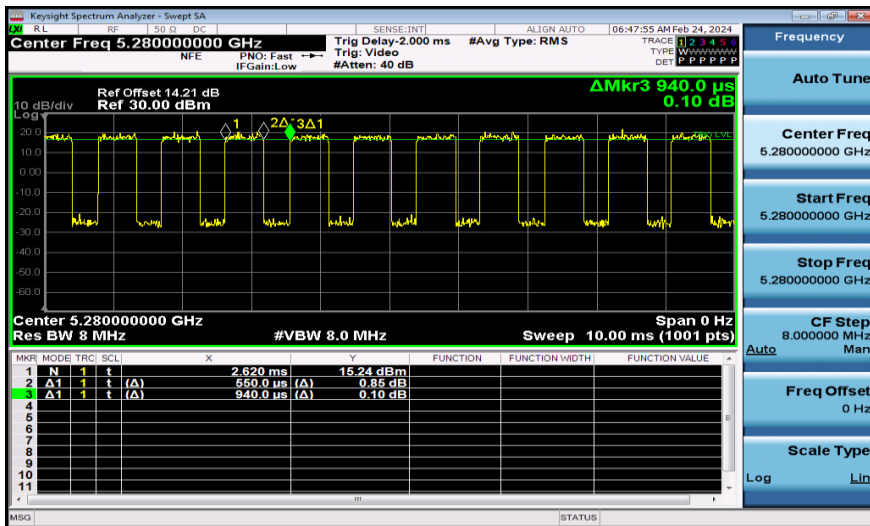
NTNV-11AX20MIMO-Ant2-5280
