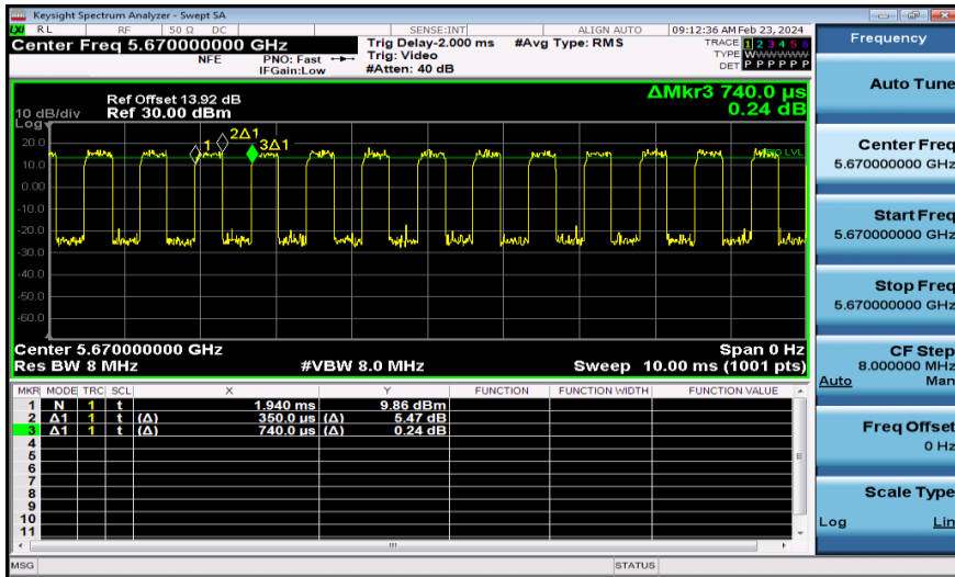
NTNV-11AC40MIMO-Ant1-5670
