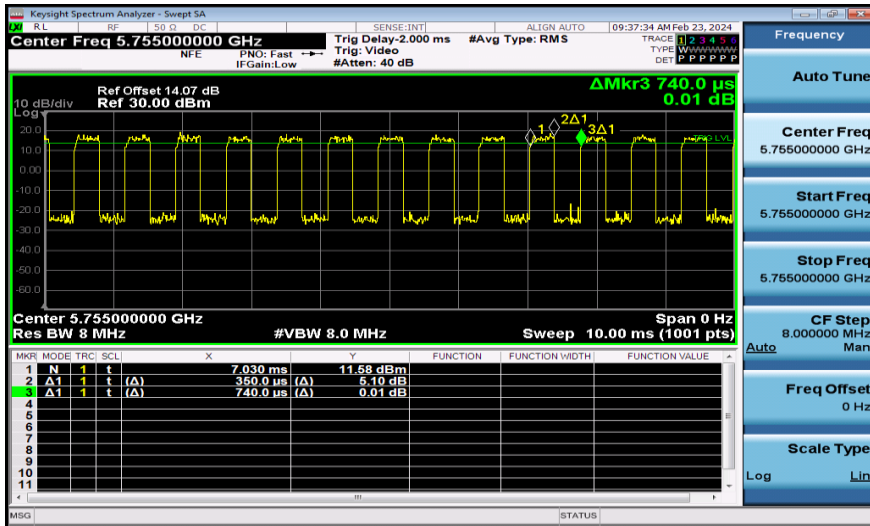
NTNV-11AC40MIMO-Ant2-5755
