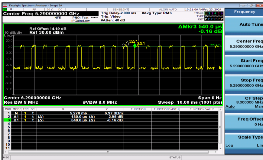
NTNV-11AC80MIMO-Ant1-5290
