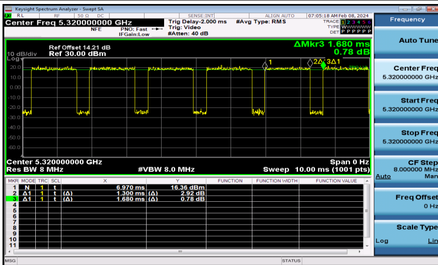
NTNV-11N20MIMO-Ant2-5320
