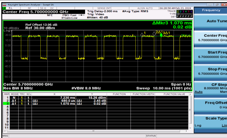
NTNV-11AC20MIMO-Ant2-5700
