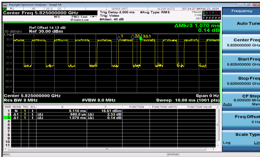
NTNV-11AC20MIMO-Ant1-5825
