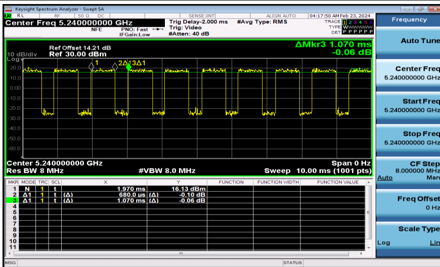
NTNV-11AC20MIMO-Ant2-5240
