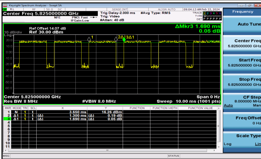
NTNV-11N20MIMO-Ant2-5825
