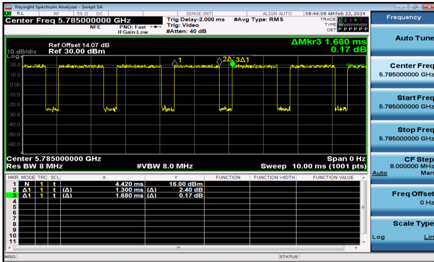
NTNV-11N20MIMO-Ant2-5785
