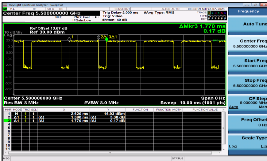
NTNV-11A-Ant2-5500
