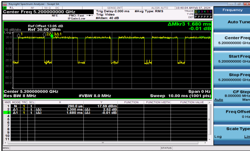
NTVN-11N20MIMO-Ant2-5200
