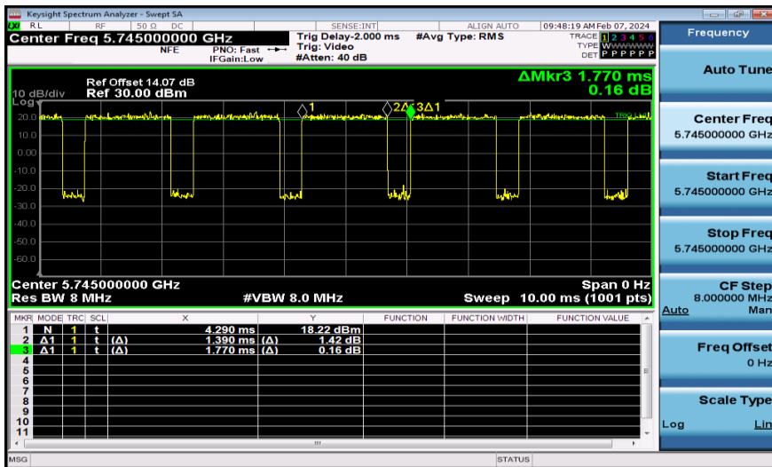
NTNV-11A-Ant2-5745
