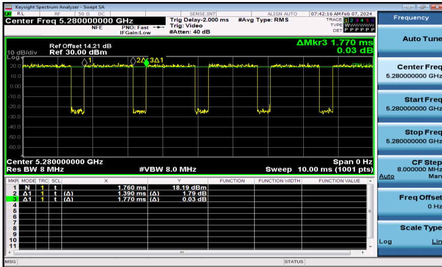
NTNV-11A-Ant2-5280
