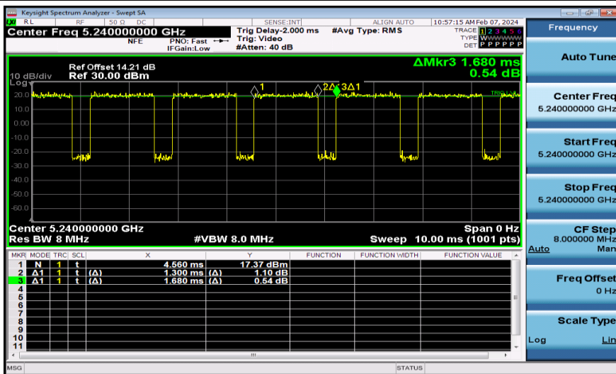
NTVN-11N20MIMO-Ant2-5240
