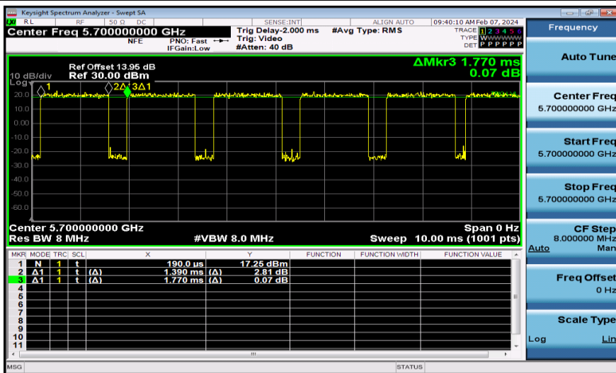
NTNV-11A-Ant2-5700
