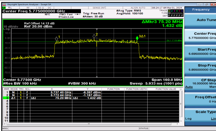
11AX80MIMO-Ant1-5775-PASS
