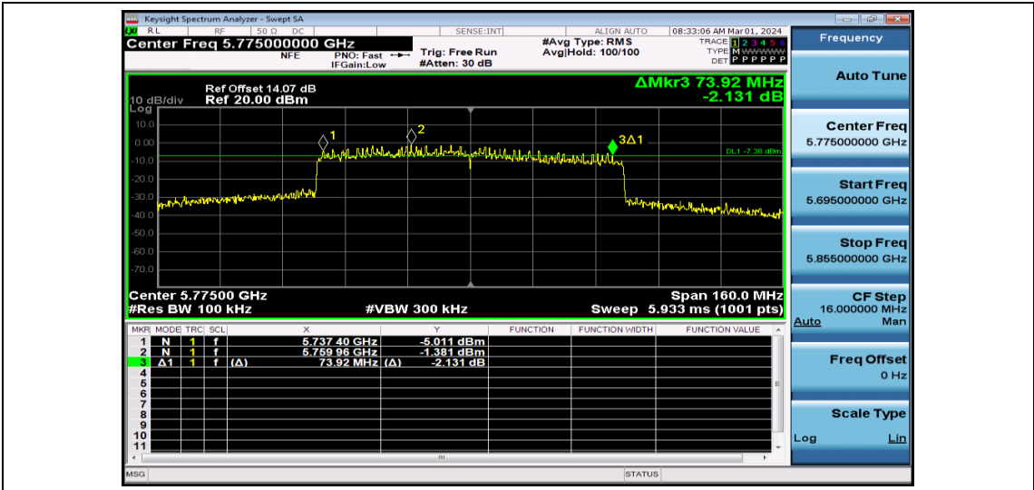
11AX80MIMO-Ant2-5775-PASS
