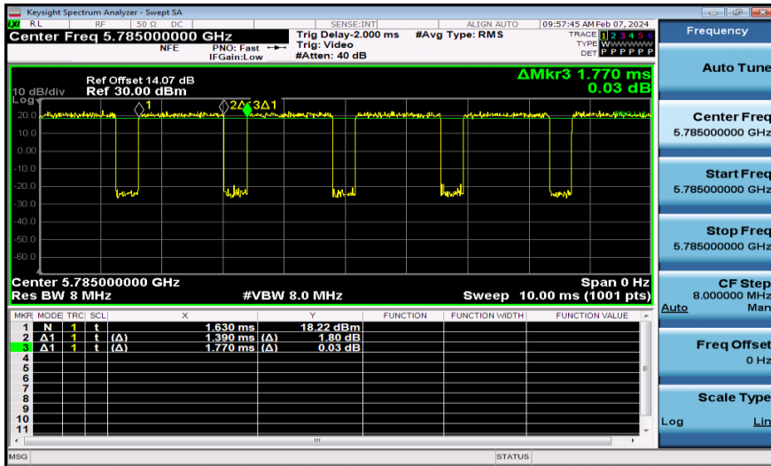
NTNV-11A-Ant2-5785
