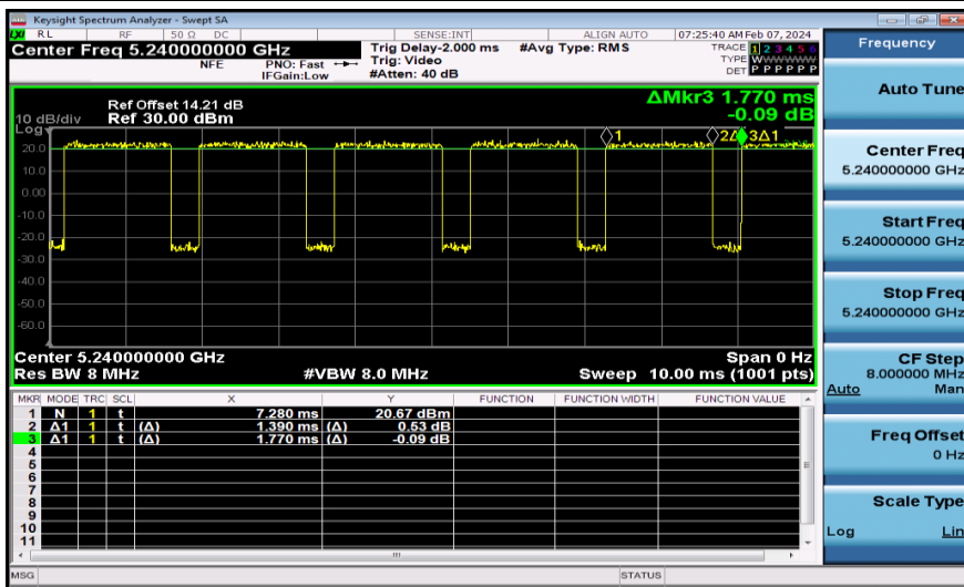
NTNV-11A-Ant2-5240
