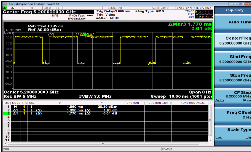
NTNV-11A-Ant2-5200
