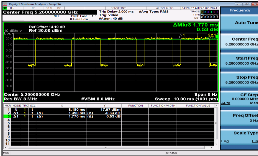
NTNV-11A-Ant1-5260
