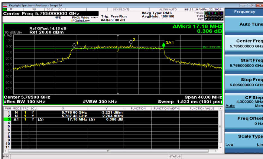
11N20MIMO-Ant1-5785-PASS
