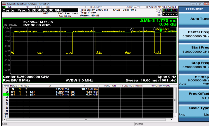
NTNV-11A-Ant2-5260
