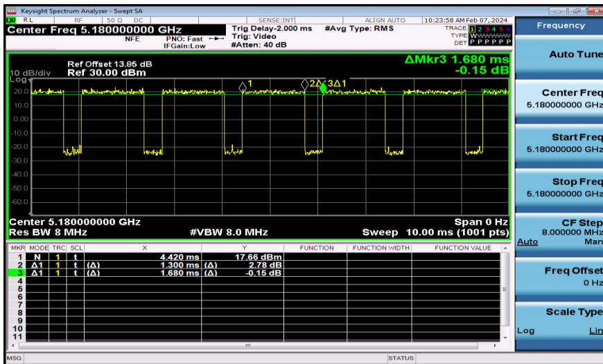
NTNV-11N20MIMO-Ant2-5180
