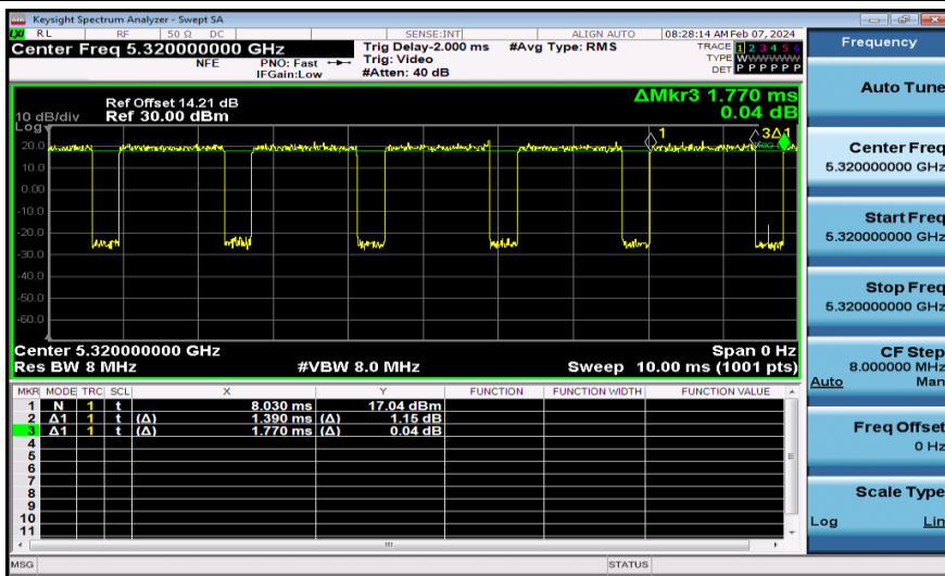
NTNV-11A-Ant2-5320
