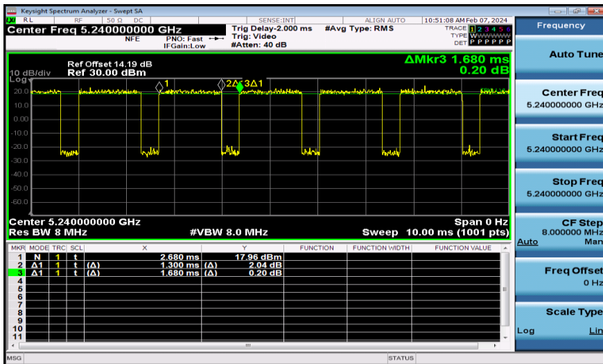
NTVN-11N20MIMO-Ant1-5240
