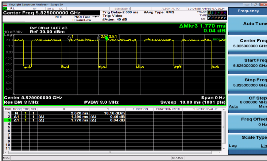
NTNV-11A-Ant2-5825
