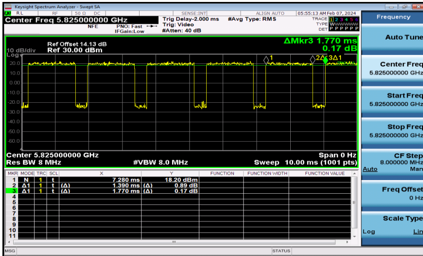
NTNV-11A-Ant1-5825
