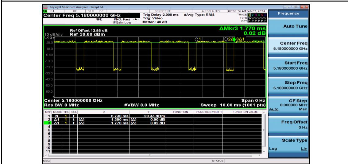
NTNV-11A-Ant2-5180
