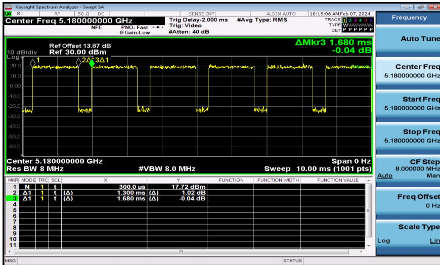
NTNV-11N20MIMO-Ant1-5180
