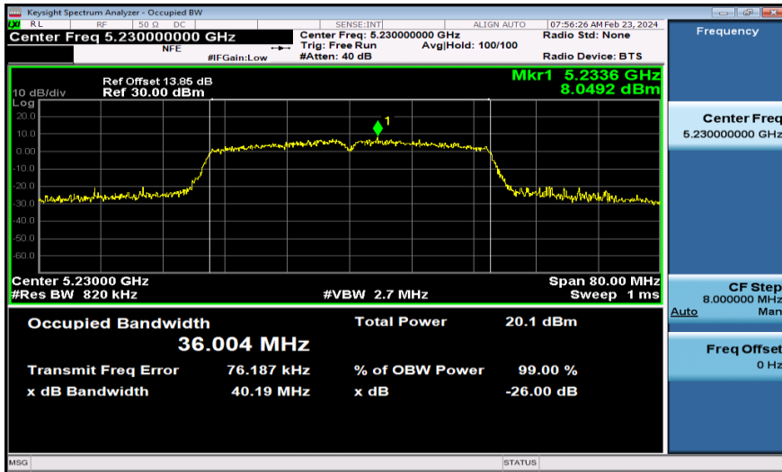
11AC40MIMO-Ant2-5230
