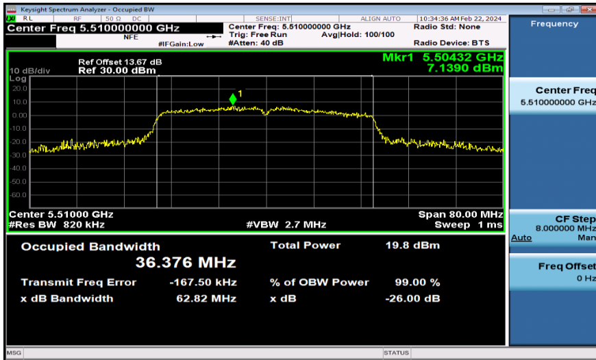
11N40MIMO-Ant2-5510
