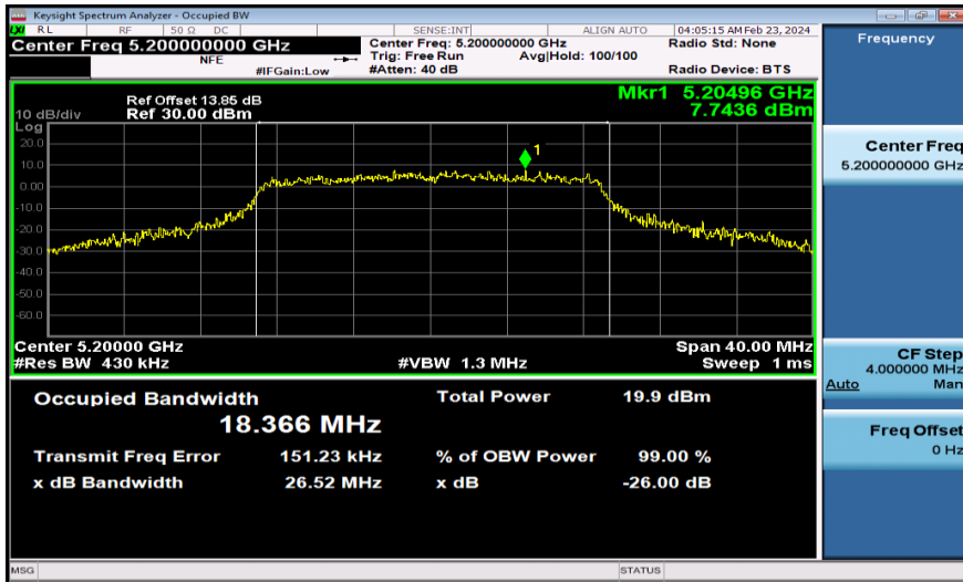
11AC20MIMO-Ant2-5200
