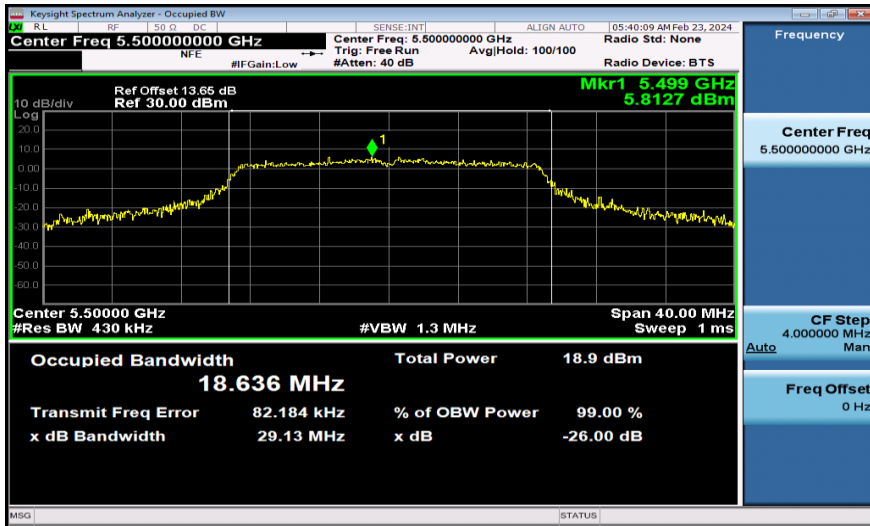
11AC20MIMO-Ant1-5500
