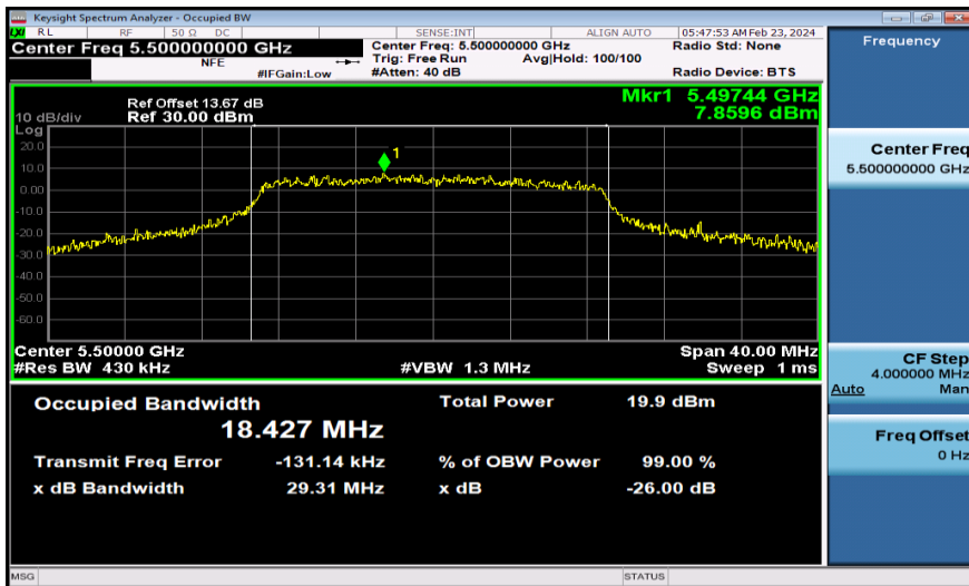
11AC20MIMO-Ant2-5500
