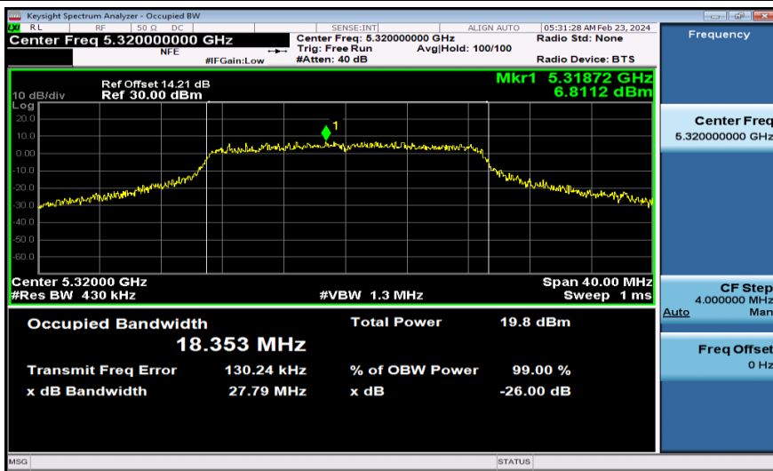
11AC20MIMO-Ant2-5320
