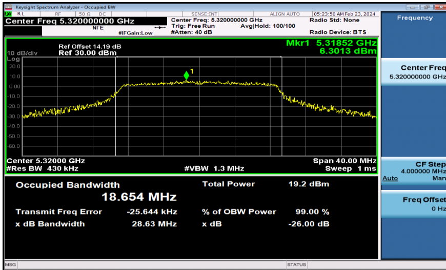
11AC20MIMO-Ant1-5320
