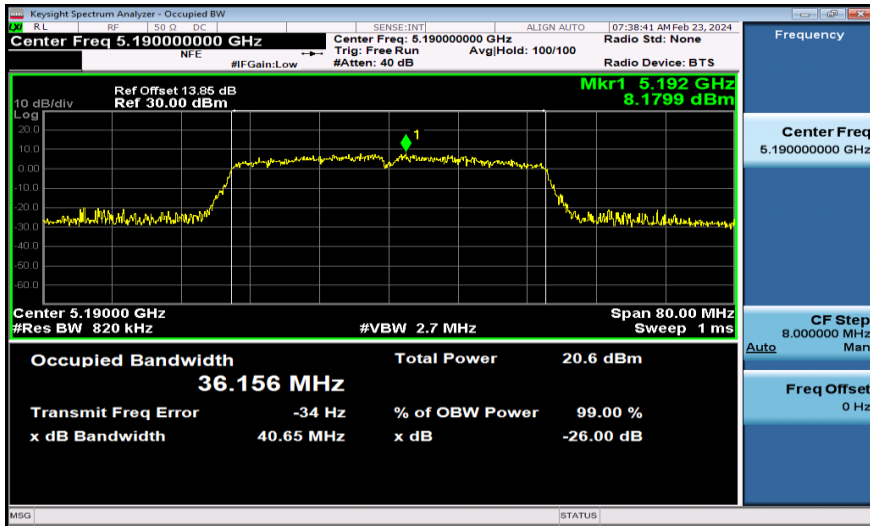
11AC40MIMO-Ant2-5190
