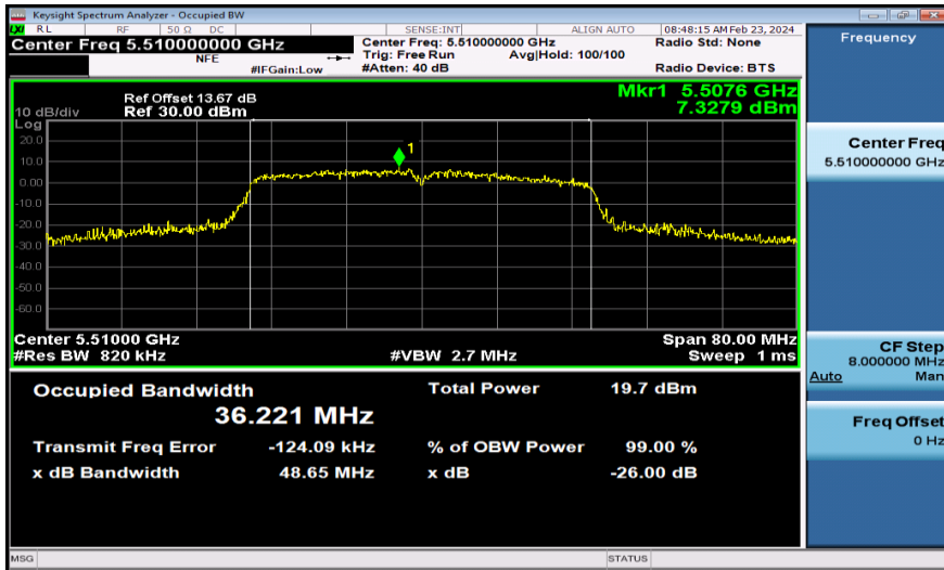
11AC40MIMO-Ant2-5510
