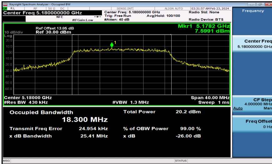
11AC20MIMO-Ant2-5180
