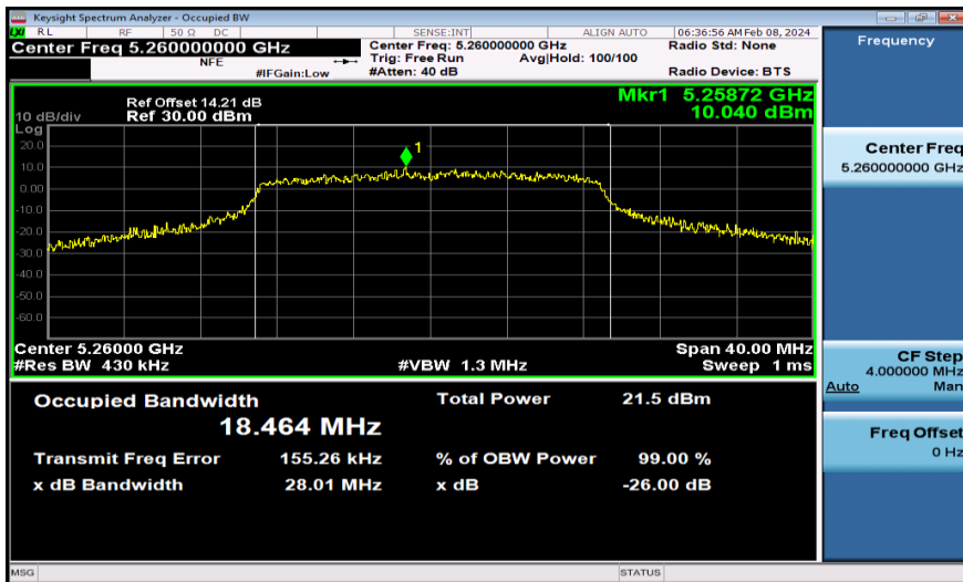
11N20MIMO-Ant2-5260
