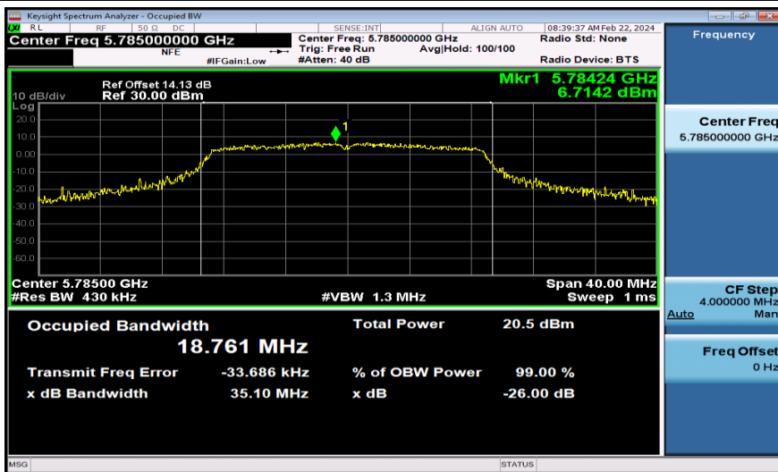
11N20MIMO-Ant1-5785
