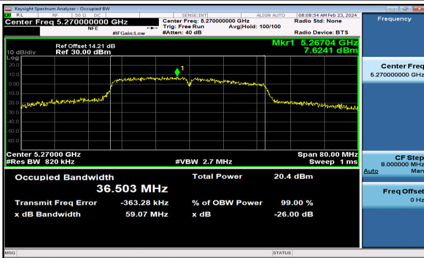
11AC40MIMO-Ant2-5270
