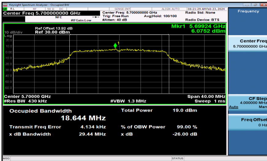
11AC20MIMO-Ant1-5700
