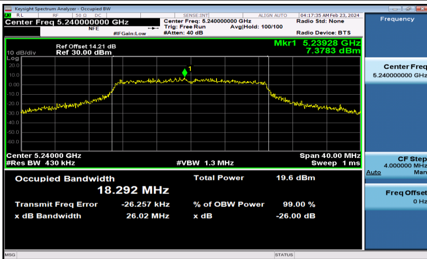
11AC20MIMO-Ant2-5240
