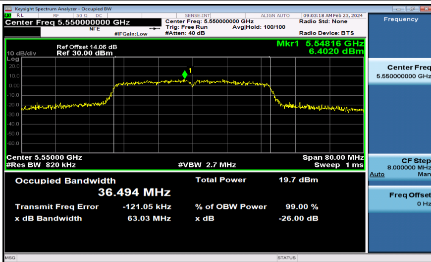
11AC40MIMO-Ant2-5550
