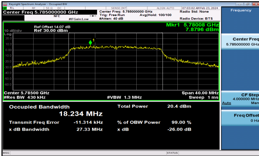
11AC20MIMO-Ant2-5785
