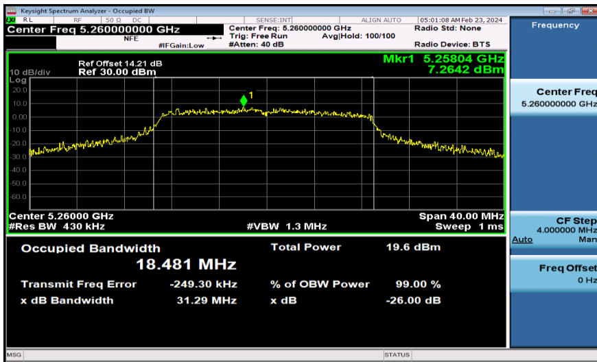
11AC20MIMO-Ant2-5260
