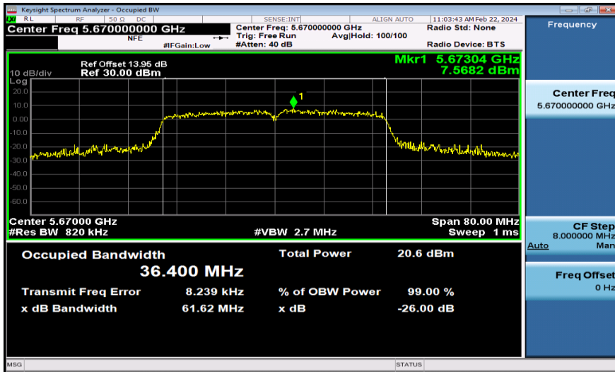
11N40MIMO-Ant2-5670
