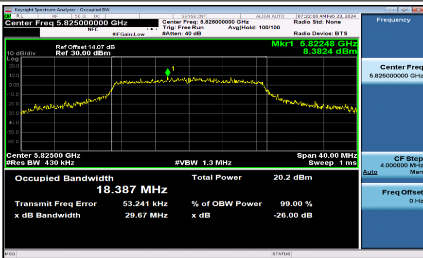
11AC20MIMO-Ant2-5825
