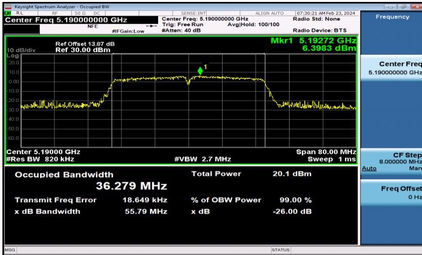
11AC40MIMO-Ant1-5190
