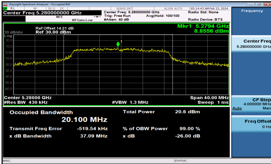
11AC20MIMO-Ant2-5280
