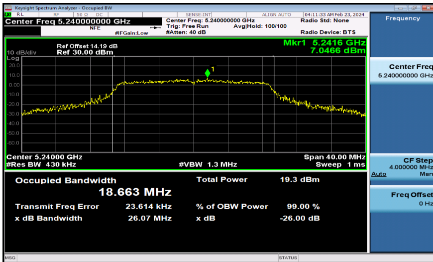
11AC20MIMO-Ant1-5240
