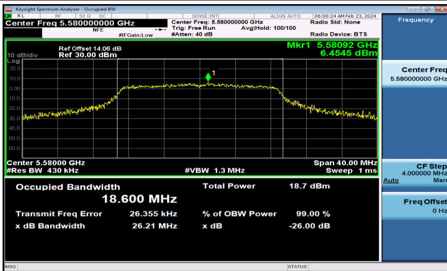
11AC20MIMO-Ant1-5580
