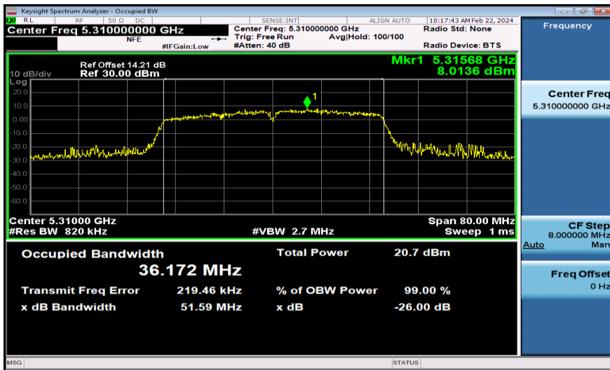
11N40MIMO-Ant2-5310
