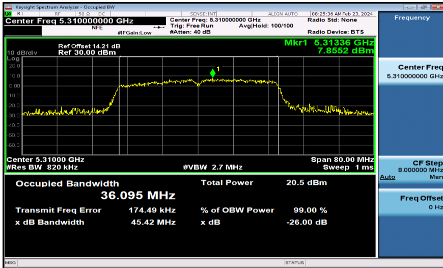
11AC40MIMO-Ant2-5310
