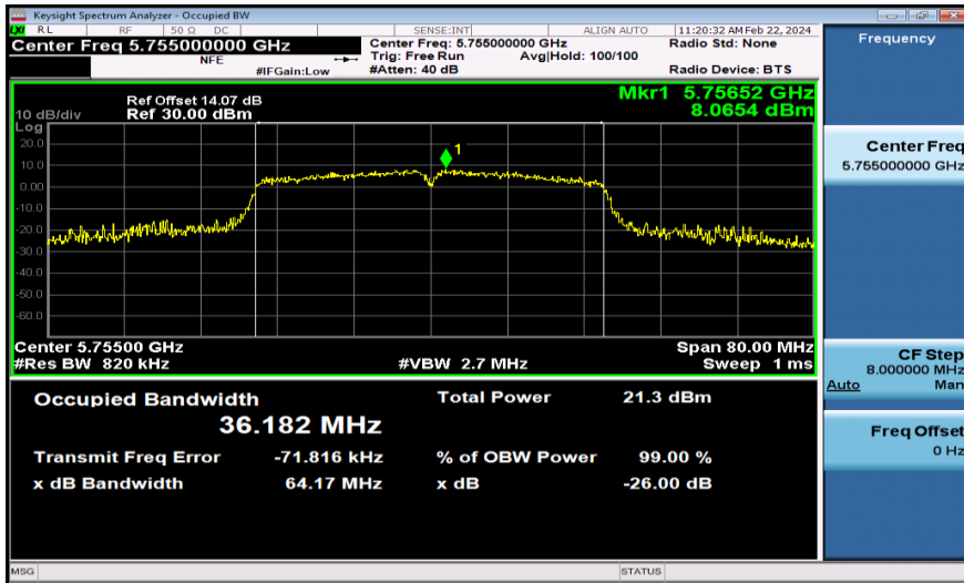
11N40MIMO-Ant2-5755
