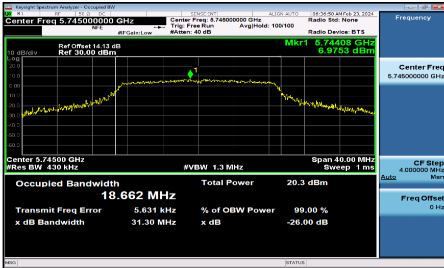
11AC20MIMO-Ant1-5745
