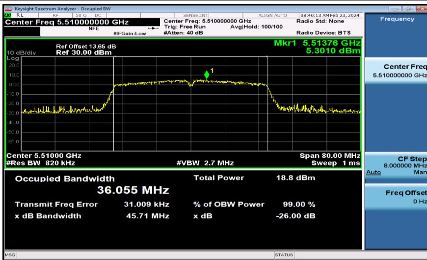
11AC40MIMO-Ant1-5510
