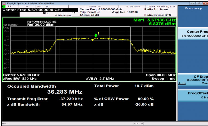
11N40MIMO-Ant1-5670
