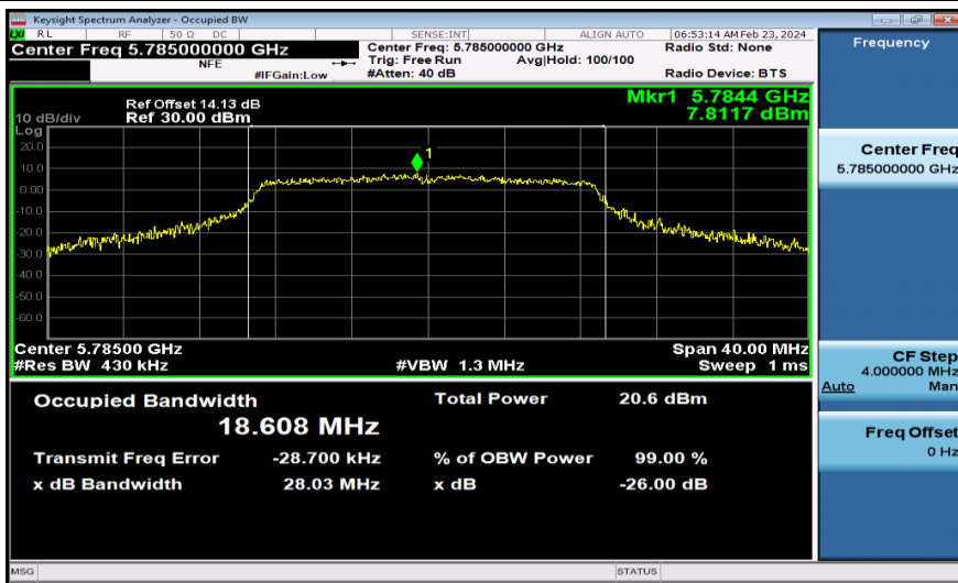
11AC20MIMO-Ant1-5785
