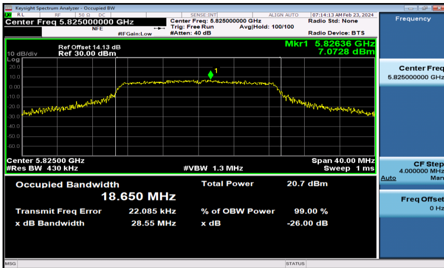
11AC20MIMO-Ant1-5825
