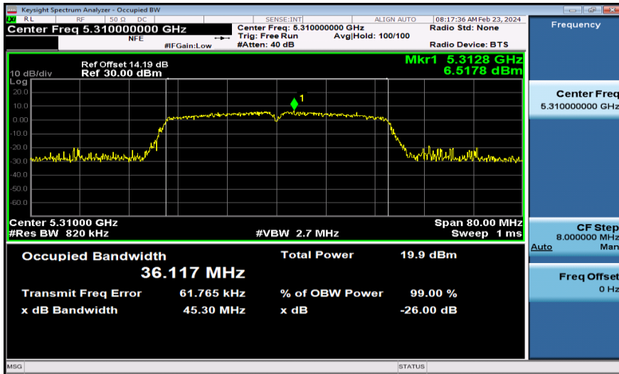
11AC40MIMO-Ant1-5310
