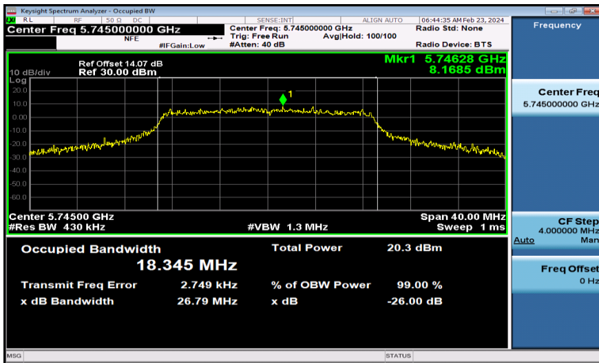
11AC20MIMO-Ant2-5745
