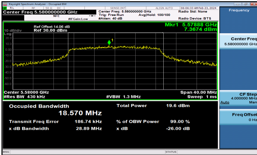
11AC20MIMO-Ant2-5580
