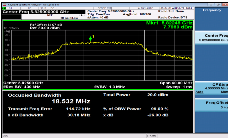
11N20MIMO-Ant2-5825
