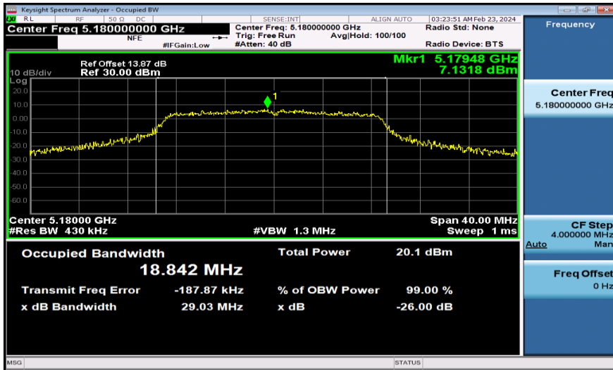
11AC20MIMO-Ant1-5180
