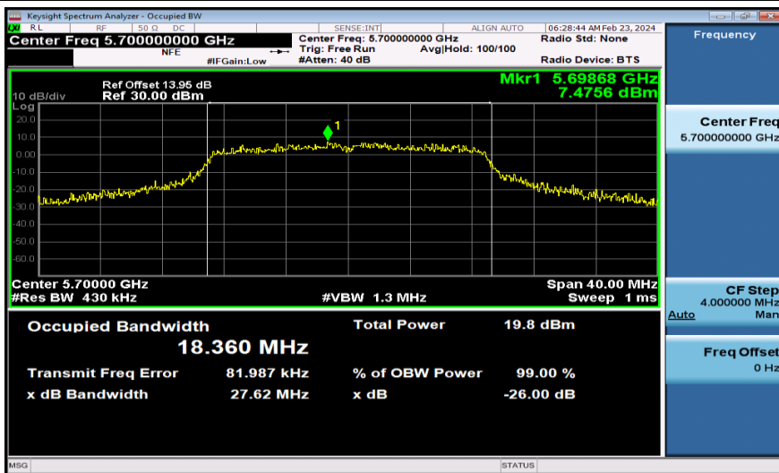
11AC20MIMO-Ant2-5700
