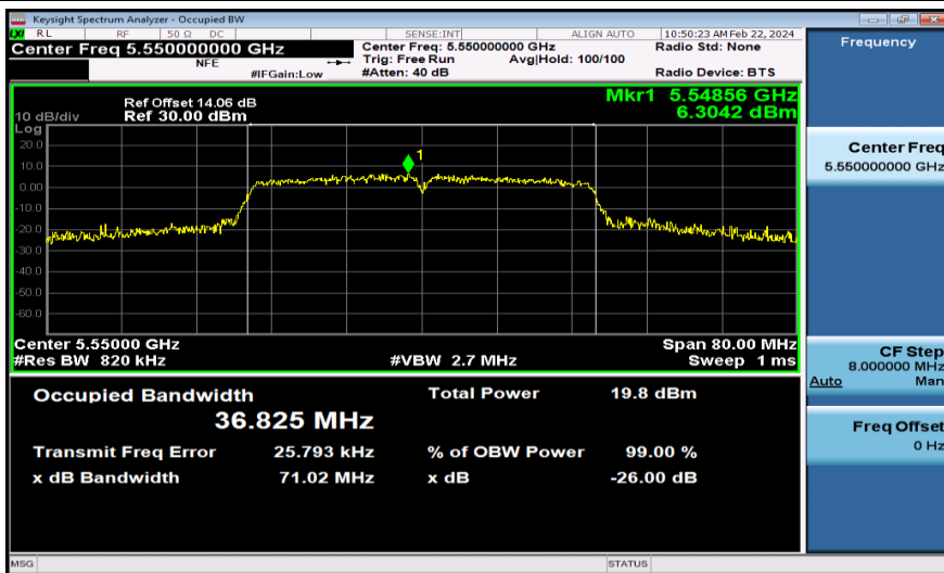
11N40MIMO-Ant2-5550
