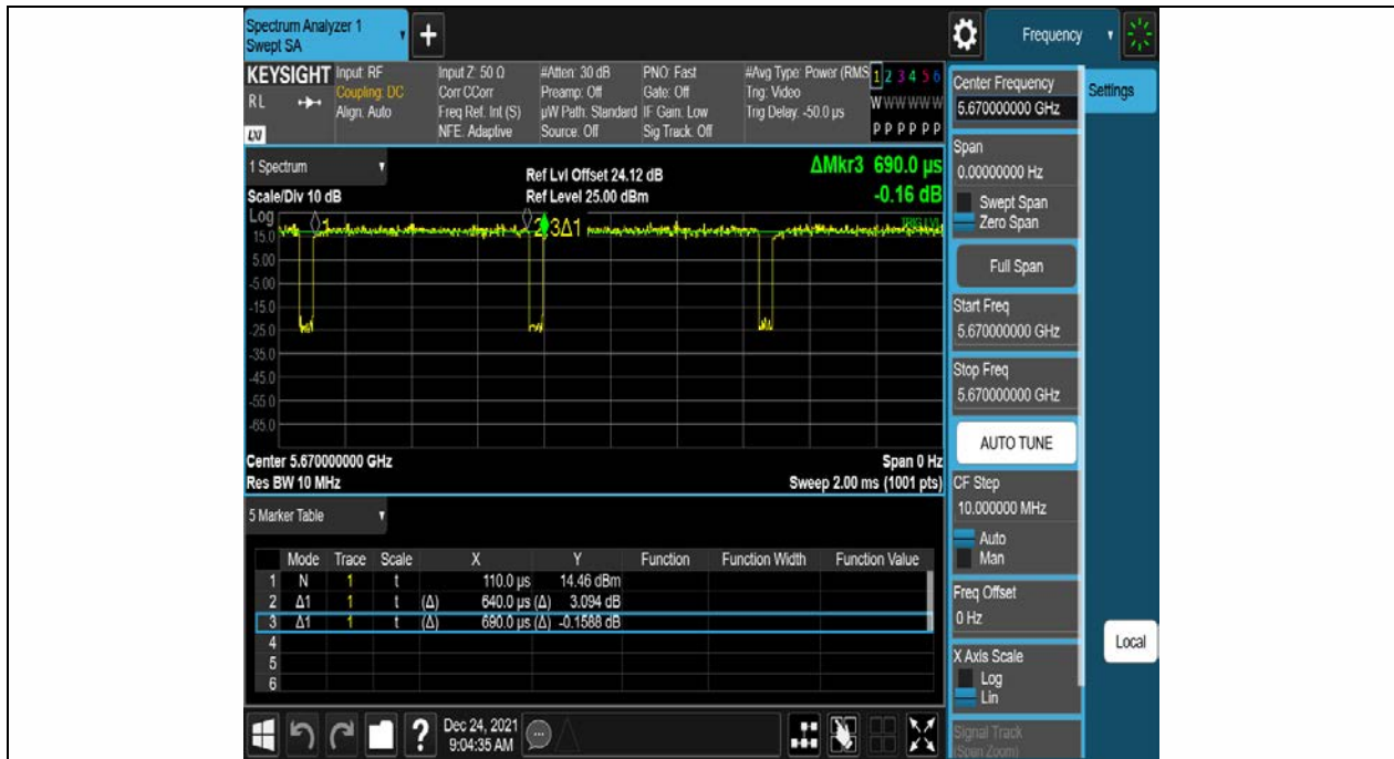
11N40SISO_Ant1_5670
