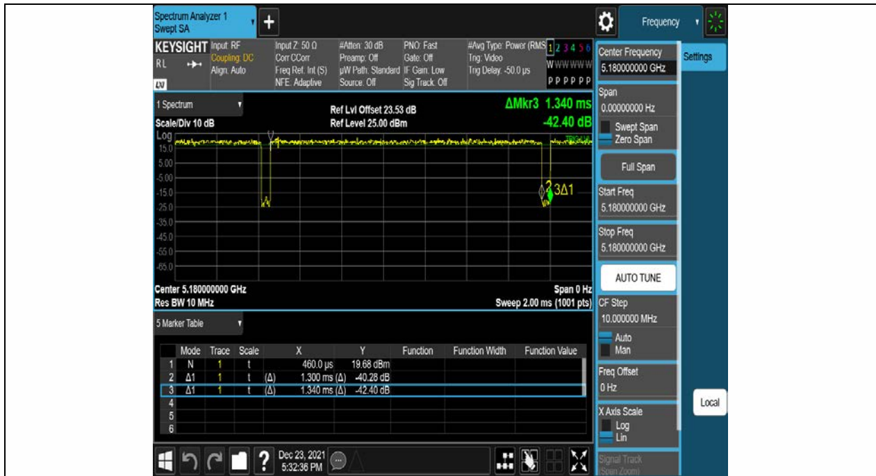
11N20SISO_Ant1_5180
