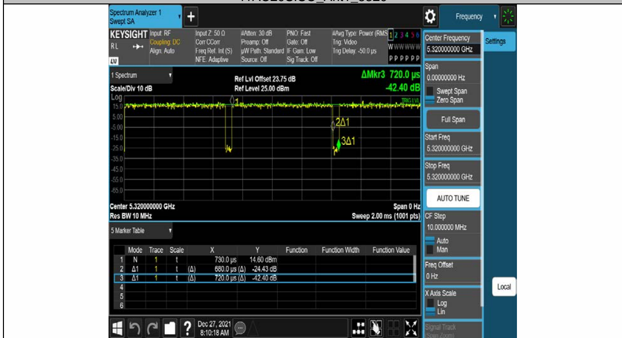
11AC20SISO_Ant2_5320
