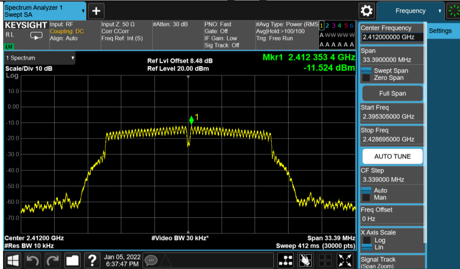
Wi-Fi 802.11 g mode, 6 Mbps
