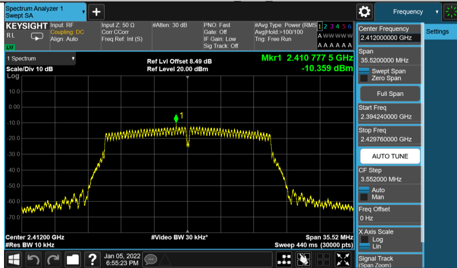
Wi-Fi 802.11 n20 mode, MCS0 Mbps
