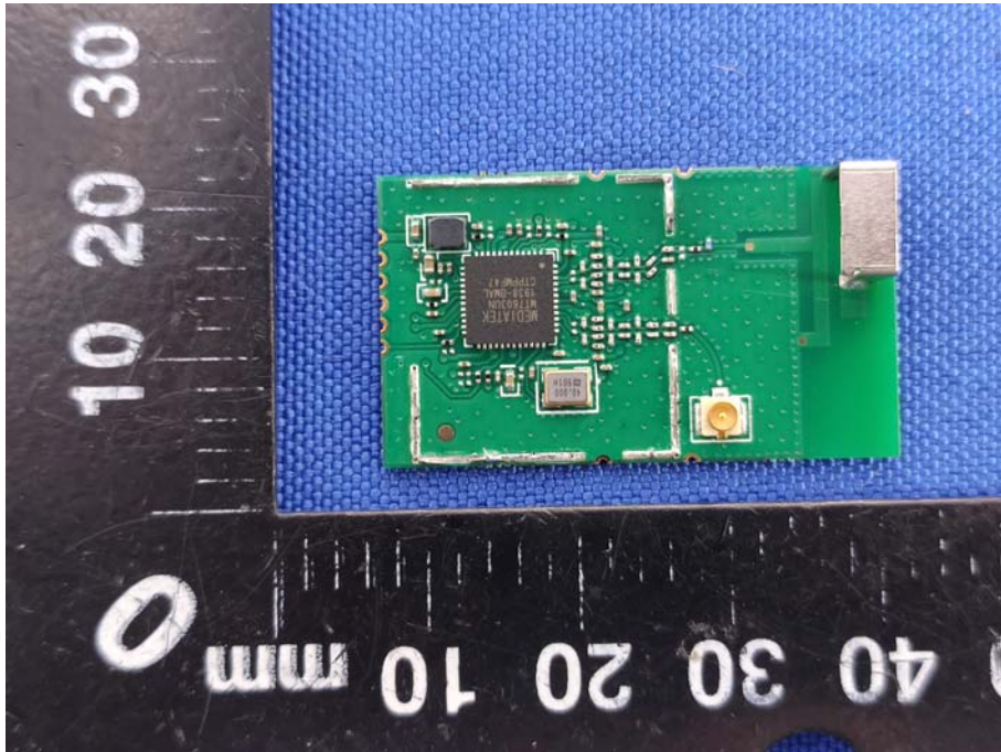
Product: WiFi Module Model: WF-M603-USB1 Internal Photos
