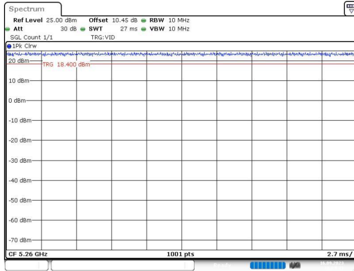
11N20SISO_Ant2_5260
