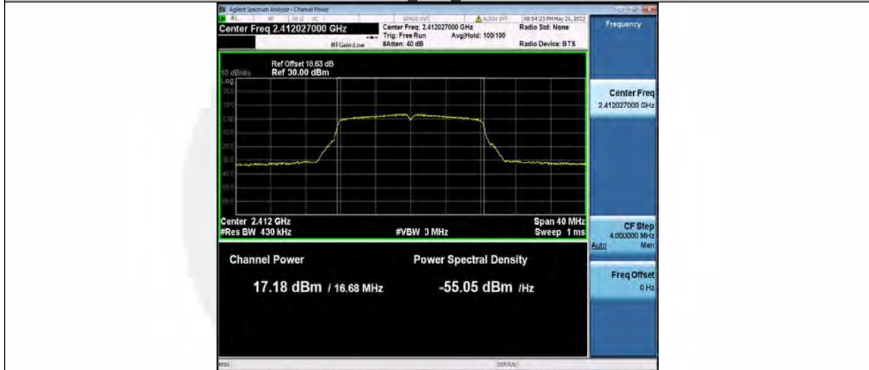
11G Ant2 2412
