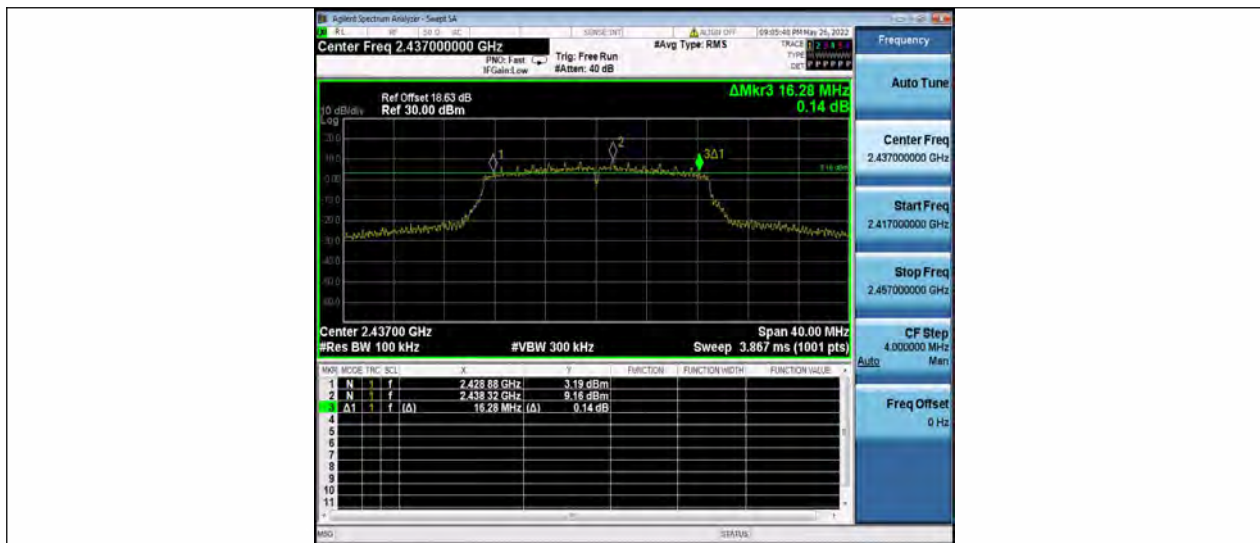
11N20SISO Ant2_2437
