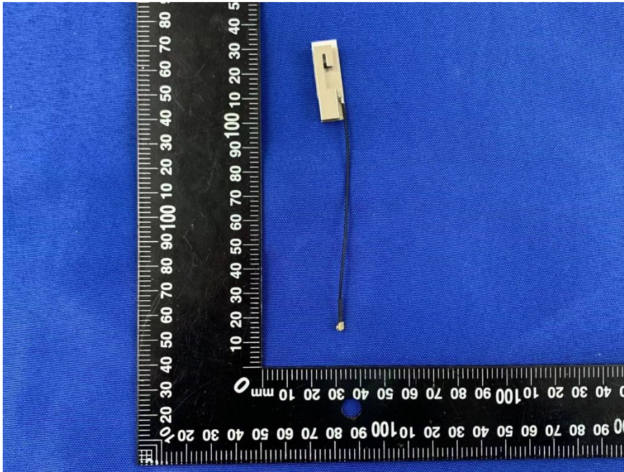
PIFA ANTENNA-85mm
